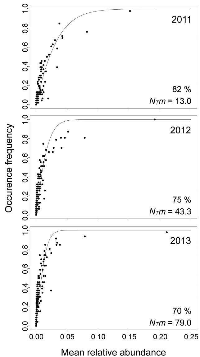
Figure 16 Relationship between the detection frequency of T-RFs and their mean relative abundance from the three years of monitoring. Each point represents a T-RF. The lines show the best fit to the neutral model with random immigration from a common source pool as described by Sloan and colleagues (2006). N_T m values represent the meta-community size multiplied by the immigration rate. Percentage represents R^2 of fit.
