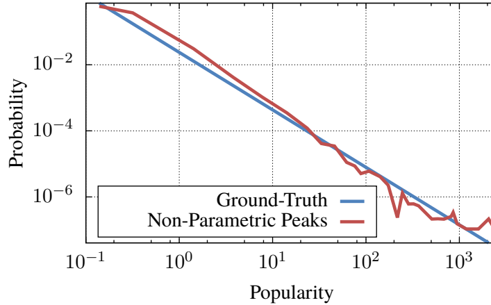
Figure 4.7: Estimation of the mixing distribution by the peak selection method
