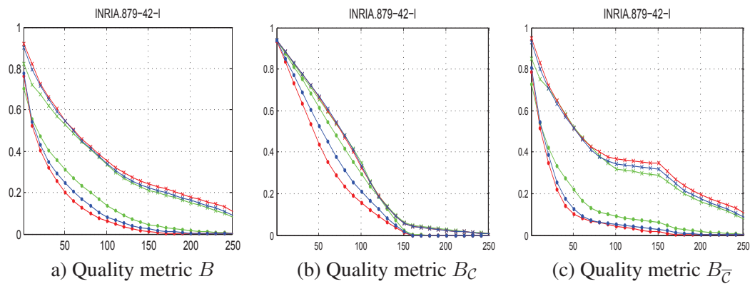
Figure 5.3: Results of crowd density estimation for different test videos from top to bottom: PETS S1.L1.13-57 V1, PETS S1.L1.13-9 V1, PETS S1.L2.14-31 V1, PETS S2.L3.14-41 V1, UCF-879, and INRIA.879-42-1. The results are in terms of bad pixels percentage, specifically, quality metric B in column a), B_C in column b), and B_{\bar{C}} in column c) and the x-axis corresponds to the density error tolerance that varies from 0 to 255. The results are shown for three different local feature types (FAST, SIFT, and GFT), and the proposed approach using feature tracks is also compared to GMM foreground segmentation. This results in 6 curves in each chart.
