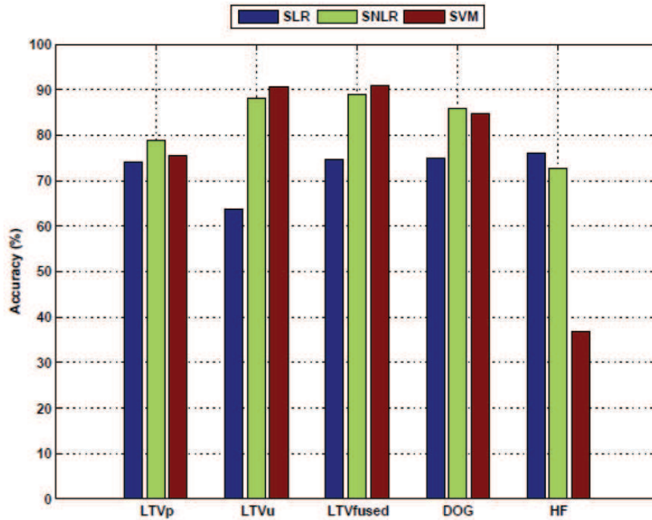
Figure 3.4: Comparison of detection rates using SLR, SNLR, SVM as classifiers and LTVp, LTVu, LTVfused, DoG and HF as input features. This figure is taken from [131].
