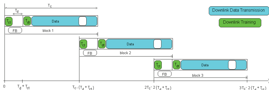
Figure 6.4: Foresighted Channel Feedback net DoF analysis.
