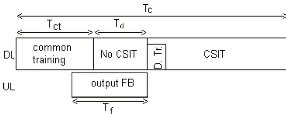
(b) Block topology for netDoF analysis.
