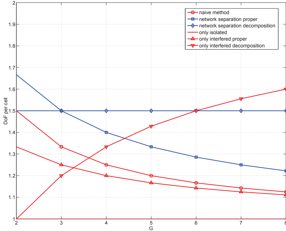
Figure 5.3: DoF per cell for different schemes.
