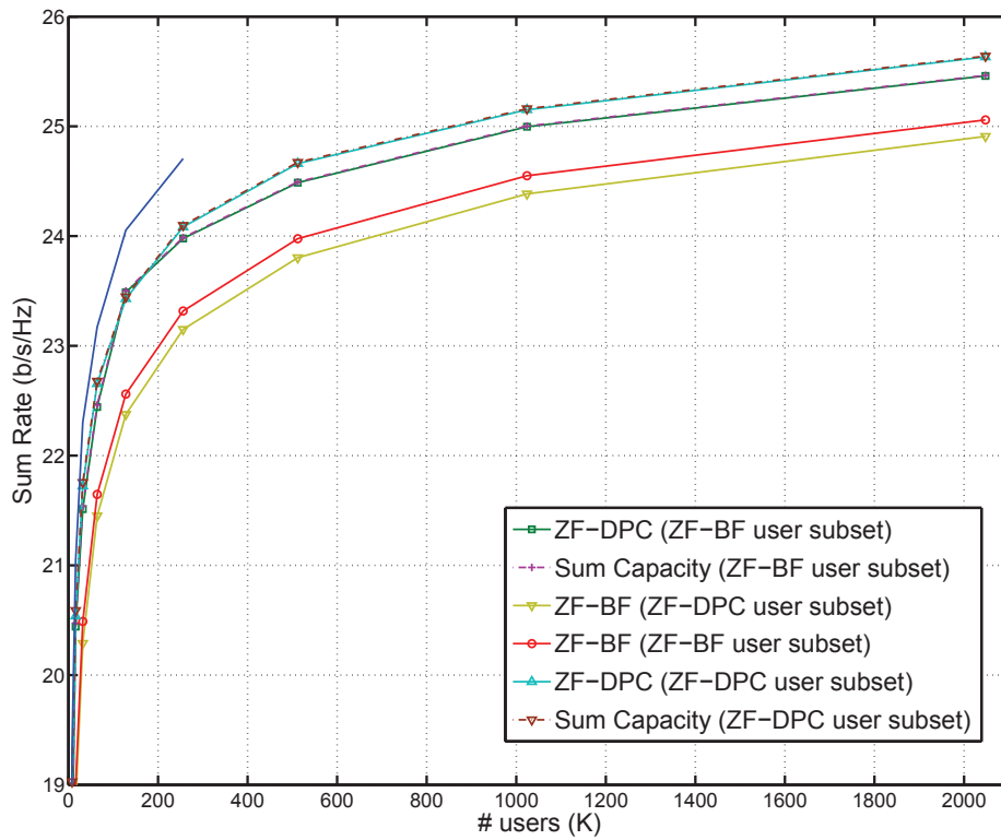
Figure 3.4: Sum rate offset between sum capacity, ZF-DPC, and ZF-BF for user subset selected for ZF-BF by the approximate criterion and ZF-DPC and ZF-BF for a user subset selected for ZF-DPC and the sum capacity for all users in the MISO BC with N_t=4 , \text{SNR}=15 dB.
