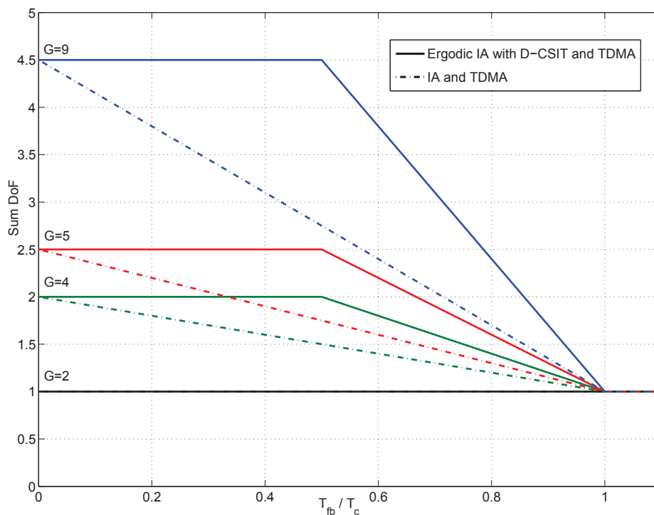
Figure 8.3: Feedback delay-DoF tradeoff in the SISO IC.
