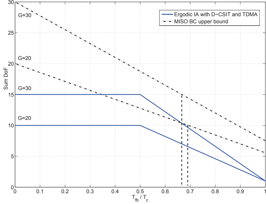
Figure 8.4: MISO BC upper bound.
