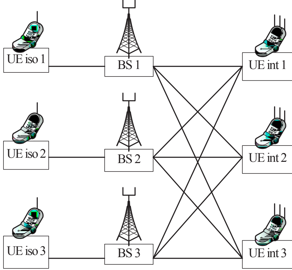
Figure 5.1: Considered configuration of partially connected IBC for G = 3 .
