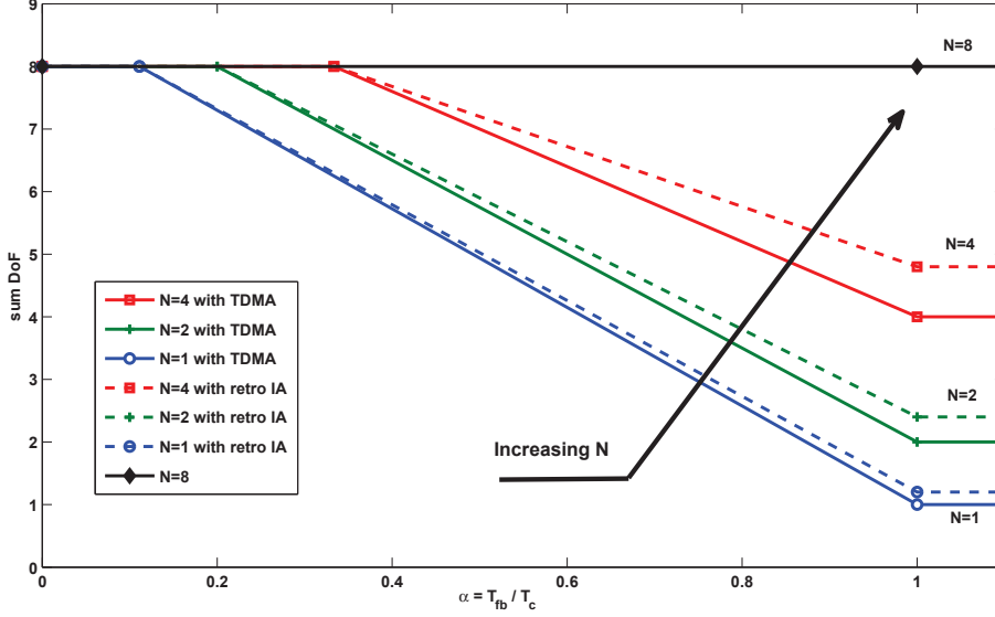
Figure B.1: Time sharing between STIA and TDMA or retrospective IA in the IC for M = 8 .
