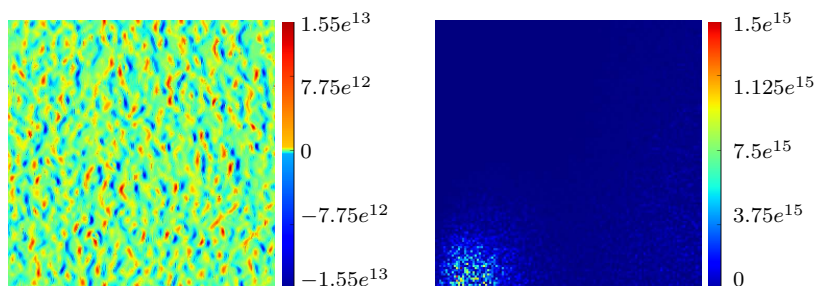
Figure 3.10: Left: snapshot of GND density field \kappa at \tilde{t} = 347 (figure 3.9). Right: Amplitude map of the corresponding Fourier transform.
