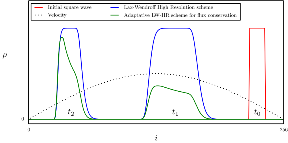
Figure 3.4: Movement of a square wave of dislocation density shifting on the left with a non-constant velocity inside a 1D periodic grid with 256 nodes. Both simulations are performed with \Delta t = 2.6 \cdot 10^{-1} \Delta t_{crit} . The snaps at t_1 and at t_2 are taken respectively at the iteration 440 and 880.
