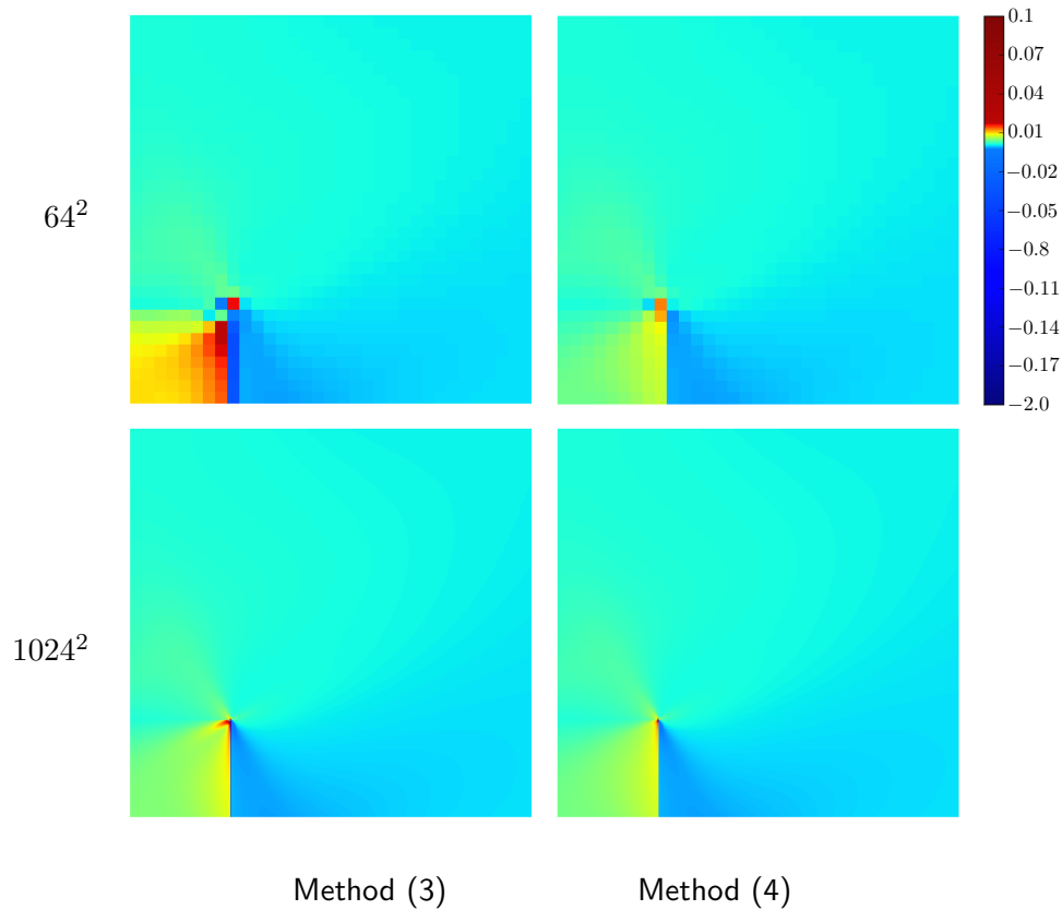
Figure 4.7: Maps of \epsilon_{11} , containing a quarter of the periodic system with the middle of the precipitate matching with the corner of the figure. Above: 64-run. Below: 1024-run. Left: method (3). Right: method (4).
