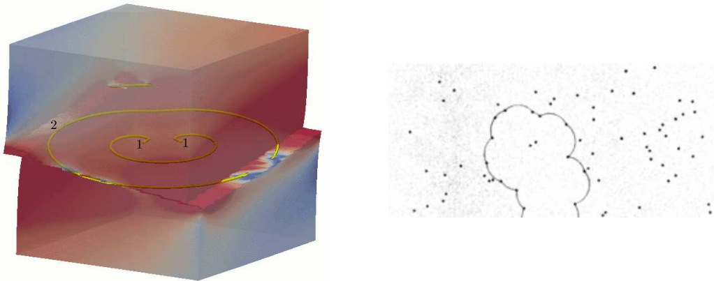
Figure 4.9: On the left: Illustration of a perfect Frank-Read source inside a shear load simulation, after [29]. On the right: Illustration inside the plane of a curved dislocation of its movement through a forest of dislocations, after [34].
