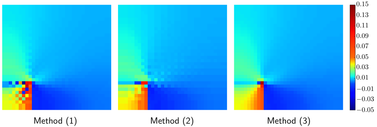
Figure 4.6: Maps of \epsilon_{11} (64-run) for each method, containing a quarter of the periodic system with the middle of the precipitate matching with the corner of the figure.
