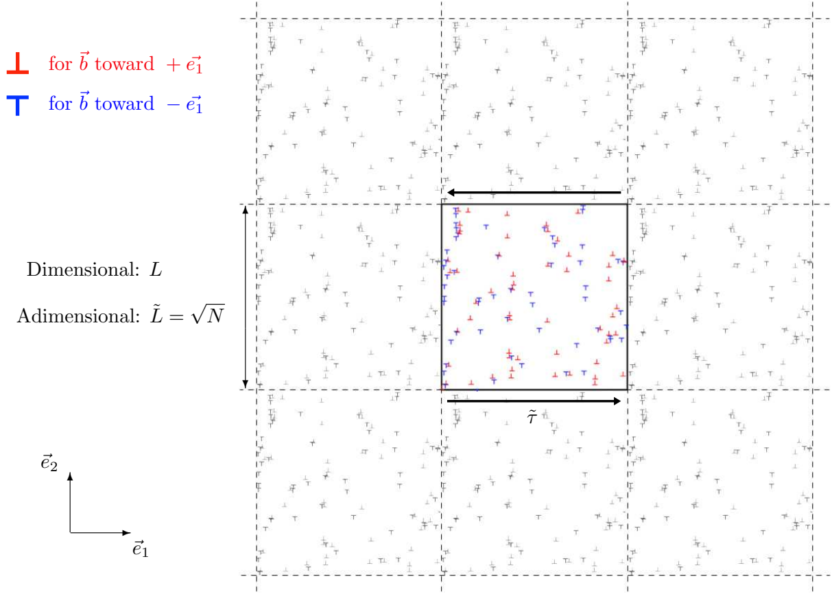
Figure 2.1: Example of a pseudo-periodic simulation with imposed shear stress \tilde{\tau} = 1 , with 50 positive dislocations in red and 50 negative dislocations in blue.
