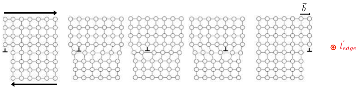
Figure I.3: Translation from the left to the right of an edge dislocation due to a shear load of the cubic lattice symbolized by two black pointers.
