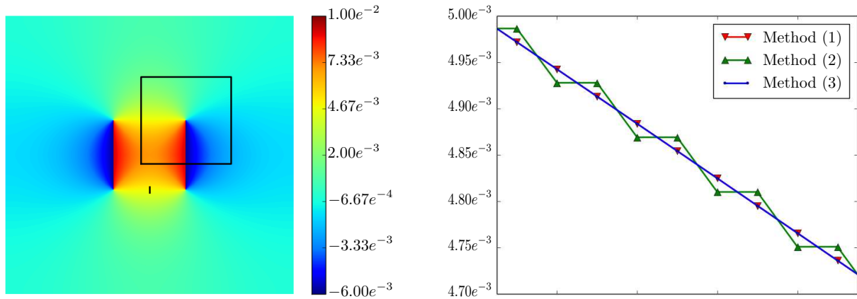
Figure 4.3: On the left: Map of \epsilon_{11} (Method (1)) with the localisation of the profil (black line) and the localisation of figure 4.4 (black square). On the right: Profil of \epsilon_{11} through the interface for each method.
