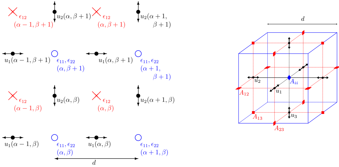
Figure 4.1: Staggered grids for mechanical fields in 2D on the left and in 3D on the right.
