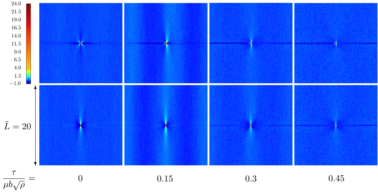
Figure 2.10: Correlation maps of size L \times L , averaged on a 256 \times 256 grid and for different applied stresses. Simulations are performed with N^+ = N^- = 200 , r_{co} = 2 and \Delta \tilde{t} = 10^{-4} . Top row: the function d^{+-}(\vec{r}) . Bottom row: the function d^{++}(\vec{r}) .
