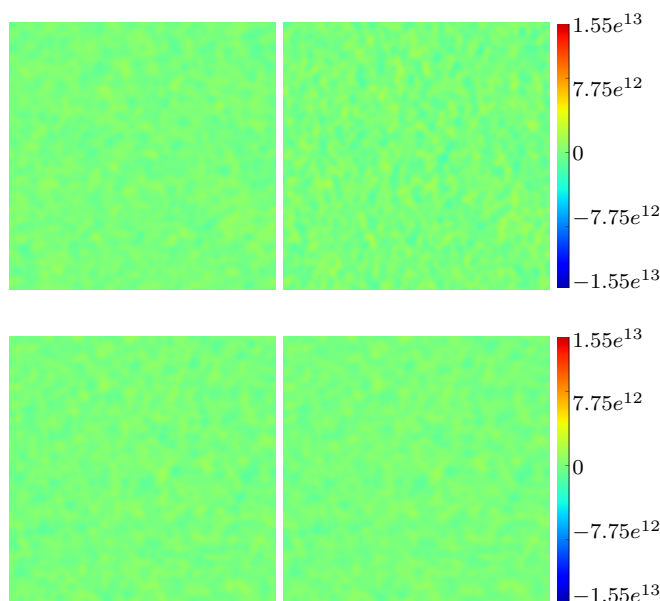
Figure 3.11: Initial configuration (left) and dislocations density fields at \tilde{t} = 347 (right) obtained with the mean field model. The top row displays \rho - \rho_0 and the bottom row \kappa . The applied stress is \tilde{\tau}_{ext} = 5.34 . The color scale is chosen to allow a direct comparison with Figure 3.9.
