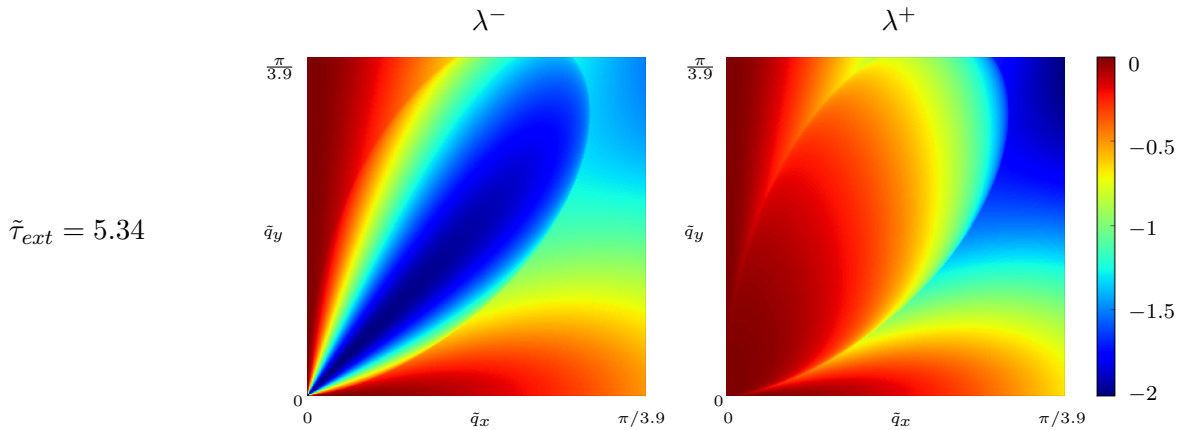
Figure 3.8: \Re(\lambda^-) (left) and \Re(\lambda^+) (right), vs the wavelength \tilde{q} of the perturbations for an applied stress \tilde{\tau}^{ext} = 5.34 .
