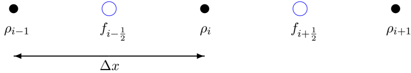
Figure 3.5: Grid along \vec{x} with the localization of the flux f between 2 nodes of the main grid.
