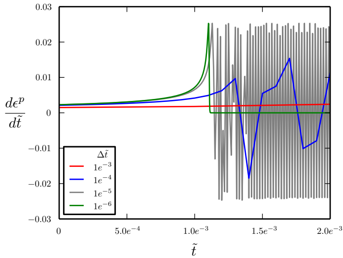
Figure 2.4: Evolution of the strain rate function of the time for different time discretization.
