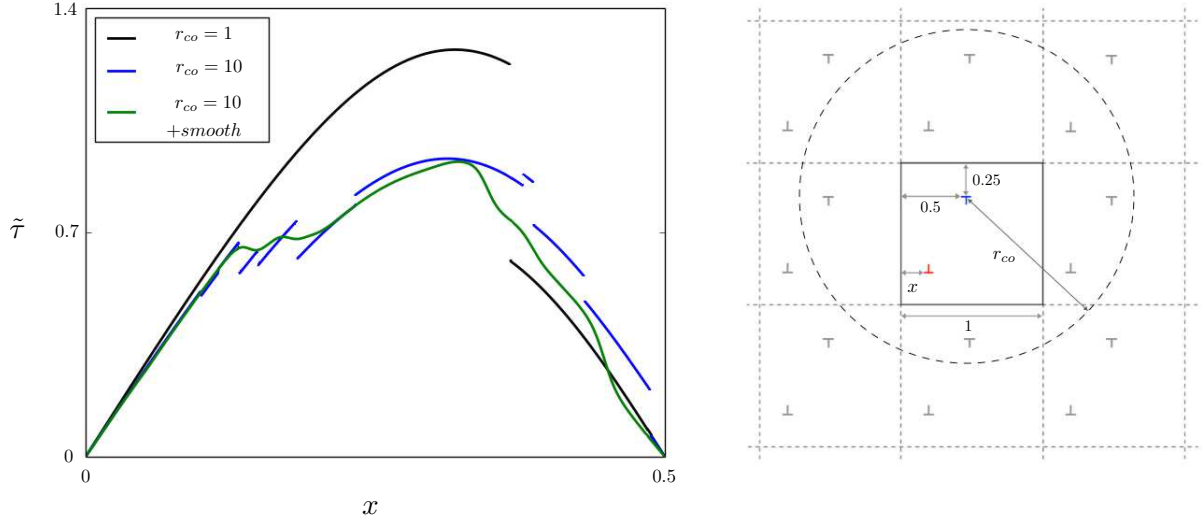
Figure 2.6: Stress received by the blue dislocation when the red dislocation moves. The right side shows the scheme of the pseudo-periodic system involving a cut-off and the left side shows the stress received function of \tilde{x} . Distances are indicated in units of the box size. A_s is equal to 5 \cdot 10^{-2} .
