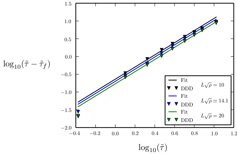
Figure 3.1: Symbols: Numerical estimation of \tau - \tau_f , coming from section 2.3.2 for three different values of L\sqrt{\rho} . Lines: corresponding fit using a power law with an exponent \alpha = 1.71 .
