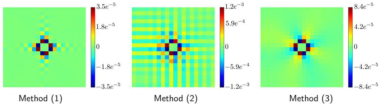
Figure 4.4: Difference between \epsilon_{11}^{(64)} (64-run) and \epsilon_{11}^{(1024)} (1024-run averaged on a 64 \times 64 grid) for each method. Only one corner of the precipitate is exhibited, localized by the square in figure 4.3.
