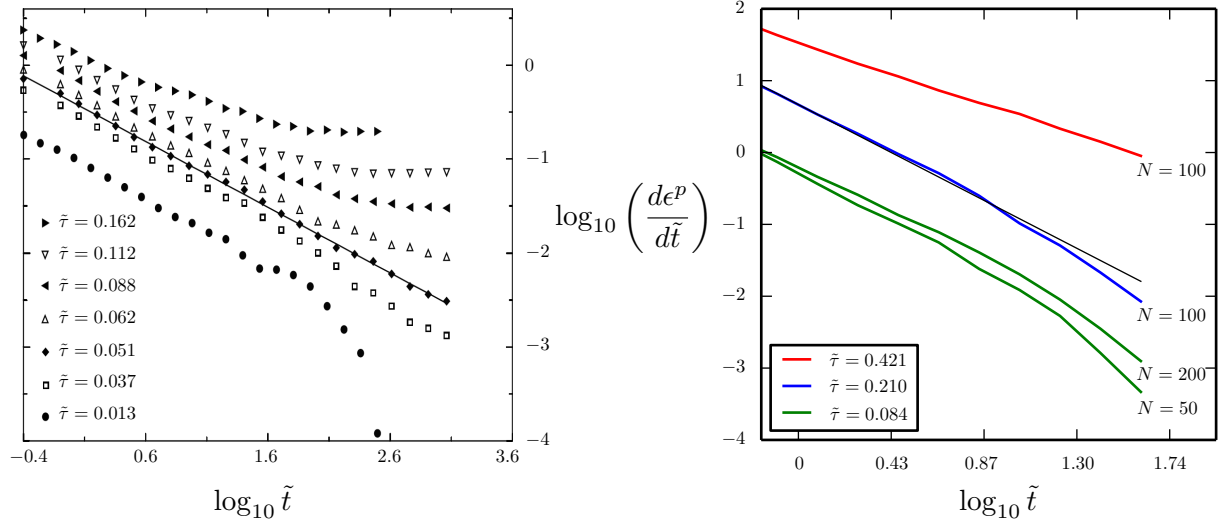
Figure 2.8: The averaged strain-rate of a high quantity of distributions during the relaxation for different applied stresses. The left investigation with 400 dislocations is performed by [77] with reviewed scales. The right side is a new investigation with a pseudo-periodic system describe previously involving different number of dislocations: N=50 , N=100 or N=200 . Our averaged strain-rate is obtained with 10^3 distributions.
