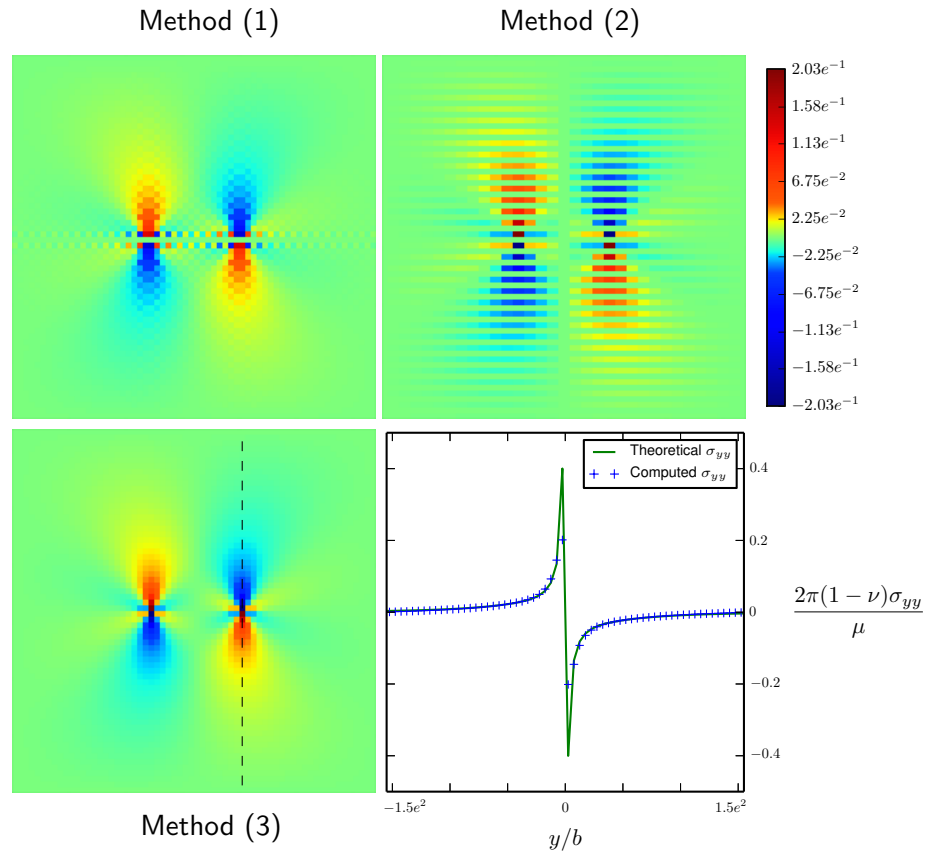
Figure 4.5: Fields of 2\pi(1-\nu)\sigma_{yy}/\mu computed in a box with 64 \times 64 nodes. The three maps are, in the order, obtained by method (1), (2) and (3). The two dislocations are positioned at (23, 31) and (39, 31) . The profil, coming from the method (3) and illustrated by the dotted line on the third map, is compared to the analytical solution.
