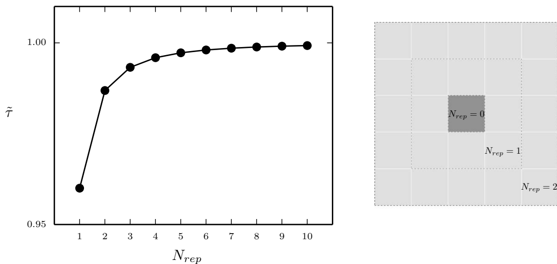
Figure 2.5: Stress jump due to the pseudo-periodicity. The right side shows the system for different N_{rep} and the left side shows the value of the stress jump depending on N_{rep} .
