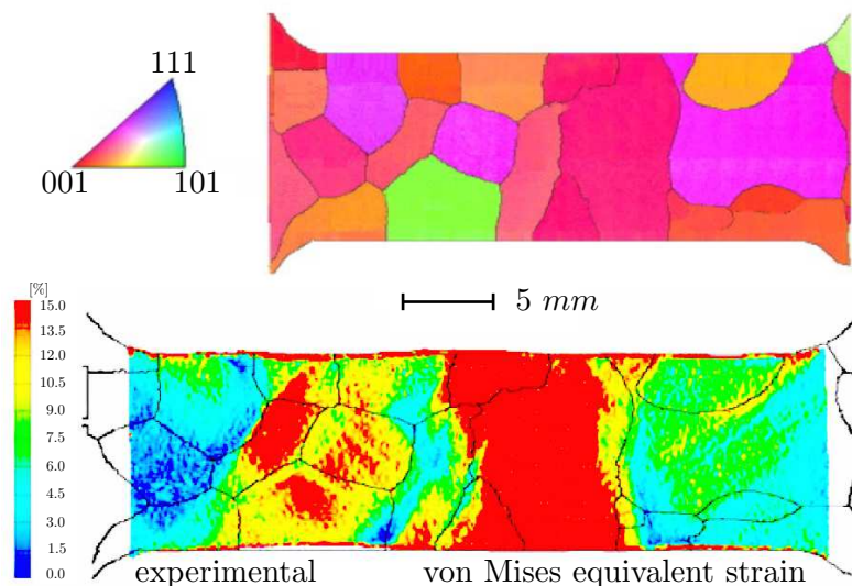
Figure I.5: Tensile test response of a polycrystal of aluminium: Above, The lattice orientation of each phase of the microstructure. Below, the inter-phases pattern of plasticity. The fluctuations of dislocation density are obtained by the DIC technique. After [112].
