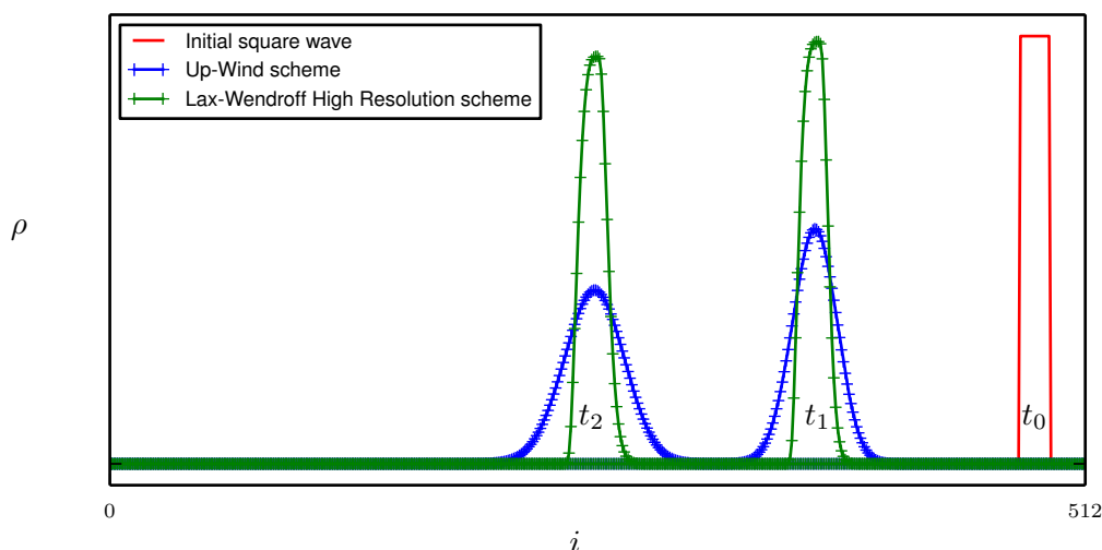
Figure 3.3: Movement of a square wave of dislocation density shifting on the left inside a 1D periodic grid with 512 nodes. Comparison between the Up-Wind scheme in blue and Lax-Wendroff High-Resolution scheme in green. Both simulations are performed with \Delta t = 2.6 \cdot 10^{-2} \Delta t_{crit} . The snapshots at t_1 and at t_2 are taken respectively at the iteration 4400 and 8800.
