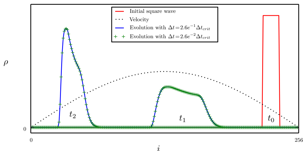
Figure 3.6: Movement of a square wave of dislocation density shifting on the left with a non-constant velocity inside a 1D periodic grid with 256 nodes. The snaps at t_1 and at t_2 are taken respectively at the iteration 440 and 880 for the blue curve and at the iteration 4400 and 8800 for the green curve.
