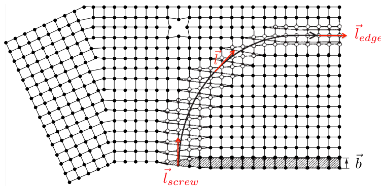
Figure I.1: Illustration of crystal defects in a crystal: On the left, there is an interface ( dim. 2) between two phases with different orientations. On the top, there is a vacancy ( dim. 0). On the right, there is a portion of dislocation loop ( dim. 1) enclosing an area sheared by an elementary translation \vec{b} , the Burgers vector. \vec{l} is the dislocation line vector. Drawing inspired by [86].
