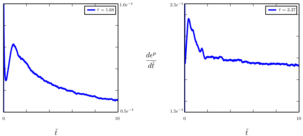
Figure 2.9: The averaged strain-rate of 10^3 distributions during the relaxation for two high applied stresses \tilde{\tau} = 1.68 and \tilde{\tau} = 3.37 with N = 100 .
