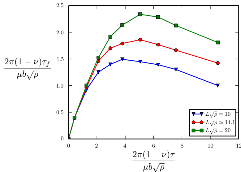
Figure 2.11: Numerical results of the friction term \tau_f depending on the applied stress and the period.
