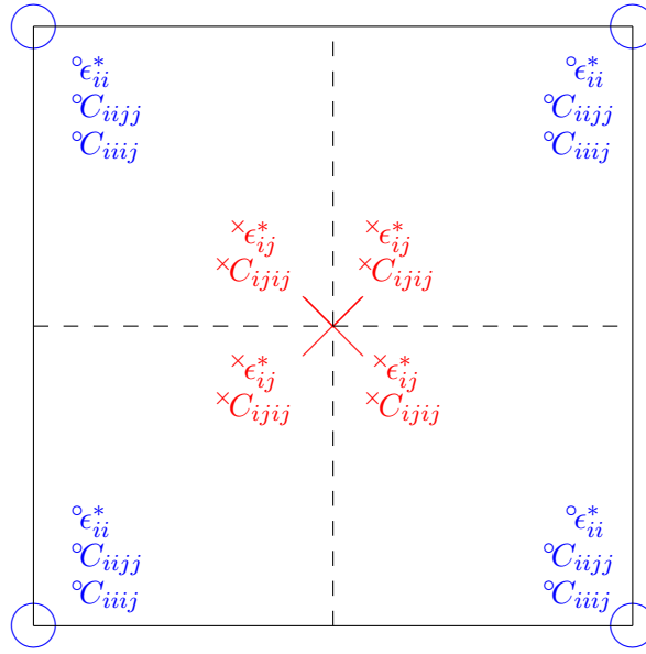
Figure 4.2: One voxel containing four sub-voxels with homogeneous elastic energy with the illustrated eigenstrain and stiffness tensors decomposition.
