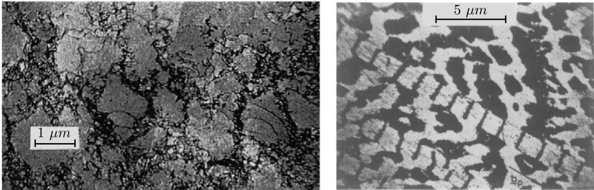
Figure I.4: Dislocation-pattern of dislocations (black regions) in a monocrystal of copper at stage II of the strain hardening on the left and cycled at a strain amplitude in the plateau on the right. Revealed by typical transmission micrographs. Respectively after [64, 71].
