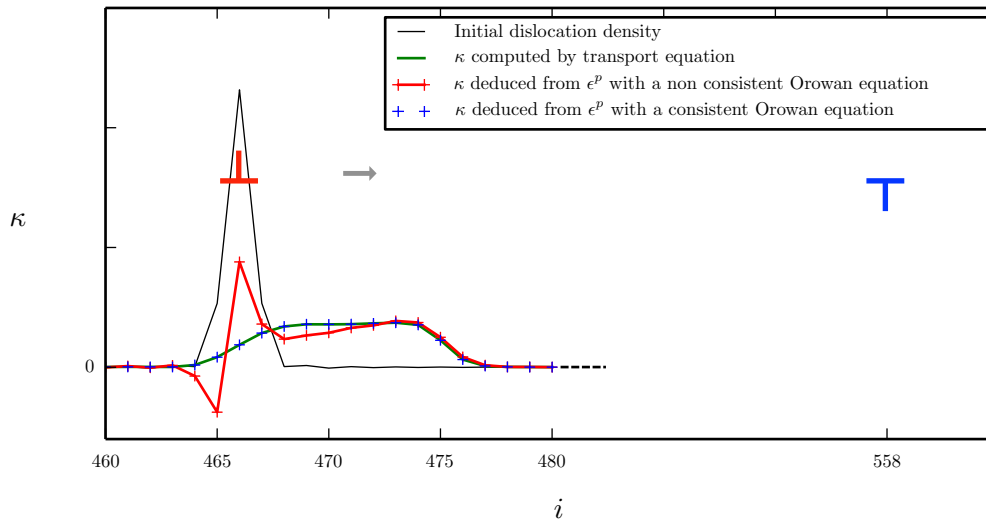
Figure 3.7: Simulation of a positive dislocation attracted by a negative dislocation inside a box of 1024 \times 64 nodes. Both dislocations are defined respectively by a bump of density of \rho^+ and \rho^- . The side of \rho^+ is represented here (equivalent behavior for \rho^- ): the initial state in black, the shifted state in green. The dot fields represent \kappa computed by the discrete Kröner equation: the red dots use a naive discretization and the blue dots use a consistent discretization.
