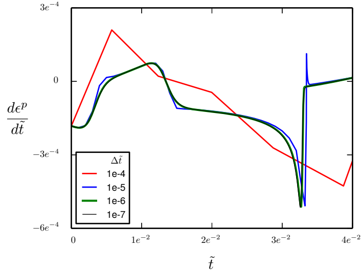
Figure 2.7: Relaxation of a random initial distribution with 100 dislocations and without external load: Strain rate of the distribution function of the time and depending on different discretization \Delta\tilde{t} . \delta\tilde{y}_{min} is equal to 10^{-2} .
