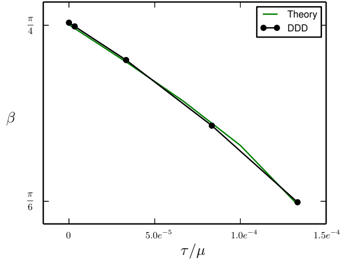
Figure 2.3: Evolution of the stationary position of a dipole of dislocations with opposite Burgers vector function of the external stress. The right side illustrate the system. The left side compare the approximation of a dipole in our pseudo-periodic system compared to the theory. The dipole size is \delta y = 3.9 \cdot 10^{-2} \cdot L .
