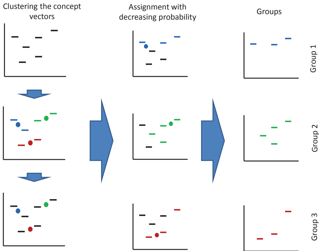
FIGURE 4.7: Clever grouping when the number of groups is less than the number of concepts.
