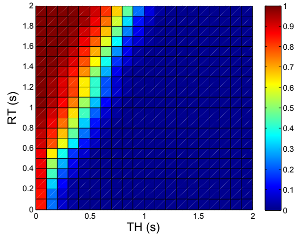
(a) \Omega_{Advice}^{Collision}(RT, FT)
