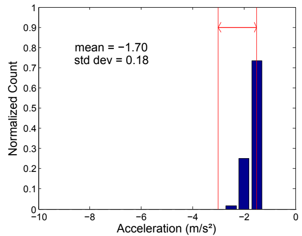
(f) Repartition of acceleration necessary to stop on time, using Model 2 in the case of advice assistance.
