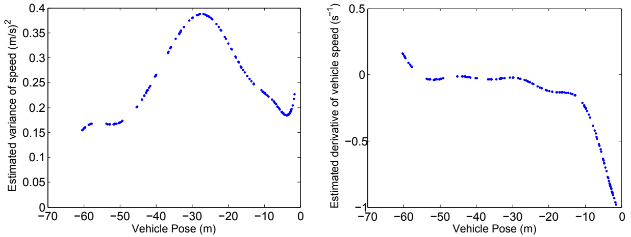
(a) Example of graphical representation of variance on vehicle speed function of vehicle pose ( r_j(x_j)^2 ). (b) Example of graphical representation of derivative of vehicle speed function of vehicle pose ( \delta_{y_j}(x_j) ).
