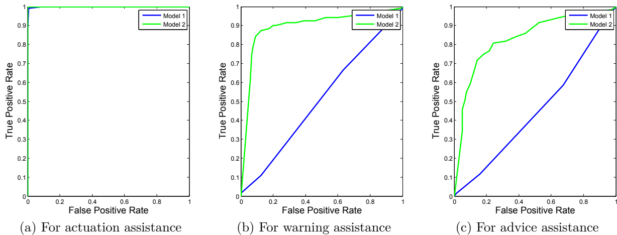
Figure 4.15: ROC curves
