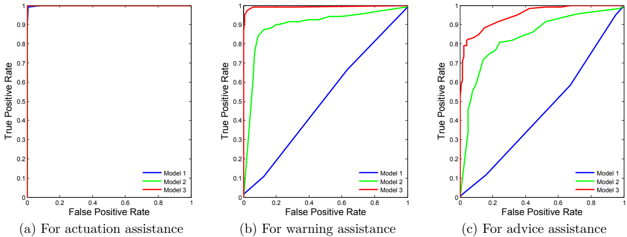
Figure 5.8: ROC curves
