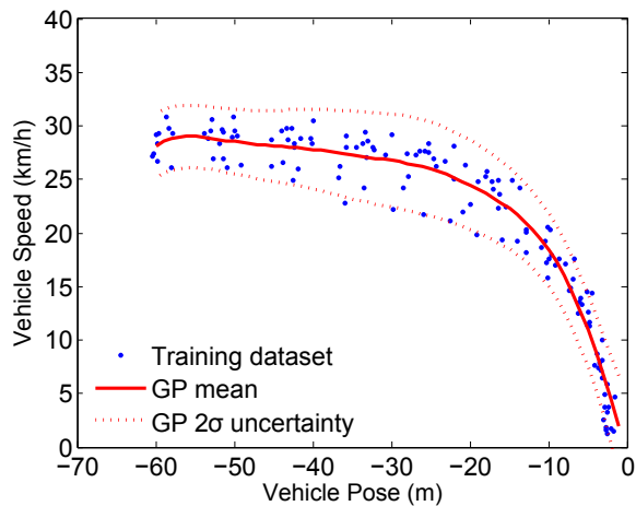
(c) Heteroscedastic Gaussian Process regression with noisy inputs.
