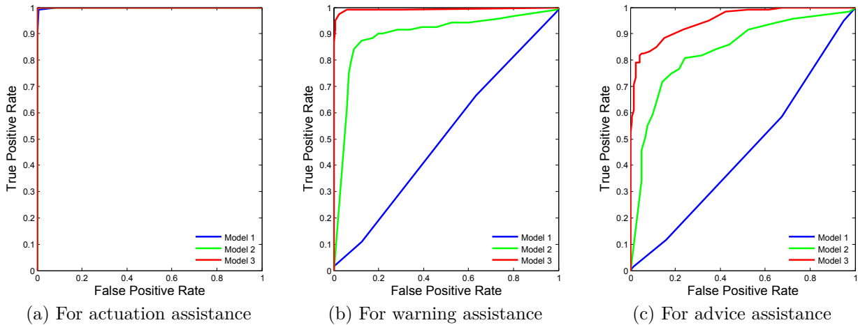
Figure 5.8: ROC curves
