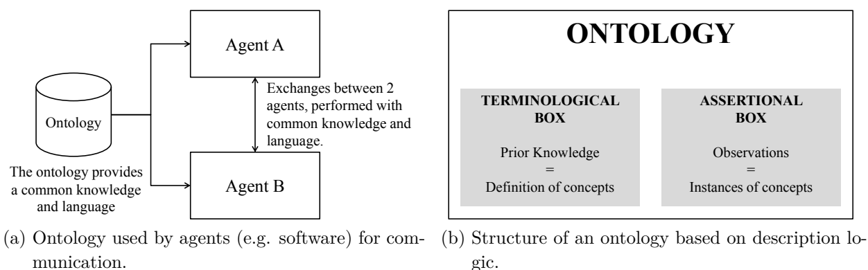
Figure 3.1: Ontology.
