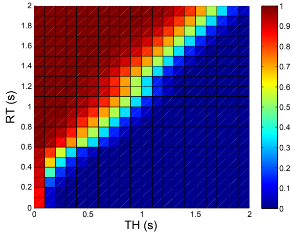
(a) \Omega_{Warning}^{Collision}(RT, TH)
