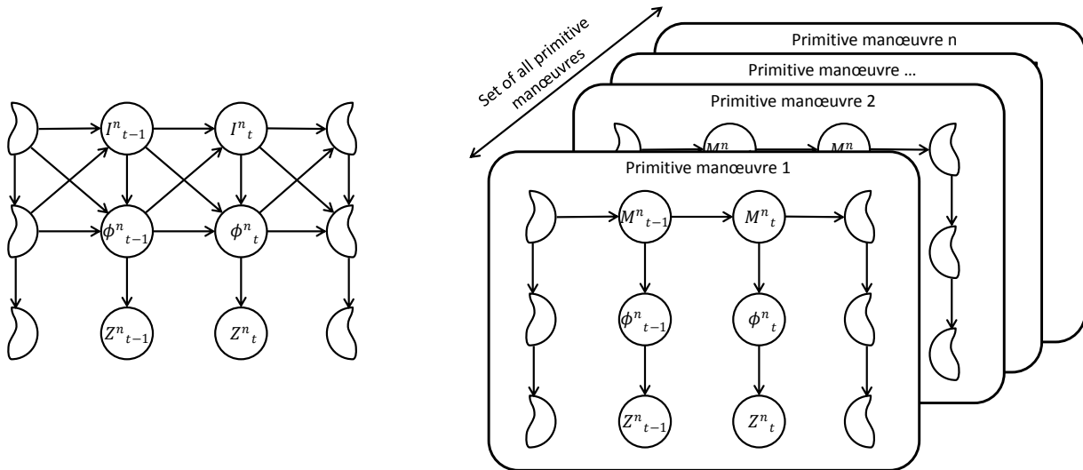
(a) Graphical representation of a single MSSM.
