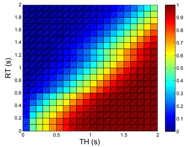
(c) \Omega_{Advice}^{Moderate}(RT, TH)
