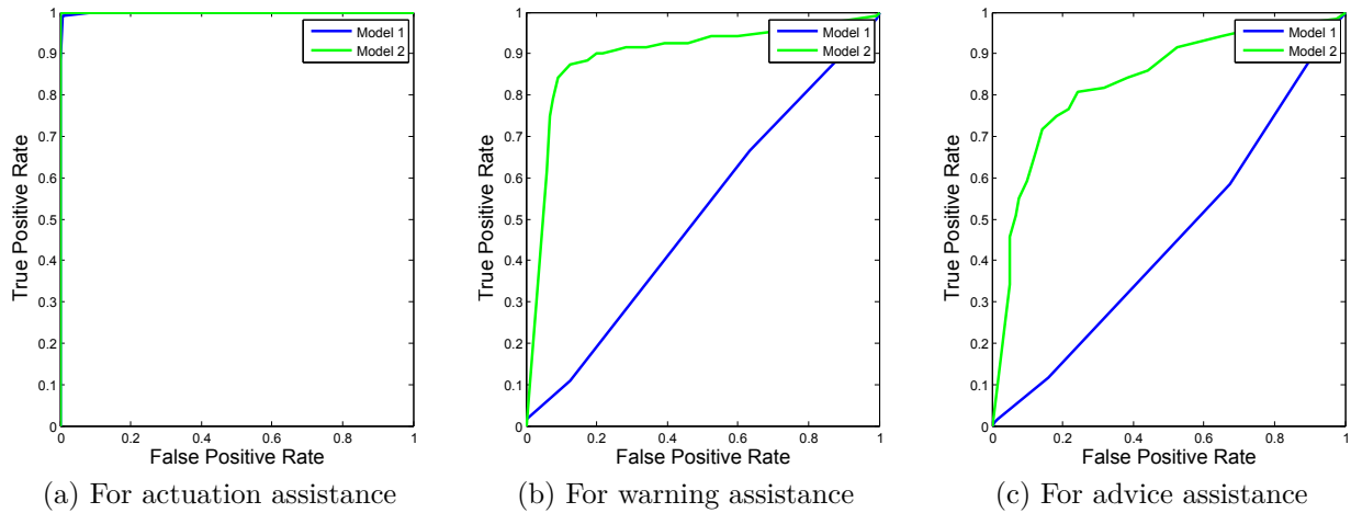
Figure 4.15: ROC curves
