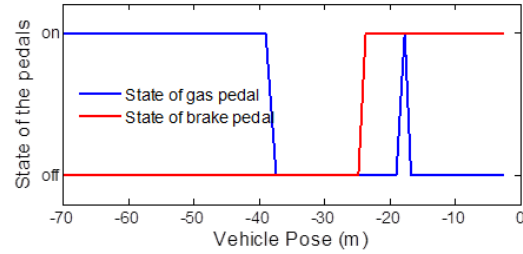
(b) State of the gas and brake pedals with respect to the vehicle pose.
