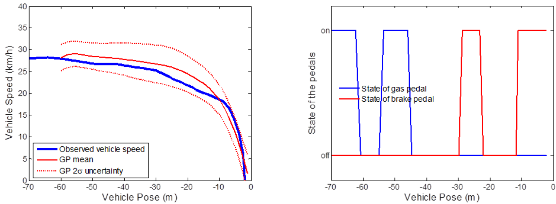
(a) Vehicle speed and learnt velocity profile with respect to the vehicle pose. (b) State of the gas and brake pedals with respect to the vehicle pose.
