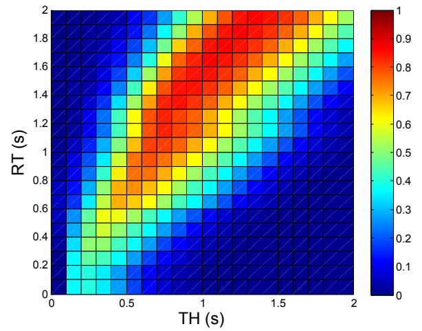
(b) \Omega_{Advice}^{Hard}(RT, TH)
