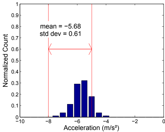
(a) Repartition of acceleration necessary to stop on time, using Model 1 in the case of automatic actuation assistance.
