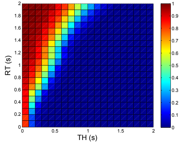
(a) \Omega_{Advice}^{Collision}(RT, TH)
