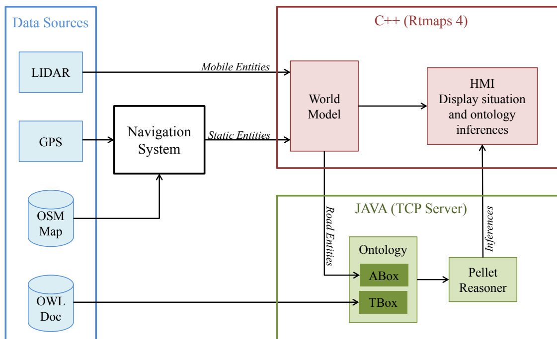
Figure 3.8: Framework for real time situation understanding.
