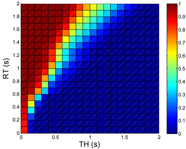
(a) \Omega_{Warning}^{Collision}(RT, FT)
