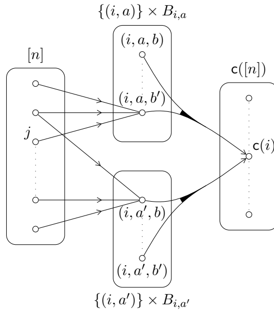
Figure 5.3: Hypergraph \mathcal{G}_s^- associated with F^-
