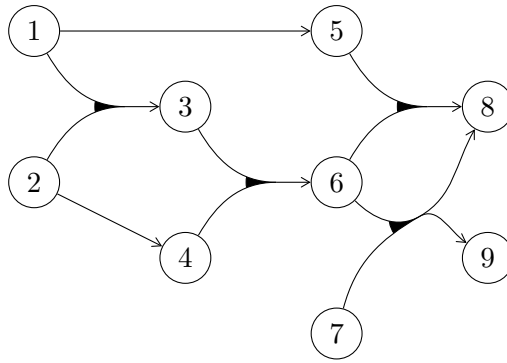
Figure 5.1: A directed hypergraph
