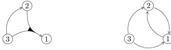
Figure 6.1: Hypergraphs \mathcal{H}^+ (left) and \mathcal{H}^- (right) associated with T
