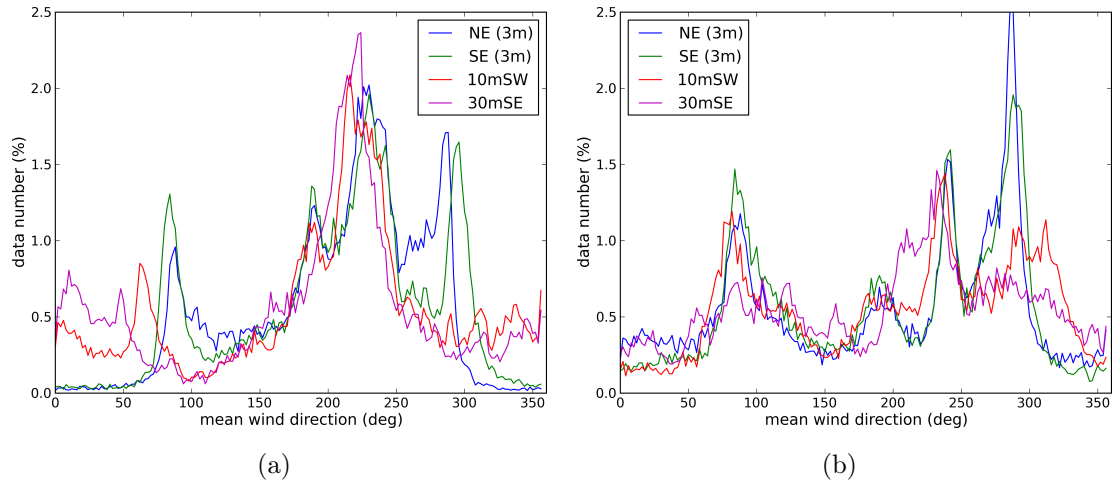
Figure 5.11 – Mean wind direction frequency distributions from measurements over two years (April 2012 - March 2014) at three levels: 3 m (NE and SE), 10 m (10mSW) and 30 m (30mSE), selected for the periods for which L_{MO} measured by 10mSW is (a) neutral |L_{MO}| > 200 m (10-min average data number: 36067) and (b) stable 0 < L_{MO} < 200 m (10-min average data number: 22174).
