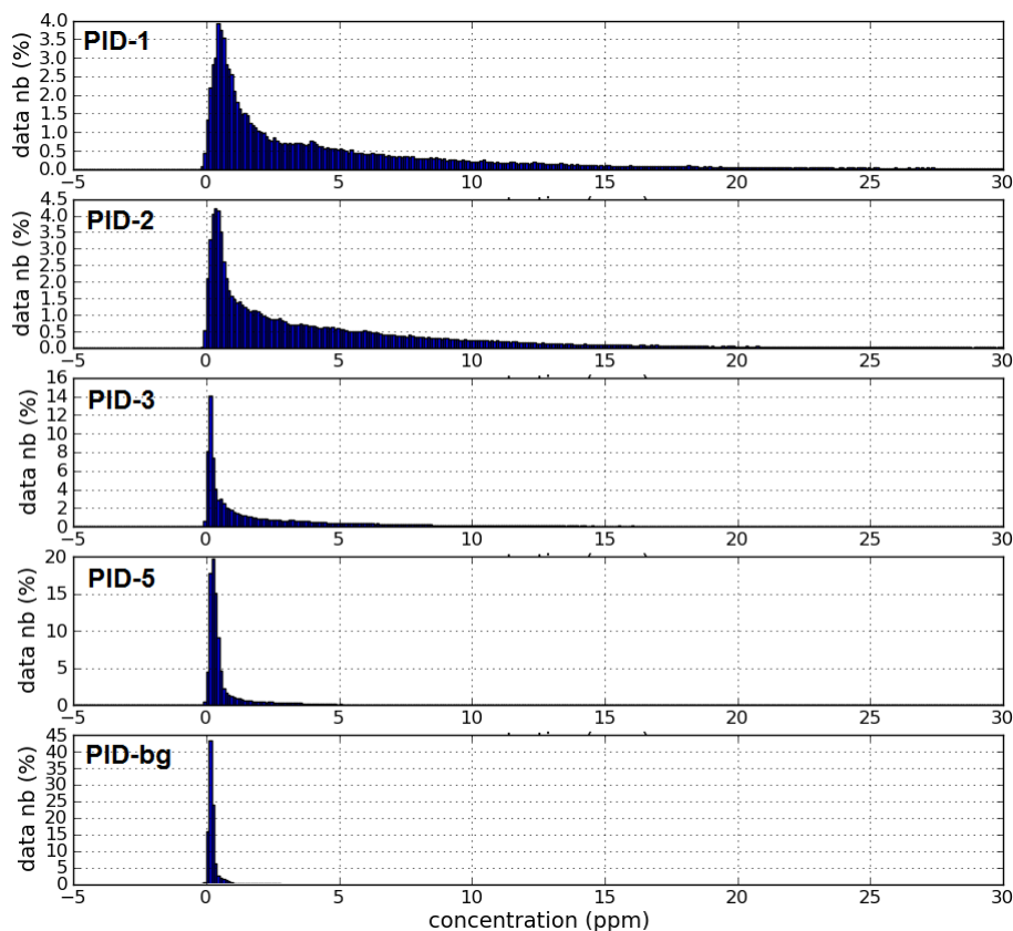
Figure 6.8 – Concentration histogram for the IOP-7; from top to bottom: PID-1, -2, -3, -5 and -background; the axis-y indicates the percentage of data number.
