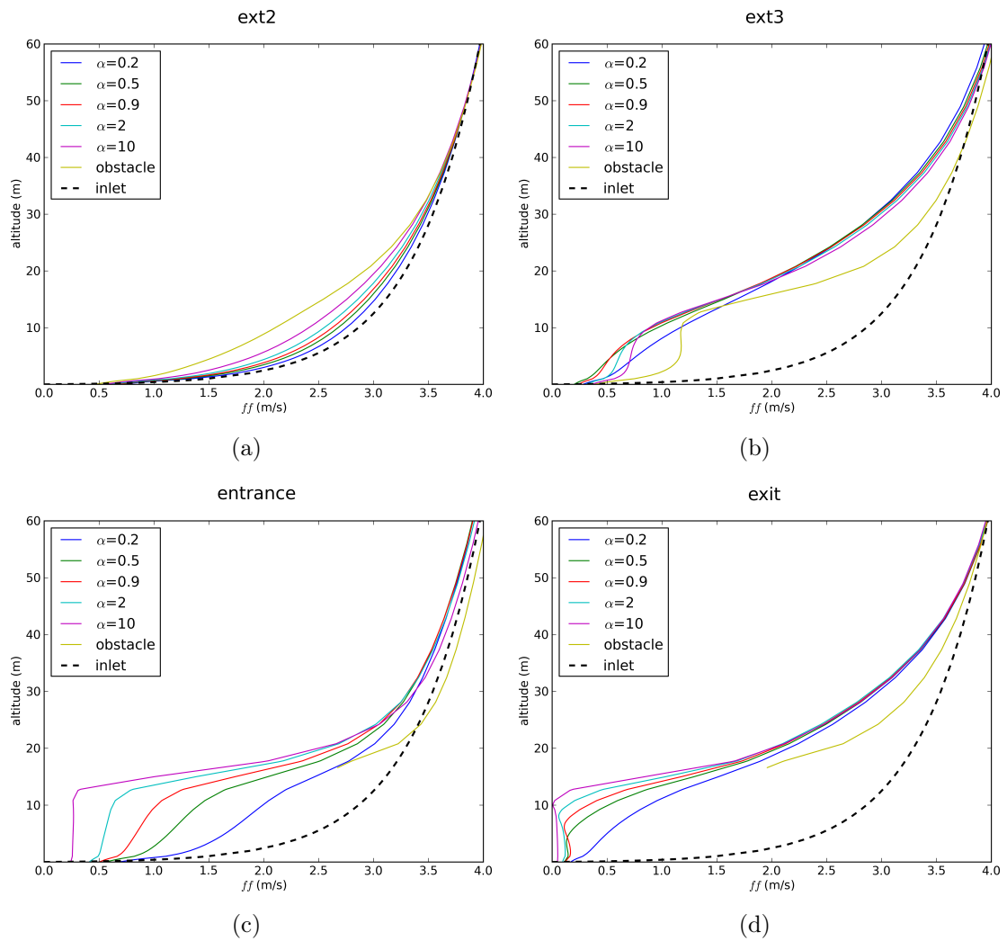
Figure 5.17 – Horizontal mean wind speed vertical profiles for several extracted points: (a) ext 2, (b) ext 3, (c) entrance and (d) exit, obtained from simulations with simplified geometry for the forest of \alpha = 0.2, 0.5, 0.9, 2 and 10 \text{ m}^{-1} , and the solid obstacle.
