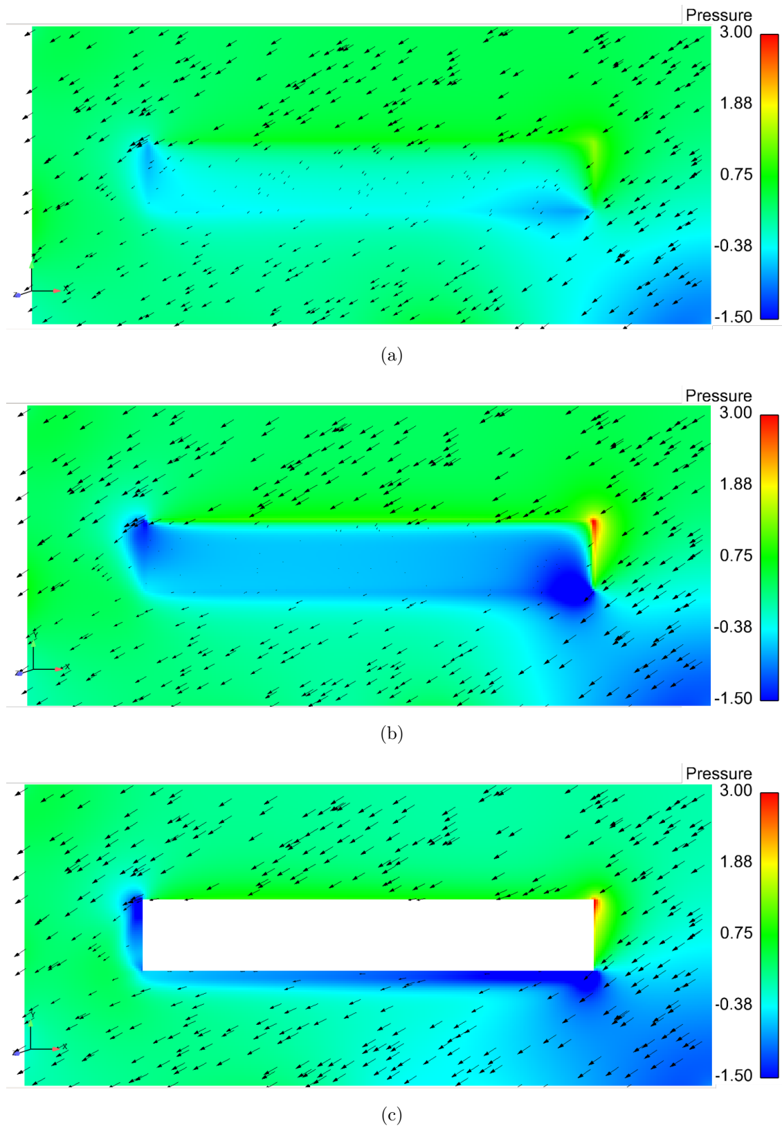
Figure 5.24 – Horizontal cross-sections of pressure (Pa) at height of 3 m, obtained from simulations with simplified geometry for the forest of (a) \alpha = 0.2 \text{ m}^{-1} , (b) \alpha = 2 \text{ m}^{-1} , and (c) the solid obstacle.
