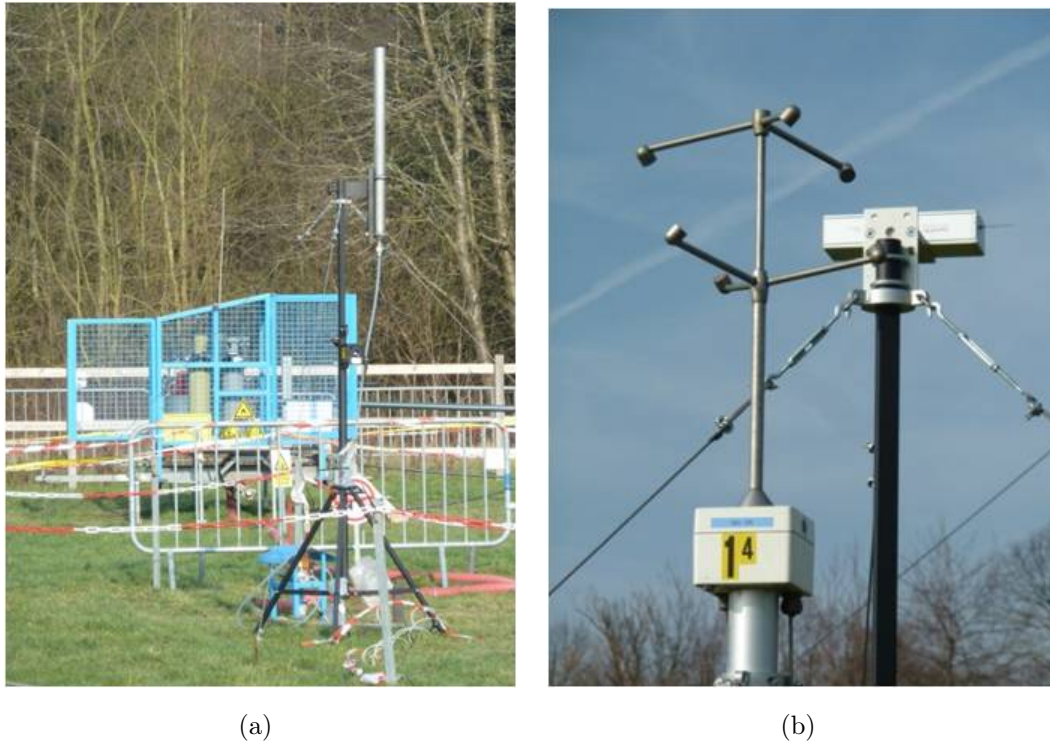
Figure 2.2 – (a) Tracer gas release point and (b) collocated ultrasonic anemometer (front) and photo ionisation detector (behind)
