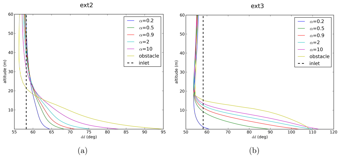
Figure 5.16 – Horizontal mean wind direction vertical profiles for several extracted points: (a) ext 2 and (b) ext 3, obtained from simulations with simplified geometry for the forest of \alpha = 0.2, 0.5, 0.9, 2 and 10 \text{ m}^{-1} , and the solid obstacle.
