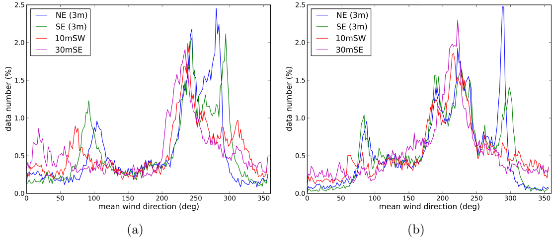
Figure 5.13 – Same as Fig. 5.11, selected for the periods during (a) summer (June, July, August) (10-min average data number: 17902) and (b) winter (Dec., Jan., Feb) (10-min average data number: 22787).
