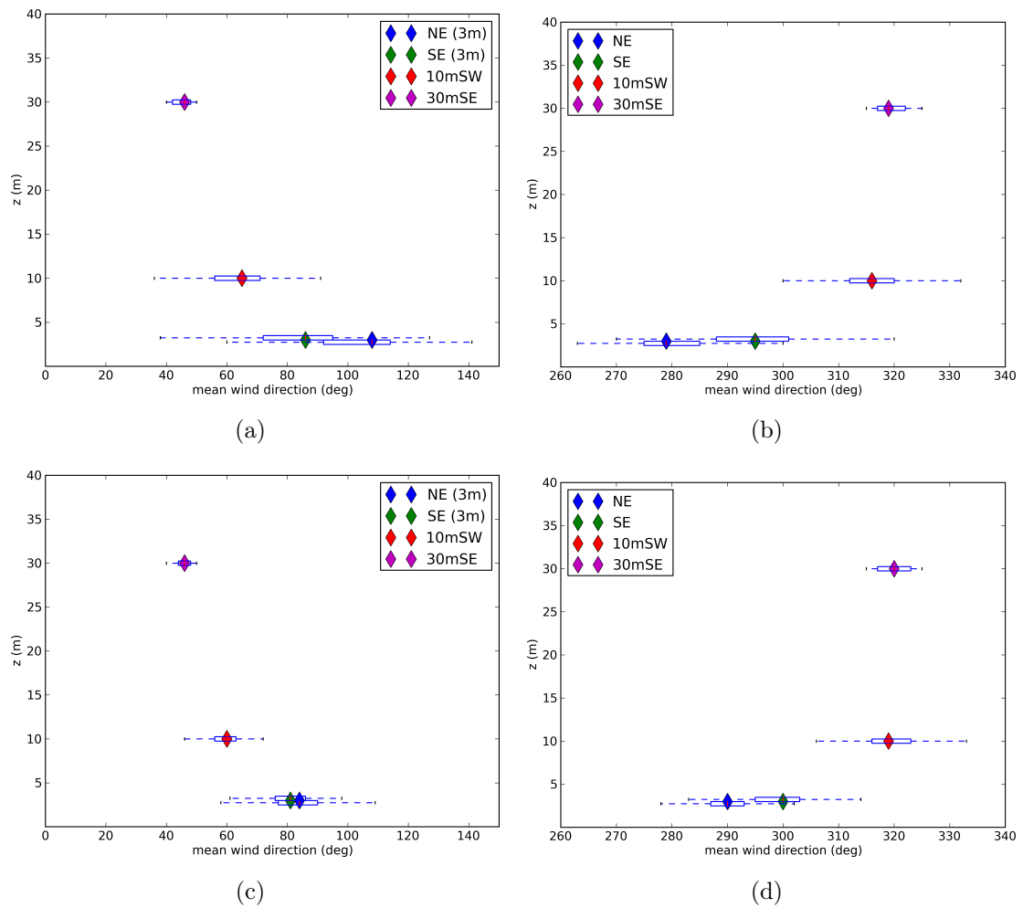
Figure 5.14 – Same as Fig.5.12, selected for the periods for which mean wind direction measured by 30mSE is (a) 40^\circ - 50^\circ during summer, (b) 315^\circ - 325^\circ during summer, (c) 40^\circ - 50^\circ during winter, and (d) 315^\circ - 325^\circ during winter.
