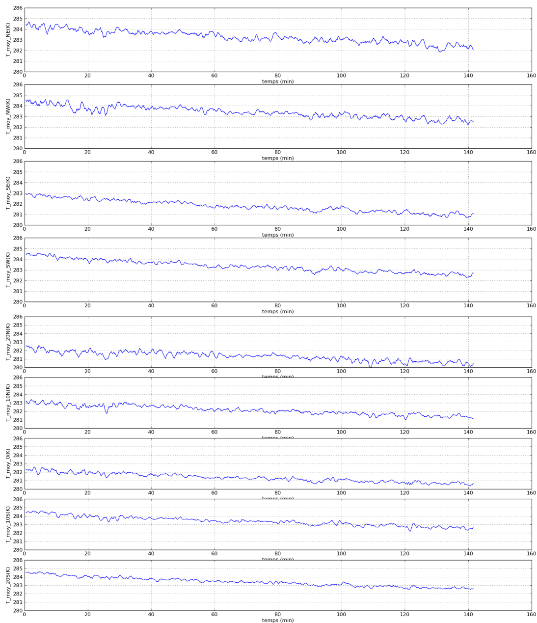
Figure B.5 – ‘Quick Look’ at temperature T_s (K) filtered by central moving average over 1min of 9 anemometers at "sonic square" and "sonic arc at 50 m" during the IOP-11; from top to bottom: NE, NW, SE, SW, 20N, 10N, 0, 10S, 20S.
