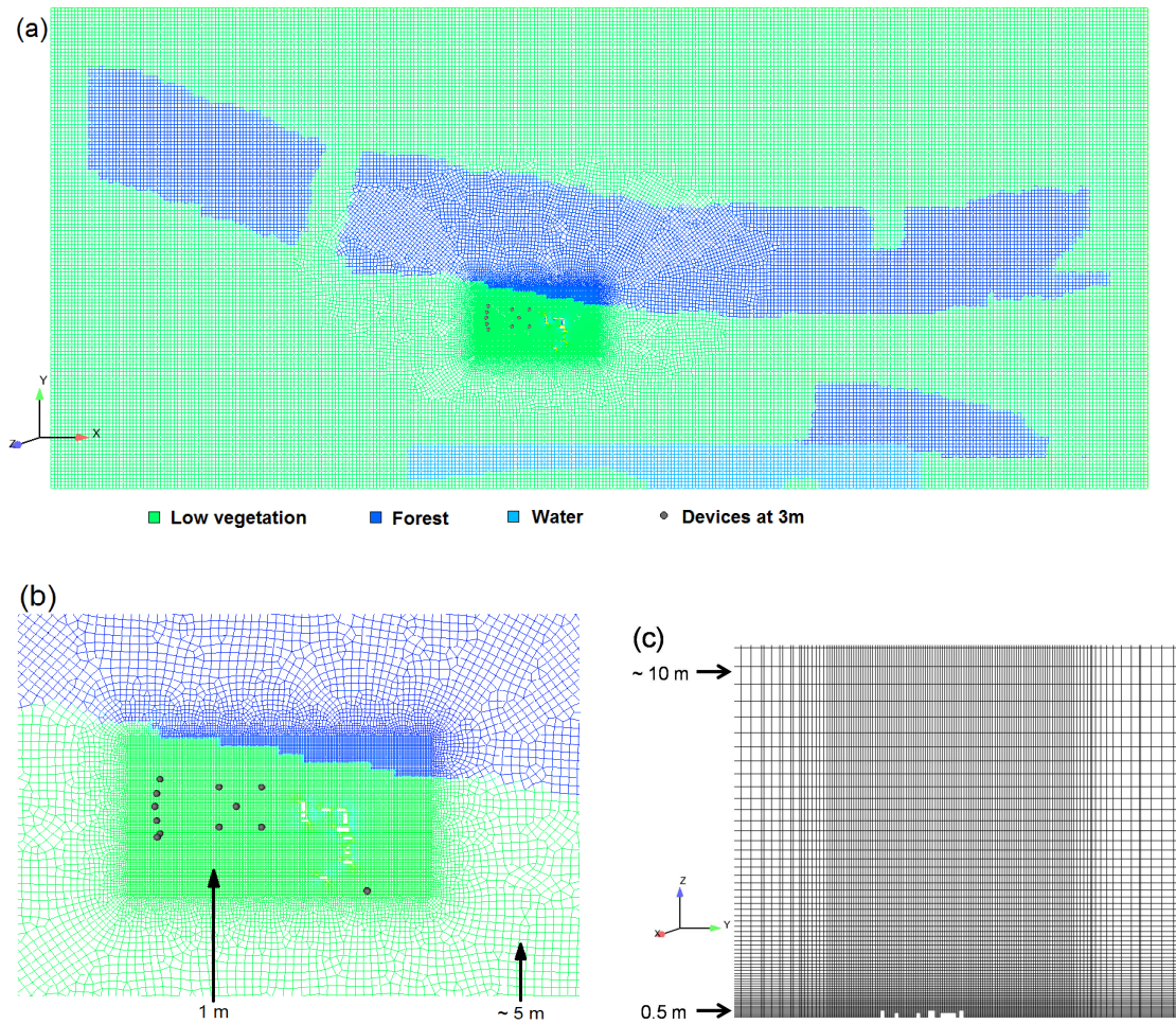
Figure 5.4 – Mesh for the modelling area taking into account the land-use map and the eastward shelters: (a) horizontal cross-section at ground level; (b) zoom on the instrumented area at ground level; (c) vertical cross-section. Grey circles indicate the positions of measurement devices.
