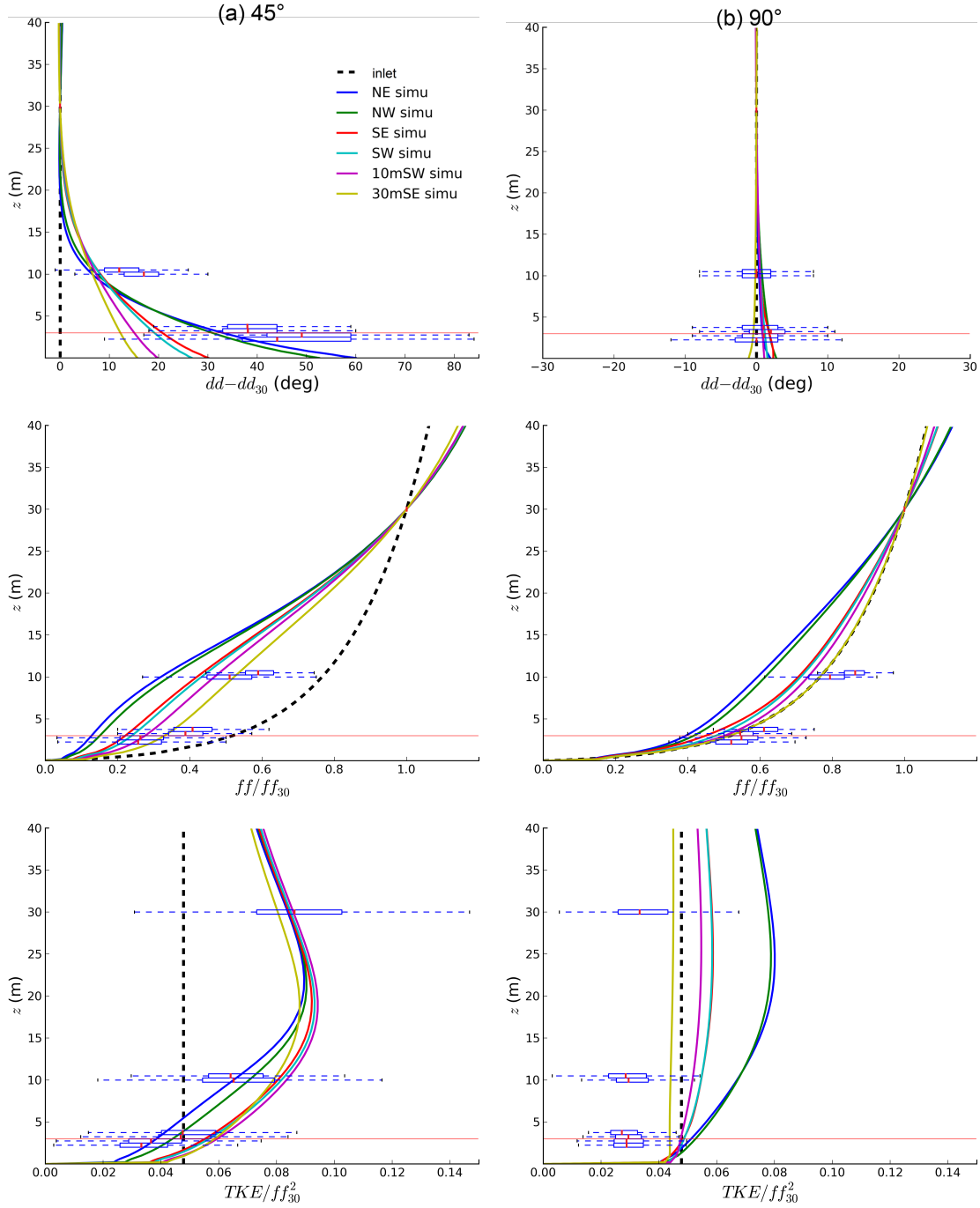
Figure 5.5 – Comparison of wind direction deviation dd - dd_{30} (top), normalized horizontal wind speed ff/ff_{30} (middle) and normalized turbulent kinetic energy TKE/ff_{30}^2 (bottom) for classical logarithmic analytical profiles (dashed lines), simulations (solid lines) under neutral conditions of wind directions: (a) 45° and (b) 90°, and continuous measurements (box plots) over two years (April 2012 - March 2014) for selected wind directions: (a) 40°-50° and (b) 85°-95° at 30 m with |L_{MO}| > 200 m at 10 m. Box plots represent measurements of anemometers, from bottom to top: NE, NW, SE, SW, 10mSW, 10mSE, and 30mSE (only for TKE/ff_{30}^2 ). The boxes extend from the lower to upper quartile values of the data with vertical red line at the median. The dashed lines extend from the lowest to the highest values of the data. The subscript ‘30’ means values of variables at 30 m. The horizontal red line indicates the vertical level of 3 m.
