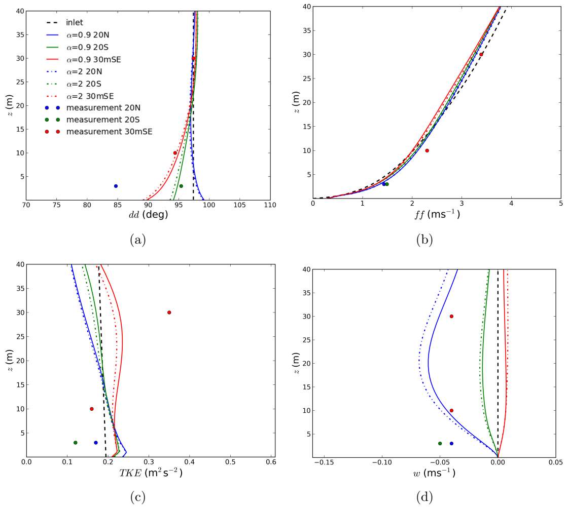
Figure B.7 – Comparison of vertical profiles of (a) horizontal wind direction, (b) horizontal wind speed, (c) TKE and (d) vertical velocity between simulations and measurements for the IOP-11 ; ‘dashed line’: inlet condition; ‘solid line’: simulations with \alpha = 0.9 ; ‘dash-dot line’: simulation with \alpha = 2 ; ‘colour circles’: measurements.
