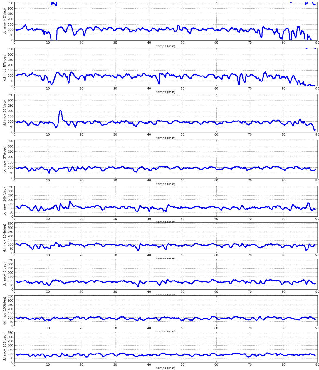
Figure A.6 – ‘Quick Look’ at the horizontal wind direction dd filtered by central moving average over 1min of 9 anemometers at "sonic square" and "sonic arc at 50 m" during the IOP-7; from top to bottom: NE, NW, SE, SW, 20N, 10N, 0, 10S, 20S.
