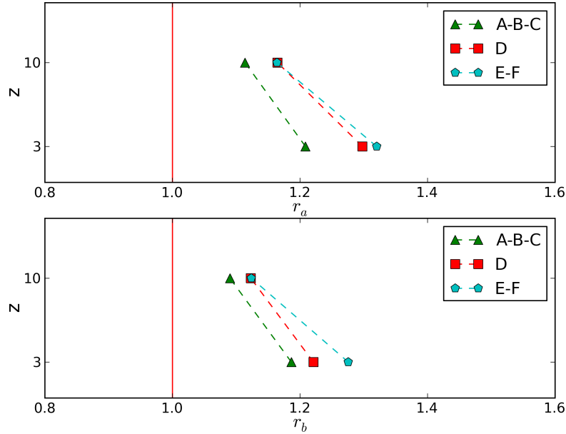
Figure 3.11 – Ratios between eddy advection velocity and mean wind speed r_a and r_b as function of measurement height for different stability classes. Values shown represent the median of ratios calculated for the selected 30-min period over two years.
