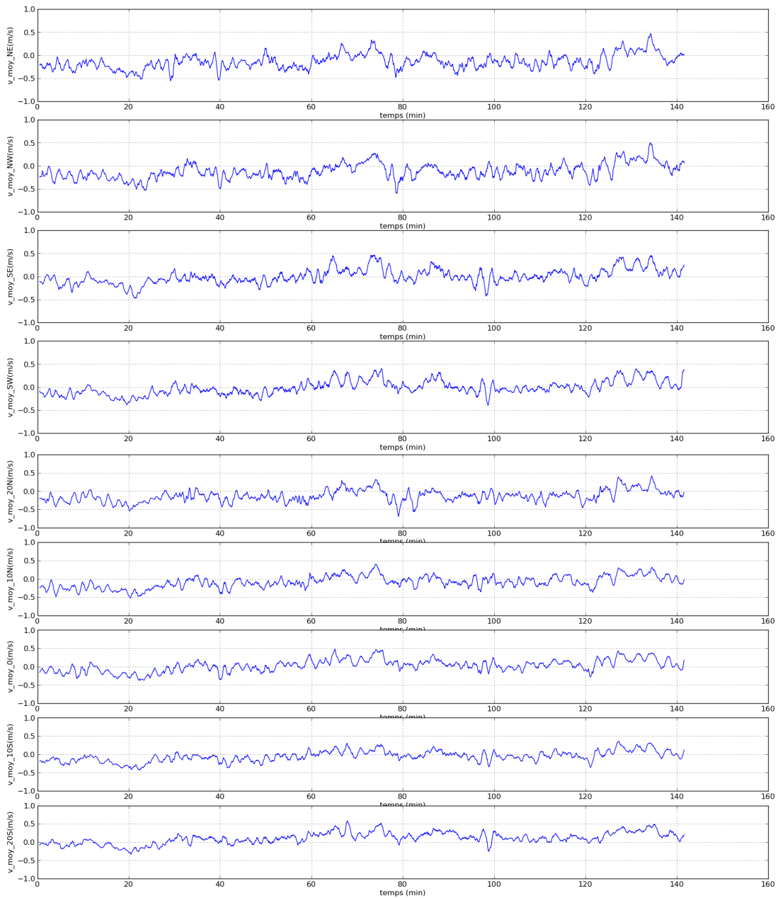
Figure B.3 – ‘Quick Look’ at wind velocity v (m/s) filtered by central moving average over 1min of 9 anemometers at "sonic square" and "sonic arc at 50 m" during the IOP-11; from top to bottom: NE, NW, SE, SW, 20N, 10N, 0, 10S, 20S.
