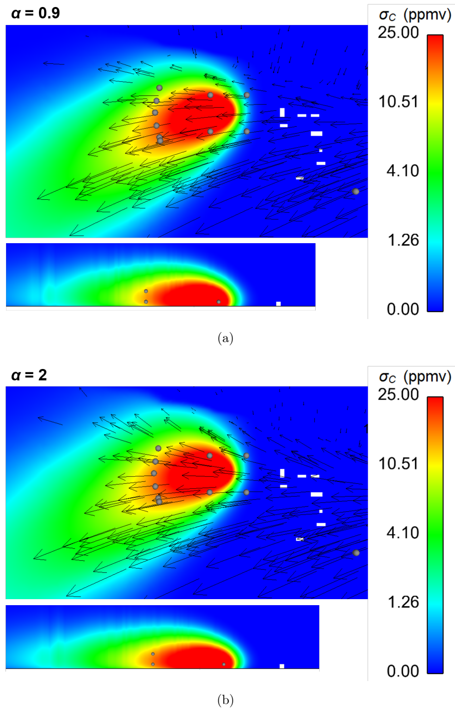
Figure 6.13 – Horizontal and vertical cross-sections of concentration fluctuation \sigma_C for simulations of the IOP-7 with R_f=0.5 and \sigma_C=1\%C at the source for (a) \alpha = 0.9 \text{ m}^{-1} and (b) \alpha = 2 \text{ m}^{-1} ; cross-sections, vectors and grey circles are identical with Fig. 6.11; color maps are in logarithmic scale.
