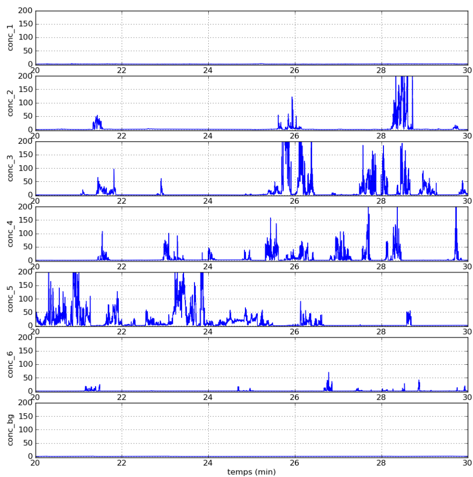
Figure 6.5 – ‘Quick Look’ at concentration data after the baseline removal for the IOP-11 from 20th to 30th minutes; from top to bottom: PID-1, -2, -3, -4, -5, -6 and -background; see the whole IOP in Fig. B.6.
