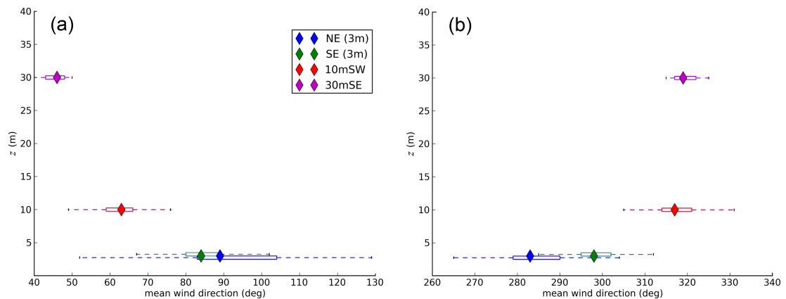
Figure 5.2 – Mean wind direction from measurements over two years (April 2012 - March 2014) at three levels: 3 m (NE and SE), 10 m (10mSW) and 30 m (30mSE), selected for the periods for which mean wind direction measured by 30mSE is (a) 40^{\circ} - 50^{\circ} and (b) 315^{\circ} - 325^{\circ} , and for |L_{MO}| > 200 m measured by 10mSW. The dashed lines extend from the lowest to highest values of the data with "diamond" at the median. The box indicates the 25th and 75th percentiles of the data.
