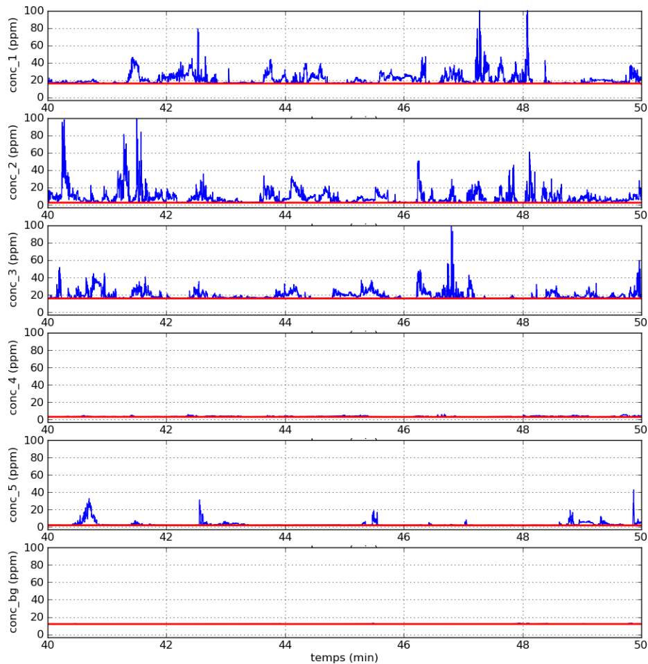
Figure 6.2 – ‘Quick Look’ at concentration data after elimination of negative values and with the baseline for the IOP-7 from 40th to 50th minutes; from top to bottom: PID-1, -2, -3, -4, -5 and -background; see the whole IOP in Fig. A.12.
