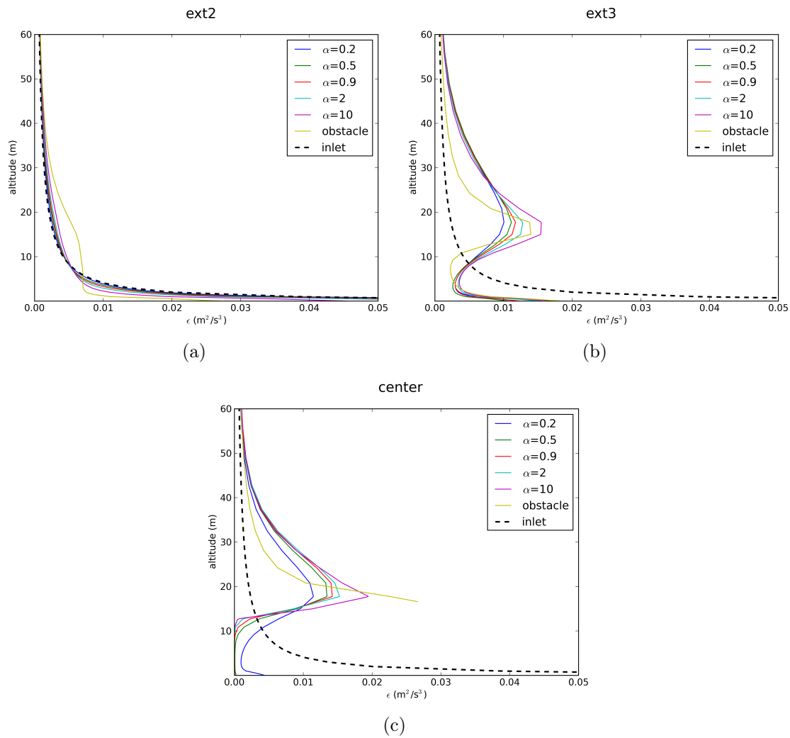
Figure 5.20 – Dissipation rate \epsilon vertical profiles for several extracted points: (a) ext 2, (b) ext 3 and (c) center. obtained from simulations with simplified geometry for the forest of \alpha = 0.2, 0.5, 0.9, 2 and 10 \text{ m}^{-1} , and the solid obstacle.
