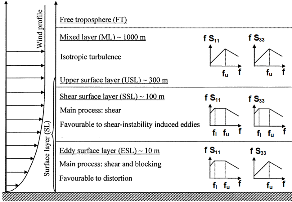
Figure 1.4 – Sketch of velocity spectra form in the surface layer [Drobinski et al., 2004]: S_{11} and S_{33} represent the spectra of longitudinal and vertical velocity components; f_l and f_u are the frequency limits with change of slope in the spectra.
