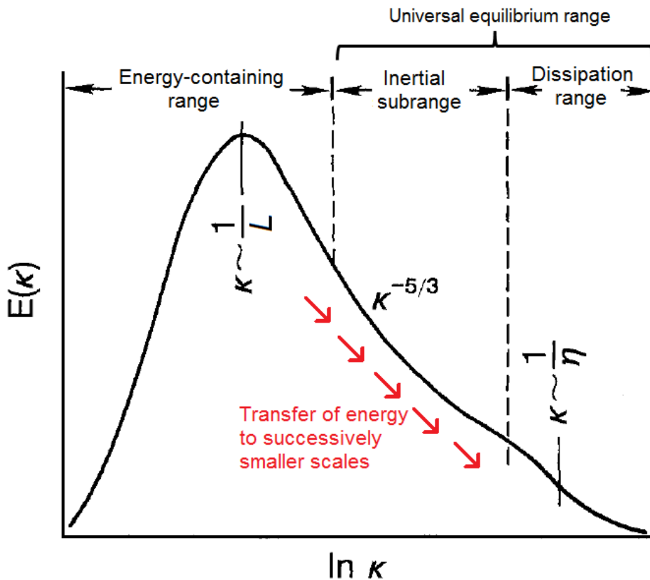
Figure 1.3 – Schematic of energy spectrum in the atmospheric boundary layer, where L is the integral length scale of turbulence and \eta is the Kolmogorov microscale (inspired by [Kaimal and Finnigan, 1994] )
