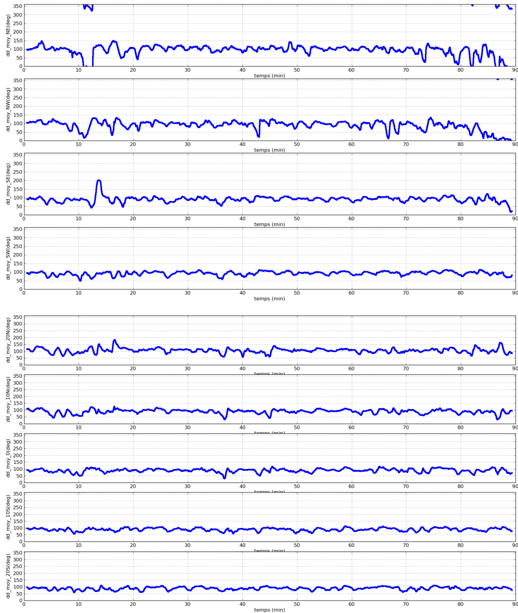
Figure 3.2 – ‘Quick Look’ at the horizontal wind direction dd filtered by central moving average over 1min of 9 anemometers at "sonic square" and "sonic arc at 50 m" during the IOP-7; from top to bottom: NE, NW, SE, SW, 20N, 10N, 0, 10S, 20S.
