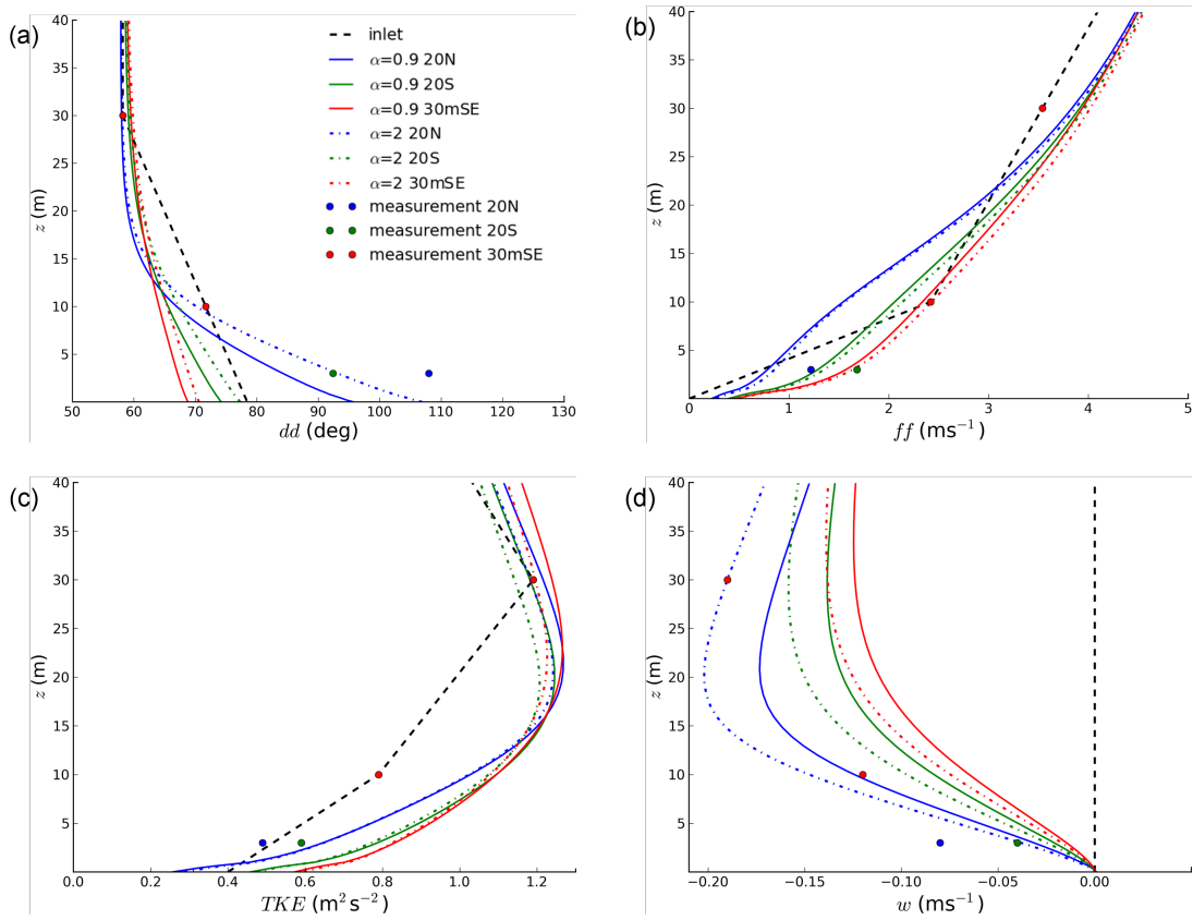
Figure 5.10 – Same as Fig. 5.9 for simulations with the inlet profiles obtained from the interpolation of the measurements at the site.
