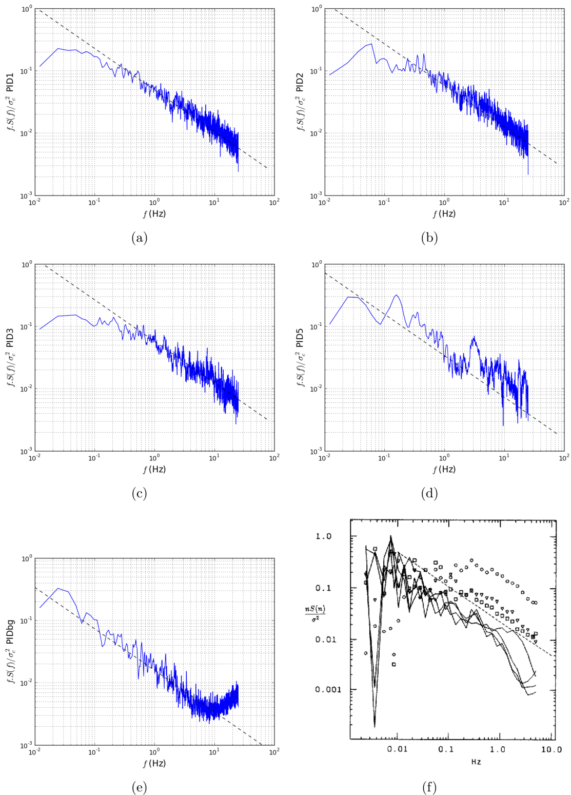
Figure 6.10 – Normalized concentration spectra f.S(f)/\sigma_c^2 for PID-1 (a), -2 (b), -3 (c), -5 (d) and -background (e) during the IOP-7, and for (f) four sample concentration spectra (continuous lines) from different points on a cross-section through a plume at 740 m range shown in [Mylne and Mason, 1991]; dashed lines on the graph indicate the -2/3 slope representing the inertial subrange.
