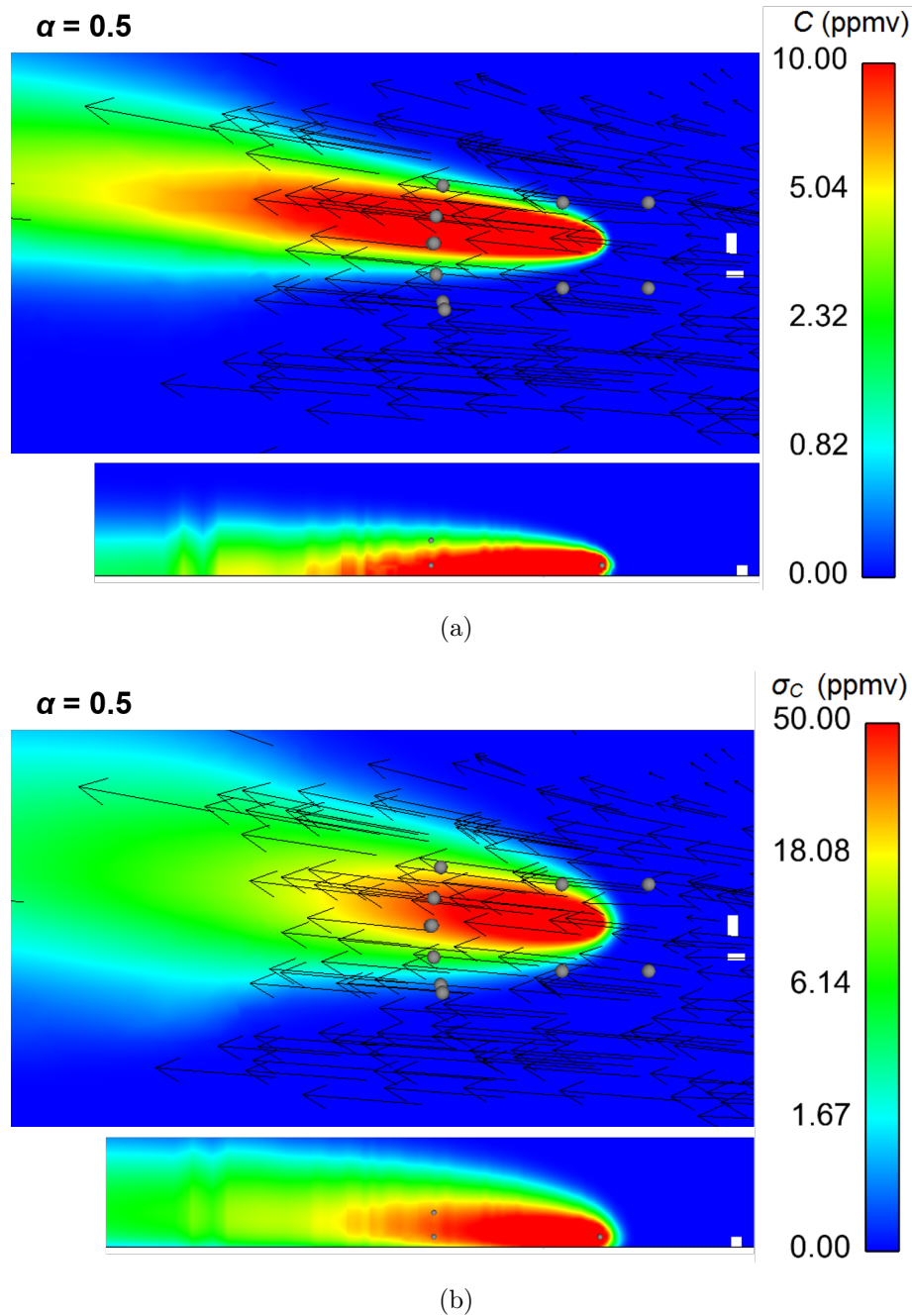
Figure 6.15 – Horizontal and vertical cross-sections of (a) mean concentration C and (b) concentration fluctuation \sigma_C for simulations of the IOP-11 with \alpha = 0.5 \text{ m}^{-1} , R_f=0.5 and \sigma_C=1\%C at the source; horizontal cross-sections (top) are at height of 3 m, with horizontal wind vectors and grey circles representing the devices; vertical cross-sections (bottom) are at the location of the source along a E-W line, with grey circles representing the source (3 m), PID-3 (3 m) and PID-6 (10 m) above PID-3; color maps are in logarithmic scale.
