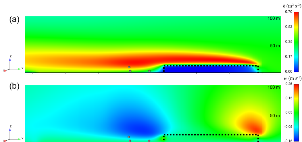
Figure 5.8 – Vertical cross-section at the location of the 10-m tower along the S-N line of (a) TKE field, and (b) vertical velocity field. Grey circles represent anemometers 20N and 20S at 3-m height and 10mSW at 10-m height.
