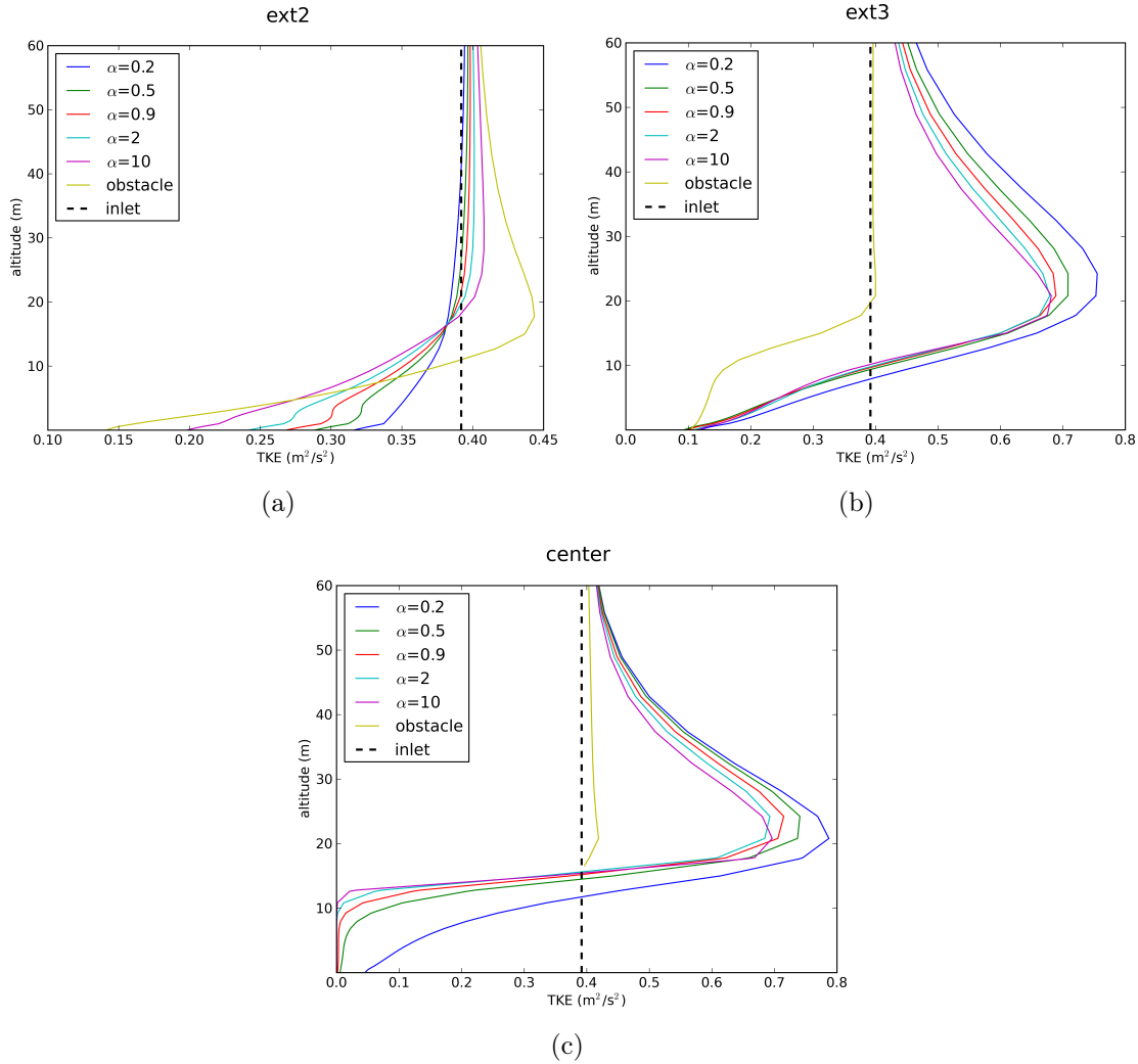
Figure 5.18 – TKE vertical profiles for several extracted points: (a) ext 2, (b) ext 3 and (c) center, obtained from simulations with simplified geometry for the forest of \alpha = 0.2, 0.5, 0.9, 2 and 10 \text{ m}^{-1} , and the solid obstacle.
