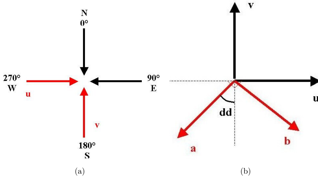
Figure 3.1 – (a) Conventional meteorological reference (u, v, w) and (b) reference in the mean wind frame (a, b, w)
