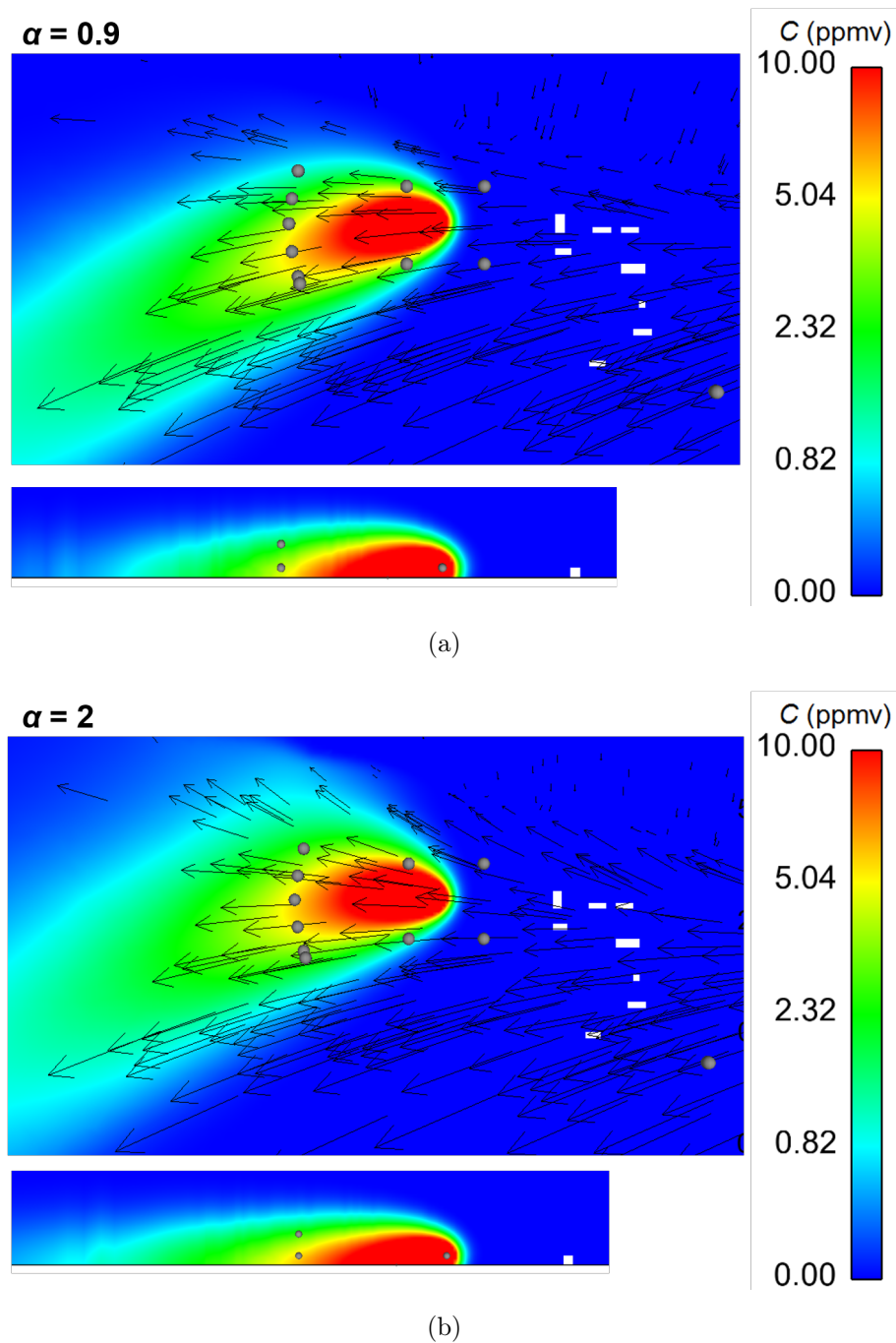
Figure 6.11 – Horizontal and vertical cross-sections of mean concentration C for simulations of the IOP-7 with (a) \alpha = 0.9 \text{ m}^{-1} and (b) \alpha = 2 \text{ m}^{-1} ; horizontal cross-sections (top) are at height of 3 m, with horizontal wind vectors and grey circles representing the devices; vertical cross-sections (bottom) are at the location of the source along a E-W line, with grey circles representing the source (3 m), PID-3 (3 m) and the future additional PID (10 m) over PID-3; color maps are in logarithmic scale.
