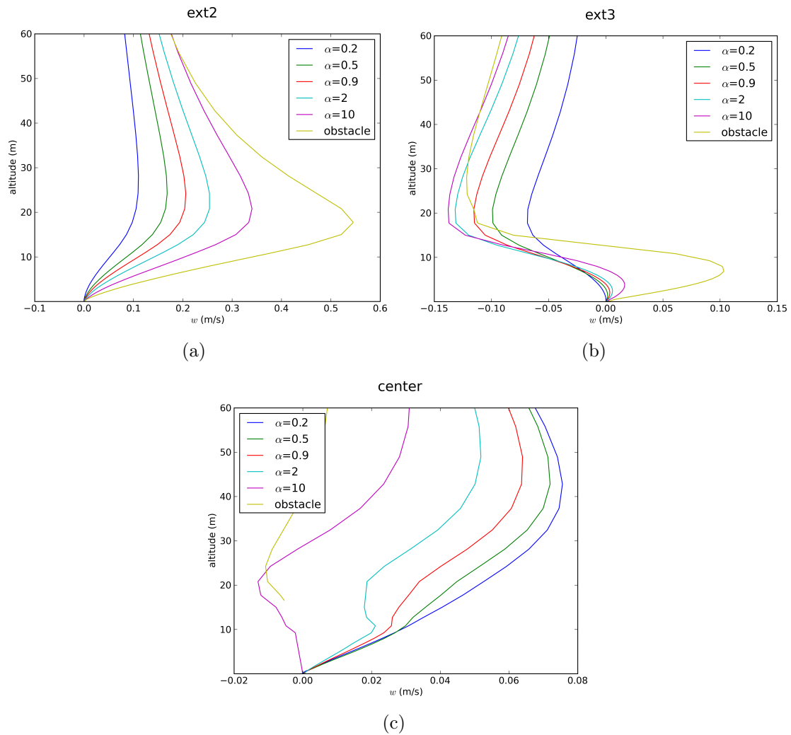
Figure 5.19 – Vertical profiles of vertical velocity w for several extracted points: (a) ext 2, (b) ext 3 and (c) center, obtained from simulations with simplified geometry for the forest of \alpha = 0.2, 0.5, 0.9, 2 and 10 \text{ m}^{-1} , and the solid obstacle.
