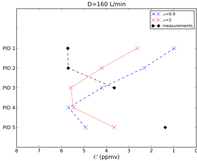
Figure 6.12 – Comparison of measured mean concentration C with simulations for \alpha = 0.9 and 2 \text{ m}^{-1} for the IOP-7.
