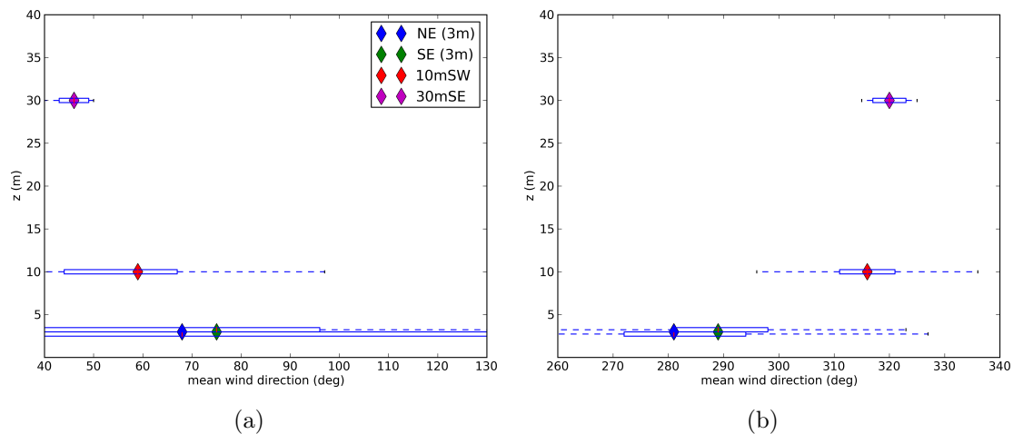
Figure 5.12 – Mean wind direction from measurements over two years (April 2012 - March 2014) at three levels: 3m (NE and SE), 10m (10mSW) and 30m (30mSE), selected for the periods for which mean wind direction measured by 30mSE is (a) 40^\circ - 50^\circ and (b) 315^\circ - 325^\circ , and for 0 < L_{MO} < 200 m measured by 10mSW. The dashed lines extend from the lowest to highest values of the data with "diamond" at the median. The box indicates the 25th and 75th percentiles of the data.
