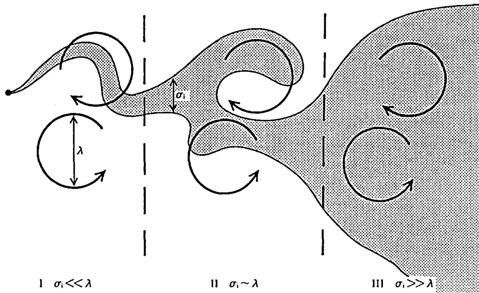
Figure 6.4 – Illustration of the conceptual model of plume dispersion [Mylné, 1992]. It shows the three different effects of eddies of length scale \lambda according to the relative size of the crosswind length scale of the instantaneous plume \sigma_i .
