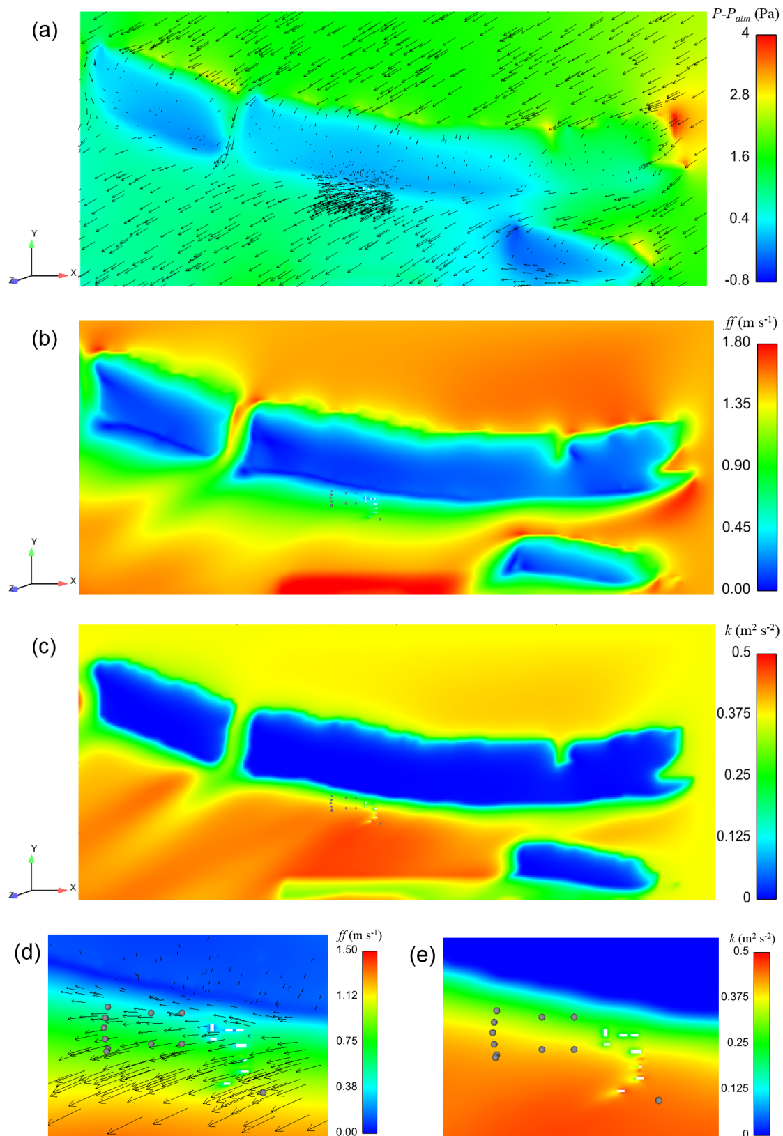
Figure 5.7 – Horizontal cross-section at 3 m of (a) pressure field with horizontal wind vectors for Zone 1, (b) velocity field for Zone 1, (c) TKE field for Zone 1, (d) velocity field with horizontal wind vectors for the instrumented area, and (e) TKE field for the instrumented area. Grey circles represent devices in the instrumented area.
