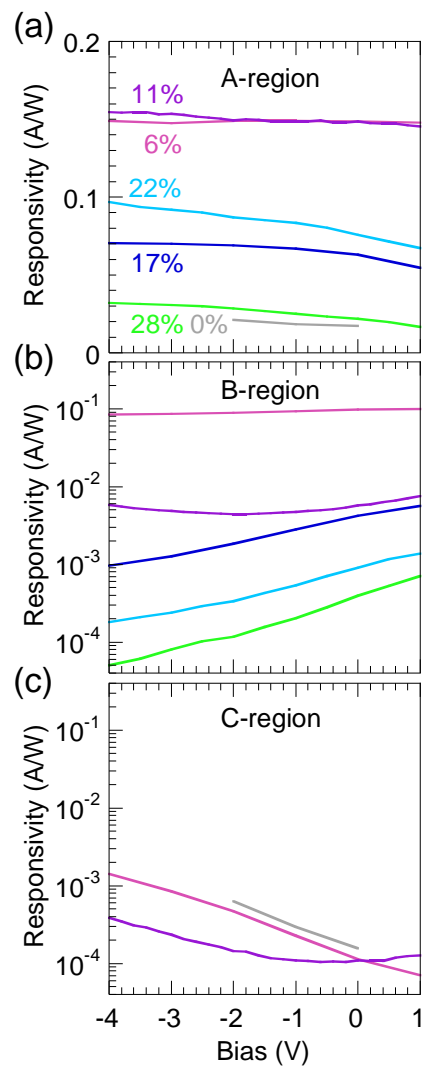
Figure 70: (a)-(c) Change in responsivity measured by BPCS as a function of applied bias at exciting photon energies belonging to the A, B, C regions of the spectra for \text{In}_x\text{Ga}_{1-x}\text{N} QW structures with different In composition. The photon energies corresponding to the different curves are marked as “A”, “B”, “C” in Figure 69.
