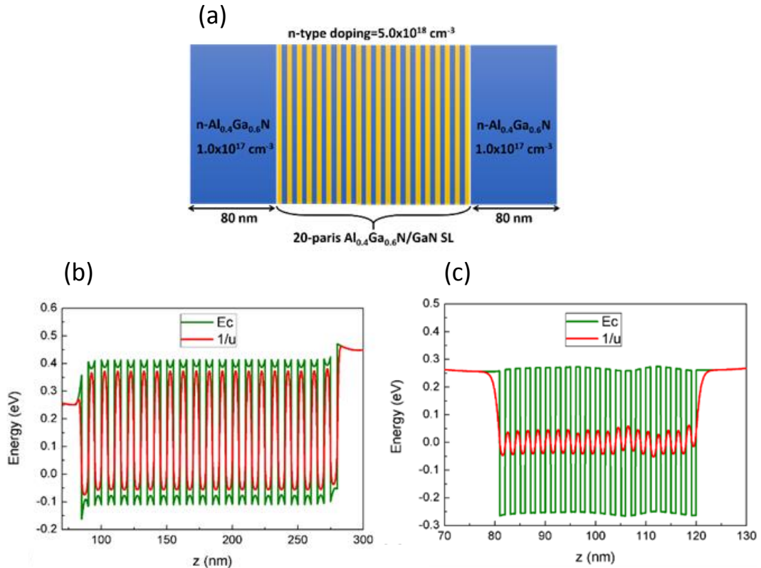
Figure 62: (a) Schematic structure of 20-period Al 0.4 Ga 0.6 N/GaN SLs. (b) and (c) are the conduction band potential ( E_c ) and effective quantum confining potential ( 1/u_c ) for 5 nm/5 nm and 1 nm/1 nm m-plane SLs.
