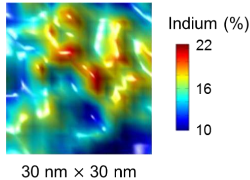
Figure 6 – 2D atomic map of indium atoms in the mid-plane of an InGaN/GaN QW measured by atom probe tomography [20]. For a mean In composition of 15% large compositional fluctuations are observed.
