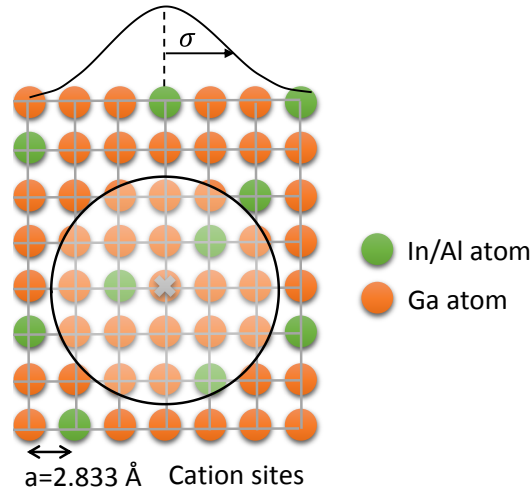
Figure 81 - The In (Al) and Ga atoms are randomly assigned at each cation lattice site by a random number generator in the InGaN (AlGaN) alloy layer. The composition at each site is then determined by a Gaussian averaging method.
