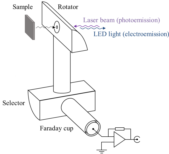
Figure 24 – Diagram of the electron spectrometer used in electro-emission experiments. The sample is mounted on a translation sample holder for alignment. The electron beam emitted into vacuum is 90°deflected in the rotator, then collimated and decelerated, and successively analyzed in energy by the selector. Finally, the selected beam is collected at the grounded Faraday cup. A hole in the rotator allows extracting light from an electro-luminescent device or shining light on a sample for photoemission.
