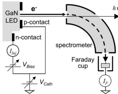
Figure 14 - Schematic of the experimental set-up used for LED electro-emission [53]: electrons are ejected into vacuum from a forward-biased LED. The kinetic energy of the electrons is analyzed in a cylindrical electrostatic deflector.
