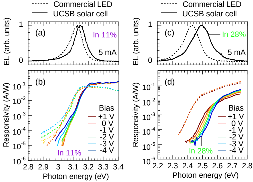
Figure 73: (a),(b) EL spectra measured at 5 mA injection and BPCS measurements of an \text{In}_{0.11}\text{Ga}_{0.89}\text{N}/\text{GaN} solar cell (continuous lines) and a commercial UV LED (dashed lines). (c),(d) EL spectra measured at 5 mA injection and BPCS measurements of an \text{In}_{0.28}\text{Ga}_{0.72}\text{N}/\text{GaN} solar cell (continuous lines) and a commercial bluish-green LED (dashed lines).
