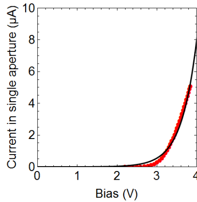
Figure 95 – Fit (black curve) based on Equation (89) of the experimental I-V characteristic (red dots) of the InGaN/GaN LED studied in Ref. [53]. For the purpose of the fit, the measured current injected in the p-electrode is scaled to the current expected to flow inside a single aperture of the electrode (see text for details).
