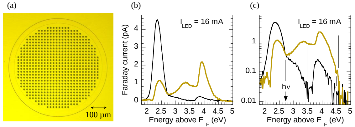
Figure 21 – (a) Optical microscope image of the holey p-contact of a sample processed for electro-emission with concentric contact geometry. (b) EDCs measured in electro-emission at an injected current of 16 mA for the Walsin LED with square electrodes studied in Ref. [53] (black curve) and a Seoul LED with concentric contacts (brown curve). (c) Same as (b) with logarithmic current scale.
