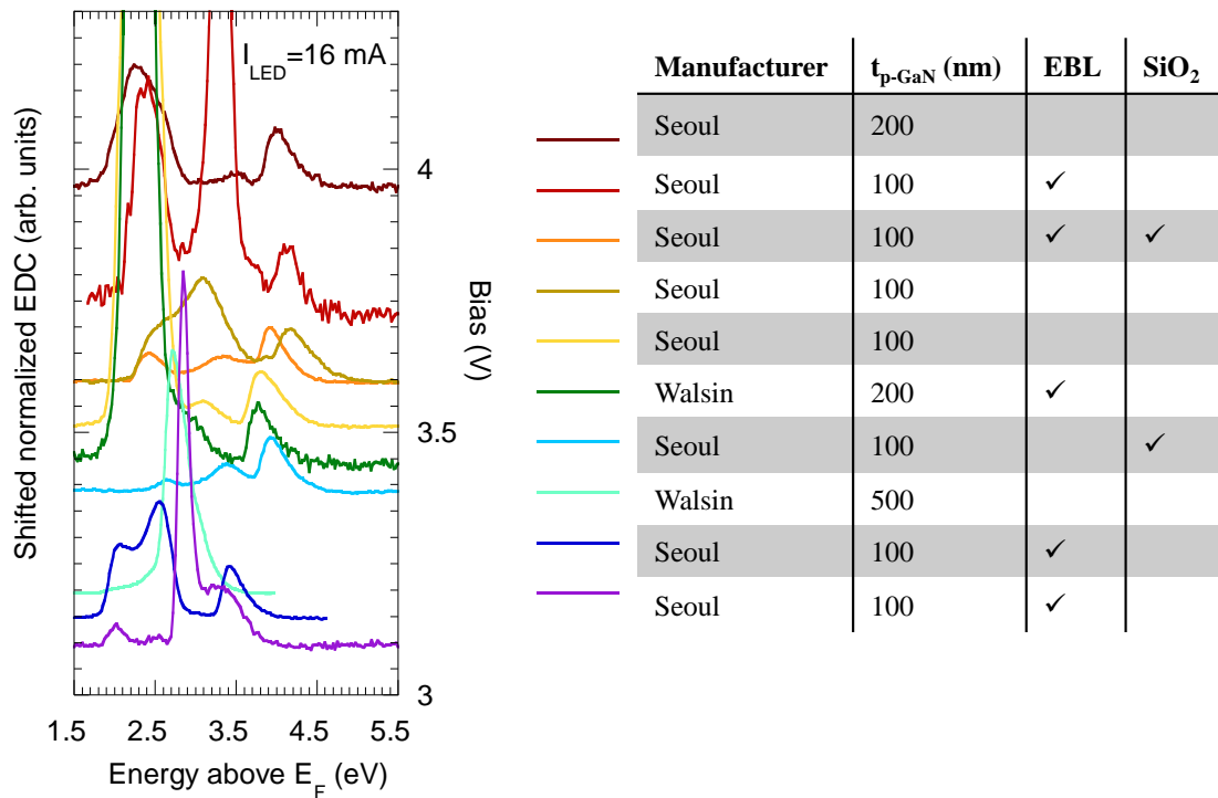
Figure 46 – EE spectra measured from different LEDs at an injected current of 16 mA. EDCs are normalized to the intensity of the high-energy peak and the baseline is shifted by the applied forward bias. The samples reported in Ref. [53] and [87] correspond to the spectra plotted as green (3.45 V) and light blue (3.39 V) curves, respectively.
