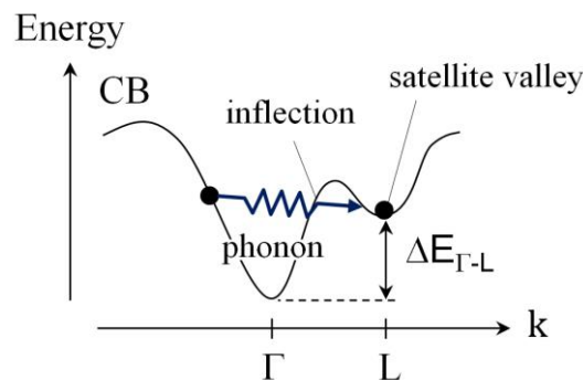
Figure 12 – Schematic showing intervalley transfer in k-space of a hot electron from the central \Gamma valley to the first satellite valley L in the conduction band of GaN. The process is mediated by a phonon which supplies momentum to the hot electron.
