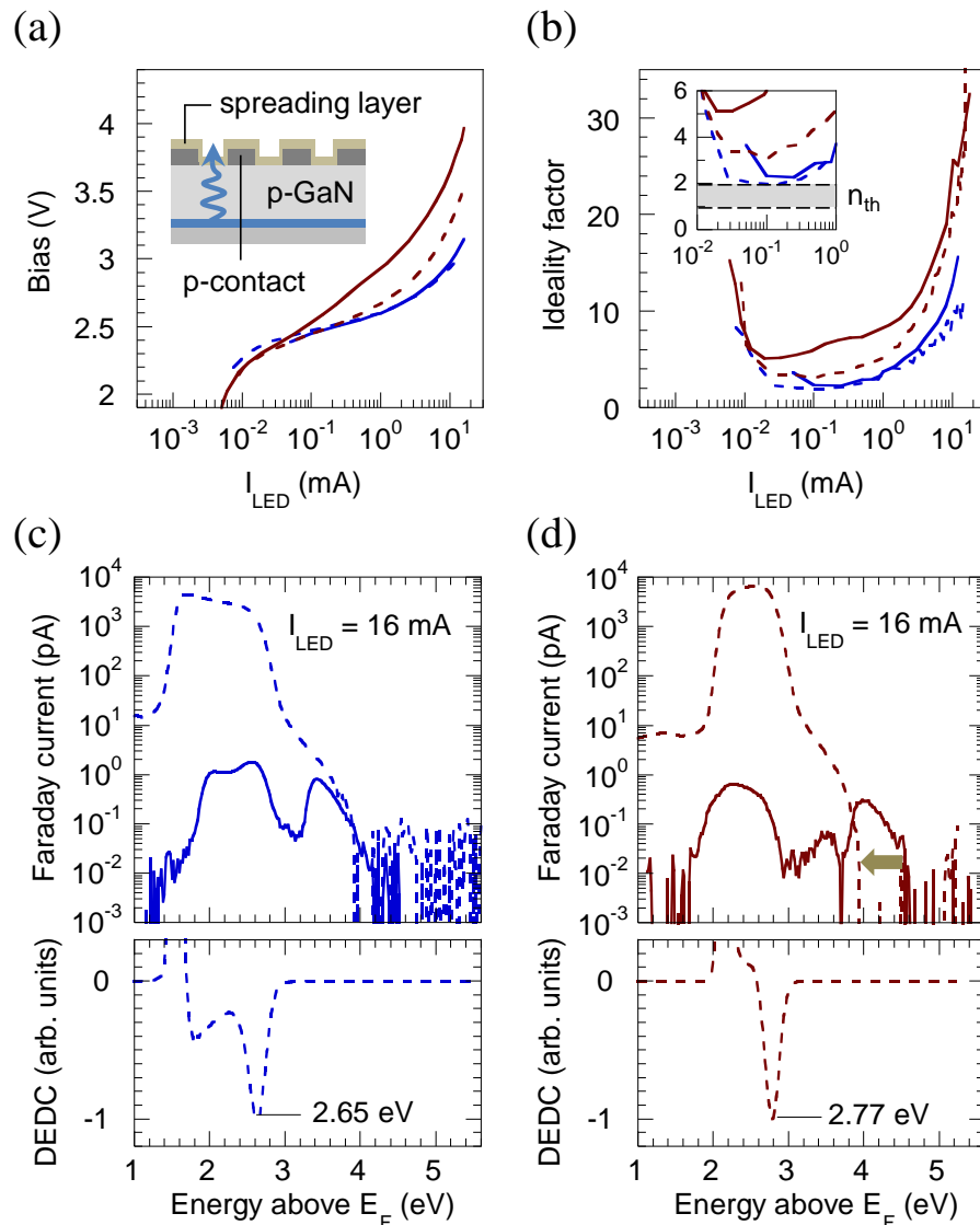
Figure 51 – Influence of a spreading layer deposition on the p-contact of two LED EE samples affecting their: (a) voltage-current characteristics; (b) ideality factors; (c) and (d) EE spectra. Both the curves measured prior (continuous lines) and after (dashed lines) deposition are plotted. Two devices are studied: one fabricated with an ohmic p-contact (blue lines) and the other fabricated with a rectifying p-contact (dark red lines), as determined from their minimum ideality factors, close or larger than the theoretical values for an ideal p-n junction.
