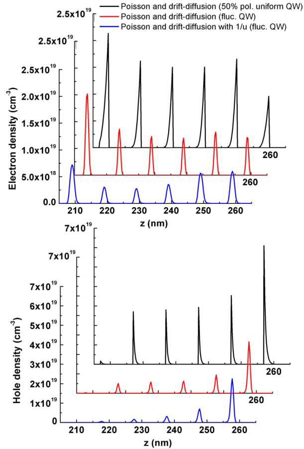
Figure 85 - Carrier distribution in the 6 QWs of the LED for electrical injection at 20 \text{ A/cm}^2 obtained using a classical Poisson-DD model for uniform layers and the landscape theory implement in Poisson-DD for a structure with random alloy fluctuations. The x- and y-axis are shifted for illustration.
