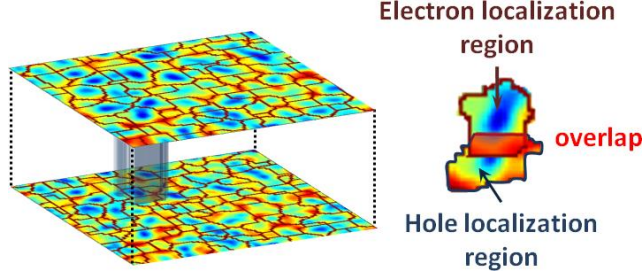
Figure 61: Overlap regions are defined as intersections between electron and hole localization subregions. (Left) superimposed electron and hole landscapes. (Right) Example of one overlapping region defined as the intersection of an electron and hole localization subregion.
