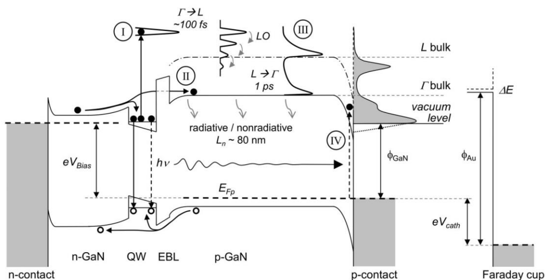
Figure 17 – Schematics of the emission of electrons from an LED in vacuum according to Ref. [53]: electrons originate from the QW with some high-energy (“hot”) electrons generated by the Auger effect. After thermalization in the different accessible valleys of the CB, they give rise to high-energy peaks in the energy distribution of electrons emitted in vacuum. Thanks to negative electron affinity of the surface due to cesium deposition, electrons with energy below the bulk CB minimum can be observed, for example due to energy relaxation in the BBR or below-gap absorption excited by the LED light, as long as their energy is above the vacuum level. The active layer of the LED is shown as a single QW, but the actual sample has 8 QWs.
