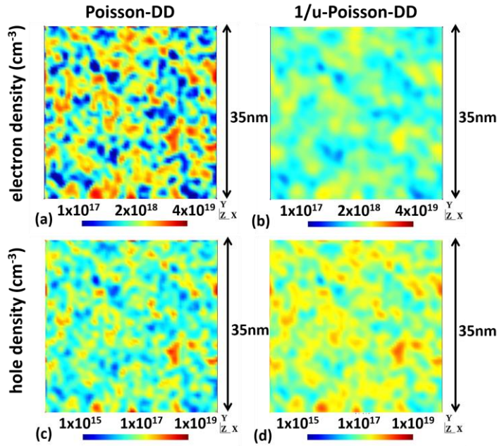
Figure 84 - Electron and hole carrier densities computed in the mid-plane of the third QW with compositional disorder at 20 \text{ A/cm}^2 current density using: (a),(c) the classical Poisson and drift-diffusion model; (b),(d) the landscape theory implemented in Poisson-DD.
