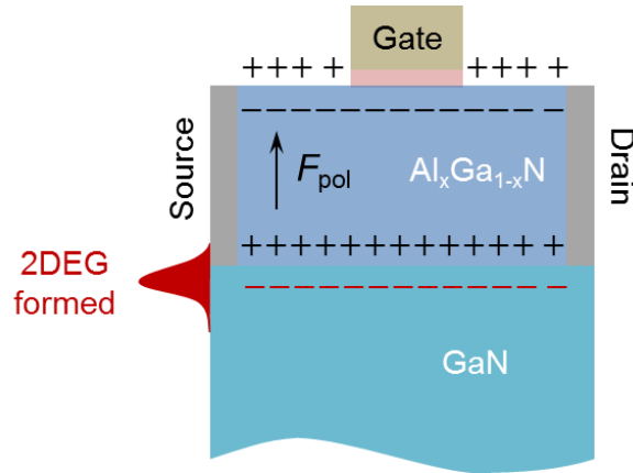
Figure 8 – Schematic of an AlGaN/GaN HEMT device. The 2DEG in the GaN channel is due to the polarization discontinuity at the AlGaN/GaN interface.
