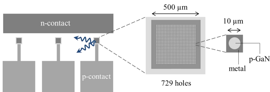
Figure 15 – Schematic representation of the contact geometry used in the LED sample studied in Ref. [53] by electro-emission. Three identical devices are present on the sample. The p-contact consists of an array of holes exposing p-GaN for electron emission into vacuum.
