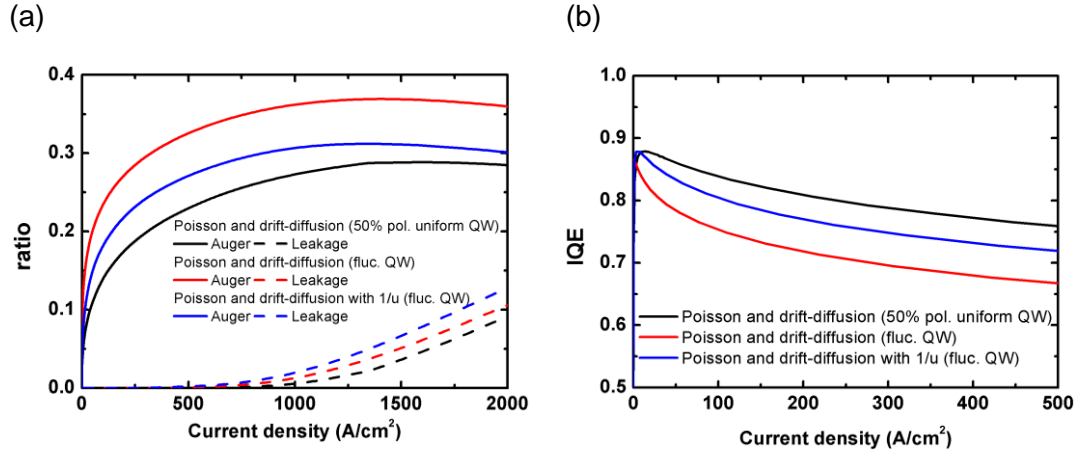
Figure 89 – (a) Ratio of Auger and leakage currents to total injected current and (b) IQE curve for the full structure LED computed from the different models.
