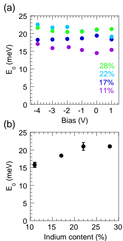
Figure 71: (a) Dependence on applied bias of the Urbach energy E_0 determined in the B-region of BPCS spectra for InGaN QW layers with different mean In content. (b) Mean values of E_0 averaged over the applied biases and plotted as a function of the mean In content of the corresponding InGaN/GaN solar cell.
