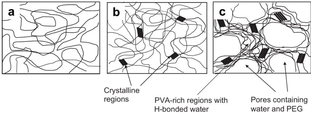
Figure 12 Schematic of a PVA theta-gel formation is shown here: a) PVA-PEG water mixture at 90 °C is a uniform solution; b) as the solution is cooled down phase separation begins and forces the PVA to form crystalline domains; c) with further cooling to near room temperature, phase separation results in the formation of pores containing water surrounded by PVA rich regions. 33
