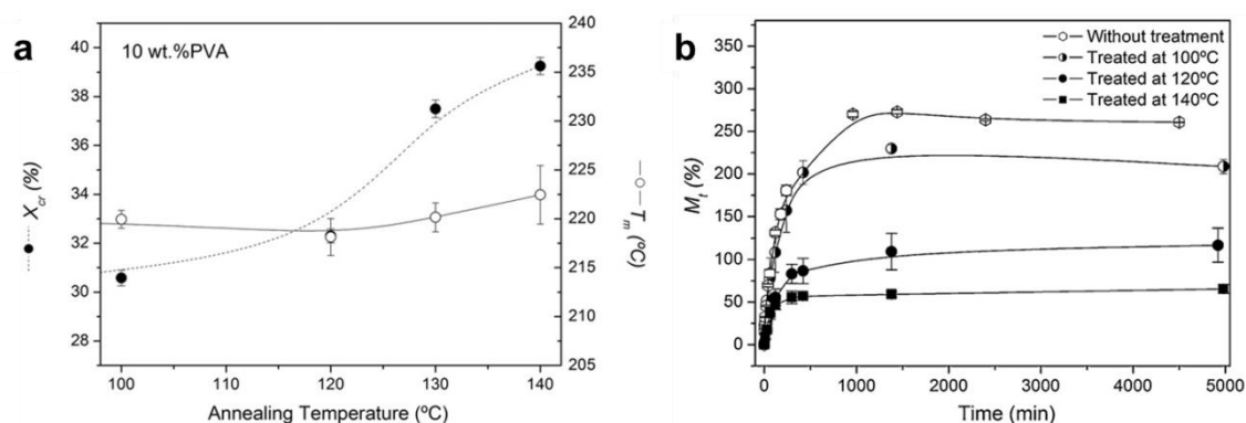
Figure 13 a) Crystallinity degree ( X_{cr} %) and melting temperature ( T_m ) of hydrogels prepared from 10 wt.% PVA solution as a function of annealing temperature; b) Absorbed saline solution (%) at 37 °C as a function of time for untreated and annealed 5 wt.% hydrogels. 40
