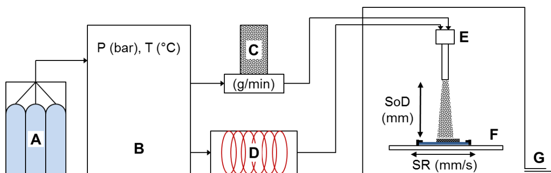
Figure 101 Schematic drawing of the cold spray apparatus: a) Gas tank bundle; b) Control cabinet c) Powder feeder; d) Gas heater; e) Spray gun; f) Moving sample holder; g) Dust extractor.
