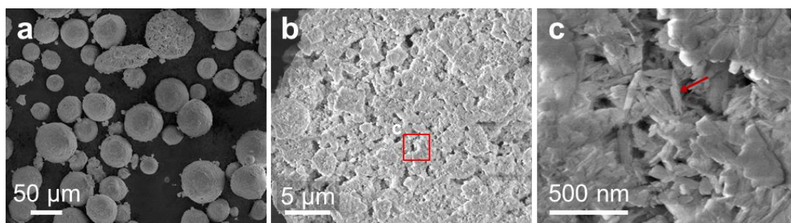
Figure 56 Scanning electron microscopy imaging of non-calcined HA particles: a) Observation of particles morphology; b) Observation of crushed particle with S.E. detector; c) Zoom of b) . Red arrow: submicronic particle.
