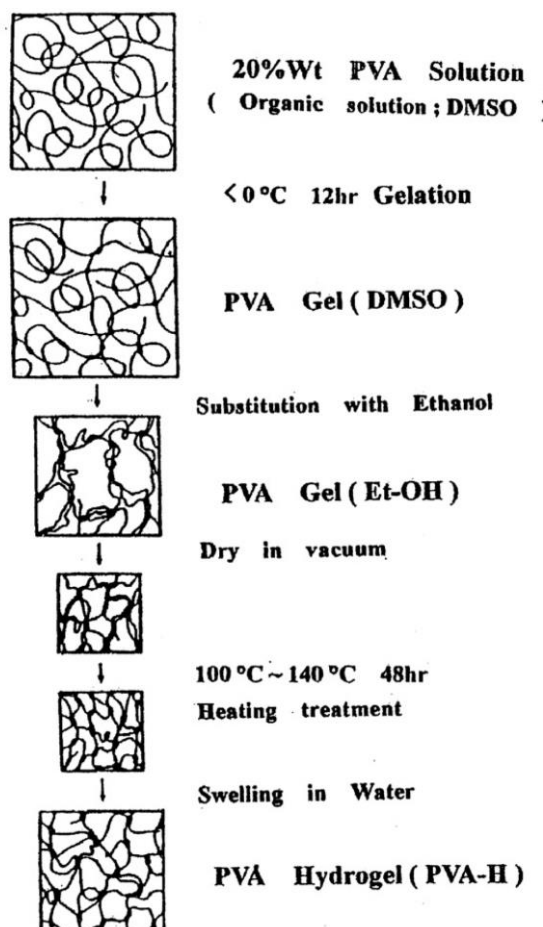
Figure 14 Steps of dehydration/annealing crosslinking method. 35,41
