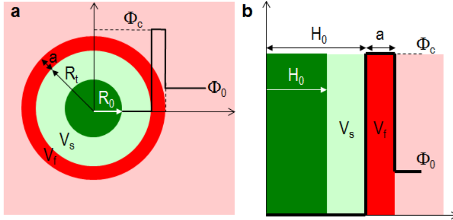
Figure 85 PVA concentration profile as a function of the distance to the substrate interface for a spherical substrate (a) and a flat substrate (b).
