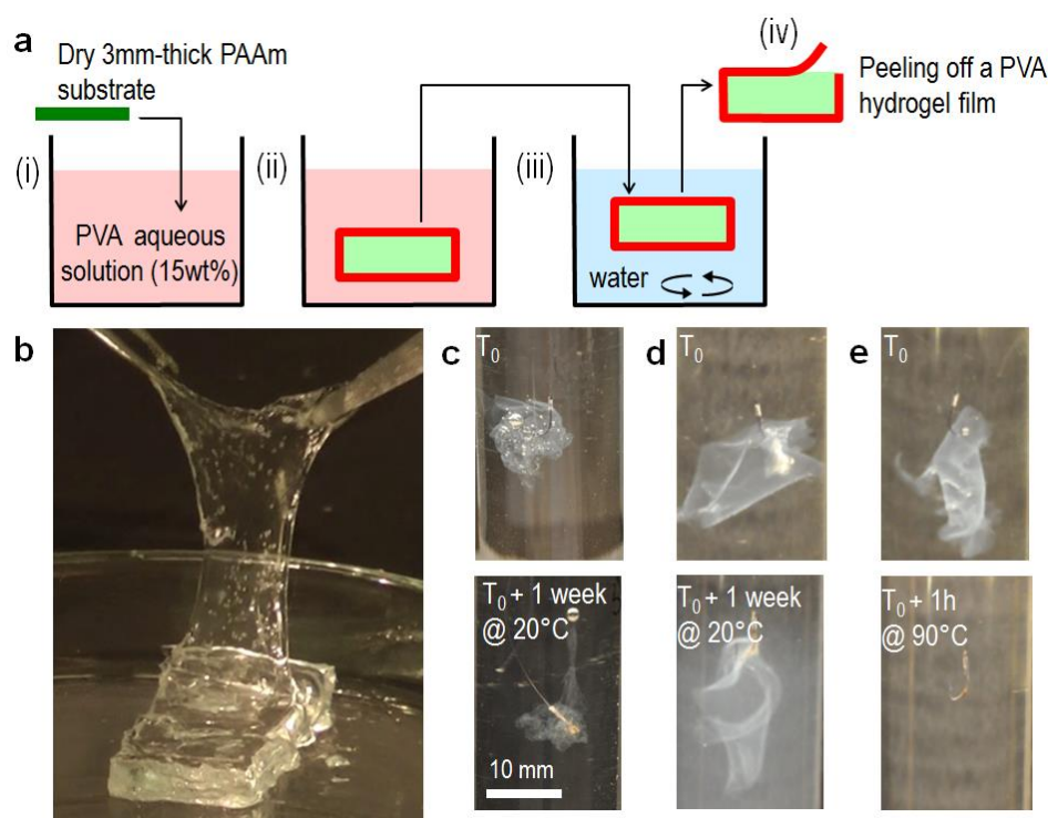
Figure 77 a) Schema of the swelling induced gelation experiment using a PAAM substrate in a 15 wt% PVA aqueous solution; b) Peeling off a PVA hydrogel film from a PAAM substrate; c-d) Stability experiment done on PVA hydrogel films produced by soaking of PAAM substrates in 10 wt% PVA aqueous solutions for 3h and in 15 wt% PVA aqueous solution for 19h, respectively; e) Dissolving of PVA hydrogel films produced by soaking of PAAM substrates in 15 wt% PVA aqueous solution for 19h.
