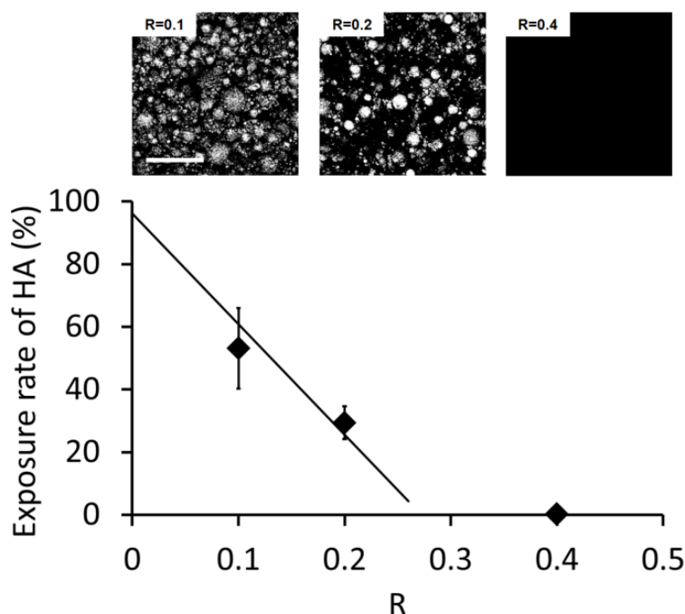
Figure 65 Surface exposure of HA as a function of R. The full line is a linear fit based on data points at R=0.2 and 0.1, going through full exposure for R=0. Top images correspond to binarized BSE images used for image analysis. Scale bar is 100 \mu m.
