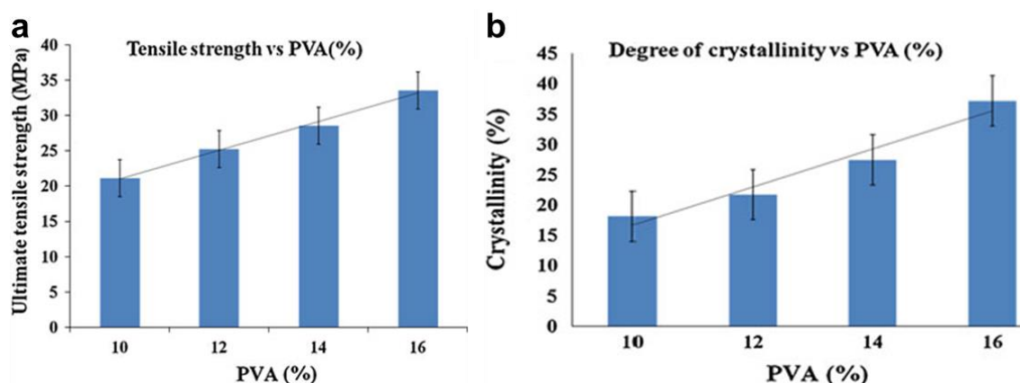
Figure 28 a) Ultimate tensile strength as a function of PVA concentration; b) Degree of crystallinity as a function of PVA concentration. 58
