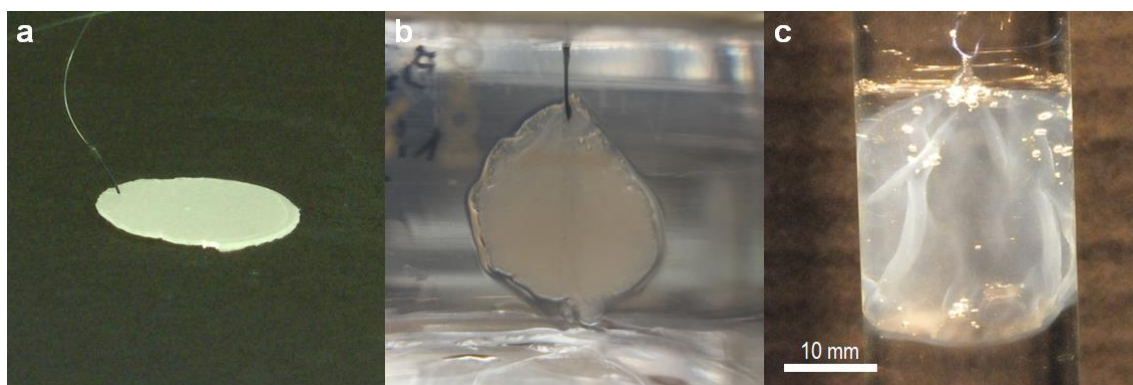
Figure 86 PVA hydrogel film gelation around hydrosoluble PEG substrate. a) Uncross-linked PEG substrate; b) Soaking in PVA aqueous solution; c) PVA film in water.
