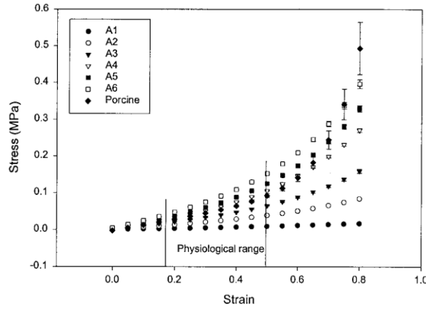
Figure 26 Stress–strain relationship of PVA hydrogel cross-linked by freezing/thawing method (1 to 6 cycles) compared to a porcine aortic root. 53
