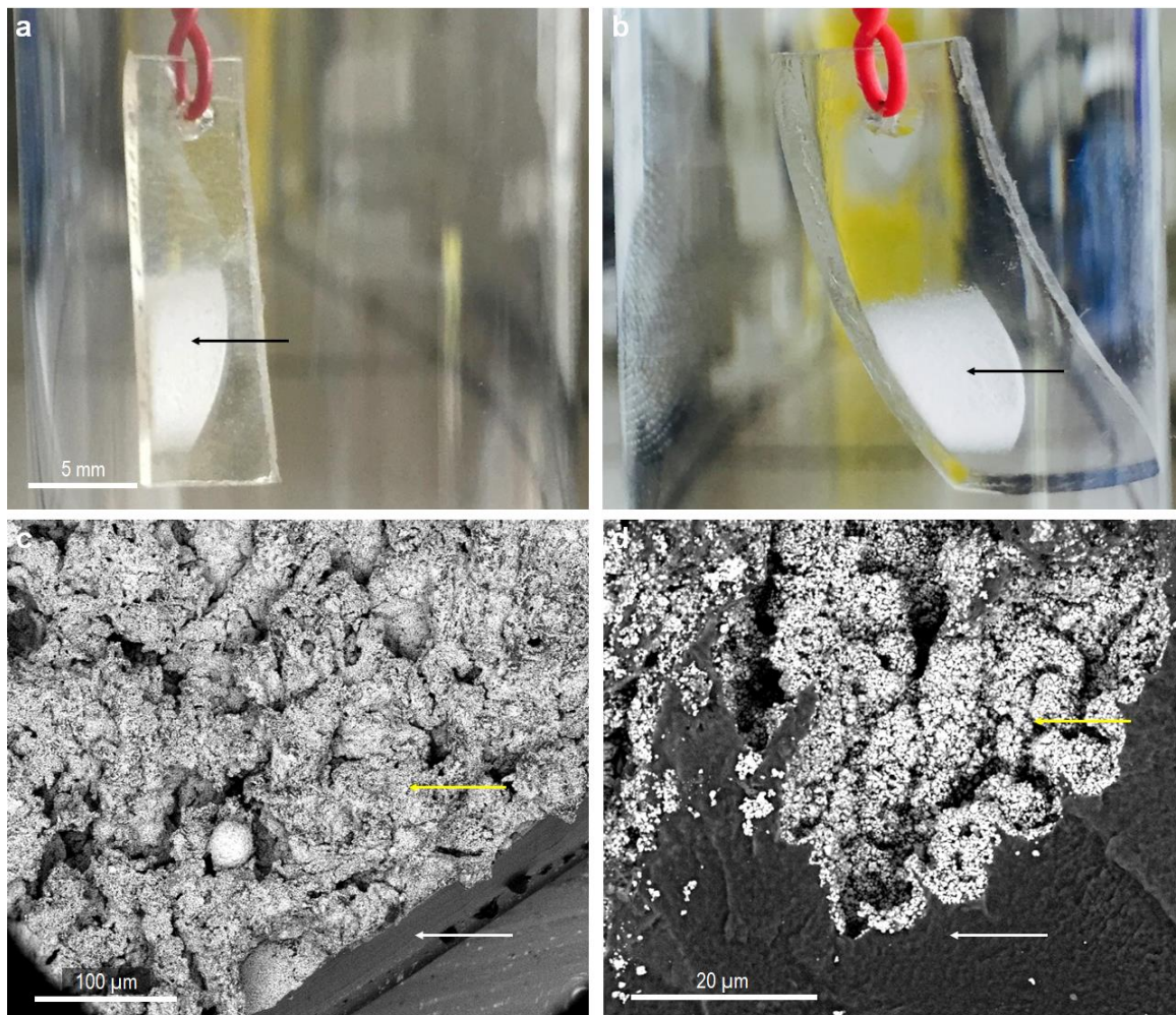
Figure 111 Swelling in water of HA coated PVA substrate ( T=200 °C, P=10 bar, D=30 mm) at T_0 (a) and after 1 week (b) under magnetic stirring at 37^\circ\text{C} . Scanning electronic microscopy using backscattered electron detector in low vacuum mode of HA coated PVA hydrogel substrate: c) Top surface view; d) Cross-section view.
