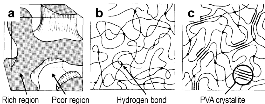
Figure 11 Schematic representations of: a) liquid-liquid phase separation, resulting in the development of an interconnected structure of polymer-rich and polymer-poor regions, b) a network formed by hydrogen bonding, c) PVA crystallite formation. (Modified from Kawanashi). 37
