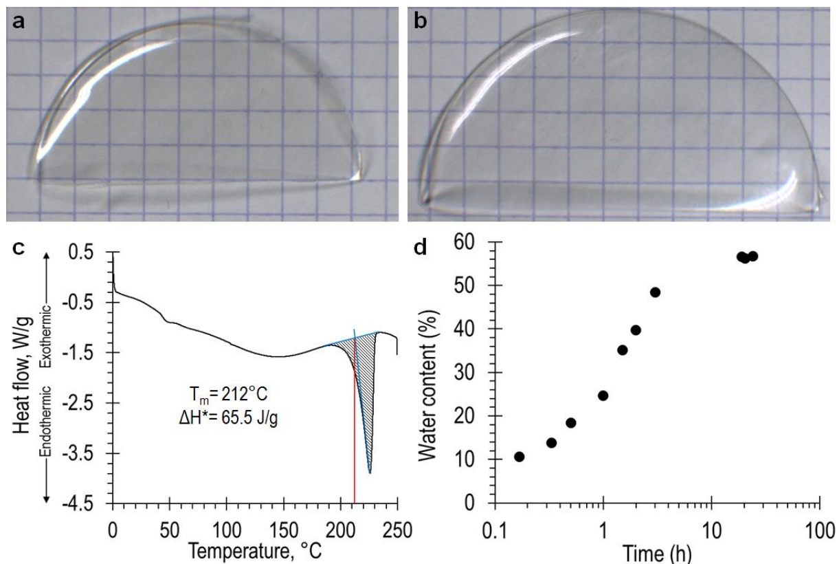
Figure 104 Characterization of PVA substrate used for cold spray: a) Dry PVA substrate obtained by solvent casting; b) Hydrogel PVA substrate swollen at equilibrium; c) DSC thermogram of dry PVA film upon heating from 0 to 250^\circ\text{C} at 10^\circ\text{C}/\text{min} ; d) Water content of bare PVA hydrogel substrate as a function of time.
