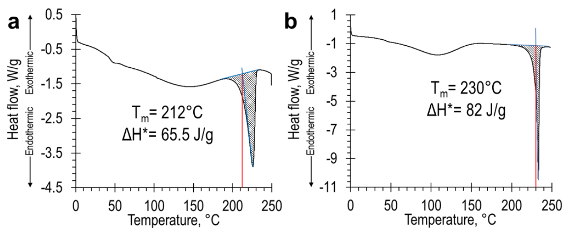
Figure 53 DSC thermogram of dry PVA film (a) and fibers (b) upon heating from 0 to 250°C at 10°C/min.
