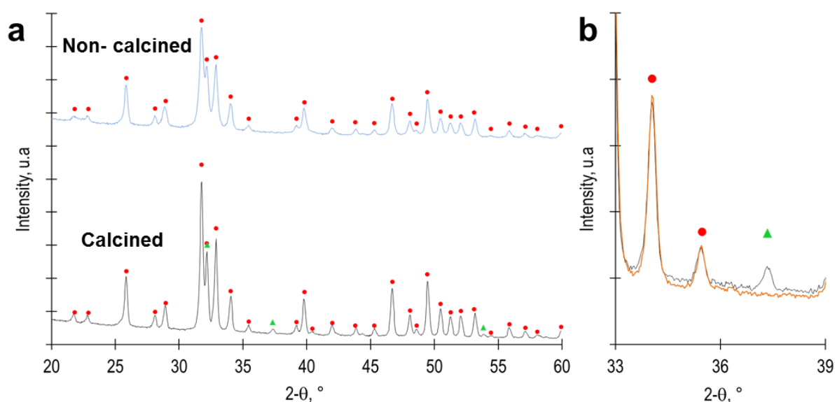
Figure 57 a) XRD spectra of calcined (—) and non-calcined (—) HA particles; b) XRD spectra, centered on 33-39°, of calcined (—) and washed calcined HA (—). ICCD-PDF: HA (9-432) (●) and CaO (37-1497) (▲).
