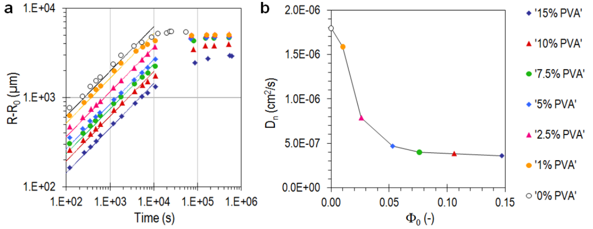
Figure 83 a) Swelling kinetics of the PAAM beads in PVA solutions with different concentration. Solid curves are fits using Eq. 1; b) Diffusion coefficients of the PAAM bead in PVA solution of different concentration, obtained from fitting the data in (a) with Equation 1. 20,21
