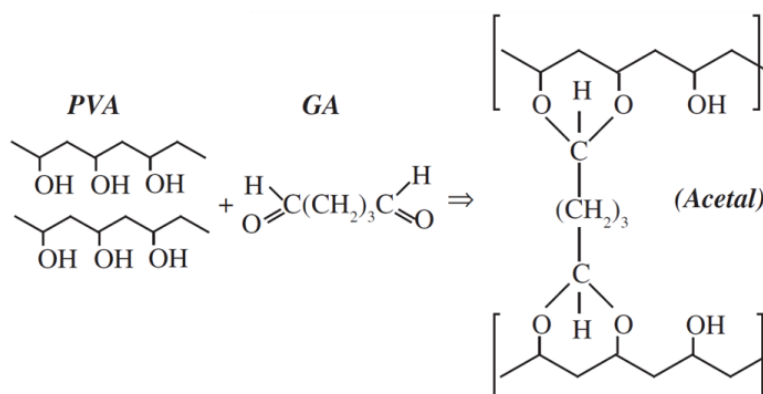
Figure 3 PVA and glutaraldehyde crosslinking in acidic environment. 16
