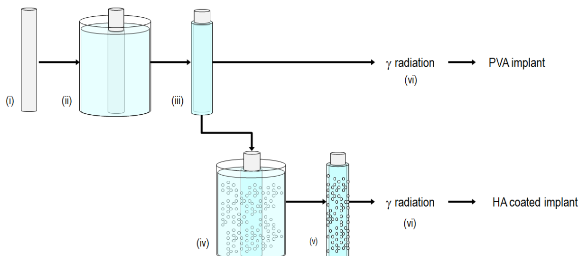
Figure 69 Schematic representation of the implant fabrication process: (i) Dry fiber bundle, (ii) Soaking in PVA aqueous solution, (iii) PVA hydrogel fibres embedded in PVA hydrogel matrix physically cross-linked by freezing-thawing cycles, (iv) Soaking of PVA coated bundle in PVA/HA aqueous solution, (v) PVA hydrogel fibres coated with HA particles embedded in a PVA hydrogel matrix physically cross-linked by freezing-thawing cycles, (vi) Sterilization by gamma-radiation at 25 kGy.
