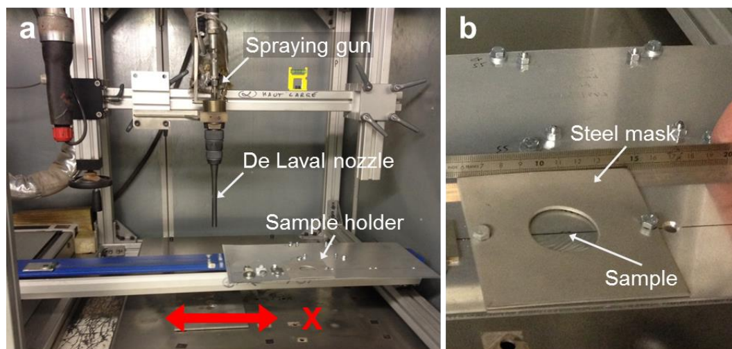
Figure 102 a) Spraying booth; b) Sample holder
