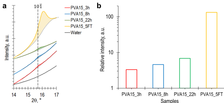
Figure 78 a) X-ray diffraction spectra of PVA hydrogel films produced by swelling induced gelation and compared to film prepared by freezing/thawing (5 cycles) and pure water; b) Relative intensity of the peaks underlined in (a).
