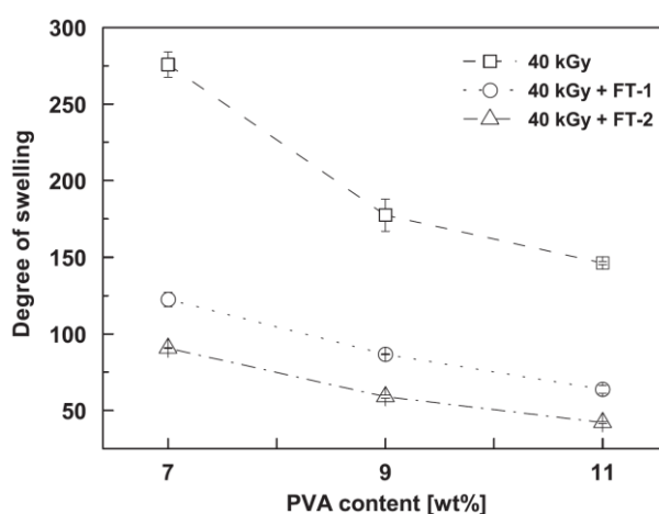
Figure 23 The degree of swelling as a function of PVA content. 21
