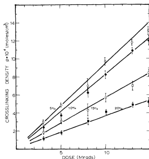
Figure 5 Variation of the crosslinking density p (mole/cms) of PVA networks with dose D , and initial concentration C , of aqueous PVA solutions. (Temperature of irradiation 30°C.) Bars represent standard error of the mean. 23
