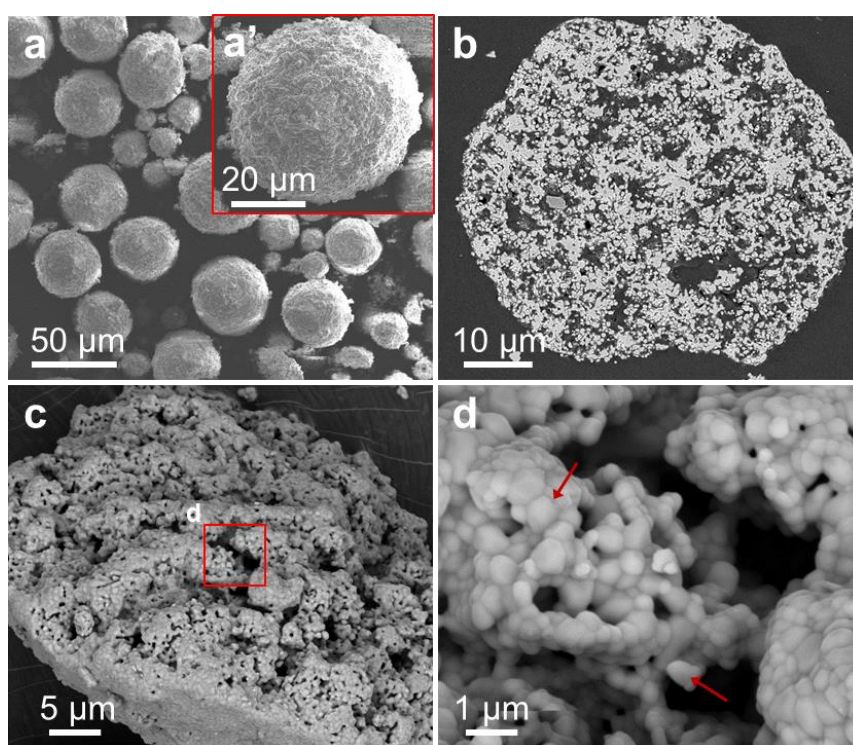
Figure 55 Scanning electronic microscopy imaging of calcined HA particles: a-a') Low magnification observations of the general aspect of the particles; b) Cross-section of a single particle observed with B.S.E. detector; c) Crushed particle observed with B.S.E. detector; d) Zoom of c) . Red arrow: submicronic particle.
