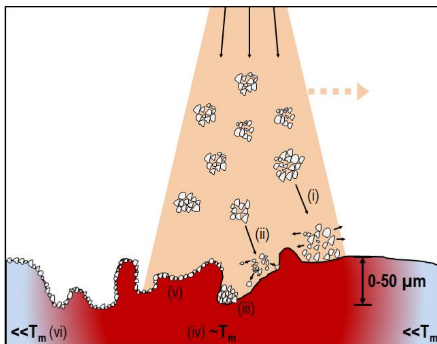
Figure 113 Schematic drawing of the coating formation mechanisms: (i) particle fragmentation at impact, (ii) particle fragmentation by impact of following particles, (iii) few particles remain intact after spraying, (iv) softening of the substrate by gas stream, (v) monolayer coating of submicronic particles, (vi) decrease of substrate temperature.
