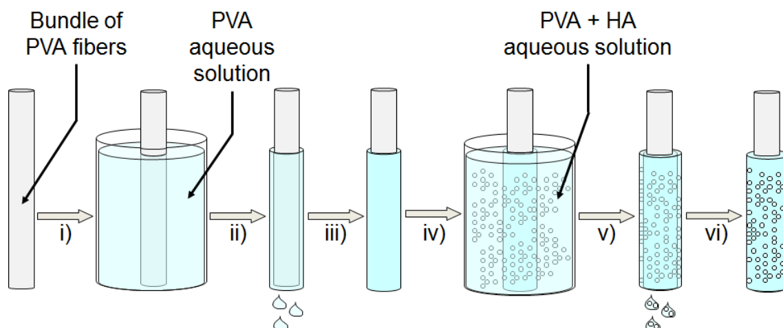
Figure 61 Schematic representation of the coating process.
