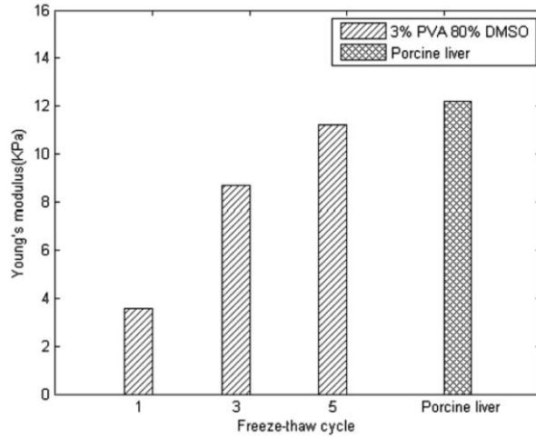
Figure 29 Young's modulus as a function of the number of Freezing/Thawing cycles. 59
