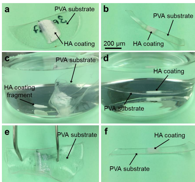
Figure 119 Swelling in water of non-calcined (a,c,e) and calcined (b,d,f) HA coated PVA substrate ( T=200\text{ }^{\circ}\text{C} , P=10\text{ bar} , D=30\text{ mm} ). After swelling (a and b); After 3h of swelling(c and d), After gentle scratching(e and f).
