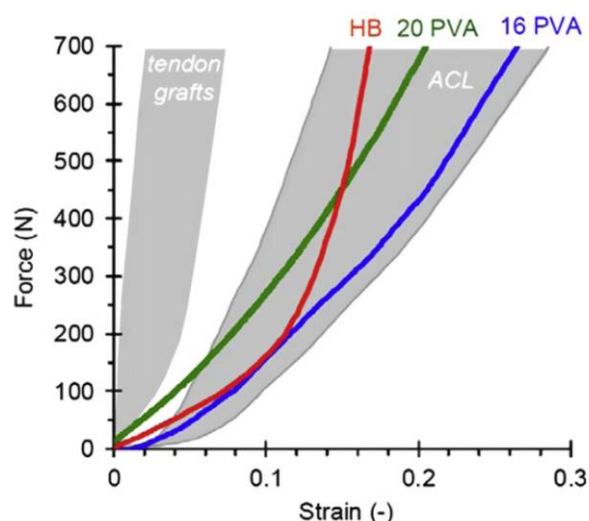
Figure 36 Tensile force versus strain for different PVA hydrogel fibre constructs (red, blue and green curves). Shaded regions show the typical ranges for the native ACL and tendons used for autografts. 65
