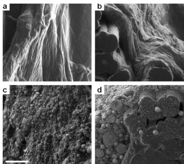
Figure 68 SEM observations of precoated PVA samples pulled out from a matrix of PVA ( a : surface view, b : cross-section) or PVA/HA ( c : surface view, d : cross-section). Scale bar is 100 \mu m.
