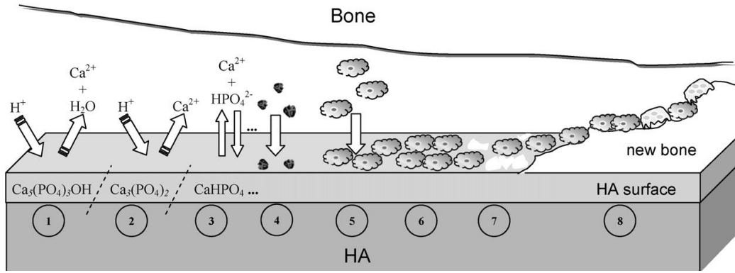
Figure 42 Schematic diagram representing the phenomena that occur on the surface of hydroxyapatite after implantation. 81
