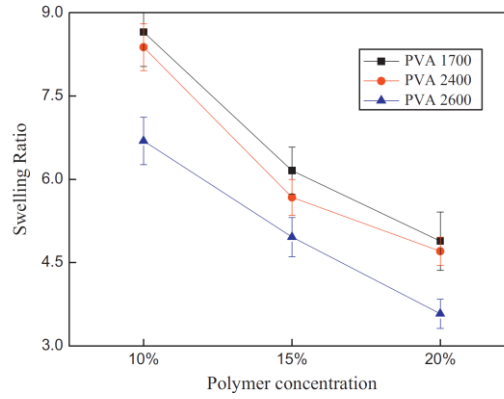
Figure 21 Swelling ratio as a function of polymerization degree and of polymer concentration for PVA hydrogels in phosphate buffer solution (PBS). 42
