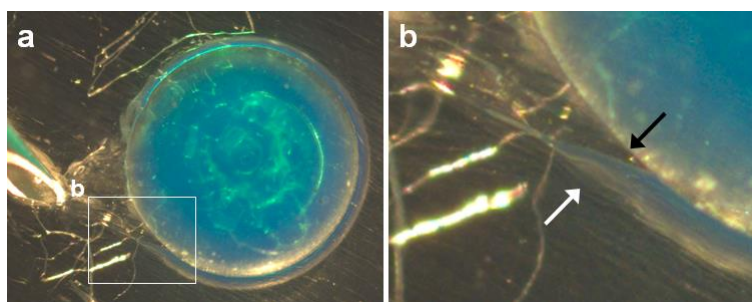
Figure 80 a-b) Microscopic observation of the in-situ detachment of a PVA hydrogel film (white arrow) formed at the surface of a PAAm bead (black arrow) swelling in a 10 wt% PVA aqueous solution after 1 h.
