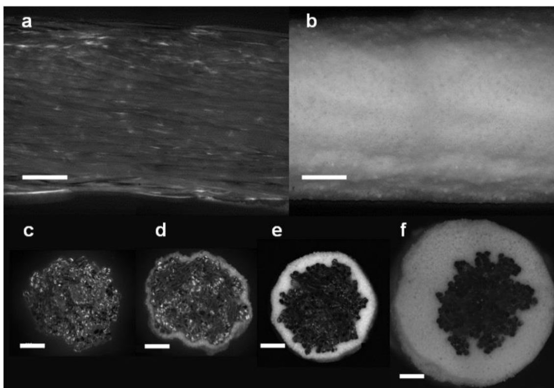
Figure 62 Optical micrographs: surface views of a PVA coated bundle (a) and a PVA/HA coated bundle with R=2.5 (b); cross-sections of a PVA coated bundle (c) and PVA/HA coated bundles with R=0.4, 0.2 and 0.1 (d-f). Scale bar is 500 \mu m.
