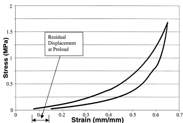
Figure 24 Compressive stress-strain curve of physically cross-linked PVA hydrogel. 50
