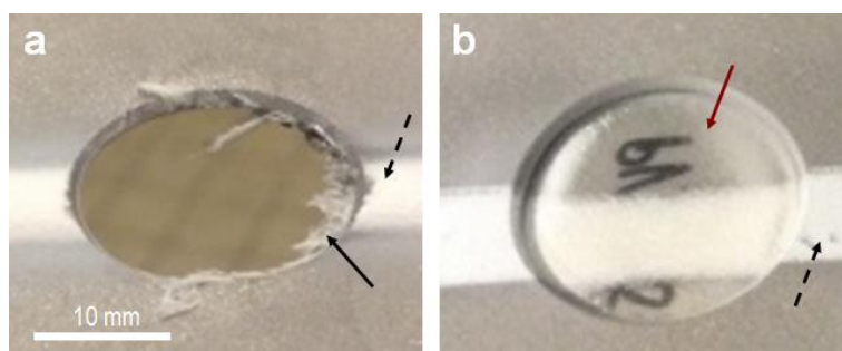
Figure 105 Substrate state after one pass at T=200\text{ }^{\circ}\text{C} , P=1\text{ Mpa} and D=30\text{ mm} : a) Cold spraying of hydrogel PVA substrate; b) Cold spraying of dry PVA substrate. Black arrow: rest of destroyed PVA hydrogel substrate; black dashed arrow: HA pass; red arrow: dry PVA substrate.
