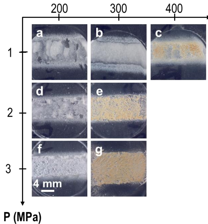
Figure 116 Macroscopic view of the surface of non-calcined HA coated PVA substrates cold sprayed with different temperature and pressure for a stand-off distance of 60 mm.
