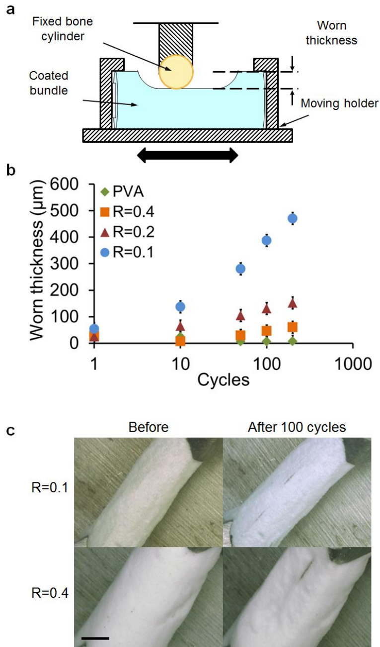
Figure 66 Characterization of the coating resistance to wear: a) Schematic representation of the experimental set up; b) Worn thickness versus number of cycles for all sample types; c) Comparison of surface states before testing and after 100 cycles for R=0.1 and 0.4. Scale bar is 1 mm.
