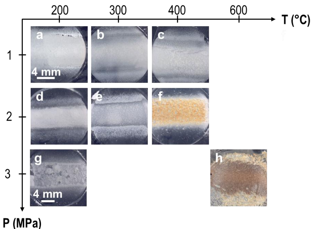
Figure 117 Macroscopic view of the surface of non-calcined HA coated PVA substrates cold sprayed with different temperature and pressure for a stand-off distance of 100 mm.
