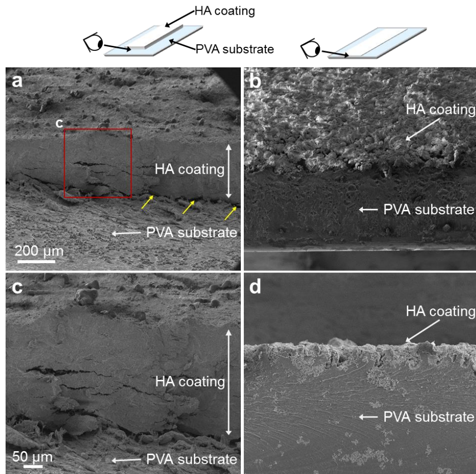
Figure 118 Scanning electronic microscopic observations of the non-calcined HA coating in tilted view ( a , c ) and of the calcined HA coating in tilted view ( b ) and in fractography ( d ).
