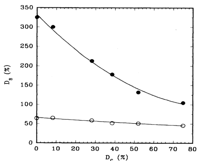
Figure 20 Swelling of chemically cross-linked PVA membrane as a function of the degree of crosslinking (● in water; ○ in ethanol). 45
