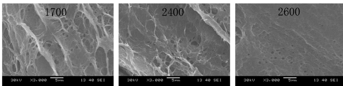
Figure 15 SEM micrographs of the cross-sections of PVA/PVP hydrogels (10%PVA/PVP) with polymerization degree of 1700, 2400 and 2600. 42
