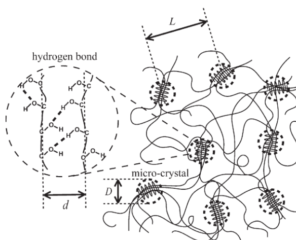
Figure 6 Schematic representation of the network structure of PVA gels crosslinked by microcrystals. 25
