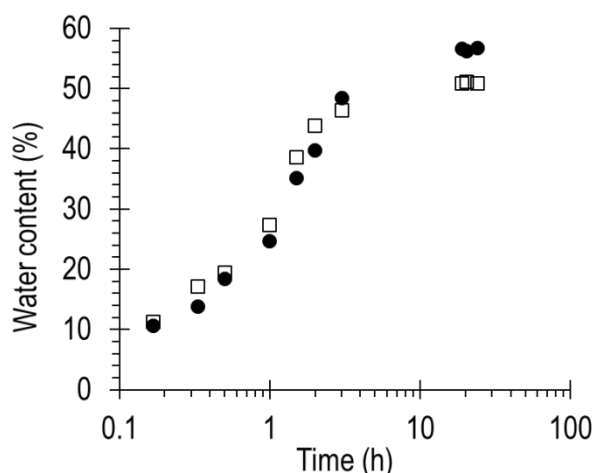
Figure 112 Water content of bare (●) and HA coated (□) PVA hydrogel substrate as a function of time.
