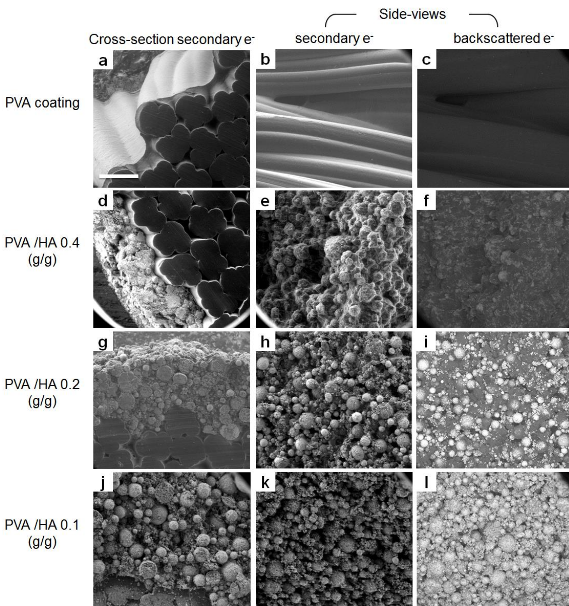
Figure 64 SEM observations of the cross-sections and surfaces of PVA coated (a-c) and PVA/HA coated samples with R=0.4 (d-f), 0.2 (g-i) and 0.1 (j-l). Images c, f, i and l show the exact same ROIs as b, e, h and k using backscattered electron imaging. Scale bar is 100 \mu m.
