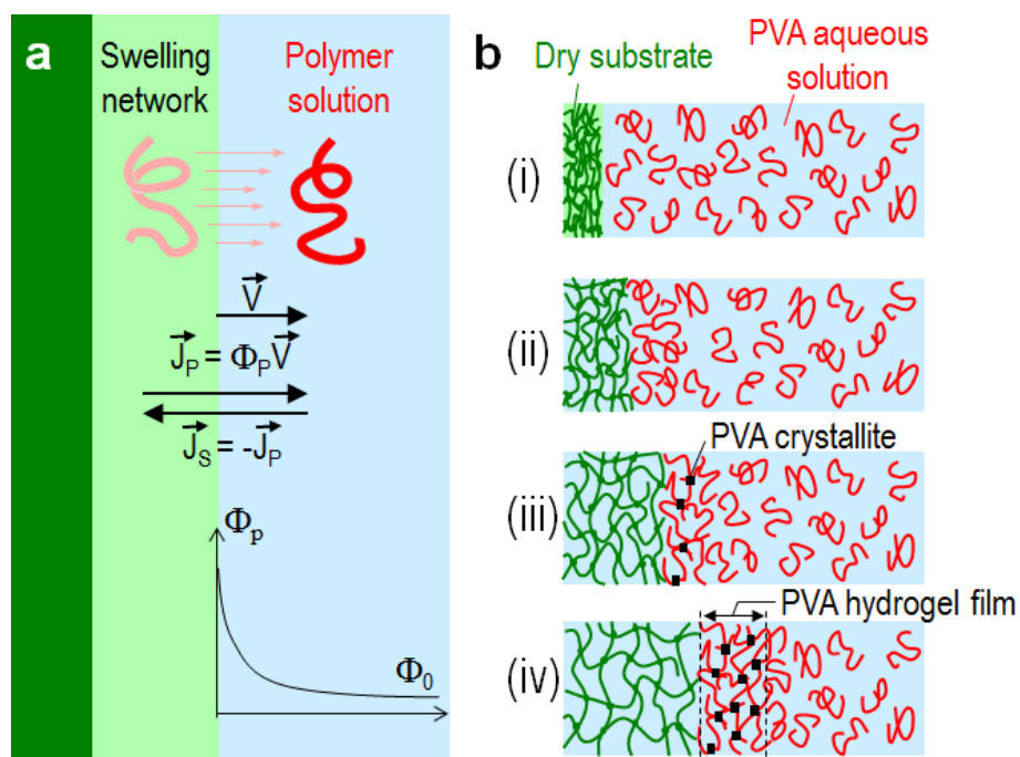
Figure 76 a) Schematic drawing of the mass transport phenomenon of the surface of a swelling substrate in a polymer solution; b) Schematic drawing of the swelling induced gelation concept.
