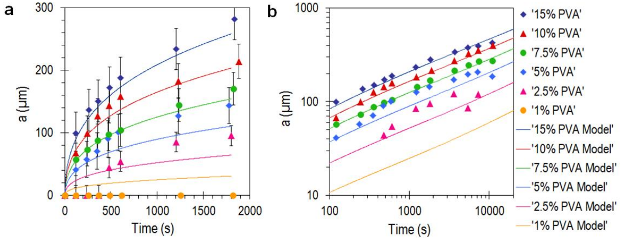
Figure 84 a) Film thickness ( a \mu\text{m} ) as a function of time ( <2000 s); b) Log-log chart of the film thickness as a function of time. Solid curves are theoretical prediction using the model given by the Equation 4.
