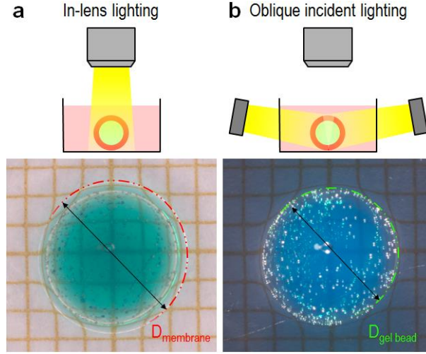
Figure 82 Measurement method: a) Film surface observation by in-lens lighting; b) Substrate surface observation by oblique incident lighting.
