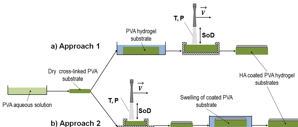
Figure 100 Studied approaches to produce cold-sprayed ceramic coatings on PVA hydrogels: a) Approach 1: swelling and spraying. b) Approach 2: spraying and swelling.
