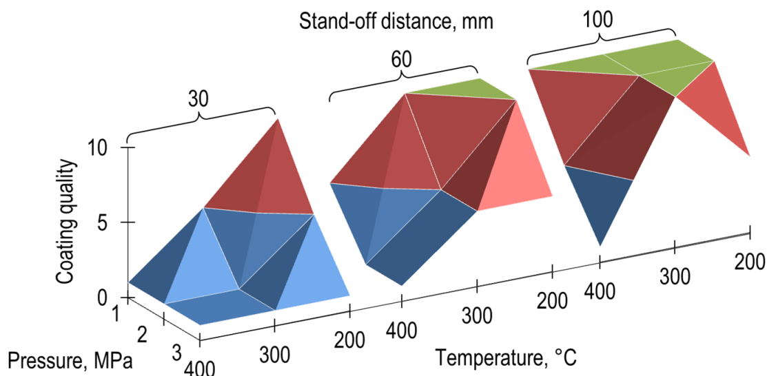
Figure 122 Non-calcined particle coating quality as a function of the temperature, the projection distance, and the pressure.
