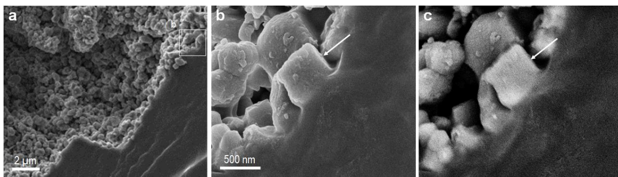
Figure 109 Ultra high magnification scanning electronic microscopy imaging of the interface between HA nano-grains and dry PVA substrate coated at T=200\text{ }^{\circ}\text{C} , P=10\text{ bar} , D=30\text{ mm} . a) Interface between HA nano-grains and dry PVA substrate; b) View of a single HA nano-grain (white arrow) in secondary electron detection; c) Same view in backscattered electron detection.
