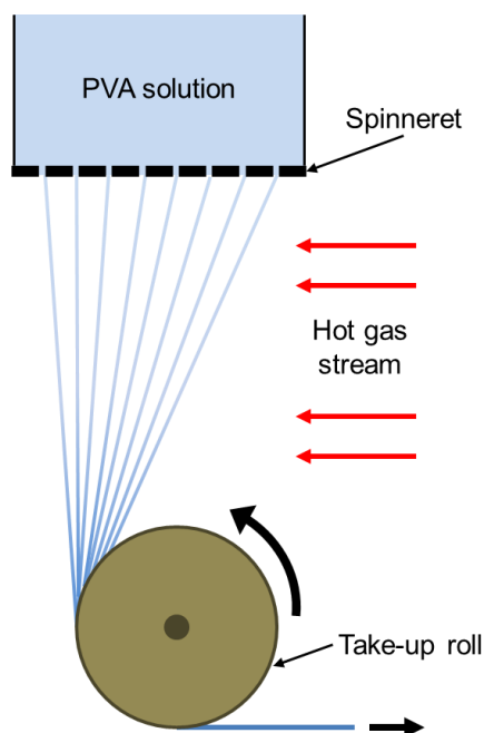
Figure 49 Schematic description of the dry spinning process
