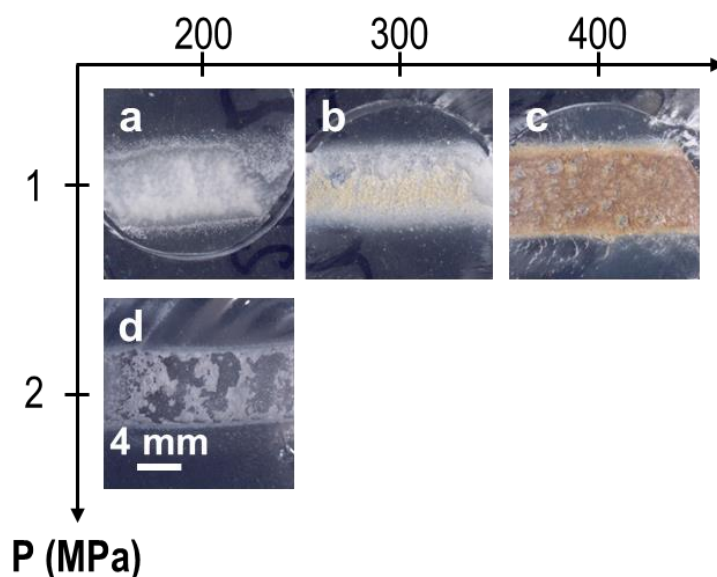
Figure 115 Macroscopic view of the surface of non-calcined HA coated PVA substrates cold sprayed with different temperature and pressure for a stand-off distance of 30 mm.
