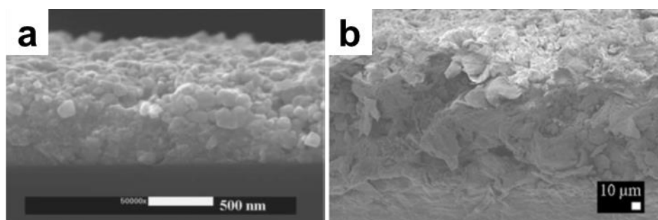
Figure 114 a) Coatings of \text{WO}_3 on silicon substrate ( 300^\circ\text{C} , 0.7 \text{ MPa} ); 1 b) HA coating on PEEK substrate ( 400^\circ\text{C} , 1.4 \text{ MPa} ). 2
