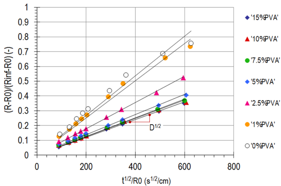
Figure 123 Log-Log plot of the Equation 2. Solid lines are linear curves of slope equals to D_n^{1/2} .
