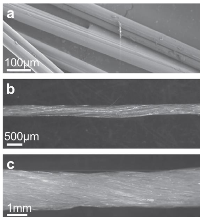
Figure 51 Microscopic observations of dry PVA fiber (a), thread (b) and bundle (c). Reproduced with the authorization of Bach et al. 1
