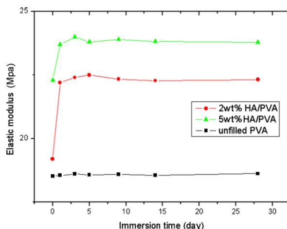
Figure 45 Effect of HA content on the Young's modulus of PVA/HA composite hydrogels. 98
