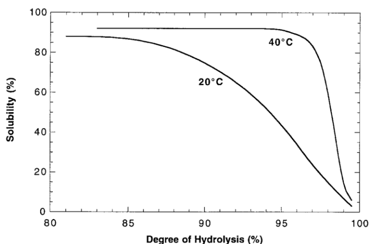
Figure 2 Solubility of PVA ( M_w=77000 g/mol) as a function of degree of hydrolysis at dissolution temperature of 20 and 40°C. 13
