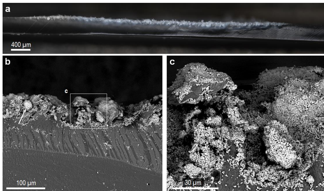
Figure 108 Cross-section views of dried PVA substrate coated at T=200\text{ }^{\circ}\text{C} , P=10\text{ bar} , D=30\text{ mm} . a) Optical microscopy of the whole HA coating; b) and c) Scanning electronic microscopy using backscattered electron detector of the interface between the HA coating and the PVA substrate.
