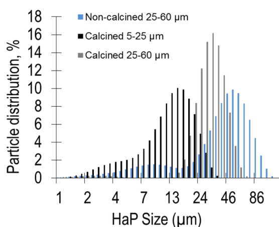
Figure 54 Volume distribution of particle diameter for non-calcined and calcined particles.
