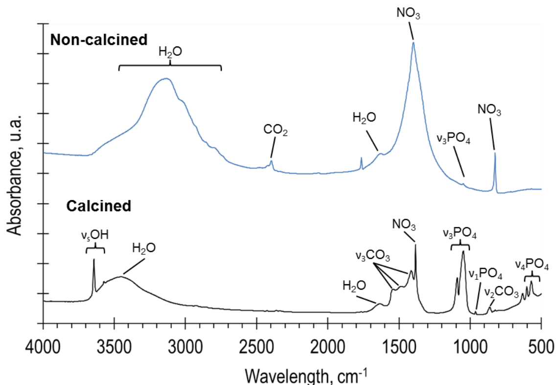
Figure 121 FTIR spectra of salts issued from waters used to wash calcined (—) and non-calcined (---) HA before spraying.
