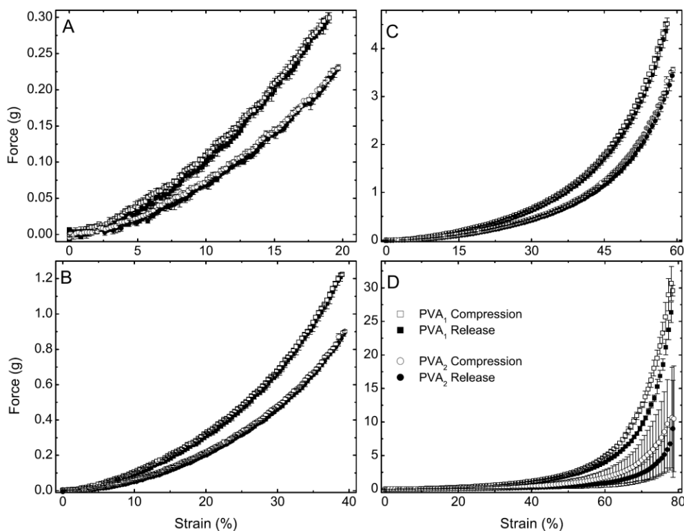
Figure 25 Typical force response profiles during a compression/release experiment performed on a PVA1 and PVA2 beads swollen in H 2 O. Beads were compressed to 20 (A), 40 (B), 60 (C), and 80% (D) strain (applied at 4% s -1 ). 51
