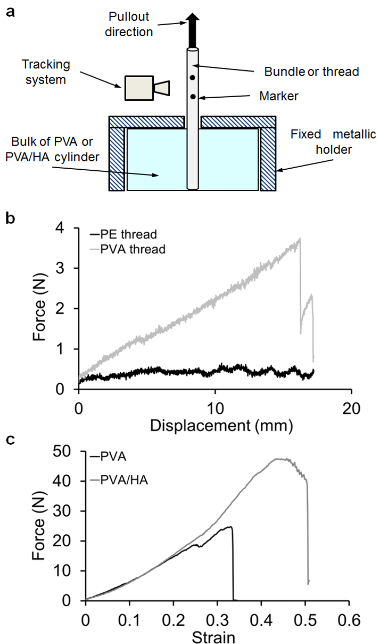
Figure 67 Characterization of the coating adhesion: a) Schematic representation of the pull out test set up. b) Force-displacement curves for PVA and PE threads pulled out of a PVA cross-linked matrix. c) Force-strain curves for PVA pre-coated bundles pulled out of a cross-linked matrix of PVA or PVA/HA (R=0.2)
