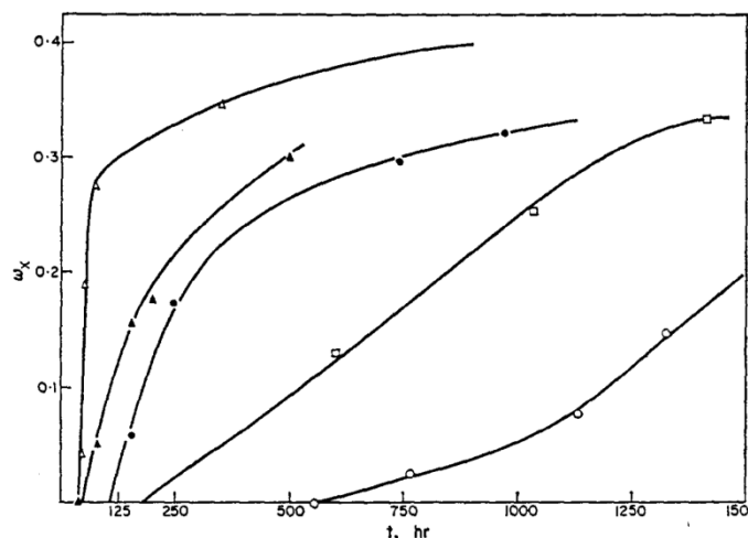
Figure 8 Degree of crystallinity ( w_x ) of PVA gel in function of drying time for different rate of evaporation depending on the nature of the drying agent ( \circ K_2Cr_2O_7 hydrate; \square KBr \bullet Ca(NO_3)_2 hydrate; \blacktriangle MgCl_2 hydrate \Delta SiO_2 ). 24
