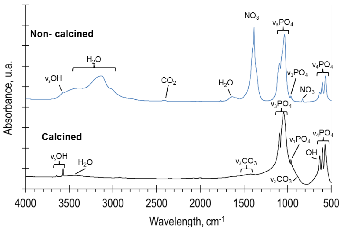
Figure 58 FT-IR spectra of calcined (—) and non-calcined (—) HA particles.
