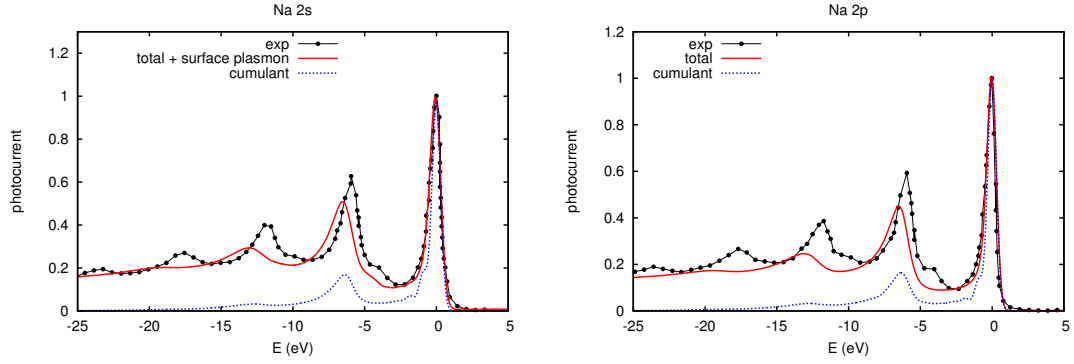
Figure 6.2: Comparison of the experimental photoemission spectrum to the spectrum calculated using the TOC11 + extrinsic + interference approach: Left, Na 2s; right: Na 2p. The red solid lines are total calculations, including secondary electron background, black with circles are experimental data [47], and blue dashed are calculated TOC11 intrinsic spectral functions. The total Na 2s calculated spectrum also includes an approximation to the surface plasmon contribution. The spectra are angle-integrated. Original experimental data were in arbitrary units: here we have normalized them to the main-peak intensities. The calculated QP energies have been aligned with respect to the experimental QP peaks otherwise the GWA 2s level is too deep by about 5 eV, and the 2p level by about 3 eV (see table 2.1). The zero of the energy axis is set to be the QP energy of the experiment. Gaussian broadening of 0.3 eV has been used in all calculated spectra. The extrinsic and interference effects have been calculated by my co-author J. Kas and J. Rehr in Ref. [20].
