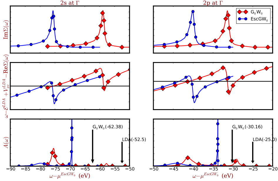
Figure 2.8: Intrinsic spectral function of the sodium 2s state at the \Gamma point (lower panel). Red curves with diamonds are G_0W_0 results, blue curves with circles are \text{EsGW}_0 results. The position of the LDA band at \Gamma is given by the black arrow labeled LDA. The arrow labeled G_0W_0 indicates the quasi-particle energy that one would obtain by the usual first-order approximation based on a linearization of the self-energy as discussed in equation (2.44). The upper two panels show the imaginary and shifted real parts of the GW self-energy. The zero of the energy axis is set to be the \text{EsGW}_0 Fermi energy.
