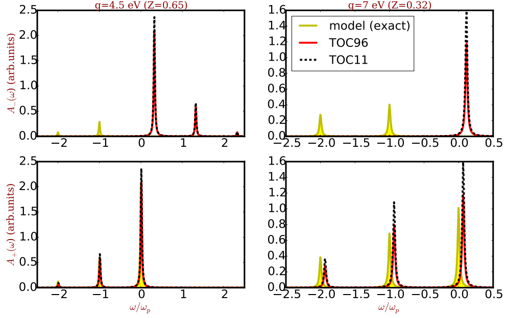
Figure 4.9: The spectral functions of the two-level hole-plasmon coupling Hamiltonian. Left panel: the coupling g = 4.5 eV that is consistent with bulk sodium bottom valence. Right panel: the coupling g = 7 eV that yields the QP renormalization factor \mathbf{Z} = 0.32 . The horizontal axis of the right panel has been kept until the range of our interest. All other parameters are the same as in Fig. 4.7. Also the horizontal axes of the left and right panels are defined analogously to previous figures. Upper and lower panels are the spectra of the anti-bonding and bonding orbitals, respectively. The Lorentzian broadening \eta = 0.1 is used in all plots. The yellow filled curves are the exact spectral functions of the model Hamiltonian in equation (4.29). The red curves are the spectral functions calculated using the TOC96 in equation (4.67). The black dashed curves are the cumulant spectral functions calculated with the TOC11 in (4.70).
