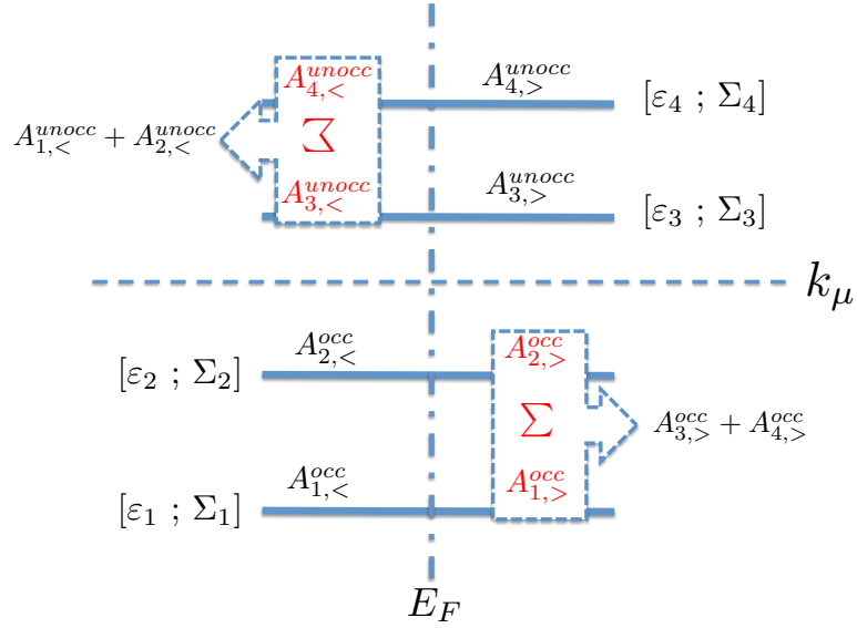
Figure 5.6: A schematic illustration of the four-level system. The states \varepsilon_1 and \varepsilon_2 are below the chemical potential \mu , \varepsilon_3 and \varepsilon_4 are states above the chemical potential. The self-energy of each state is \Sigma_i . The electron removal spectral functions of the occupied states (below the chemical potential) are A_{1,<}^{occ} and A_{2,<}^{occ} . The electron addition spectral functions of the unoccupied states (above the chemical potential) are A_{3,>}^{unocc} and A_{4,>}^{unocc} . The total electron removal spectrum of the unoccupied states are A_{1,<}^{unocc} + A_{2,<}^{unocc} , which equals to the sum of electron removal spectrum of each unoccupied state A_{3,<}^{unocc} + A_{4,<}^{unocc} , however the individual spectrum of A_{3(4),<}^{unocc} (in red color) cannot be obtained by the constrained retarded cumulant. Analogously the total electron addition spectrum of the occupied states A_{1,>}^{occ} + A_{2,>}^{occ} equals A_{3,>}^{occ} + A_{4,>}^{occ} but the individual spectrum of A_{1(2),>}^{occ} (in red color) is missing.
