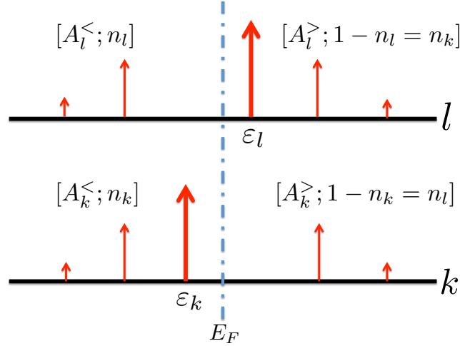
Figure 5.4: Schematic illustration of the spectrum of a two-level system. There are two quasi-particle states in the system: the state k and l are below and above the Fermi level, respectively. The quasi-particle energies of these two states are \varepsilon_k and \varepsilon_l as represented by the thick red peaks. The thin red peaks represent the satellites.
