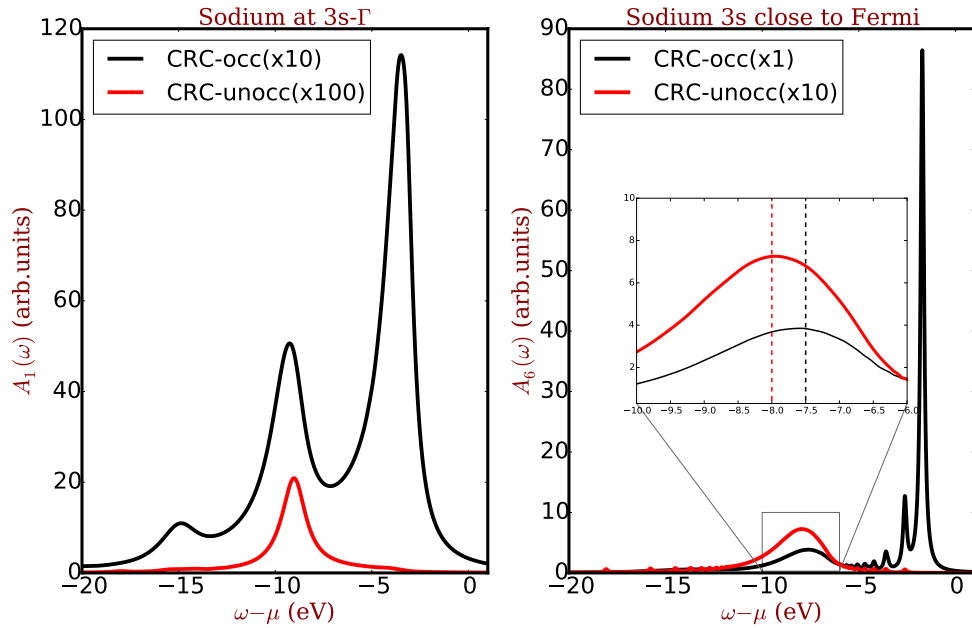
Figure 6.7: Intrinsic k -resolved spectra of Na 3s. Left panel: A_{k,<}^{occ} in Eq. (5.34) (black curve) and A_{k,<}^{unocc} in Eq. (5.36) where k_1 = [0, 0, 0] , i.e. the \Gamma point. Right panel: A_{k,<}^{occ} in Eq. (5.34) (black curve) and A_{k,<}^{unocc} in Eq. (5.36) where k_6 = [0.3125, 0, 0] , i.e. a state closer to the Fermi than \Gamma . All the spectra have been scaled (the \times numbers in the legend) in order to have a better comparison. The insert plots in the right panel show the \approx 0.5 eV discrepancy between the satellites of the A_{k,<}^{occ} and A_{k,<}^{unocc} .
