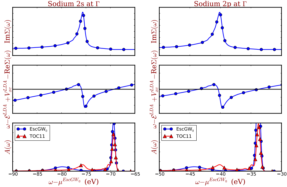
Figure 6.1: Intrinsic spectral functions of sodium 2s (left lower panel) and 2p (right lower panel) at the \Gamma point. Blue line with circles and red line with up-triangles are the results of the \text{EscGW}_0 and TOC11, respectively. The upper panels are the imaginary part of the \text{EscGW}_0 self-energies of these two core states. The middle panels are the shifted real part of the \text{EscGW}_0 self-energies that crosses zero at the QP energy. The lower panels show the intrinsic spectral functions where a 0.3 eV Gaussian broadening has been used in both the \text{EscGW}_0 and TOC11 spectral functions. The zero of the energy axis is set to be the \text{EscGW}_0 Fermi energy. The shoulders on the left hand side of the TOC11 QP peaks are spurious effects induced by the algorithm of the present multipole sampling, which is discussed in Fig. 6.3.
