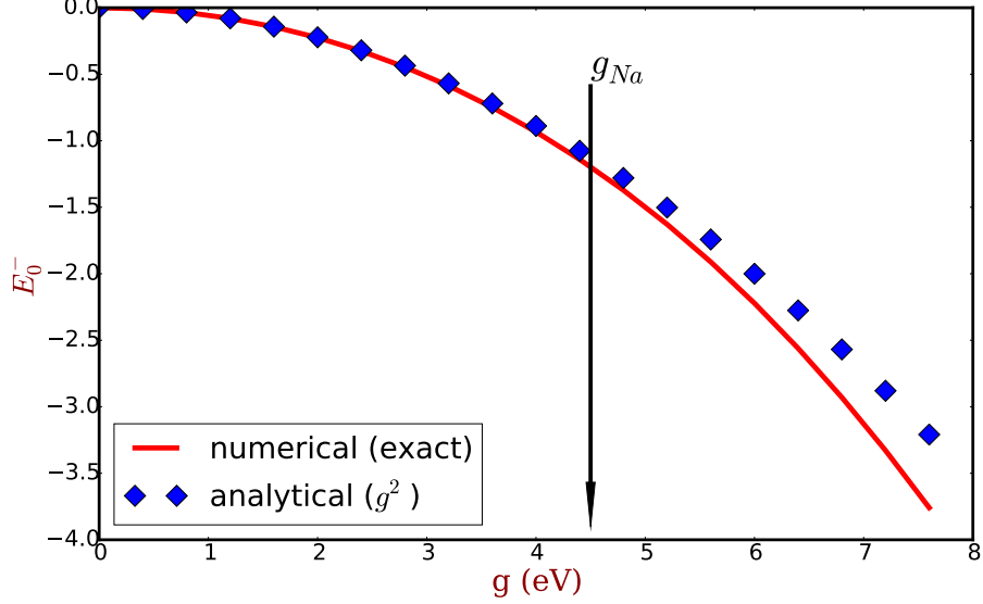
Figure 5.1: The performance of the second order expansion of the ground state energy in equation (5.1). The parameters are corresponding to bulk sodium bottom valence state, i.e. \varepsilon_0 = \mathbf{t} = 1.5 eV and \omega_p = 6 eV. Red curve is the exact numerical total energy E_0^- and blue diamonds are the total energy calculated from the second order expression in Eq. (5.1). In particular, g = 4.5 eV (black arrow labeled “ g_{Na} ”) corresponds to the sodium case where the error of the second order expansion is about 6%. This figure shows that Eq. (5.1) is a sufficiently good approximation to the exact total energy of the HPC-2.
