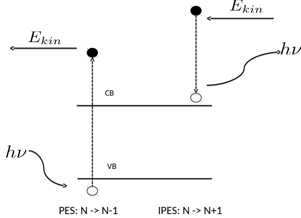
Figure 1.1: Schematic view of direct (on the left) and inverse (on the right) photoemission spectroscopy. The Fermi energy is between the valence (VB) and conduction (CB) band. In PES an electron is emitted with energy E_{kin} due to the excitation induced by the photon of energy h\nu . The IPES is the inverse process of PES where one electron is added to the system and one photon is emitted as Bremsstrahlung. In both processes we can measure E_{kin} and h\nu from which we can access the energy levels of the system using the energy conservation rule. The total number of electrons in the sample has been changed (from N to N \pm 1 ) in both processes. This is the reason why the excitations in (I)PES are called charged excitations, as opposed to the neutral excitations (e.g., excitons and plasmons) where the number of electrons is conserved during the excitation.
