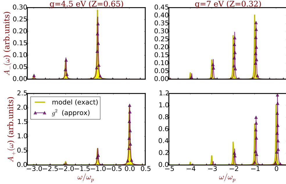
Figure 5.3: The spectral functions of the two-level hole-plasmon coupling Hamiltonian. Left panel: the coupling g = 4.5 eV yielding \mathbf{Z} = 0.65 . Right panel: a stronger coupling g = 7 eV yielding \mathbf{Z} = 0.32 . Yellow filled and purple curves with up-triangles are the exact and approximate (Eq. (5.12)) spectral functions, respectively.
