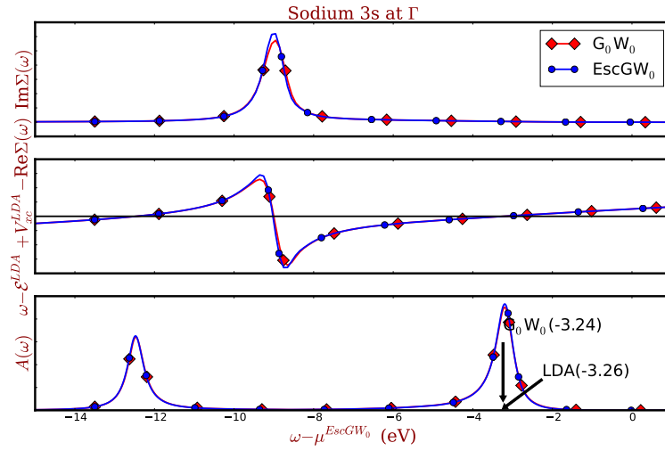
Figure 2.6: Intrinsic spectral functions of the sodium 3s band at the \Gamma point (lower panel). Red curves with diamonds are G_0W_0 results, blue curves with circles are \text{EscGW}_0 results. The position of the LDA band at \Gamma is given by the black arrow labeled LDA. The arrow labeled G_0W_0 indicates the quasi-particle energy that one would obtain by the usual first-order approximation based on a linearization of the self-energy as discussed in equation (2.44). The upper two panels show the imaginary and shifted real parts of the GW self-energy. The zero of the energy axis is set to be the \text{EscGW}_0 Fermi energy.
