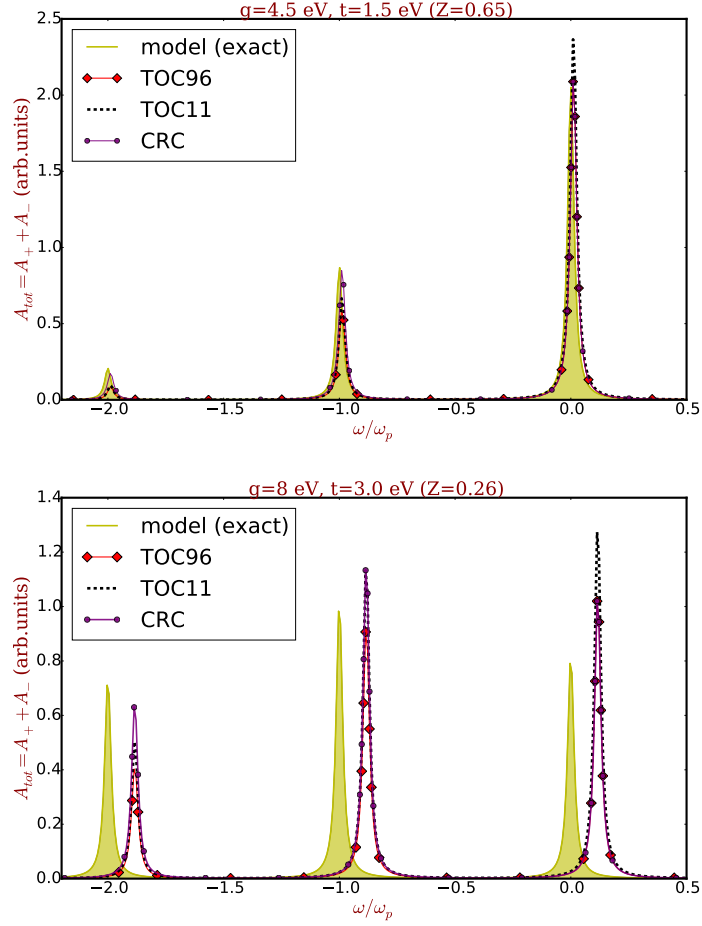
Figure 5.7: The total electron removal spectrum of the HPC-2. Upper panel: parameters are consistent with the sodium bottom valence state. Lower panel: relatively large coupling strength g = 8 eV and large bandwidth t = 3 eV instead of 1.5 eV, leading to Z = 0.26 . The yellow filled curve is the exact total spectra of the model that come from the sum of the bonding and anti-bonding spectral functions in Eq. 4.29. The red line with diamonds, black dashed and purple line with circles show the total electron removal spectra calculated using the TOC96, TOC11 and CRC, respectively. The Lorentzian broadening \eta = 0.1 eV has been used for all plots.
