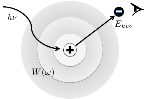
Figure 1.4: Schematic illustration of electron removal and the resulting reaction of the remaining electrons. The hole induced by the removal of one electron is dressed by the wave-like oscillation of all other electrons. This is a screening effect described by the dynamically screened Coulomb interaction W .
