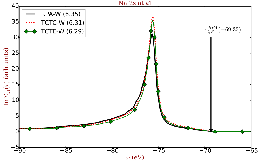
Figure 6.10: The imaginary part of the GW self-energy using the dynamically screened Coulomb interactions in the RPA (black curve) Eq. (C.20a), the TCTC dielectric function (red dashed curve) Eq. (C.20b), and the TCTE dielectric function (green curve with diamonds) Eq. (C.20c). All the plots have been aligned according to the quasi-particle energy calculated using the RPA W as indicated by the black arrow labeled “ \epsilon_{QP}^{RPA} ”, for good comparison. The real QP energies for the RPA, TCTC, and TCTE are -69.33 , -68.74 , and -69.82 eV, respectively. The numbers in the legend represent the distance between the QP peak and the peak in \text{Im}\Sigma for different approximations. The experimental distance between the QP and the first satellite of sodium 2s in Fig. 6.2 (i.e. from the experiment in Ref. [47]) is \approx 5.9 eV.
