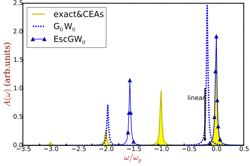
Figure 4.4: The electron removal spectral functions of the one-level hole-plasmon coupling Hamiltonian (HPC-1). The yellow filled curve is the exact spectral function of the model Hamiltonian in equation (4.12). The cumulant expansion approximation yields the exact spectral function of the HPC-1 as shown in equation (4.47). The blue dashed curve is the spectral function calculated from the one-shot GW ( G_0W_0 ) in equation (4.36). The blue solid line with up-triangles represents the spectral function calculated using the energy self-consistent GW in Eq. (4.42). The black arrow labeled “linear” represents the quasi-particle energy from the linearization approximation in Eq. (2.44). The exact quasi-particle energy has been shifted to zero. I have used the Lorentzian broadening \eta = 0.1 in all plots. The parameters are corresponding to bulk sodium bottom valence state.
