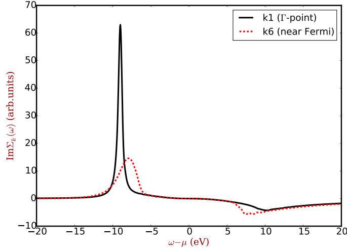
Figure 6.8: The imaginary part of the GW self-energy \text{Im}\Sigma at k_1 = [0, 0, 0] , i.e. \Gamma point (black curve) and at k_6 = [0.3125, 0, 0] , i.e. a state closer to the Fermi than \Gamma .
