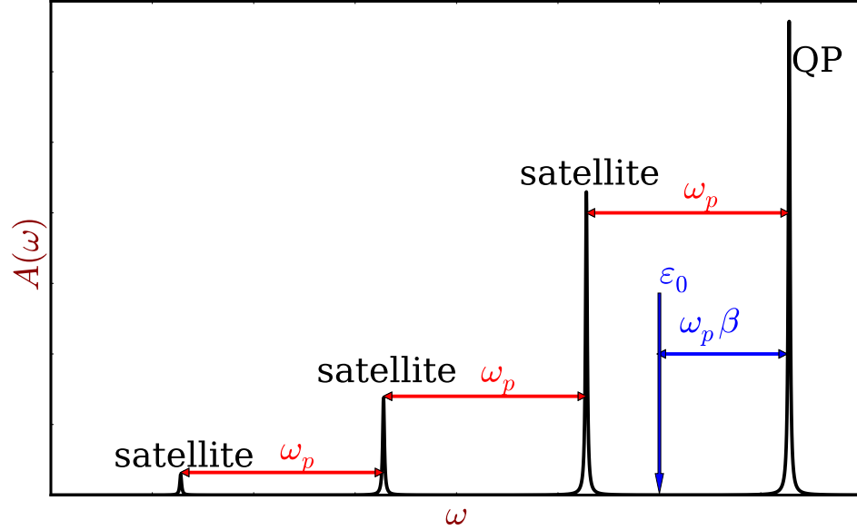
Figure 1.6: The spectral function Eq. (1.5) of the quasi-boson model Hamiltonian. The strong peak labeled QP represents the QP peak of energy \varepsilon_0 + \omega_p \beta and renormalized weight \mathbf{Z} = e^{-\beta} . All the other peaks are the plasmon satellites and the energy difference between peaks is the plasmon energy \omega_p . The blue arrow labeled \varepsilon_0 represents the position of the \delta -peak that we would obtain in the case of g_q = 0 , i.e. the non-interacting limit.
