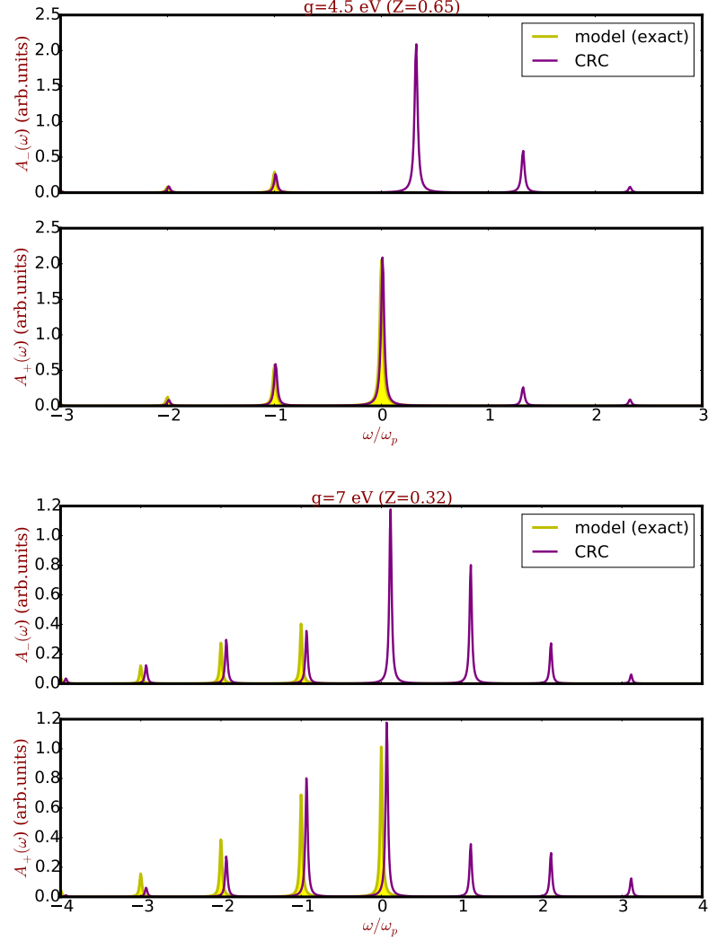
Figure 5.5: The spectral functions of the two-level hole-plasmon coupling Hamiltonian. All parameters are the same as in Fig. 5.3. Upper panel (two figures): the coupling g = 4.5 eV yielding Z = 0.65 . Lower panel (two figure): a stronger coupling g = 7 eV yielding Z = 0.32 . Yellow filled and purple curves are the exact and CRC spectral functions (Eq. (5.17)), respectively. The Lorentzian broadening \eta = 0.1 eV has been used for all plots.
