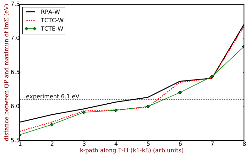
Figure 6.11: The distance between the QP and the peak in \text{Im}\Sigma for the sodium valence. The horizontal axis shows the k-points along the \Gamma -H path (see the sodium band structure in Fig. 2.1) in the first Brillouin zone. As in Fig. 6.10, the black solid curve, red dashed curve, and green line with diamonds are the results using the RPA, TCTC, and TCTE screenings, respectively. The black dashed horizontal curve represents the distance between the QP and first satellite in the experimental spectrum in Ref. [28].
