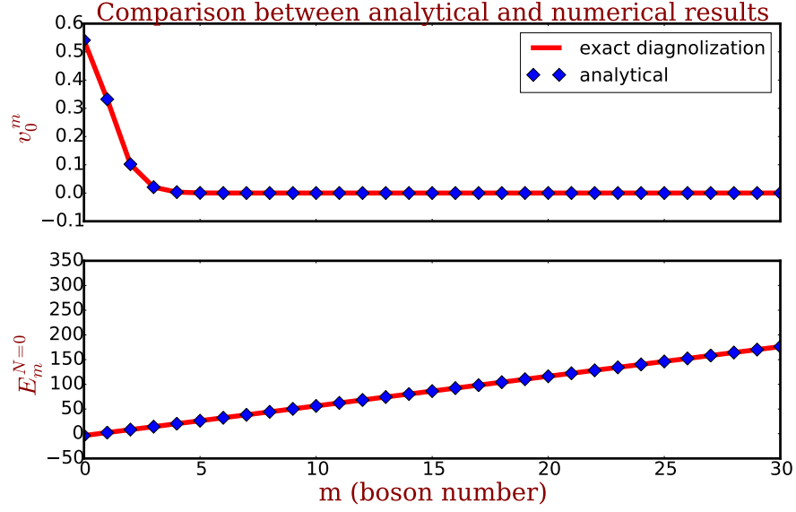
Figure 4.1: The upper and lower panels show the coefficients of the eigenfunctions and the eigenvalues of \hat{H}^{N=0} , respectively. Red curves are the dataset from the exact numerical diagonalization of \hat{H}^{N=0} whose matrix elements are shown in Eq. (4.10). Blue diamonds are our analytical results v_0^{\tilde{m}} (upper panel) in Eq. (4.9) (only these coefficients are used to calculate the Green's function in Eq. (4.11)) and E_m^{N=0} (lower panel) in Eq. (4.7), respectively. Note that in the plot I have replaced the symbol \tilde{m} by m , which is equivalent to the original equations.
