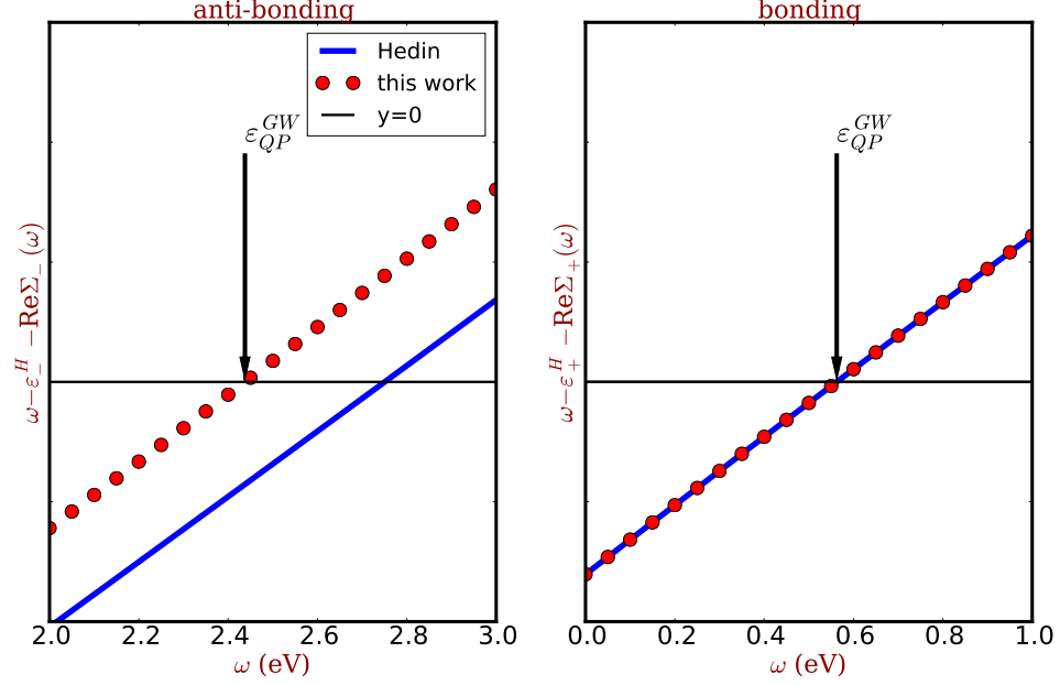
Figure 4.6: The quasi-particle energies calculated from different approximately energy self-consistent self-energies. The shifted real part of \Sigma_{\pm}^{Hedin} Eq. (4.59) and \Sigma_{\pm}^{EscGW_0} are shown as blue solid curve and red circles, respectively. Left panel is the anti-bonding results and right panel is the bonding orbital results. The black arrows labeled \varepsilon_{QP}^{GW} are the QP energies from the QP equation which are shown in Eq. (4.61). The parameters are chosen consistent with the bulk sodium bottom valence state, i.e. the same as in Fig. 4.3. Note that in Fig. 4.3, the horizontal axis has been defined as \omega/\omega_p and the bonding orbital QP energy has been shifted to zero. Here the horizontal axis is \omega and there is no shift on the QP energy.
