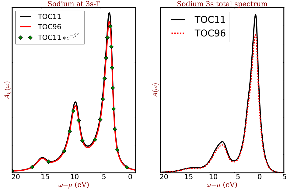
Figure 6.6: Intrinsic spectra of Na 3s. Left panel: k-resolved spectrum at the \Gamma point. Right panel: total k-summed spectrum. The black and red curves (red dashed in the right panel) are the spectra of the TOC11 and TOC96, respectively. The green diamonds in the left panel shows A^{C11}e^{-\beta >} that is supposed to be the same as A^{C96} from our derivation. Our cumulant code gives indeed what we have expected in sodium valence calculation. The plots in the right panel have Gaussian broadening of 0.3 eV because they are the k-summed total spectra.
