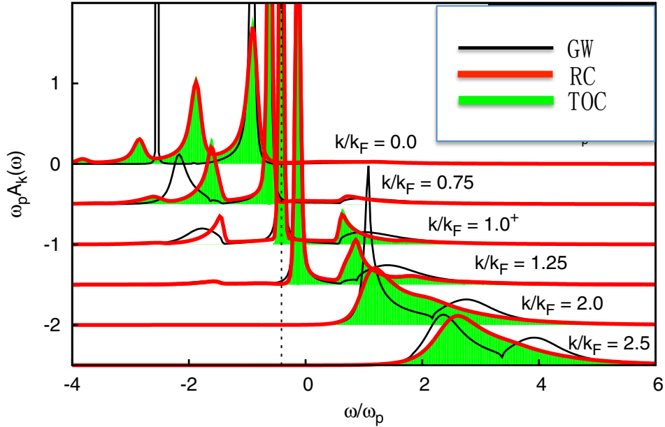
Figure 2.10: The comparison of the spectra calculated from the GWA ( G_0W_0 ), the time-ordered cumulant, and the retarded cumulant in the homogeneous electron gas at zero temperature for r_s = 4.0 (which corresponds to the sodium density) in units of the plasmon energy \omega/\omega_p . The figure is taken from Ref. [19]. The spectral functions A_k(\omega) for a range of states k are shown. The black curves are the GWA results, the thick red curves are the retarded cumulant results and the time-ordered cumulant (TOC) spectra are shown by the green filled curves. The dashed vertical line is set at the chemical potential \mu .
