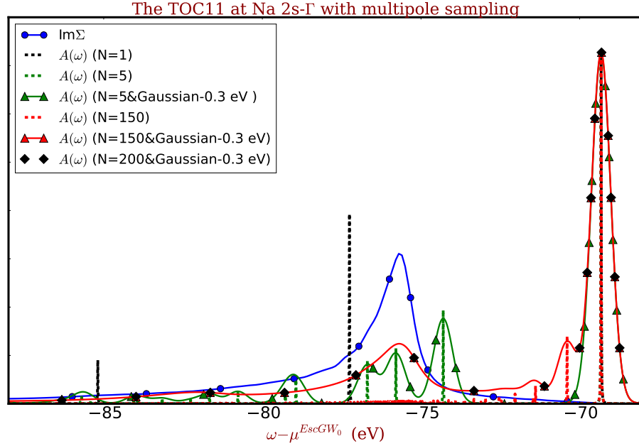
Figure 6.3: Cumulant intrinsic spectra of Na 2s \Gamma point with different number of poles in the sampling of \text{Im}\Sigma (only the lesser part is shown). The blue curve with circles is the imaginary part of the self-energy at \Gamma . The black, green and red dashed curves are the cumulant spectra calculated from 1, 5 and 150 poles of sampling, respectively. The green and red lines with up-triangles are the cumulant spectra with 5 and 150 poles sampling and a 0.3 eV Gaussian broadening. The black diamonds are the spectrum calculated using 200 poles which is on top of the spectrum using 150 poles. The zero of the energy axis is set to be the \text{EsGW}_0 Fermi energy.
