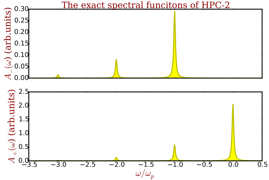
Figure 4.3: The exact spectral functions of the two-level hole-plasmon coupling Hamiltonian (HPC-2) . The parameters in Eq. (4.18) are chosen consistent with the bulk sodium bottom valence state, i.e. the plasmon energy \omega_p = 6.0 eV, \varepsilon_0 = \mathbf{t} = 1.5 eV yielding a 3 eV bandwidth, as well as the coupling constant g = 4.5 eV yielding the exact renormalization factor \mathbf{Z} = 0.65 . The upper and lower panels show the spectral function of the anti-bonding and bonding orbitals, respectively. The exact QP energy has been shifted to zero, i.e. E_0^- + \frac{g^2}{2\omega_p} = 0 . I have used \eta = 0.1 Lorentzian to broaden both spectral functions. Note the change of scale between the two plots.
