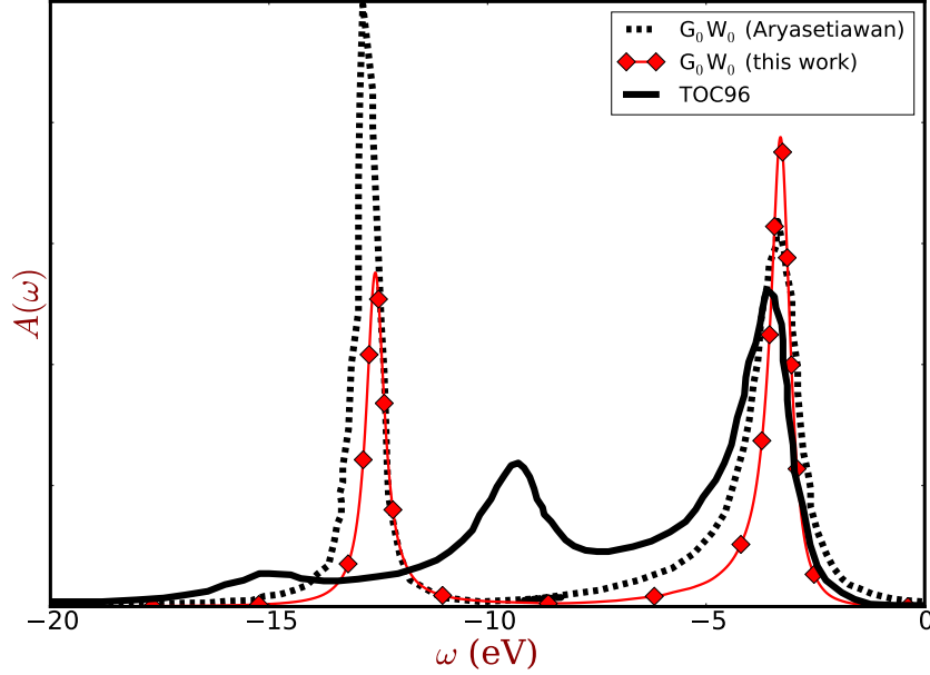
Figure 2.9: Intrinsic spectral function of the sodium valence 3s at the \Gamma point. Black curves are reproduced from Ref. [9]. Dashed and solid curves are G_0W_0 and cumulant spectral functions, respectively. The red curve with diamonds is the G_0W_0 spectral function from my calculation that was also shown in the lower panel of figure 2.7. To have a good comparison, I have shifted the my G_0W_0 spectrum by 0.1 eV such that the QP peak is centered at the same energy as the result of Aryasetiawan et al. [9].
