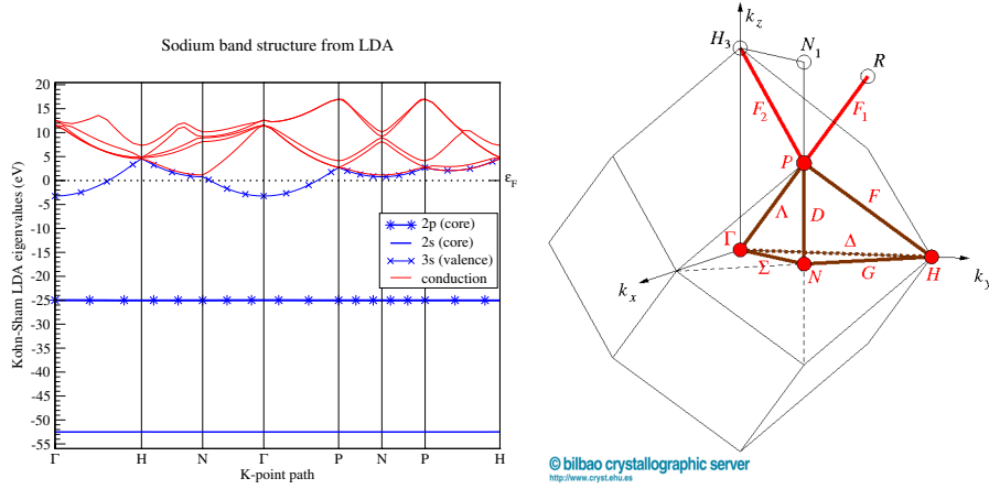
Figure 2.1: The band structure of bulk sodium calculated from KS-LDA using the ABINIT code is shown in the left panel. The right panel is the first Brillouin zone (BZ) of bulk sodium (which is body-centered cubic in real space) where all the high symmetry points are indicated. This figure of the Brillouin zone is taken from Refs. [50,51]. In the left panel, the chemical potential ( \varepsilon_F ) has been shifted to zero. The bands represented by the red curves are conduction bands. The two core bands contained in my calculation are shown in thick blue ( 2s ) and thick blue with stars ( 2p ), respectively. The valence band ( 3s ) is shown in thin blue curve with crosses.
