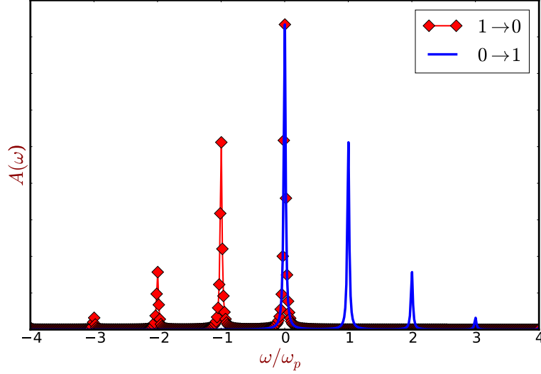
Figure 4.2: The spectral functions of the one-level hole-plasmon coupling Hamiltonian (HPC-1) in Eq. (4.2). The red line with diamonds and blue solid line are electron removal (PES) Eq. (4.12) and addition (IPES) Eq. (4.17b) spectra, respectively. I have put Lorentzian broadening \eta = 0.1 in both spectral functions. The quasi-particle energy has been shifted to zero, i.e. \varepsilon_{QP} = \varepsilon_0 - \frac{g^2}{\omega_p} = 0 .
