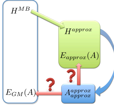
Figure 7.3: Schematic view of the relation between the total energy formulas and the Hamiltonians. The exact total energy formula of the exact many-body Hamiltonian is proven to be the Galitskii-Migdal formula. However, the Galitskii-Migdal formula requires the exact Green's function to reproduce the exact total energy. It is impossible to calculate the exact Green's function of a many-body system. Instead some approximate Hamiltonians ( H^{approx} ) are introduced (e.g. the hole-plasmon coupling Hamiltonian) which allow us to have the exact Green's functions (of the corresponding approximate Hamiltonians). Consequently, the exact total energy formula of the approximate Hamiltonian H^{approx} may not be the Galitskii-Migdal formula any more, as indicated on the right side. We might have to derive a new total energy formula E_{approx}[A] (i.e. a functional of the spectral function hence the Green's function) corresponding to the approximate Hamiltonian such that the exact spectral function of H^{approx} yields its exact total energy using E_{approx}[A] . Since the GW approximation and the cumulant expansion approximation can be considered as some good approximate solution to the approximate hole-plasmon coupling Hamiltonian, the question becomes “ which formula should we use when we have the spectral functions of the GWA or the CEA? ” The direct answer to this question will not be provided in the present thesis, but I will show some studies that reflect the importance of this issue in the following total energy calculations.
