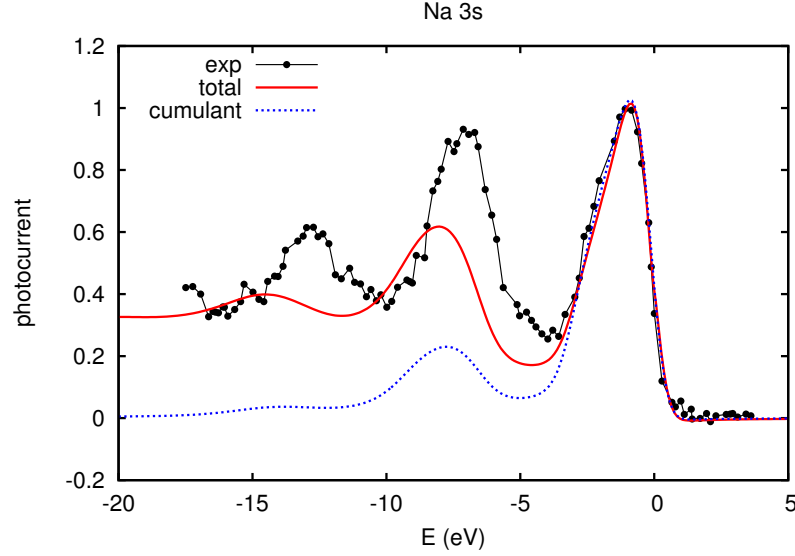
Figure 6.5: Comparison of the experimental photoemission spectrum to the spectrum calculated using the TOC11 + extrinsic + interference approach: valence band. Red solid is total calculation, including a secondary electron background, black with circles is experiment [28], and blue dashed is the intrinsic TOC11 spectral function. The spectra are angle-integrated. Original experimental data were in arbitrary units: here we have normalized them to the main-peak intensities. All the calculated spectra have been Gaussian broadened with 0.3 eV and the QP peak is shifted to the experimental value, otherwise the GWA 3s level is too deep by about 0.5 eV.
