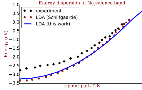
Figure 2.2: Dispersion of the sodium valence band along \Gamma -N k-point path. The black diamonds are experimental data reproduced from Ref. [49]. The red circles are the LDA result reproduced from the same article. The blue solid curve is the result from my own calculation.
