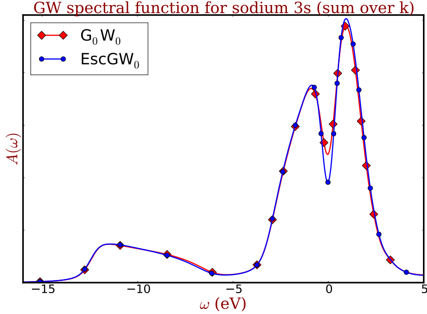
Figure 2.7: Intrinsic spectral function of the sodium 3s band where the spectral function of each k-point in the BZ has been summed. Red curve with diamonds are G_0W_0 results, blue curve with circles are \text{EscGW}_0 results. The zero of the energy axis is set to be the \text{EscGW}_0 Fermi energy. A Gaussian broadening of 0.3 eV has been used when plotting these two spectral functions.
