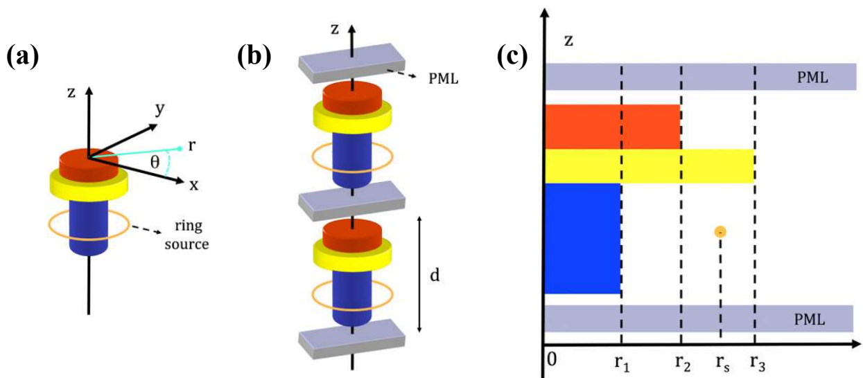
Figure B.2: (a) Example of a rotationally invariant nanostructure with the presence of a ring source. (b) The aperiodic nanostructure is periodized with period d along the symmetry axis. The cells are separated by either a PML or, in our calculations, by complex coordinate transforms. (c) In the radial direction, the structure is divided in slabs for which the optical properties are invariant along the radial direction. Figure has been extracted from Ref. [140].
