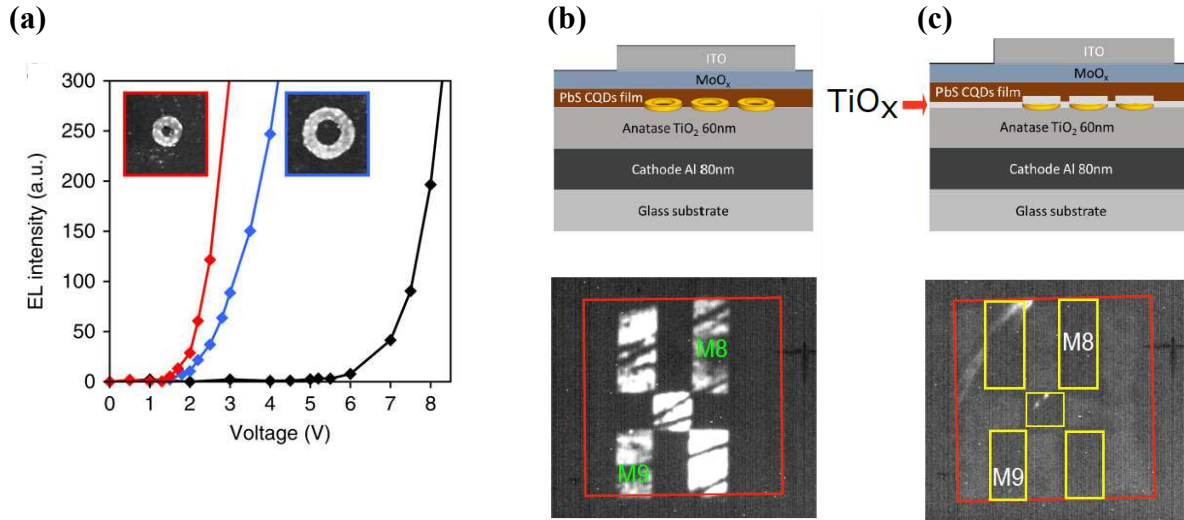
Figure 6.3: (a) The EL intensity in arbitrary units is given as a function of the applied voltage for different devices. From left to right: “small” rings, “large rings”, and no gold nanoantennas. The “small” and “large” rings have been visualized in the graph. The turn-on voltage goes down from 6 V to 1.3 V when gold nanorings are introduced. (b,c) A schematic view of experiments without (b) and with (c) a 5-nm-thick \text{TiO}_x spacer between the PbS cQDs and the nanorings are presented in the upper parts of Fig. 6.3(b) and Fig. 6.3(c). Below the electroluminescence signals are shown. The applied voltage was (b) 5 V and (c) 10.5 V. The yellow rectangles indicate the regions in which gold nanorings are present. In (c), no electroluminescence is observed from these regions. The differences between the patches and the symbols M8 and M9 are irrelevant for this thesis. Courtesy of Quynh Le-Van.
