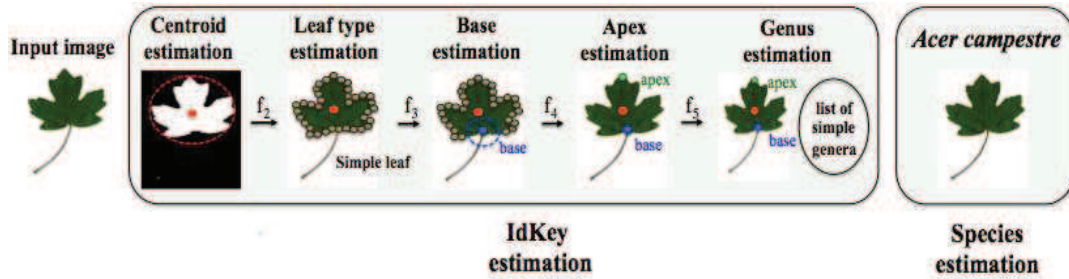
Figure 3.6: Botanical idKeys estimation for species identification.
