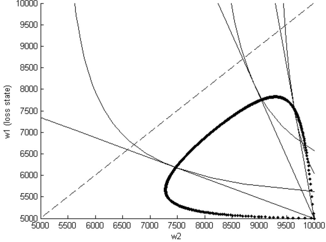
Figure 3.5: w = 10000, L = 5000, u(x) = \frac{x^{-3}}{3}, r = 0.05, \lambda = 0.3, q = 0.5
