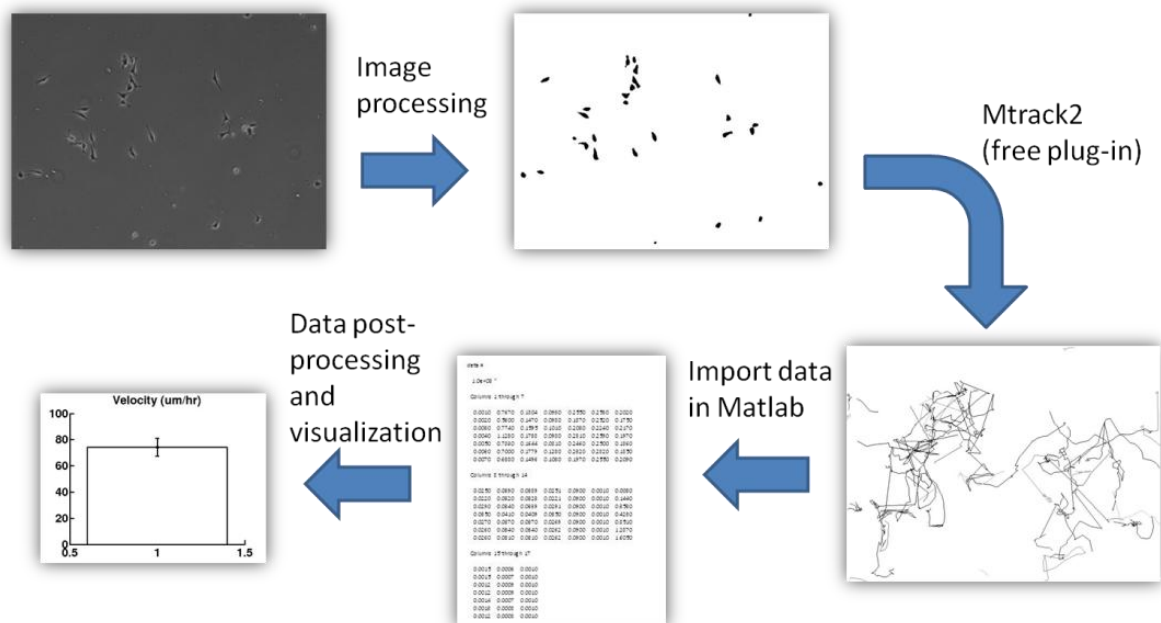
FIGURE 4.17: Key algorithm steps to track cells automatically.
