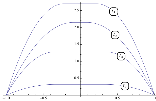
FIGURE 2.2 – L_i , i = 1, 2, 3, 4 are the graph of w for (m, A) = (0.5, 0.5), (2, 2), (3, 0.5), (4, 2) respectively.
