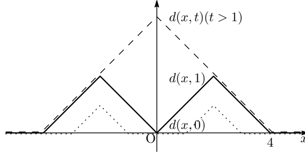
FIGURE 1.1 – The graph of d .
