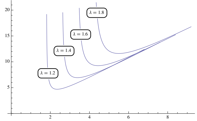
FIGURE 2.6 – \Pi(\lambda, \lambda_1^*) for \lambda = 1.2, 1.4, 1.6, 1.8
