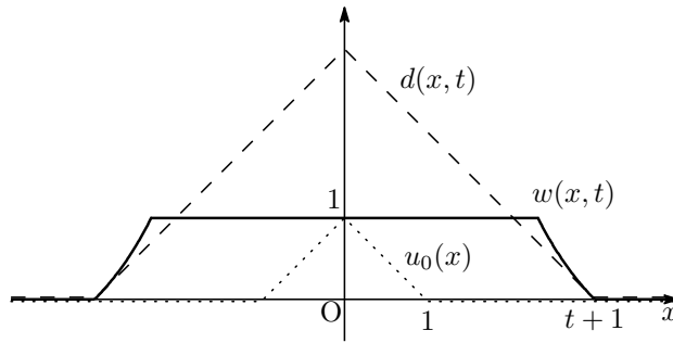
FIGURE 1.2 – The graph of w when t \geq \log 2 .
