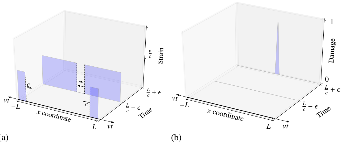
Figure 4.2 – Strain (a) and damage (b) before and after the wave crossing at t = \frac{L}{c} in the dynamic gradient damage model with \widehat{\eta} = 0.01
