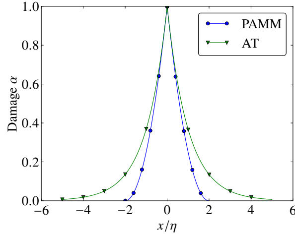
Figure 2.2 – Optimal damage profiles for the (PAMM) and (AT) damage constitutive models
