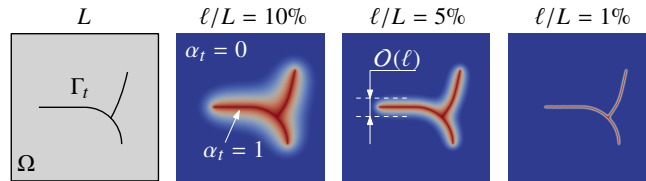
Figure 1.8 – Approximation of the discrete crack \Gamma_t by a continuous field \alpha_t parametrized by \ell
