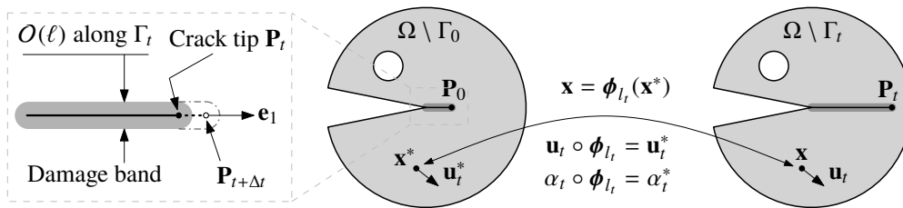
Figure 2.11 – Propagation of an existing damage band via the diffeomorphism \phi
