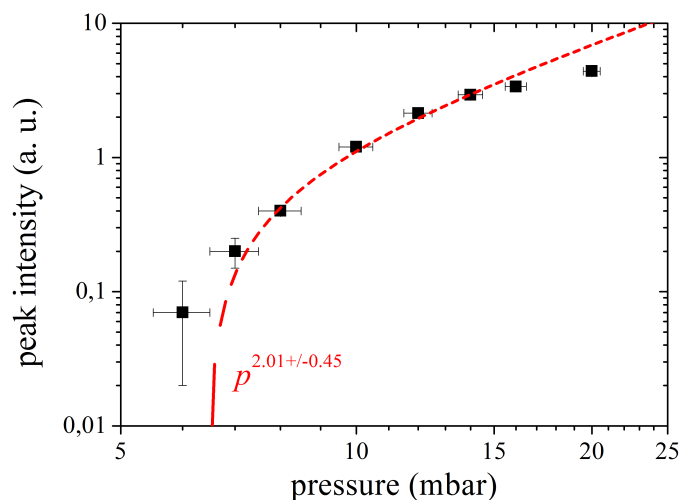
Figure 6.9: The extracted peak intensity from the temporal profiles of 391 nm lasing pulses as a function of nitrogen pressure. The dashed line presents the fitting by expression form ap^b + c , where p denotes the pressure.
