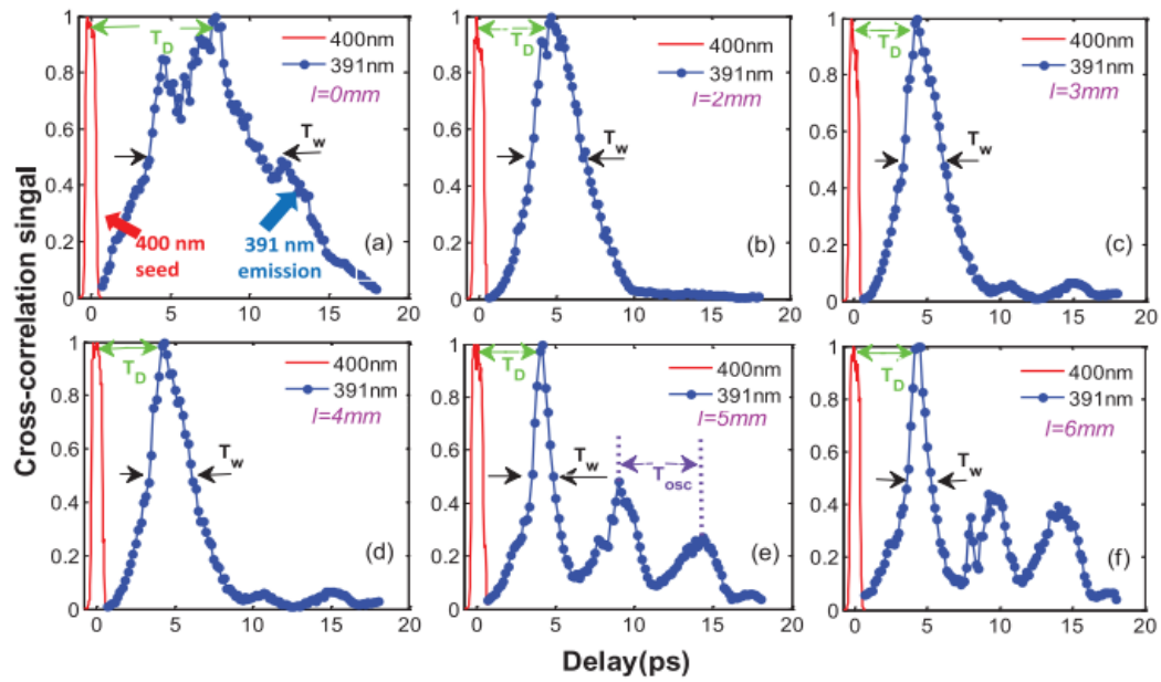
Figure 6.12: Measured temporal waveforms of 391 nm lasing pulses for the plasma channel lengths of (a) 0 mm, (b) 2 mm, (c) 3 mm, (d) 4 mm, (e) 5 mm, (f) 6 mm, respectively. The red solid line represents the cross-correlation signal between the 800 nm and 400 nm seed pulses, pointing the time of the pump pulse. Courtesy to Ref [68].
