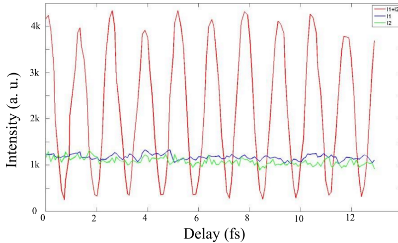
Figure 6.13: Coherent control of the 391 nm lasing emission in double (red line) and single (violet and green lines) seeding scheme. The oscillation period in this figure is about 1.3 fs, the period of 391 nm emission. The nitrogen pressure was 4 mbar.
