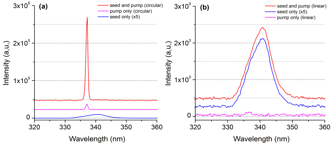
Figure 3.14: Spectra of the backward emission with circularly (a) and linearly (b) polarized pump pulsed at 800 nm. The spectra of the seed pulses and those of the backward emission from the pump pulses are also presented for comparison. The spectrum of the seed pulse is magnified by a factor of 5 for better comparison.
