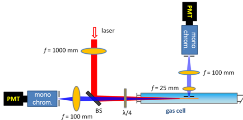
Figure 2.4: Schematic illustration of the experimental setup. Here, the signal of interest is measured by a monochromator combined with a photomultiplier tube.
