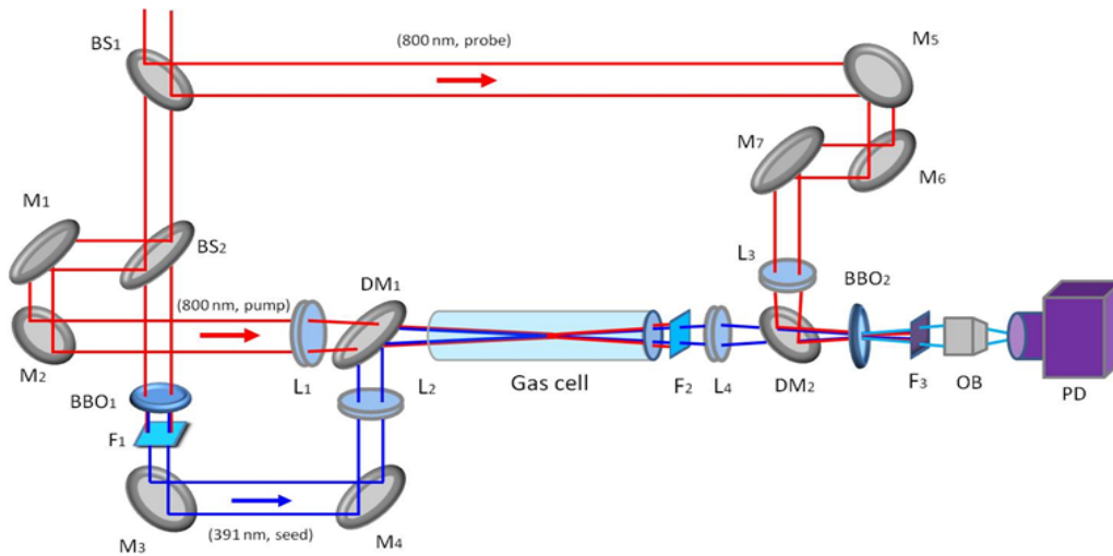
Figure 5.3: Schematic illustration of experimental setup for measuring 391 nm and 428 nm lasing emissions. BS denotes beamsplitter, M the high reflective mirror, L the focusing lens, DM the dichromatic mirror, F the interference filter, OB the collecting lens and PD the photodiode detector.
