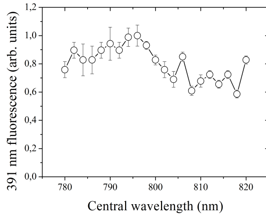
Figure 6.6: The side fluorescence signal at 391 nm as a function of pump laser wavelength. This experiment was performed in gas jet in order to collect the side fluorescence by using a fiber pointer. The pulse duration of pump laser is 35 fs.
