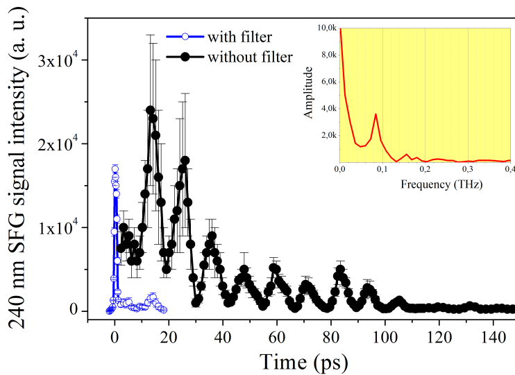
Figure 3.19: The measured results of the temporal profile of backward seeded 337 nm lasing pulse for two cases, with and without 240 nm bandwidth ( \sim 10 nm) filter. The inset is the FFT result of the black curve obtained without filter.
