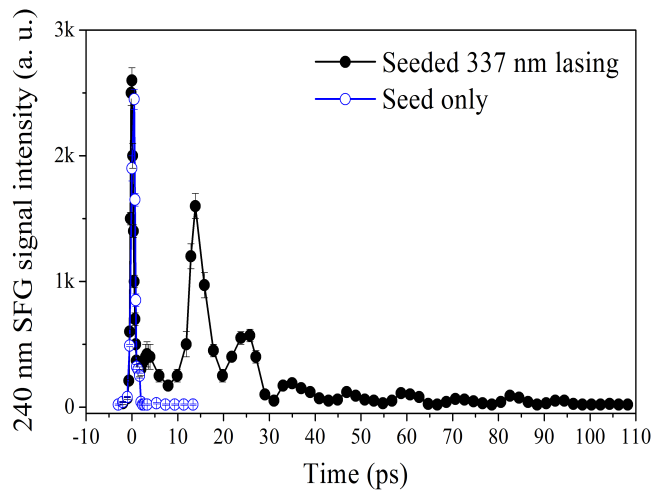
Figure 3.18: The measured results of the temporal profile of backward 337 nm signal in the cases of with circular pump (e.g., seeded 337 nm lasing) and without pump (e.g., only seed pulse). The 240 nm SFG signal is measured by a spectrometer.
