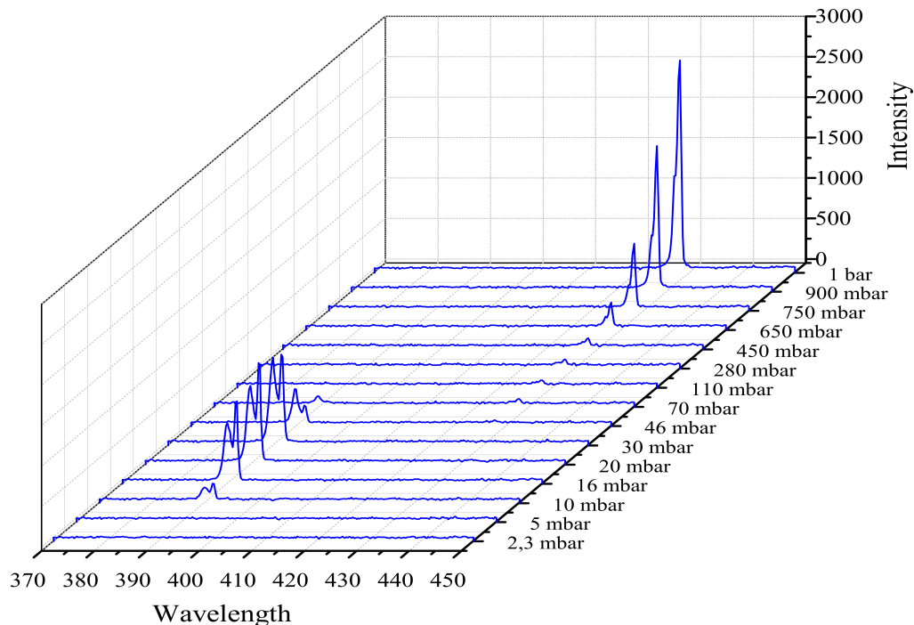
Figure 5.5: Spectrum of the forward lasing emission in nitrogen at different gas pressures. The incident pump pulse energy is 1.8 mJ.
