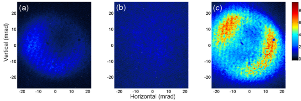
Figure 3.3: Measured spatial profiles of forward 337 nm ASE (a), seed pulse (b) and externally-seeded 337 nm lasing pulse (c) in pure nitrogen gas with pump pulse energy of \sim 9.0 mJ.
