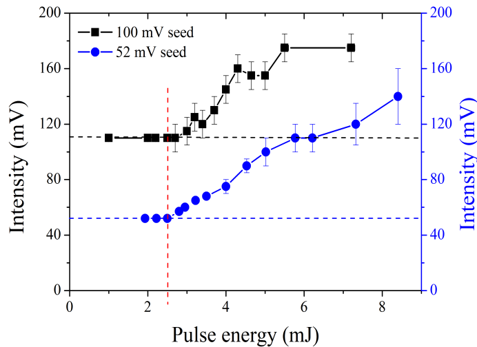
Figure 5.15: The externally-seeded 391 nm lasing intensity in backward direction as a function of pump pulse energy, for two seed intensities. The pump laser pulses were focused by a 40 cm convex lens into gas chamber filled with 30 mbar nitrogen, and the lasing emission was detected by a photodiode.
