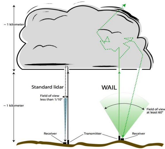
Figure 2.2: Lidar observations of a dense cloud. Left: standard (single-scattering/on-beam) lidar. Right: multiple-scattering/off-beam lidar. Courtesy to the research on website: http://asr.science.energy.gov/science/research-highlights/RMTQw/view .
