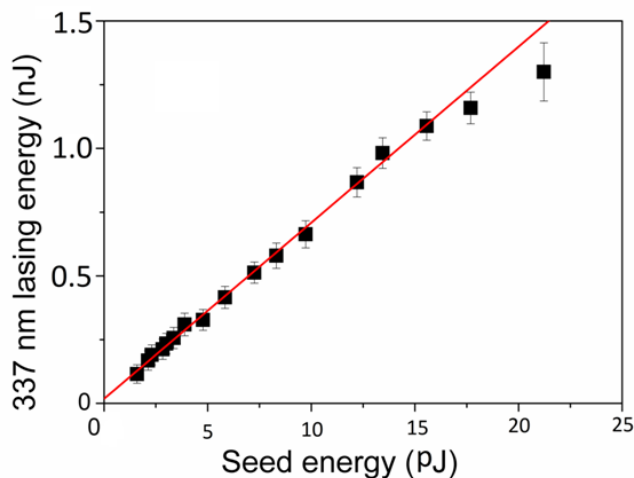
Figure 3.17: The calibrated seeded 337 nm lasing pulse energy in the backward direction as a function of the seed pulse energy. The red line curve denotes linear fit.
