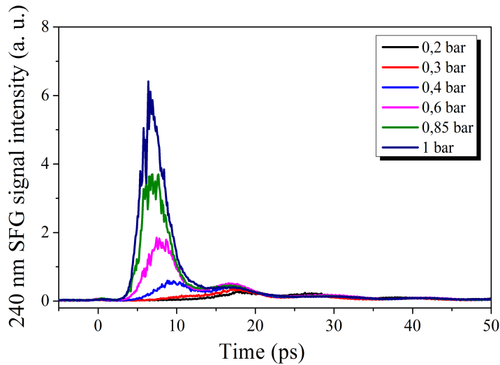
Figure 3.7: Temporal profiles of forward externally-seeded 337 nm lasing pulse for different nitrogen pressures.
