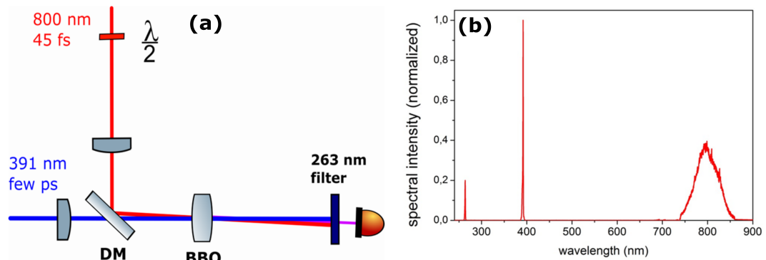
Figure 5.4: (a) Schematic illustration of the cross-correlation method. \lambda/2 denotes half wave plate, used to change the polarization of 800 nm probe pulse. (b) Spectra of the fundamental 800 nm pump laser, the 391 nm lasing emission and their sum-frequency signal at 263 nm wavelength.
