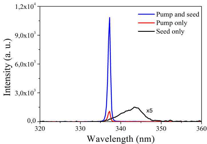
Figure 3.2: Spectra of forward externally-seeded 337 nm lasing emission, the forward 337 nm ASE and the seed pulse. The pump pulse energy is about 7.2 mJ. The intensity of seed pulse is magnified by 5 times for better vision.
