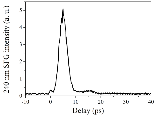
Figure 3.10: The temporal profile of forward seeded 337 nm lasing pulse in ambient air measured through cross-correlation method.
