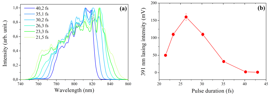
Figure 6.7: (a) The spectra of pump laser pulses with same central wavelength of 800 nm but different durations (or bandwidths) ranging from 21.5 fs to 40.2 fs. The laser intensity in filament for each pulse was kept almost as 8 \times 10^{13} \text{ W/cm}^2 by assuming the diameter of filament inside gas chamber as 100 \mu\text{m} . (b) The measured 391 nm lasing energy as a function of pulse duration of pump laser. The nitrogen gas pressure is at 5.5 mbar.
