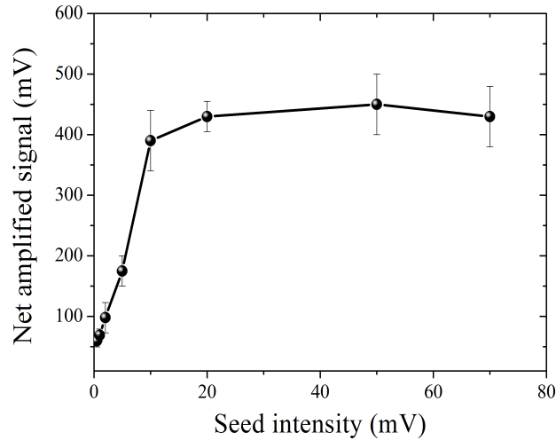
Figure 5.16: The seed intensity dependence of externally-seeded 391 nm lasing emission in forward direction. The net amplified signal is the result by subtracting the seed signal from the detected total 391 nm emission signal.
