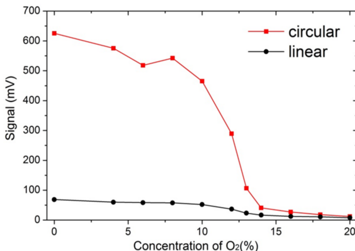
Figure 2.16: Measured backward 337 nm lasing signal from filament plasma in a mixture of nitrogen and oxygen as a function of oxygen gas concentration, for both circular and linear polarized laser pulses. The incident pulse energy is 9.3 mJ.
