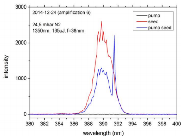
Figure 6.18: Measured spectrum of the seed pulse, spectrum with only 1.35 \mu\text{m} mid-IR pump laser, and that with both the seed and pump pulses. The experimental parameters has been denoted in the figure.
