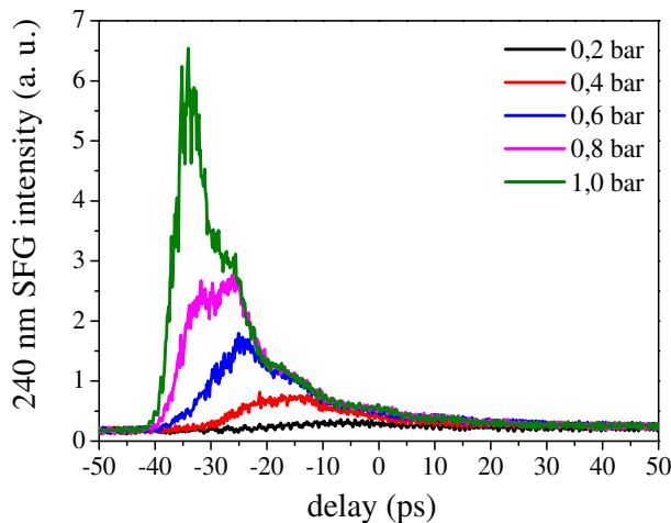
Figure 2.18: Measured temporal profiles of forward 337 nm ASE at nitrogen pressures ranging from 0.2 bar to 1.0 bar.
