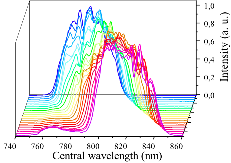
Figure 6.4: Tunability of the central wavelength of the 1 kHz infrared laser source with keeping a bandwidth of about 50 nm and pulse duration of 40 fs. The various colors represent different settings in the laser system.
