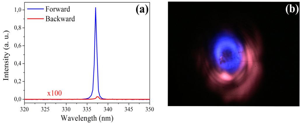
Figure 2.11: (a) Spectra of 337 nm laser in the forward (blue) and backward (red) direction, where the latter is enlarged by 100 times as denoted in the figure. (b) Photo of the forward 337 nm lasing emission beam after UG11 filter taken by mobile phone.
