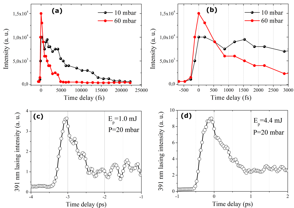
Figure 5.20: (a) Measured gain dynamics of 391 nm lasing emission at 10 mbar and 60 mbar nitrogen gas, respectively. The pump pulse energy was 1.8 mJ. The signal was detected by spectrometer. (b) The details of gain dynamics in the delay range from -500 fs to 3000 fs. (c)-(d) Measured gain dynamics of 391 nm lasing emission with pump pulse energies of 1.0 mJ and 4.4 mJ, respectively. The nitrogen pressure was fixed at 20 mbar.
