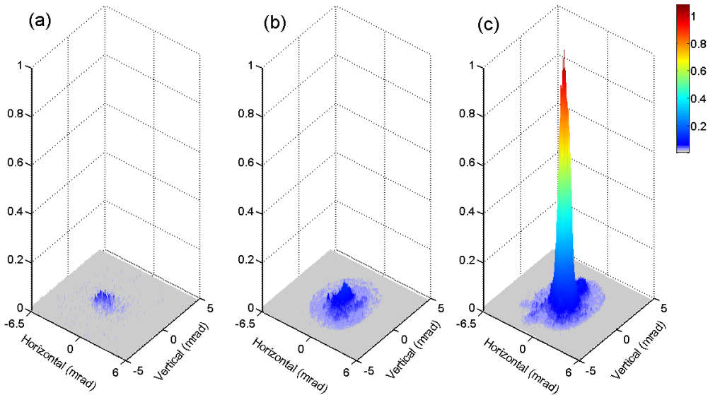
Figure 3.15: Spatial profile of the backward ASE (a), the seed pulse (b), and the externally-seeded 337 nm emission (c). The opening angle of each panel is 12.5 \text{ mrad} \times 10.0 \text{ mrad} . The color bar indicates the normalized emission intensity.
