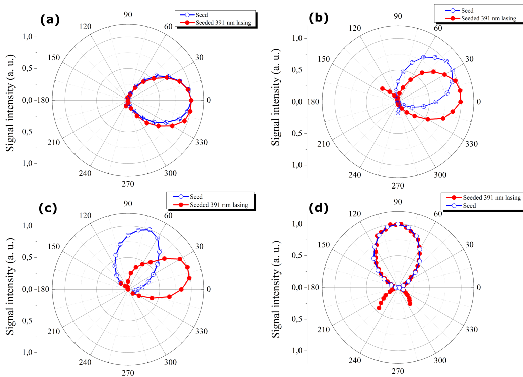
Figure 5.17: Measured intensities of forward seeded 391 nm lasing emission and the seed pulse as a function of the rotation angle of Glan-Taylor prism, for four polarizations of the seed pulse: 0° (horizontal polarization, parallel to the polarization direction of the pump pulse) (a), 35°, 70° and 90° (vertical polarization).
