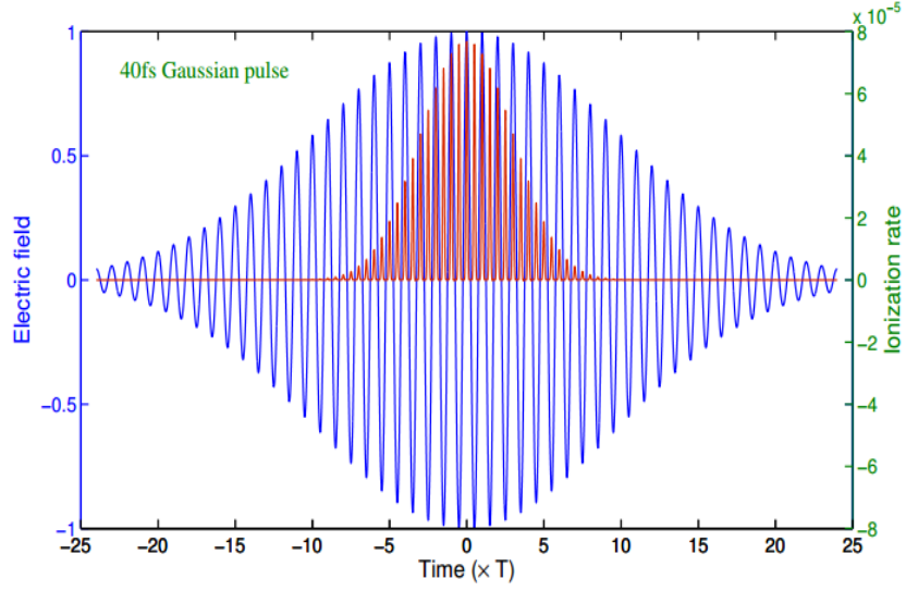
Figure 6.1: Calculated laser electric field and ionization rate of N_2 molecule from Eq. (6.1) for unchirped Gaussian laser field.
