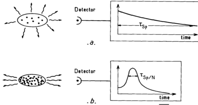
Figure 6.8: Comparison between the general characteristics of spontaneous emission and superradiance. (a) Ordinary spontaneous emission is essentially isotropic with an exponentially decaying intensity (time constant \tau_{sp} ). (b) Superradiance is anisotropic with an emission occurring in a short burst of duration \sim \tau_{sp}/N where N is the atom number. Courtesy to the literature [51].
