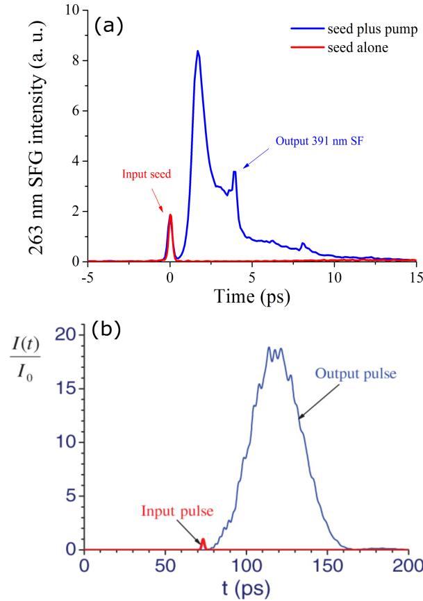
Figure 6.17: (a) Temporal profile of the seeded 391 nm lasing emission after it passes through 3-cm-long filament plasma in 20 mbar nitrogen gas. The red solid line denotes the seed pulse. (b) Simulated temporal profiles of the input and output UV laser pulse after it propagates through 1 cm of He gas driven by an IR coherent field. Courtesy to the Ref. [84].
