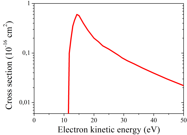
Figure 4.1: Cross-section of the electron-molecule inelastic collision excitation N_2(X^1\Sigma_g^+) + e = N_2(C^3\Pi_u^+) + e . Courtesy to the reference [40].
