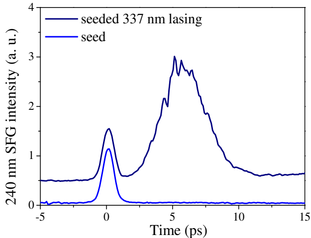
Figure 3.5: Temporal profiles of seed pulse and externally-seeded 337 nm lasing pulse measured with cross-correlation method. Before detector, we used BG40 and UG11 filters to block the IR pump light, and 240 nm bandwidth filter to select the sum-frequency signal.
