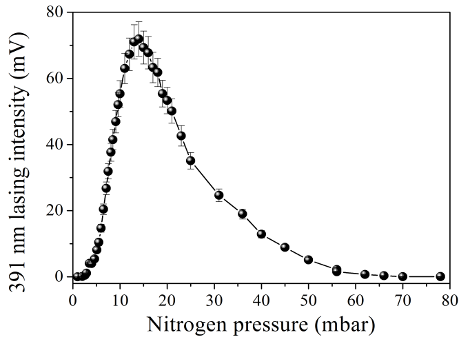
Figure 5.10: Intensity of 391 nm lasing emission as a function of nitrogen pressure, measured by a photodiode. In the measurement, the focal length was 50 cm, and the pump pulse energy was about 1.7 mJ after the dichromatic mirror.
