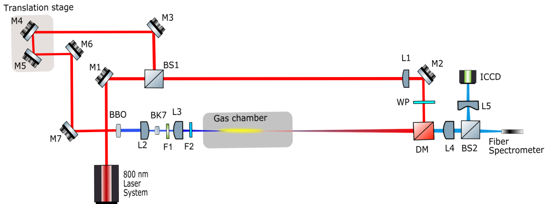
Figure 3.13: The schematic illustration of experimental setup for backward seeded 337 nm lasing emission.
