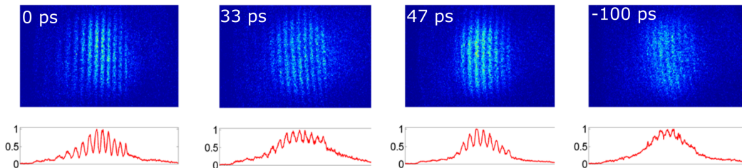
Figure 2.20: Interference pattern of backward 337 nm ASE lasing pulse for time delay of 0 ps, 33 ps, 47 ps and -100 ps. Vertical fringes were observed because we elaborately set a small angle between two identical arms of incident 337 nm ASE. The red curve shows normalized integrated intensity along vertical direction.
