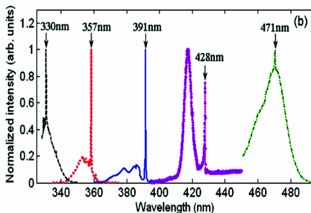
Figure 5.2: Measured lasing peaks at 330, 357, 391, 428 and 471 nm achieved with different pump wavelengths of 1682, 1760, 1920, 2050 and 1415 nm respectively. Taken from the ref. [20].
