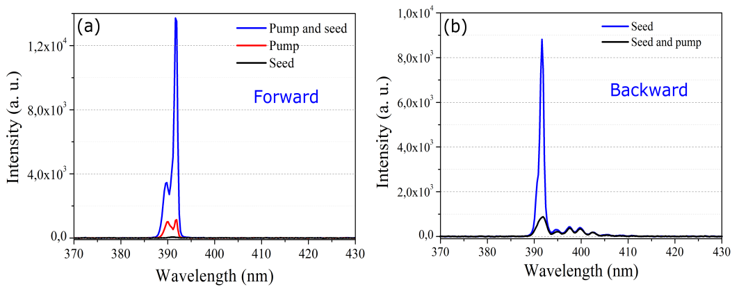
Figure 5.13: (a) The spectra of externally-seeded 391 nm lasing emission in forward direction. In the experiment, the pump pulses with energy of 1.8 mJ was focused by a 40 cm convex lens into 30 mbar nitrogen gas. The black line represents the seed signal, and the red line represents the lasing signal generated by only pump pulses and the blue the lasing signal represents the seeded lasing signal when the pump and seed pulses spatiotemporally overlapped. (b) The spectrum of seeded 391 nm lasing emission in backward direction. The used pump pulse energy was 7.5 mJ. No backward self-seeded 391 nm lasing signal was detected.
