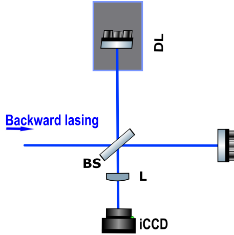
Figure 2.19: Schematic illustration of Michelson interferometer for measuring the interference pattern of backward 337 nm lasing emission. BS denotes a beamsplitter with a thickness of 500\mu\text{m} . DL is a time delay line controlled by a motorized stage. L is a 10 cm fused silica lens for collecting the light to iCCD camera.
