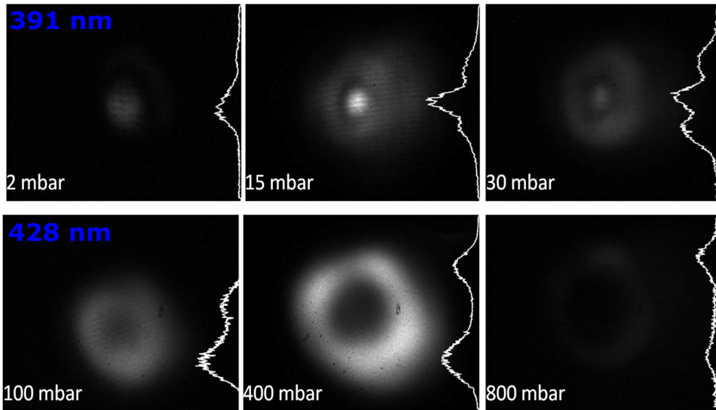
Figure 5.7: Spatial profiles of the 391 nm (upper panel) and 428 nm (lower panel) lasing beams at different nitrogen pressures. In each panel, the pressure is denoted. The angle of view of each panel is 60 \times 40 mrad. The white lines on the right of each panel present the vertical line-cut of each intensity distribution on the center.
