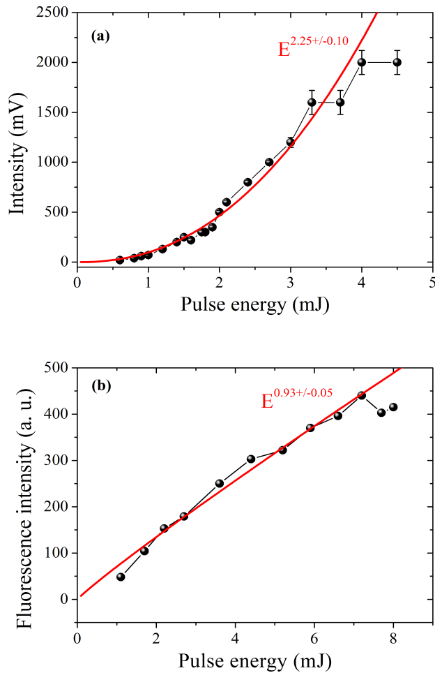
Figure 5.9: (a) The incident pump pulse energy dependence of 391 nm lasing emission of N_2^+ molecules, under experiment conditions: 30 mbar pure nitrogen, the focal length of f = 40 cm and a photodiode as detector. (b) The incident pump pulse energy dependence of transverse 391 nm fluorescence intensity. The red curves represent fit with the form I = aE^b with the coefficients denoted beside.
