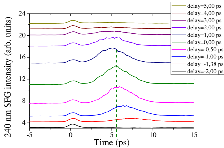
Figure 3.6: Temporal profiles of forward externally-seeded 337 nm lasing pulse for different delays between the IR pump and the seed pulse. The green dashed line denotes the peak position of the wake pulse in the case of zero delay.
