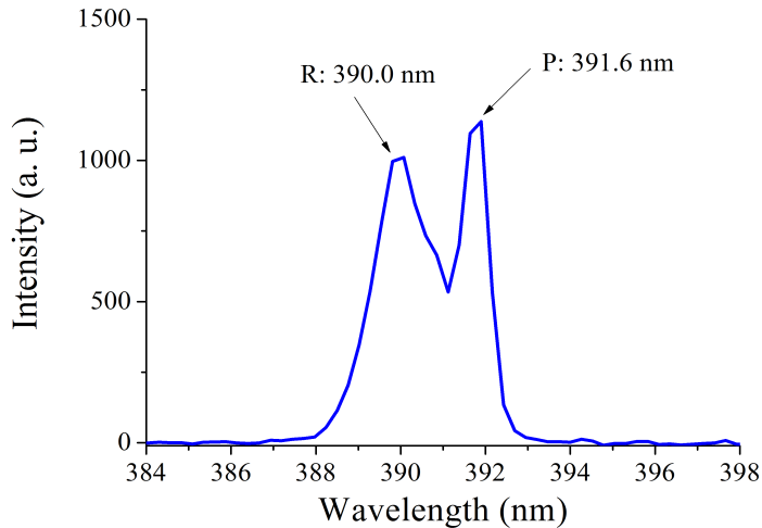
Figure 5.6: Typical spectrum of the 391 nm lasing emission of N_2^+ molecules.
