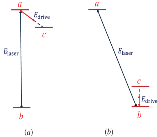
Figure 6.16: Energy level diagram in \Lambda - and V -schemes. Courtesy to the Ref. [84].
