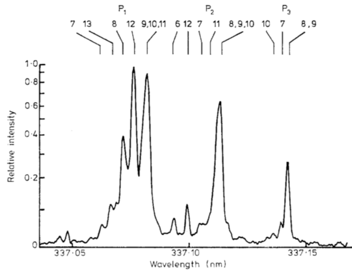
Figure 3.9: Fine spectrum of 337 nm C^3\Pi_u^+(v' = 0) \rightarrow B^3\Pi_g^+(v = 0) transition consisting of P_1 , P_2 and P_3 branches. Courtesy to the reference [34].
