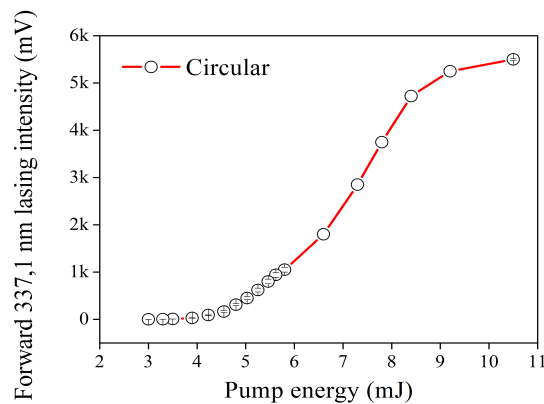
Figure 2.12: Pump energy dependence of 337 nm lasing emission in forward directions. The signal was detected by a calibrated photodiode.
