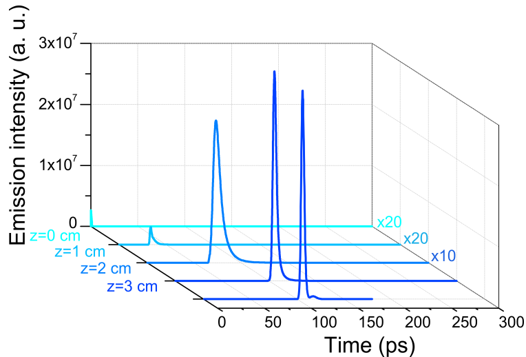
Figure 4.8: Simulation result of temporal profiles of forward seeded 337 nm lasing pulse at different positions ( z ) of the filament plasma amplifier with n_e = 1.2 \times 10^{16} \text{ cm}^{-3} and T_e = 16 \text{ eV} . Note that the intensity is magnified by factors denoted on the right for the sake of visualization.
