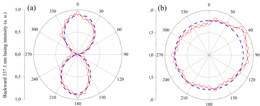
Figure 3.16: Polarization of the seeded backward stimulated emission with linearly (a) and circularly (b) polarized seed pulses at 337 nm. The dots present the experimental results and the dashed lines denote the theoretical fitting with Malus' law.
