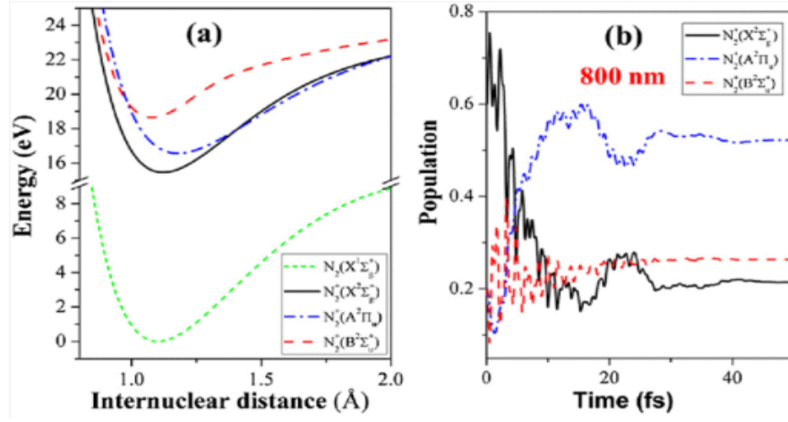
Figure 6.14: (a) Potential energy curves of the electronic states of N_2 and N_2^+ molecules. (b) The temporal evolution of the population distributions in the electronic states of N_2^+ in the 800 nm laser field with an intensity of 2.2 \times 10^{14} \text{ W/cm}^2 . Courtesy to the Ref. [63].
