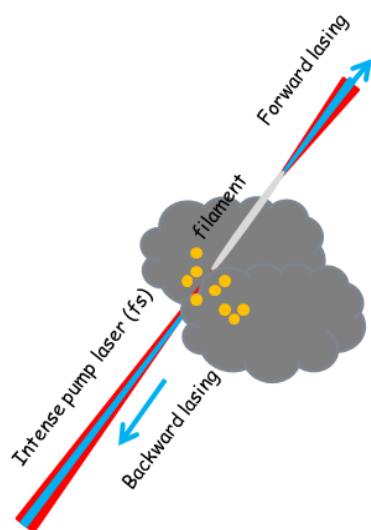
Figure 2.3: The schematic illustration of the concept of backward lasing-based remote sensing. The yellow dots denotes molecules of interest.
