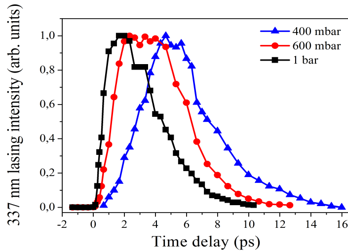
Figure 3.12: Measured forward amplified 337 nm lasing signal as a function of the relative time delay between the pump and seeding pulse. The focal length is 50 cm.
