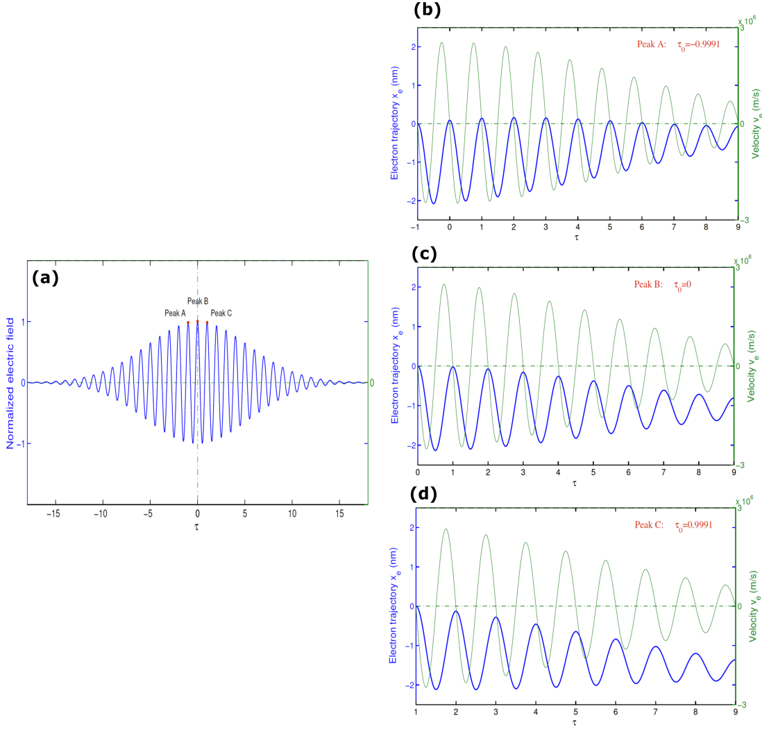
Figure 6.2: Calculated electron trajectory and velocity in laser field for electrons born at three different positions, peak A ( \tau_0 = -0.9991 ), peak B ( \tau_0 = 0 ) and peak C ( \tau_0 = 0.9991 ) respectively.
