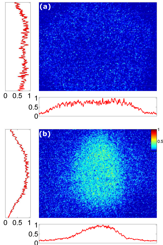
Figure 2.7: The spatial profiles of 337 nm emissions measured by iCCD camera in backward direction for linearly (a) and circularly polarized (b) 800 nm pump laser pulses in 1 bar nitrogen gas. The red curve represents the normalized space-integrated intensity along the corresponding axis.
