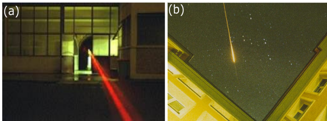
Figure 1.1: (a) Propagation of an 800 nm laser beam in atmosphere in the Laboratoire d'Optique Appliquée (École Polytechnique, Palaiseau). (b) Self-guided propagation the Teramobile laser beam in the sky. Courtesy to the Teramobile project ( see the official website of Teramobile project ).
