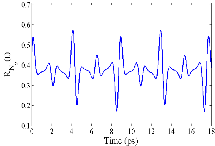
Figure 1.5: Calculated Raman response function of N_2 molecule as a function of time.
