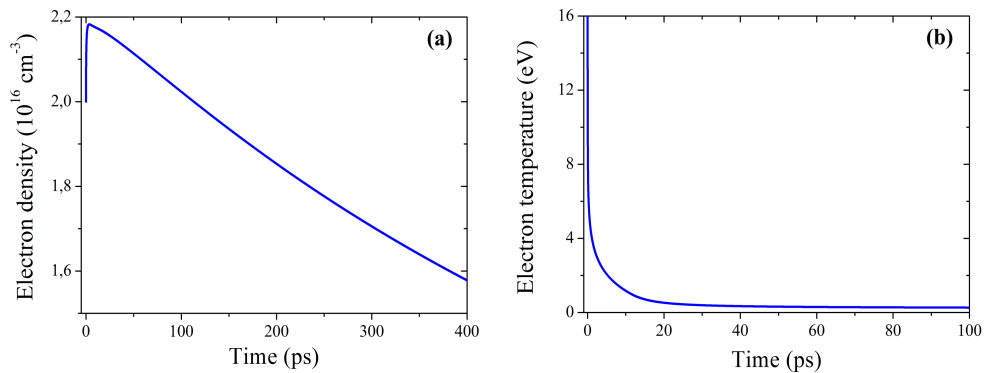
Figure 4.4: (a) Temporal evolution of the electron density along 400 ps. (b) Temporal evolution of the electron temperature along 100 ps.
