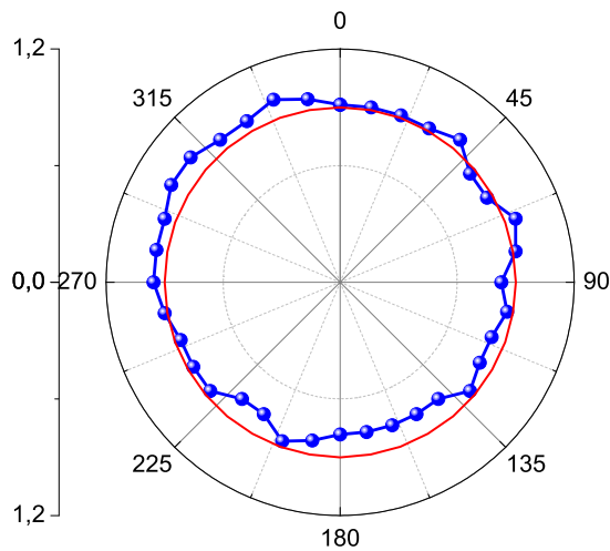
Figure 2.8: Polarization of the backward 337 nm ASE with circularly polarized pump laser. The solid-red line denotes the theoretical fit of Malus' law .
