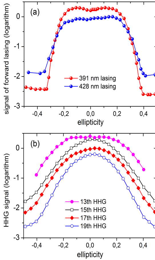
Figure 5.12: (a) 391 and 428 nm lasing emission as a function of the ellipticity of the pump pulses at 800 nm. The gas pressures were 45 and 300 mbar, respectively. (b) Dependence of the high-order harmonic yield in nitrogen gas as a function of the laser ellipticity. The experiments were performed in a 15-mm-long gas cell with two 150 \mu\text{m} holes on the entrance and exit surfaces of the gas cell, which were drilled by the laser pulse itself on the 100 \mu\text{m} thick aluminum foil windows. Each data point was an average over 10 000 laser shots. The nitrogen gas pressure was about 65 mbar and the pump pulse energy was 3.8 mJ.
