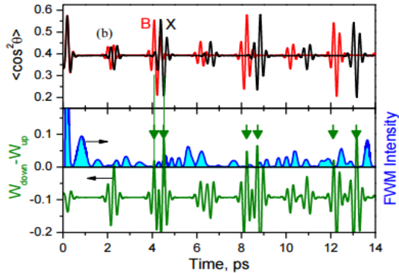
Figure 6.15: Evolution of the rotational alignment factor \langle \cos^2(\theta(t)) \rangle , calculated probability difference between UV absorption and emission for P_B = 3/4P_X , and theoretical UV emission intensity due to four-wave mixing. Courtesy to the ref [71].
