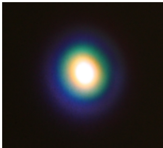
Figure 1.4: Photograph of the conical emission by femtosecond laser filamentation in air.
