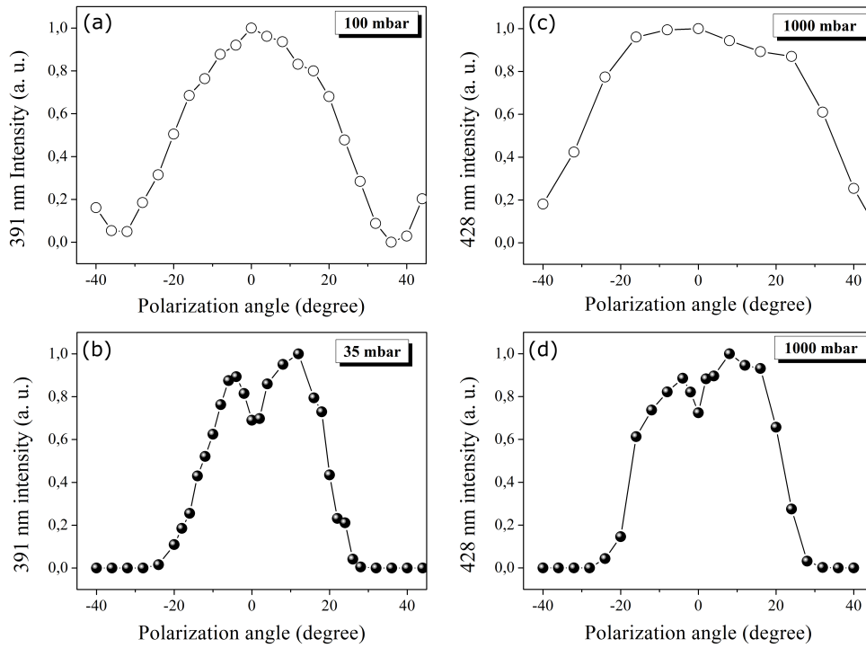
Figure 5.11: The 391 nm and 428 nm transverse fluorescence and forward lasing emission at a function of the ellipticity of the pump laser pulses at 800 nm. The polarization angle of 0^\circ ( 45^\circ ) corresponds to ellipticity of 0 (1), e.g., linear (circular) polarization. (a) The 391 nm transverse fluorescence was measured by using 2.5 mJ pump pulse energy under 100 mbar nitrogen pressure; (b) The forward 391 nm lasing emission was measured by using 2.7 mJ pump pulse energy under 35 mbar nitrogen pressure; (c) The transverse 428 nm fluorescence was measured by 3.5 mJ pump pulse energy under 1 bar air; (d) The forward 428 nm lasing emission was measured by using 2.7 mJ pump pulse energy under 1 bar nitrogen. In all these measurements, the focusing length was 40 cm.
