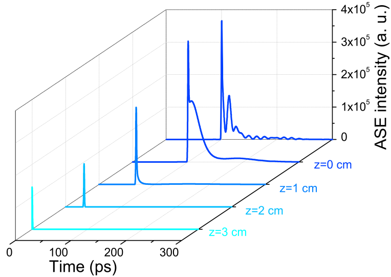
Figure 4.9: Simulation result of temporal profiles of backward seeded 337 nm lasing pulse at different positions ( z ) of the filament plasma amplifier with n_e = 1.2 \times 10^{16} \text{ cm}^{-3} and T_e = 16 \text{ eV} .
