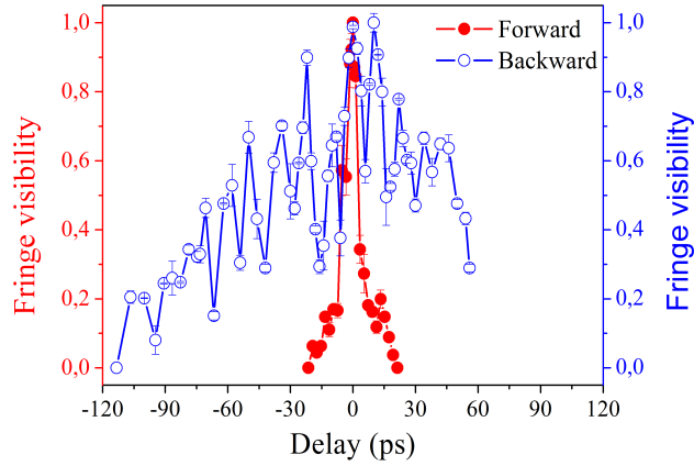
Figure 2.21: Fringe visibility of both forward and backward 337 nm ASE lasing as a function of time delay between two identical arms in Michelson Interferometer. The measurement in positive delay range is incomplete because of setup limitation.
