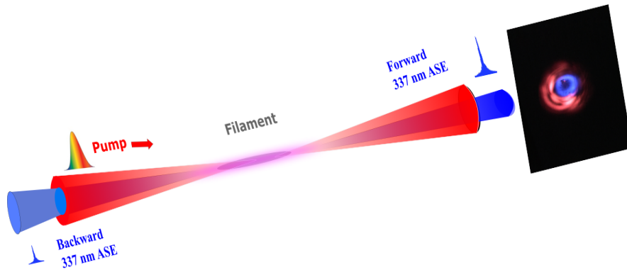
Figure 1.6: Schematic illustration of 337 nm ASE-type lasing effect of neutral nitrogen molecules in filament plasma. The photograph for forward 337 nm ASE is shown on the right.
