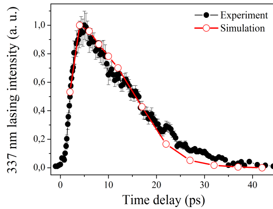
Figure 4.5: Experimental (solid black dots) and simulation (red circles) results of the gain dynamics of 337 nm lasing emission with 7.5 mJ pump pulse energy under 1 bar nitrogen gas.
