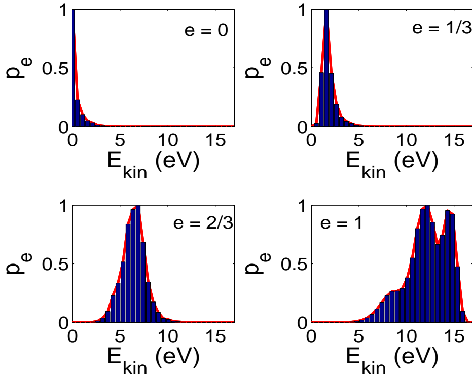
Figure 4.3: Distribution of kinetic energies for electrons generated by a laser pulse with peak intensity of 10^{14} \text{ W/cm}^2 and ellipticity e = 0 , e = 1/3 , e = 2/3 and e = 1 . The curves show the theoretical result. The blue bars show the result of a direct numerical simulation.
