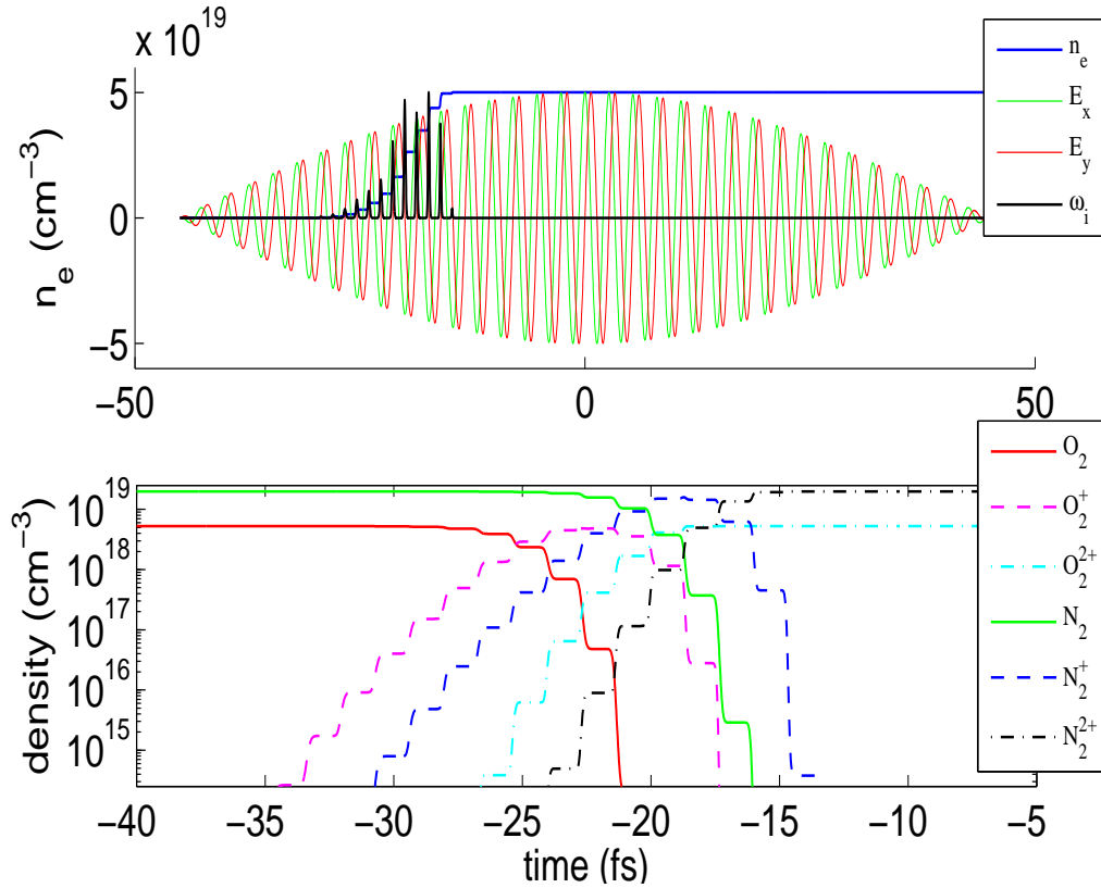
Figure 4.2: Ionization of air for a laser pulse with peak intensity of 10^{14} \text{ W/cm}^2 and ellipticity e = 1/3 . (a) Electron density (blue curve) and ionization probability \omega_i in arbitrary unit (black curve). The component of the electric field E_x and E_y are superimposed as a guide for the eye to see the instant of ionization. (b) Densities of oxygen and nitrogen molecules, and ions.
