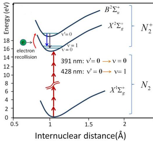
Figure 5.1: Schematic diagram of relevant energy levels of nitrogen ions. The symbols \nu and \nu' denotes the quantum numbers of vibrational levels.
