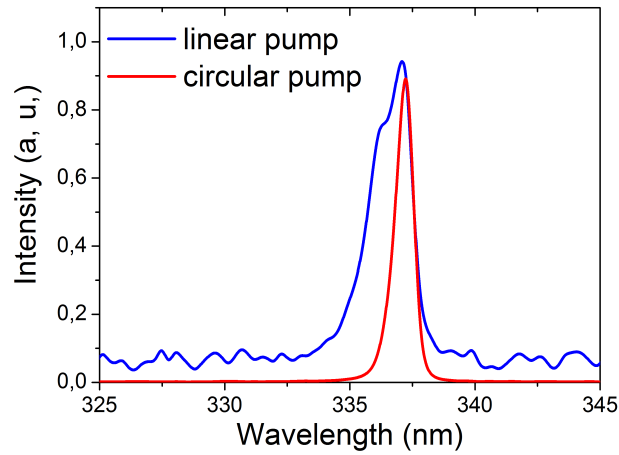
Figure 2.6: The spectra of 337 nm emission in the backward direction for linear and circular pump laser, in which their intensities are normalized.
