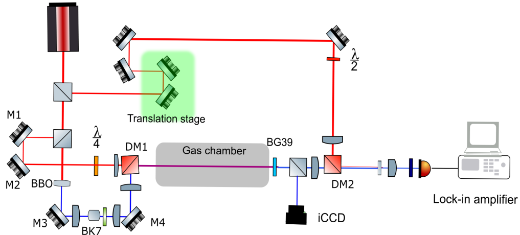
Figure 3.1: Schematic illustration of co-propagating configuration for measuring the gain dynamics and temporal profile of 337 nm lasing emission.
