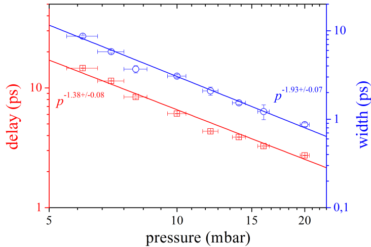
Figure 6.10: Pressure dependence of the pulse width and delay of 391 nm lasing emission in filament plasma in nitrogen.
