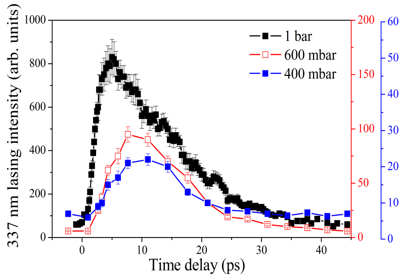
Figure 3.11: Measured forward amplified 337 nm lasing signal as a function of the relative time delay between the pump and seeding pulse. The pump pulse energy was 7.5 mJ and the focal length is 1 m.
