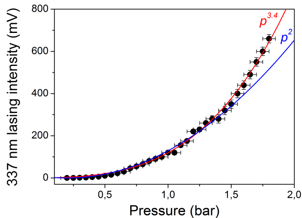
Figure 2.13: 337 nm lasing emission in forward direction as a function of the nitrogen gas pressure. The pump pulse energy is about 9 mJ and the focal length is 1 m. The polarization of pump pulse was set to be circular. The line curves show the polynomial fits.
