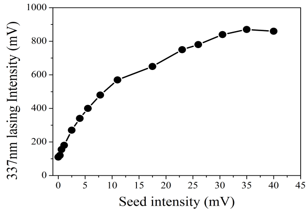
Figure 3.4: The forward externally-seeded 337 nm lasing intensity as a function of the seed intensity. The pump pulse energy was kept as 7.2 mJ.
