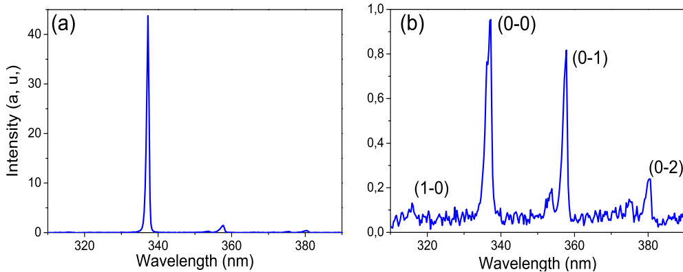
Figure 2.5: Backward emission spectra from 6-cm long filament plasma generated by circularly (a) and linearly (b) polarized pump pulses in 1-bar nitrogen gas.
