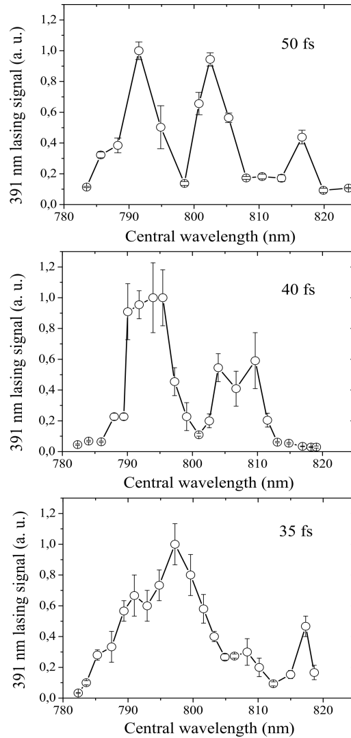
Figure 6.5: Measured forward 391 nm lasing intensity as a function of central wavelength of pump laser pulse for three different pulse durations, respectively 35 fs, 40 fs and 50 fs. In the case of 35 fs duration, the pump pulse energy is about 0.38 mJ and the nitrogen gas pressure was kept at 5 mbar. In the case of 40 fs duration, the pump energy can be maximal as 1.1 mJ and the pressure was kept at 2.5 mbar. In the case of 50 fs, the pump pulse energy is 0.7 mJ and the gas pressure was 5 mbar. The detector we used is a calibrated photodiode.
