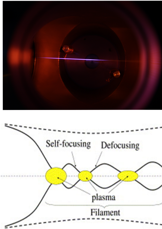
Figure 1.3: (upper panel) A 10-cm-long filament created by focusing 10 mJ 800 nm laser pulse in 1 bar nitrogen gas. (lower panel) Schematic illustration of the focusing-defocusing cycles undergone by the laser pulse along the propagation axis. Courtesy to the ref. [1].
