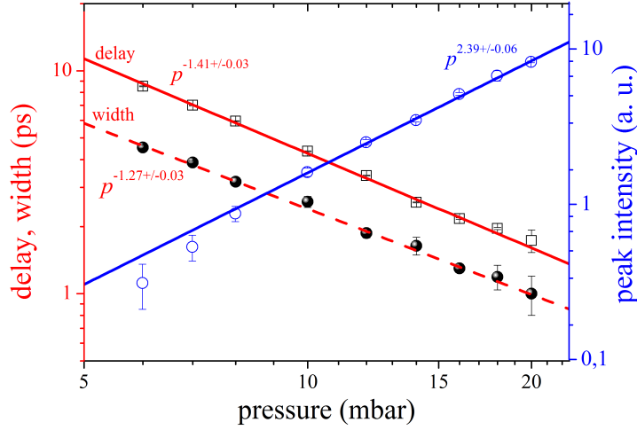
Figure 6.11: Pressure dependence of the pulse width, delay and peak intensity of externally-seeded 391 nm lasing emission. The solid lines are fitting of the form ap^b + c to the extracted delay and width.
