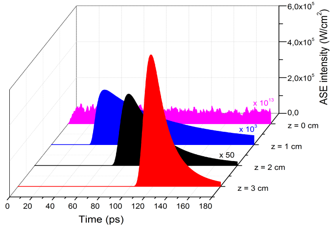
Figure 4.6: Simulated temporal profile evolutions of the 337 nm ASE-type lasing pulse along the 3-cm-long filament plasma in the forward direction. The z term denotes position on filament plasma along the propagation direction of IR pump laser. For better comparison, some curves are enlarged by different factors, which are denoted beside the curves.
