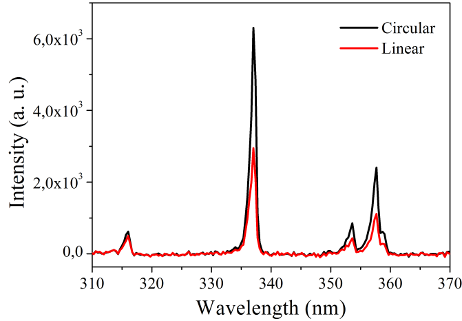
Figure 2.15: Spectra of backward 337 nm emission from filament plasma in 1 bar air both for circular and linear pump laser.
