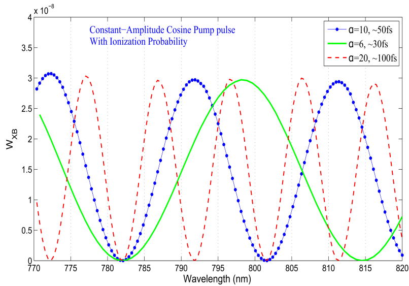
Figure 6.3: Simulated total excitation probability as a function of pump laser wavelength for three different numbers of optical cycles, i.e., \alpha = 6, 10, 20 , corresponding to pulse durations of \sim 30 fs, \sim 50 fs and \sim 100 fs, respectively.
