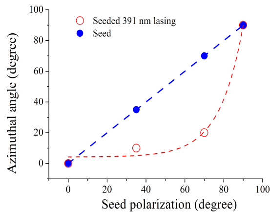
Figure 5.18: The azimuthal angle \phi of the polarization direction of seeded 391 nm lasing emission as a function of the polarization angle \theta of the seed pulse. The azimuthal angle of polarization direction of the seed pulse is equivalent to \theta , shown by the dashed blue line. The dashed red line represents an exponential fit to the data of seeded 391 nm lasing emission.
