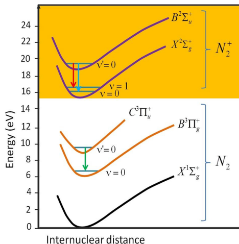
Figure 2.1: Schematic diagram of the potential energy levels of the neutral and ionic nitrogen molecule. The symbols \nu and \nu' denotes the quantum numbers of vibrational levels.
