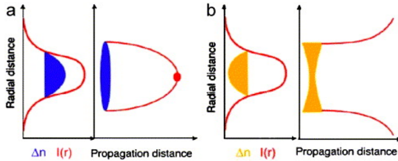
Figure 1.2: (a) Schematic illustration of the self-focusing of a laser beam. The varying refractive index of the medium with the strength distribution of laser beam converges the initially collimated beam, acting as a positive lens. (b) Plasma defocusing of the laser beam. The ionization of the medium initially takes place along the axis, where the laser intensity is maximal. The weakly ionized plasma decreases the local refractive index and therefore causes beam defocusing. Courtesy to the ref. [1].
