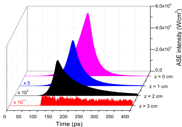
Figure 4.7: Simulated temporal profile evolutions of backward 337 nm ASE-type lasing pulse along the 3-cm-long filament plasma. The z term denotes position on filament plasma along the propagation direction of IR pump laser.
