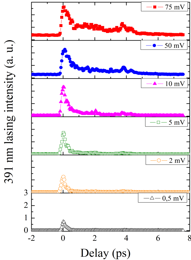
Figure 5.19: Gain dynamics of 391 nm lasing emission for different seed intensity ranging from 0.5 mV to 75 mV. The zero delay is defined as the time when the maximal signal is detected.
