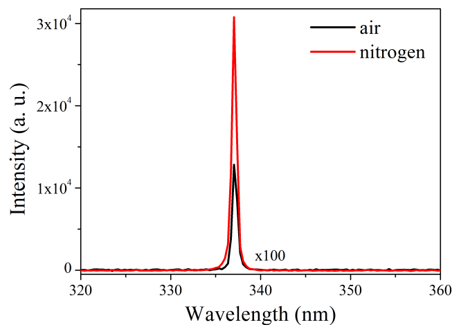
Figure 2.14: Spectra of forward 337 nm ASE lasing emission from filament plasma in air and nitrogen with pressure of 1 bar. The lasing intensity in air was magnified by one hundred times for easier comparison.
