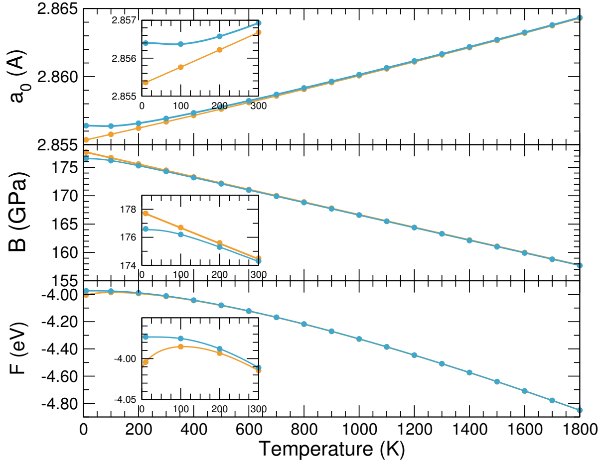
Figure 5.4: The values of lattice parameter ( a_0 ), isothermal bulk modulus ( B ) and the free energy ( F ) of the bcc phase of iron (Ackland-Mendelev potential (99)) from QHA approximation implemented in this thesis and force brute calculation (as it is explained in the text). The solid line and circles emphasize the QHA and brute force calculations, respectively. The phonon gas is quantized (blue) or treated in classical approximation (orange).
