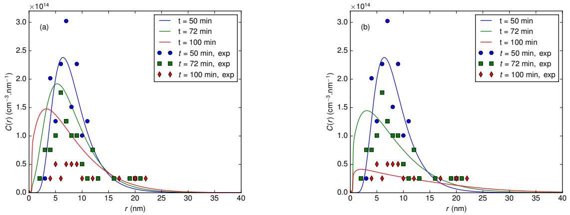
Figure 5.17: Loop distributions obtained at different times with a capillary law, for a migration free energy of the vacancy equal to (a) 0.51 eV and (b) 0.45 eV.
