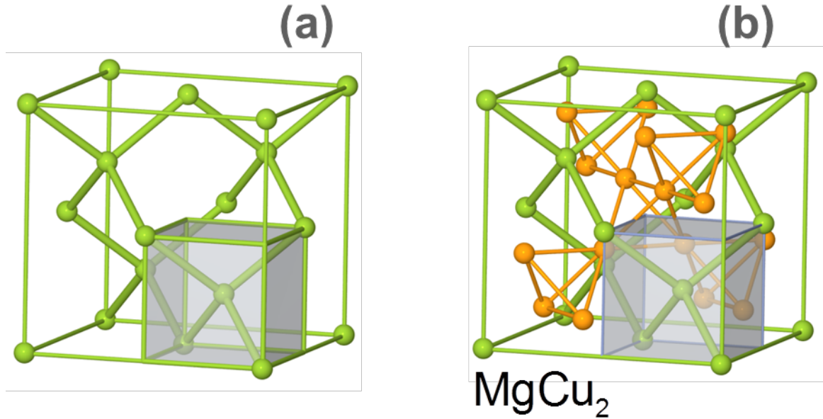
Figure 3.6: (a) The spheres in green represent the possible centers of the Z16 polyhedra. We can easily recognize the diamond structure. The plotted cube is the cubic unit cell of the original bcc lattice. (b) The unit cell of the cubic phase of Laves C15 or MgCu_2 , with the Mg atoms in green and the Cu atoms in orange. In our convention the green atoms correspond to the atoms which are the center of Z16 polyhedra and the orange atoms are the atoms which are in the interstitial positions.
