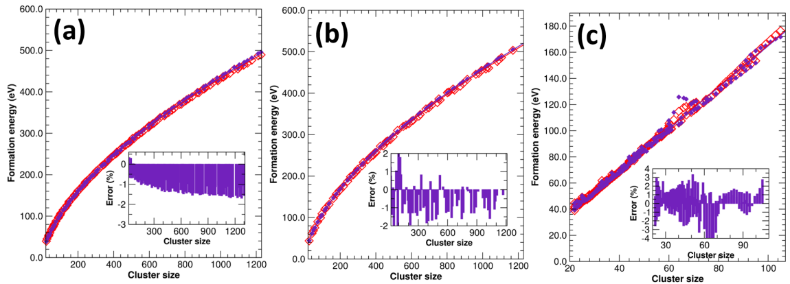
Figure 4.10: Cluster formation energies as a function of cluster size for (a) 1/2\langle 111 \rangle and (b) \langle 100 \rangle loops and for (c) C15 SIA clusters in Fe calculated using the Ackland-Mendelev potential for Fe (99). Open diamonds represent the direct EAM results derived from simulations using large cells while the blue full diamonds represent values predicted by the discrete-continuum model. The relative errors are plotted as insets. Note that for the nanometric clusters the relative error is less than 3%.
