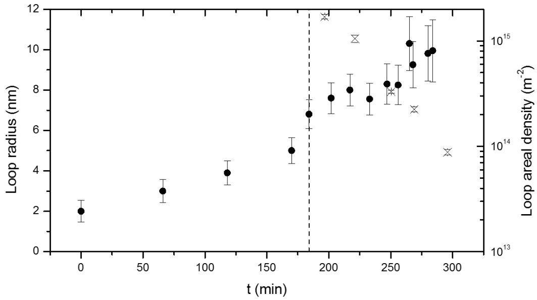
Figure 5.12: Loop radius as a function of time. The two regions separated by a vertical dotted line represent isochronal annealing at 3K/\text{min} . and isothermal in-situ annealing at 830\text{ K} , respectively.
