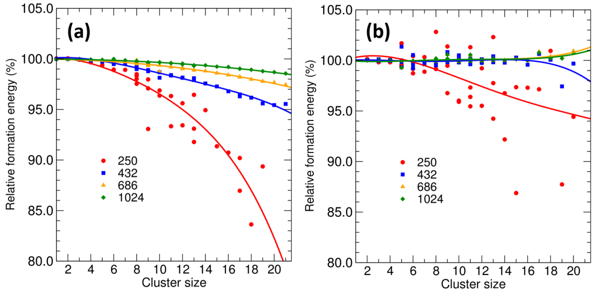
Figure 4.9: Formation energies of n SIA clusters of (a) 1/2\langle 111 \rangle and (b) \langle 100 \rangle dislocation loops in Fe, computed with an EAM potential (99) with different configurations in cubic simulation cells containing 250 + n (red circle), 432 + n (blue square), 686 + n (orange triangle up) and 1024 + n (green rhombus) atoms. All energies are normalized to the asymptotic limit, taken as the formation energy in a simulation cell containing 207646 + n atoms. Lines are guides for the eyes, obtained using a fit to a 4 th order polynomial. Formation energies have been corrected using the elastic dipole correction method to account for the finite size of the simulation cells (230).
