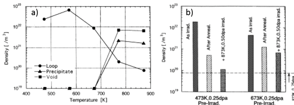
Figure 1.13: Defect density evolution in Vanadium, irradiated using 3 MeV Cu^{3+} ions, is studied at various temperature variations a) shows the variation in density of three types of defects (loops, precipitates and voids) as a function of temperature b) shows number density of interstitial dislocation loops at various temperatures and irradiation conditions. Figure taken from Ref. (157)
