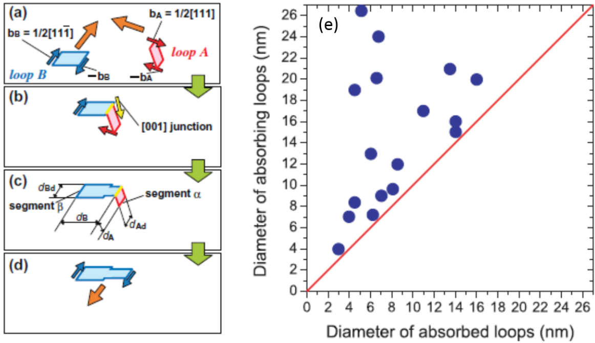
Figure 1.9: (a)-(d) Schematical representation of the experimentally observed absorption of a smaller loop by a larger loop with a change in Burgers vector of the smaller loop while (e) Plot showing the diameter of absorbing and absorbed loops (in nm). This graph illustrates that absorbed loop size is always found to be smaller than the absorbing loop size. Figure taken from Ref. (104)
