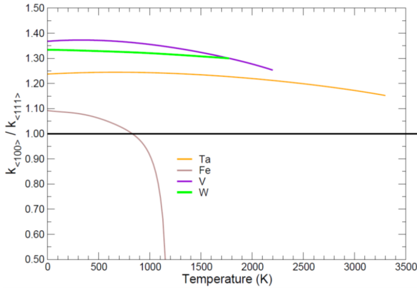
Figure 4.3: Ratio of k_b = Kb^2 of \langle 100 \rangle dislocation loops to k_b value of 1/2 \langle 111 \rangle dislocation loops is plotted as a function of temperature. This ratio provides information regarding the relative stability of the compared dislocation loops. On the basis of this graph, the 1/2 \langle 111 \rangle dislocation loops are more stable than \langle 100 \rangle for bcc metals, except for iron at higher temperatures (greater than 830 K). The k_b -values are plotted up to melting point for the bcc metals, except iron where the plot is limited till its Curie temperature.
