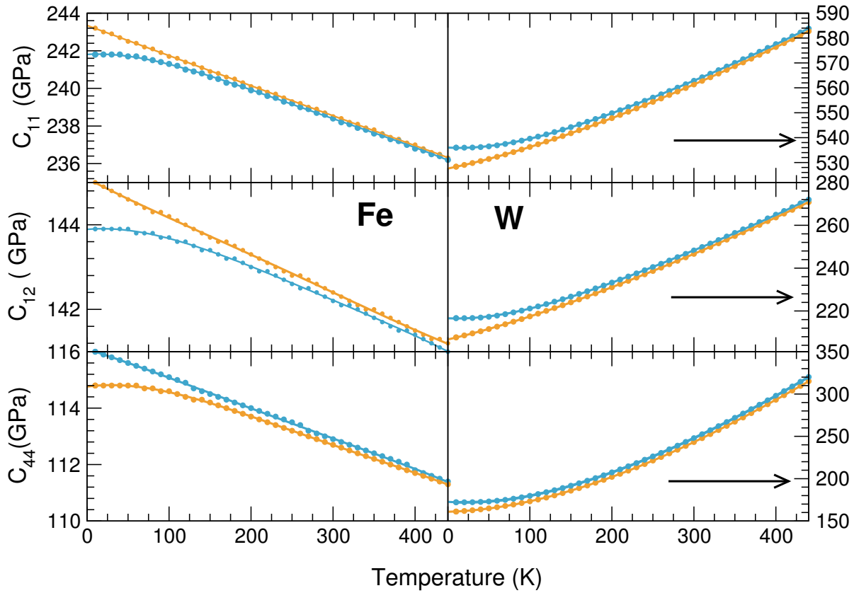
Figure 5.6: The values from QHA approximation of the isothermal elastic constant of bcc phase using two empirical potentials for iron ( 99 ) (left) and W ( 135 ) (right). The phonon gas is quantized (blue) or treated in classical approximation (orange).
