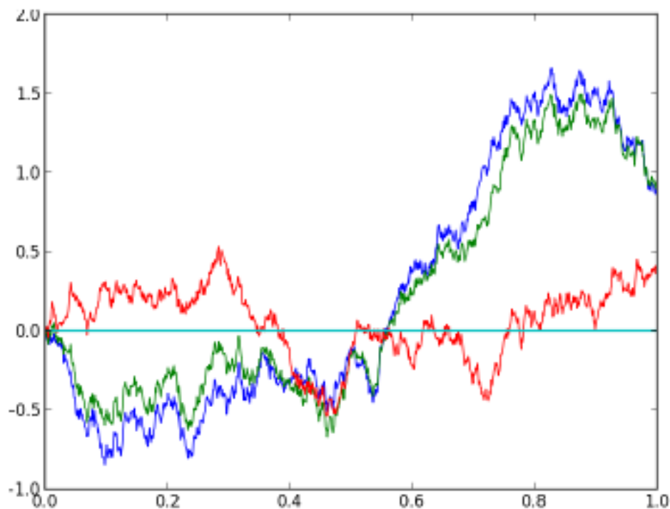
FIGURE 1.2: Gaussian shaking transformation applied on the entire path of an Ornstein-Uhlenbeck process with different shaking parameters: path before shaking in blue, paths after shaking in red and green
