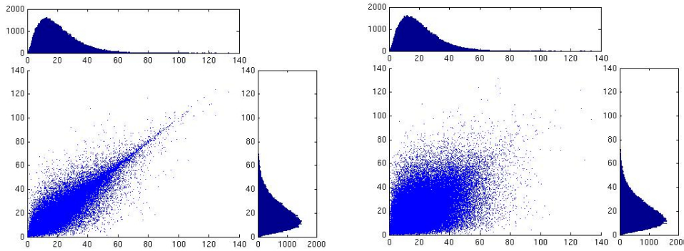
FIGURE 5.4: Shaking Gamma(2.5, 0.12) variables with p = 0.1 (left) and p = 0.5 (right)
