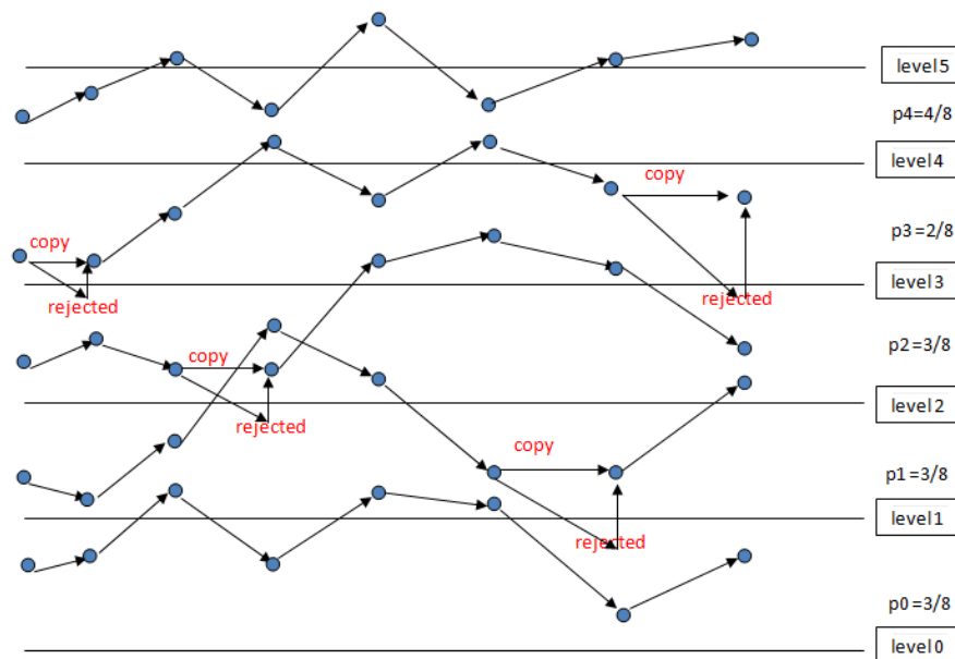
FIGURE 5.2: POP method illustration, computing probability that X as a point lies above level 5
