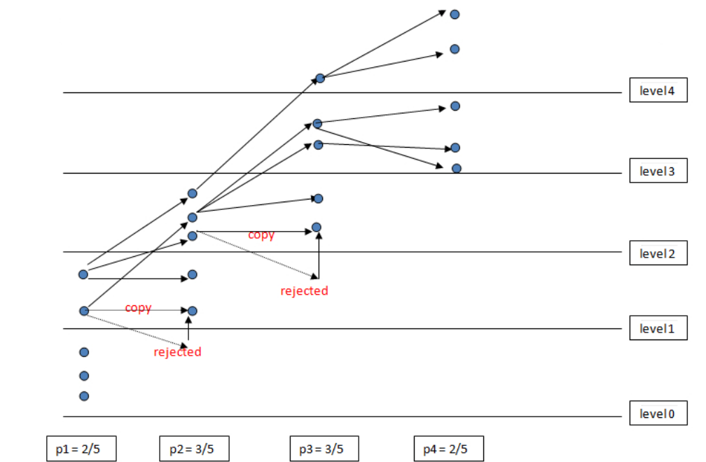
FIGURE 5.1: IPS method illustration, computing probability that X as a point lies above level 4
