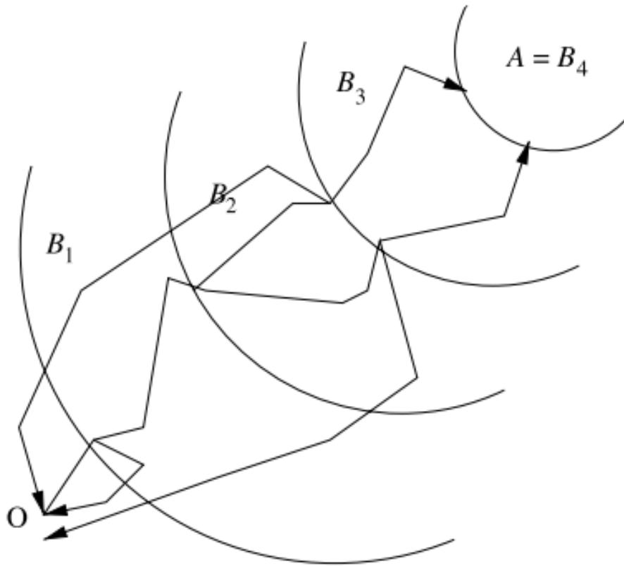
FIGURE 3.3: Splitting illustration from [93]
