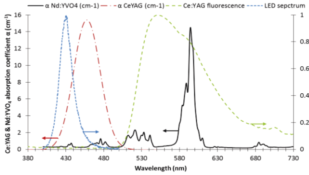
Fig. 2. Ce:YAG (red) and Nd:YVO 4 absorption coefficient (average of c and a axes, black) and emission spectra of Ce:YAG (green) and LED in pulsed regime (100 μs, 4 A, 10 Hz, room temperature, blue).
