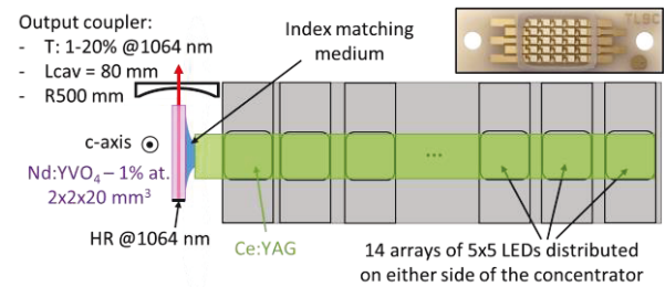
Fig. 3. Overall setup of the experiment. Inset: illustration of an LED array.
