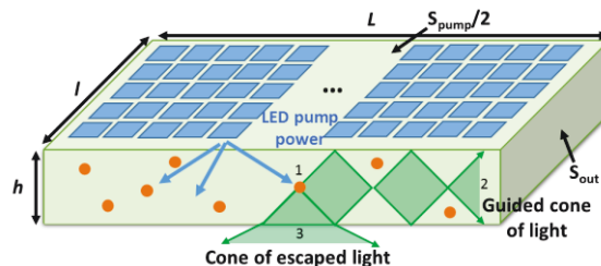
Fig. 1. Schematic representation of a light concentrator pumped by LEDs. (1) Pump light is absorbed by a luminophore. (2) Light is reemitted and guided toward the edges of the LC by TIR. (3) A part of the reemitted light escapes the LC and is lost.
