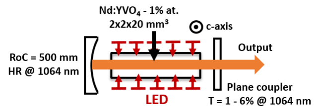
Fig. 3. Experimental setup.
