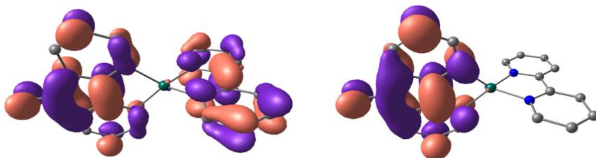
Figure 4.9. SOMO of \mathbf{I}^{*+} computed at the B3LYP (left) and LC-BLYP (right) level.
