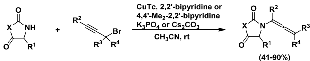
Scheme 2-4 Straightforward synthesis of allenamides from propargyl bromides
