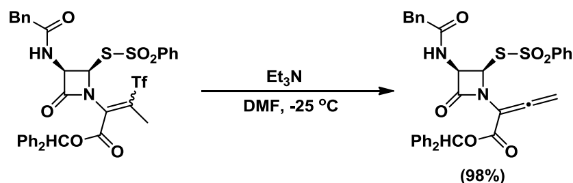
Scheme 2-7 Synthesis of allenamide via E2 elimination
