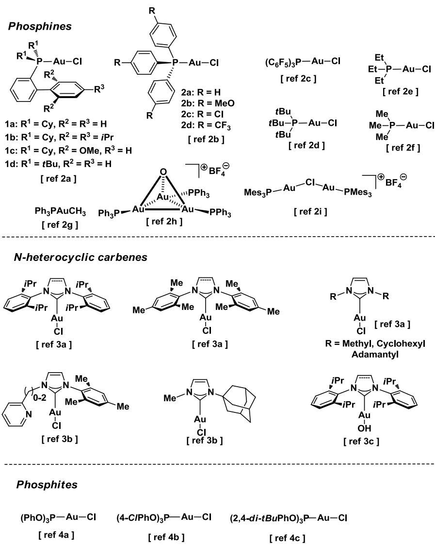
Figure 1-8 Representative examples of gold(I) complexes
