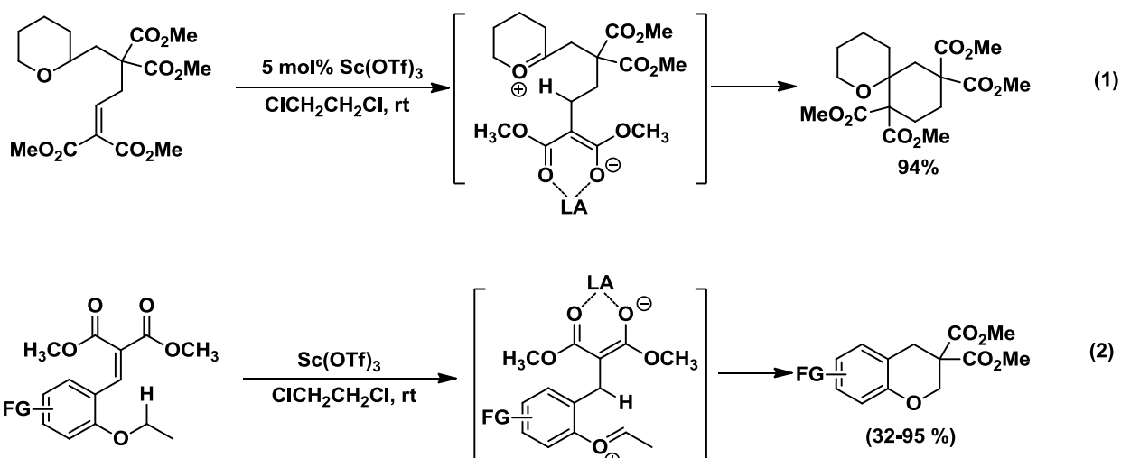
Scheme 2-9 [1,5]-hydride transfer with alkylidenemalates as hydride acceptors
