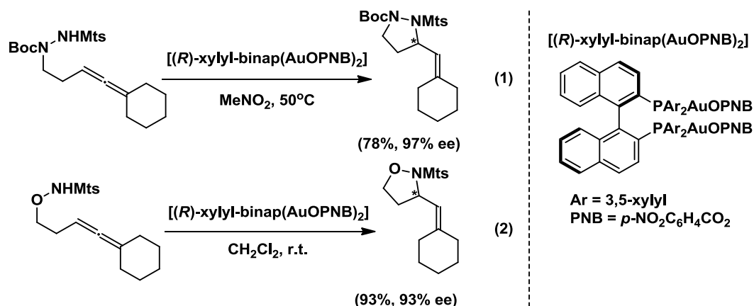
Scheme 1-13 Enantioselective hydroaminations of allenes
