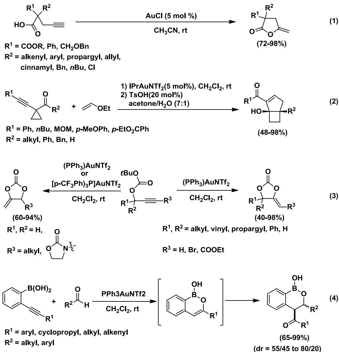
Scheme 1-6 Cycloisomerizations of alkynes bearing various O -nucleophiles
