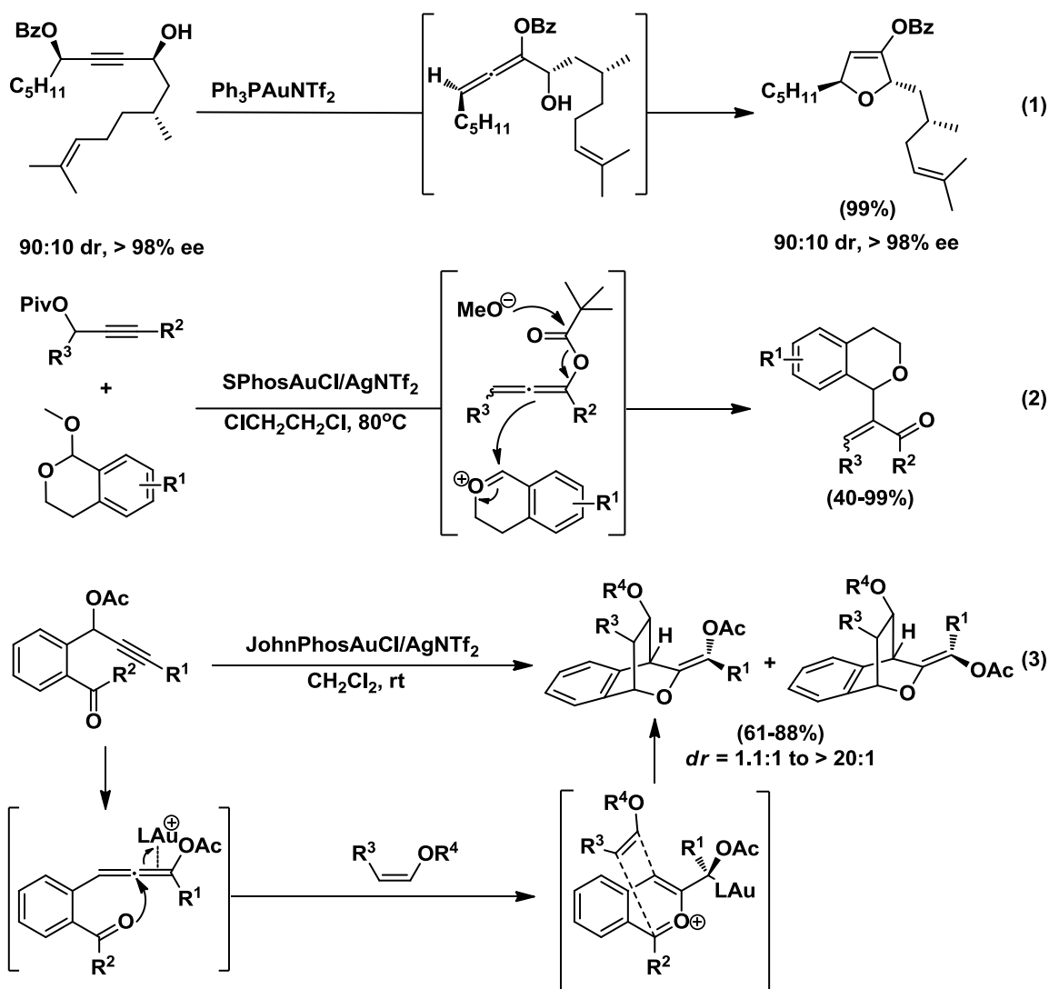
Scheme 1-24 Au(I)-mediated transformations of propargylic carboxylates
