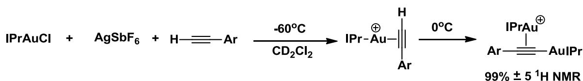
Scheme 3-6 formation of \sigma , \pi -digold acetylides
