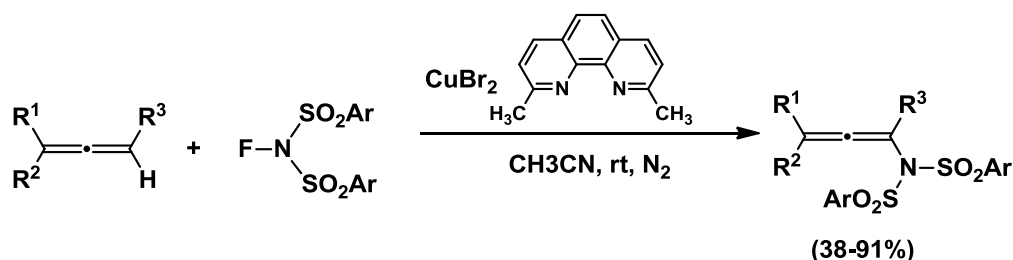
Scheme 2-8 Allenamides synthesis by radical amination strategy
