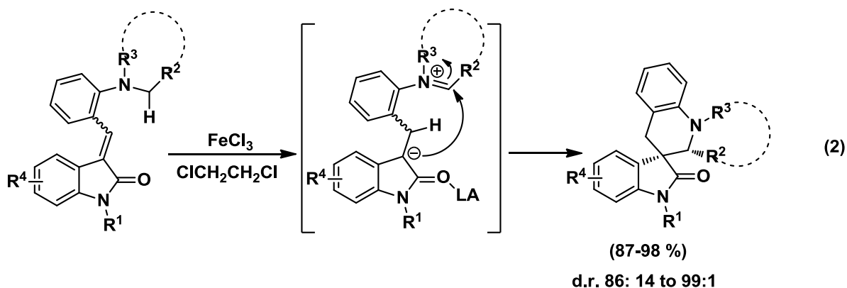
Scheme 2-12 Functionalization of C-H bond \alpha to amines
