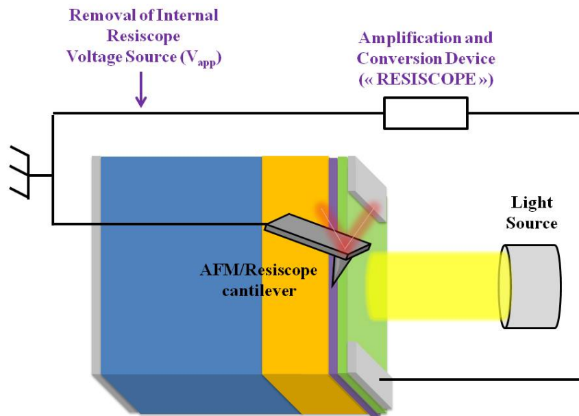
Fig. 6.21 – Resiscope setup used to investigate the cross-section of epitaxial silicon solar cell under illumination. Compared to the conventional Resiscope setup, the DC voltage source has been removed to be sensitive only to the photocurrent.
