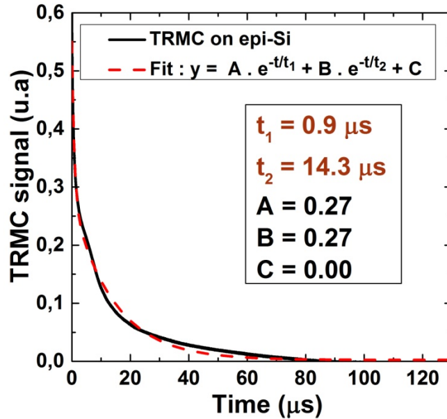
Fig. 6.16 – TRMC measurement on 5 \mu m both sides HF passivated epi-Si sample. A fitting with two exponential curves is required. The first time constant is around 1 \mu s. The second time constant is around 10 \mu s.
