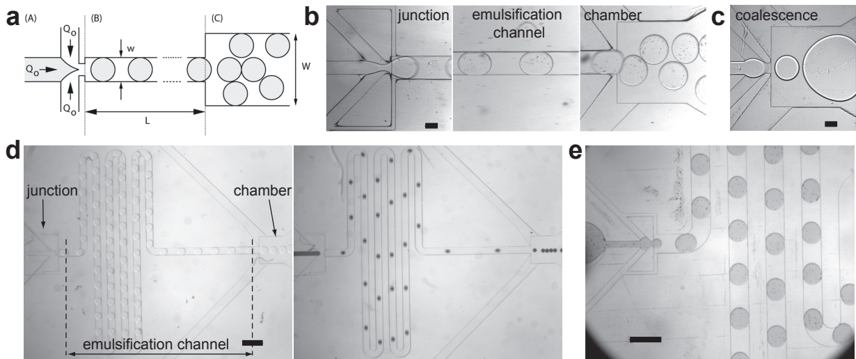
Figure 1.9: EMULSIFICATION CHANNEL. (a) Schematic principle of the emulsification channel (reproduced from Baret et al. [47]). w is the width of the emulsification channel. (b) Images of the droplet production at different stages for a straight emulsification channel. w = 350 \mu\text{m} . Scale bar is 200 \mu\text{m} . (c) Droplet production with the same surfactant concentration as in (b) but without an emulsification channel. Scale bar is 200 \mu\text{m} . (d-e) Droplet production with a serpentine emulsification channel for various droplet sizes. Scale bars are 1 \text{ mm} . (d) w = 325 \mu\text{m} . (e) w = 600 \mu\text{m} .
