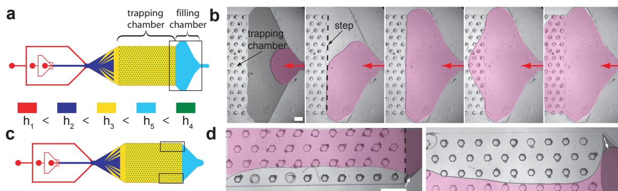
Figure 2.4: GUIDING THE MEDIUM FILLING WITH A STEP. (a) Schematic representation of the chip design. The filling chamber is the cyan area and it has a height h_5 higher than the height h_3 of the trapping chamber in yellow. The black rectangle represents the location of the images in (b). (b) Time lapse images of the medium perfusion with a filling chamber. The red arrows represent the medium flow. (c) Schematic representation of the chip design with a triangular filling chamber. (d) Images of the corners of the trapping chamber after the phase change. White arrows show the curvature of the aqueous phase in the wedges of the triangular filling chamber. Red and black overlays highlight respectively the aqueous medium and the filling chamber. The black dashed lines show the location of the step. Scale bars are 1 mm.
