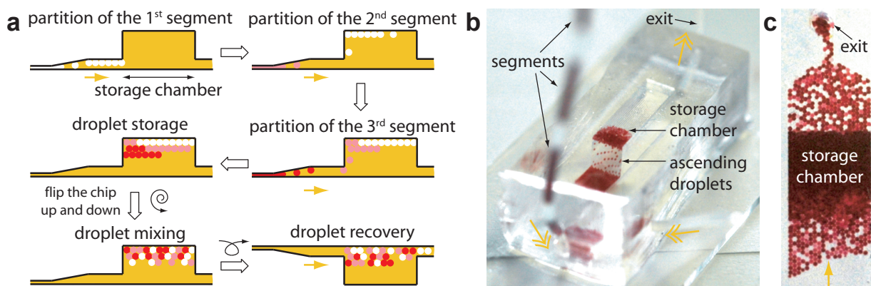
Figure B.7: PARTITION OF THE SEGMENTED FLOWS AND DROPLET MIXING. (a) Schematized protocol showing at every step a side view of the droplet production chip. The spiral arrow indicates that the chip is flipped several times to ensure a good mixing of the droplets in the storage chamber. (b) Image of an experiment showing the production of the droplets from the segments. (c) Top bottom view of a droplet production chip during the droplet recovery after mixing in the storage chamber. Yellow arrows represent the oil flowrate.
