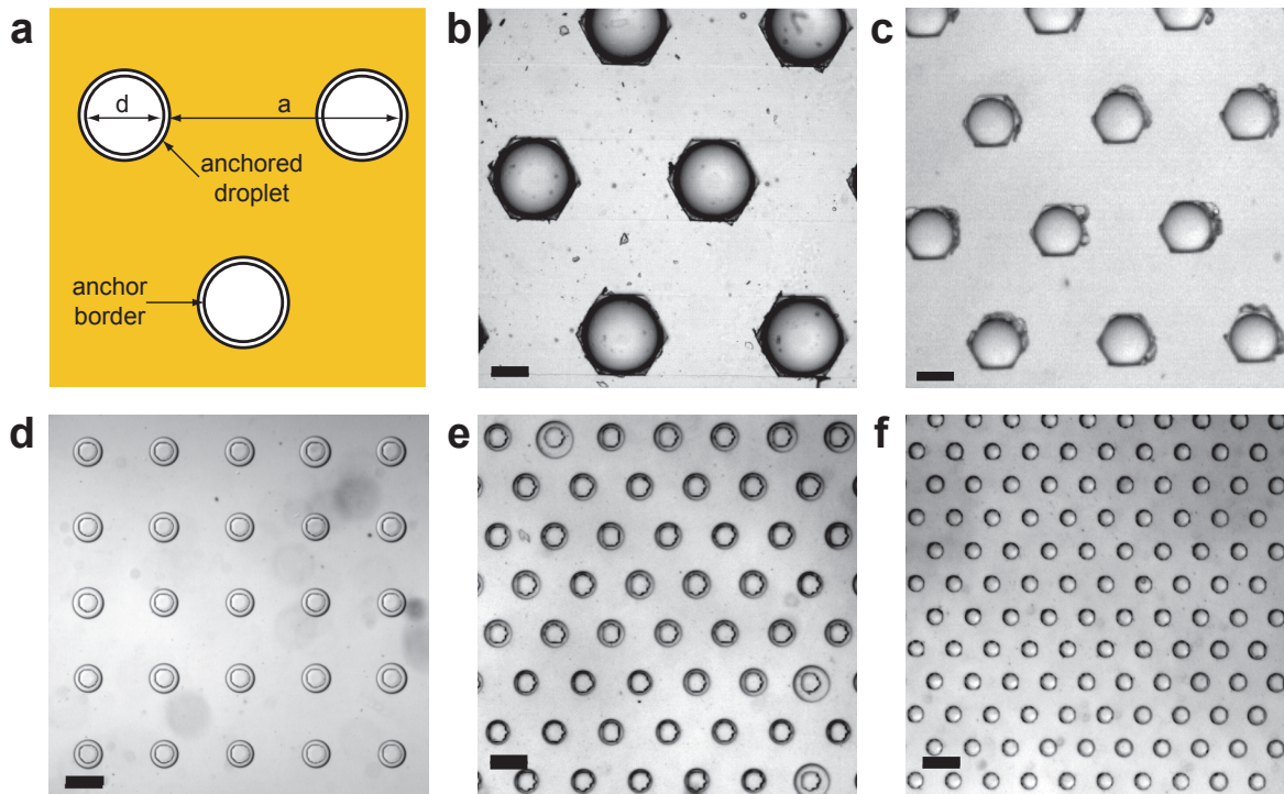
Figure 1.10: DROPLET ARRAYS WITH INCREASING DENSITIES. (a) Schematic representation of 3 aqueous droplets in oil trapped on anchors in a array with a hexagonal symmetry. d is the anchor diameter and a is the array pitch. (b-f) Images of droplet arrays with various densities. Array densities: (b) 128, (c) 250, (d) 625, (e) 1,283 and (f) 2,887 anchors/cm 2 . Scale bars are 200 \mu\text{m} .
