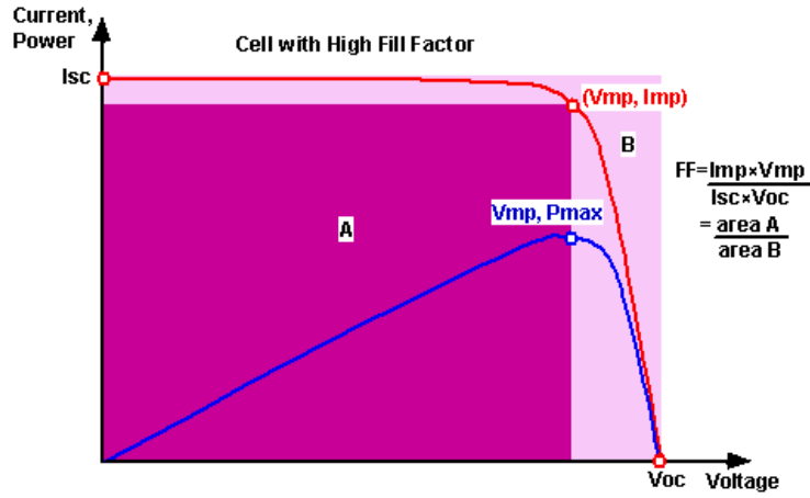
Figure 2-3: (I,V) curve of a solar cell and definition of the photovoltaic parameters [40].
