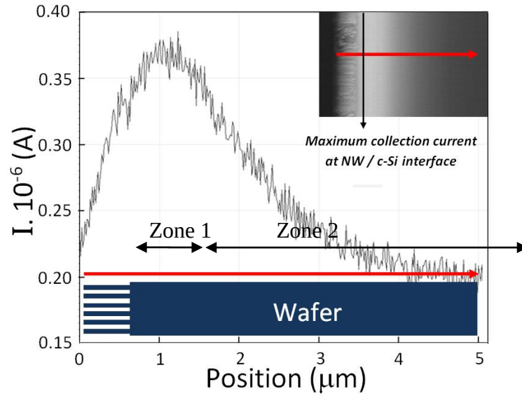
Figure 6-17: EBIC current profile at 10 keV as a function of position of the beam on the sample C with the corresponding EBIC mapping in the inset. The red arrow in the inset indicates the corresponding signal position on the sample. A cross-section schematic of the structure is displayed at the bottom.
