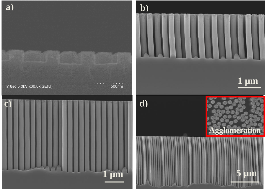
Figure 5-5: Cross-section SEM images of ordered SiNW arrays with a pitch of 330 nm, an average diameters between 239-259 nm and lengths of (a) 163 nm, (b) 2.1 \mu\text{m} , (c) 4.2 \mu\text{m} and (d) 8.2 \mu\text{m} , respectively. The inset in (d) shows the corresponding top-view SEM image.
