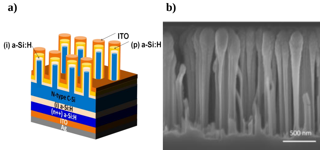
Figure 6-3: (a) Schematic of the structure of the HIT solar cell where the n-type c-Si wafer has been nanostructured to improve light trapping. (b) SEM cross-section of a fabricated device.
