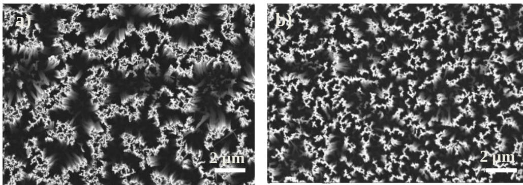
Figure 4-12: SEM pictures of SiNWs arrays (a) before and (b) after RIE post-treatment.
