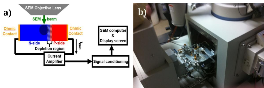
Figure 3-23: (a) Schematics of the EBIC set up [178] and (b) photograph of the EBIC equipment.
