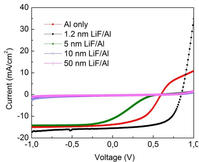
Figure 7-20: (J,V) curves of the thin film devices with LiF/Al cathode (black) and Al cathode (red).
