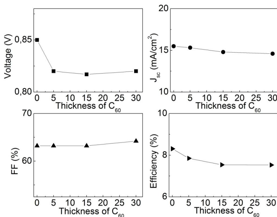
Figure 7-14: Effect of C 60 thickness on the performance of the solar cells.
