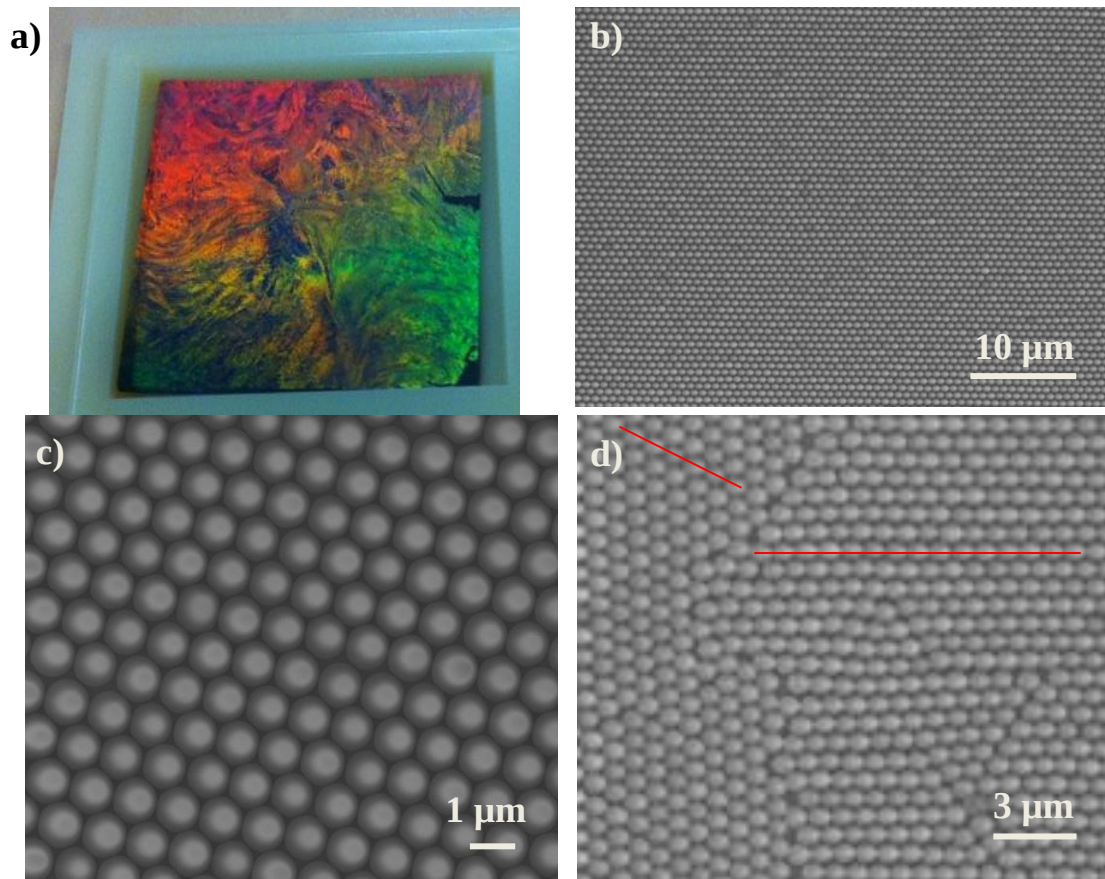
Figure 3-7: (a) Photograph of the Si substrate covered by a monolayer of PS spheres. (b) Low-magnification SEM image of perfectly ordered PS spheres arranged into a hexagonal compact arrangement. (c) ) High-magnification SEM pictures of perfectly ordered PS spheres arranged into a hexagonal compact arrangement. (d) SEM picture of the PS film showing that the film is not uniform everywhere. Small domains coexist with different orientations.
