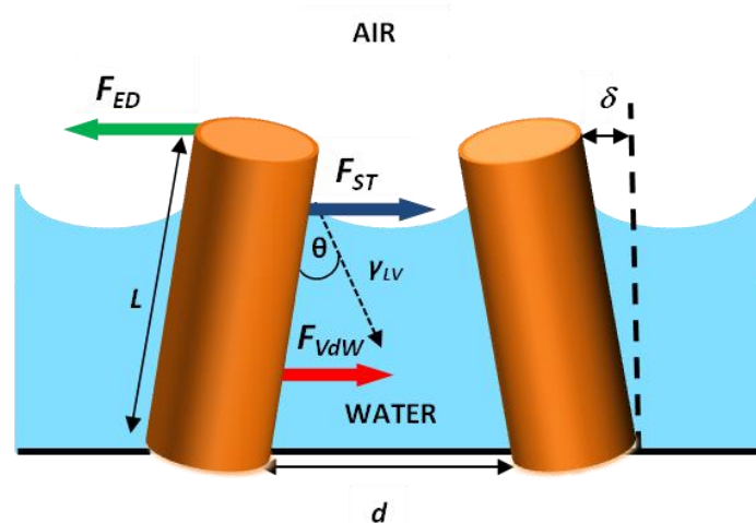
Figure 4-2: Schematic illustration of the forces acting on two SiNWs partially immersed in a liquid. The bending of the SiNWs stems from a balance between the Van der Waals ( F_{vdW} ) and the surface tension ( F_{ST} ) attractive forces and the repulsive elastic deformation force F_{ED} . \gamma_{LV} is the surface tension which characterizes the liquid/vapor interface. \delta is the deflection of the NW.
