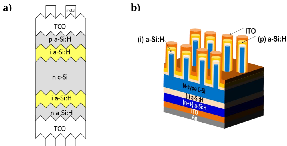
Figure 6-1: Schematic of the structure of (a) a HIT solar cells [125] (b) a HIT solar cell where the n-type c-Si wafer has been nanostructured to improve light trapping.
