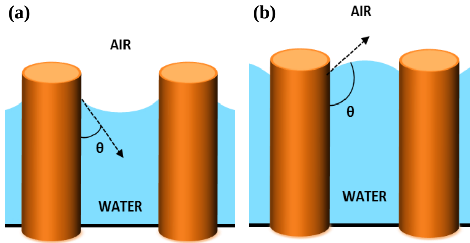
Figure 4-18: Schematic illustration of the water meniscus shape according to the wettability of SiNWs. For hydrophilic SiNWs, the water is wetting on the surface and the meniscus is concave (a) while for hydrophobic SiNWs, the water is non-wetting and the meniscus is convex (b).
