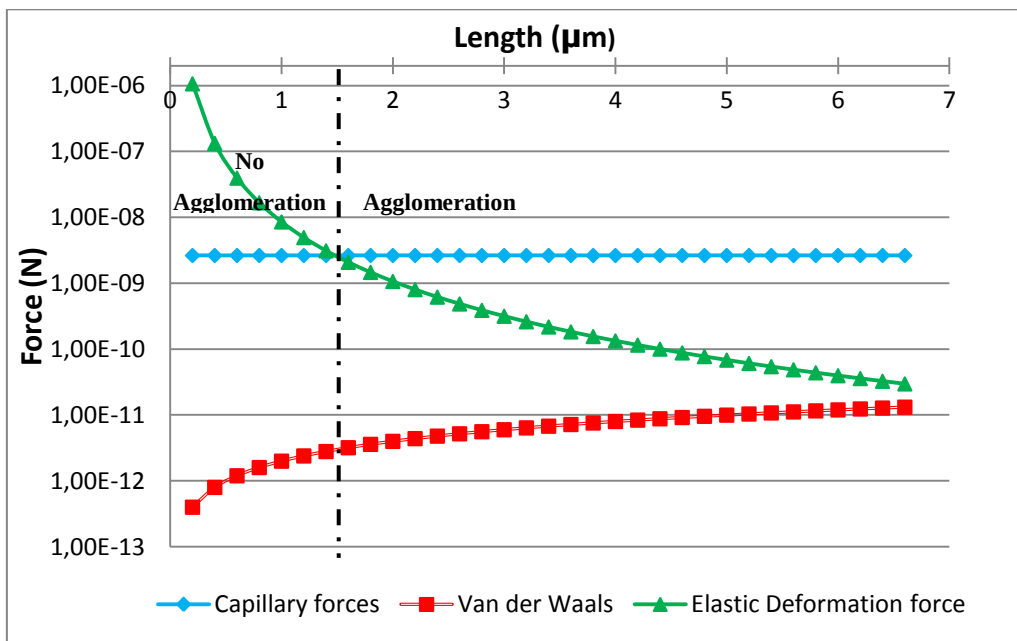
Figure 4-5: Effect of the length on the Van der Waals, capillary and elastic deformation forces
