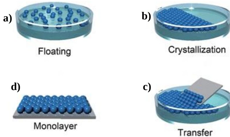
Figure 3-4: Schematics of the floating-transferring technique to achieve an hexagonal compact arrangement of PS spheres on a silicon substrate [143].
