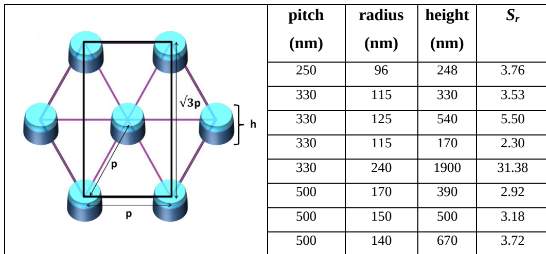
Figure 6-2: Illustration of a hexagonal SiNWs arrays with a pitch p and a height h (left) and calculation of the surface ratios for different geometries (right).
