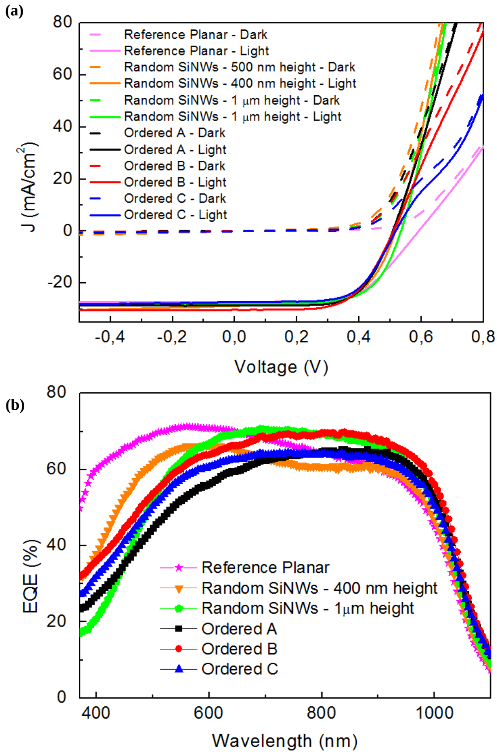
Figure 7-4: (a) (J,V) and (b) EQE of hybrid devices based on disordered and ordered SiNWs.
