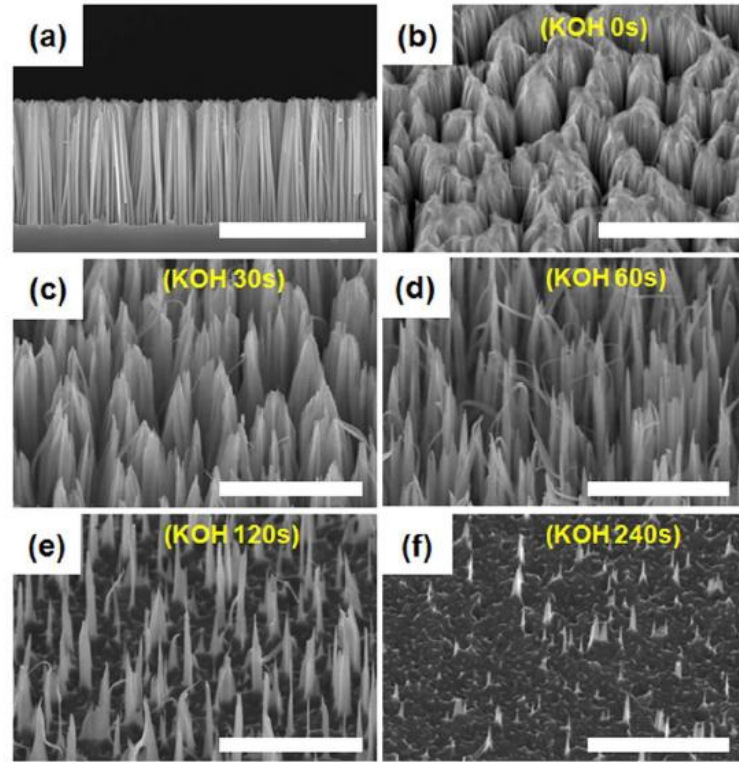
Figure 4-7: (a) Cross-section SEM images of the SiNW array after MACE with a scale bar of 10 \mu\text{m} . Inclined ( 30^\circ ) SEM images showing the effect of KOH post-etching treatment on the morphology of SiNWs as a function of the etching time: (b) 0 s, (c) 30 s, (d) 60 s, (e) 120 s, and (f) 240 s. Scale bars in (b)–(f) are 5 \mu\text{m} [186], [193].
