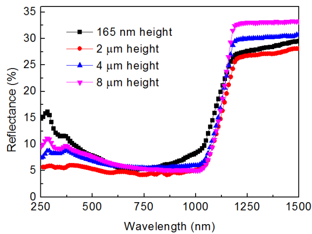
Figure 5-4: Spectral dependence of the total reflectance measured on ordered SiNWs with pitch of 330 nm, diameter of 250 nm (+/- 10 nm) and lengths of 165 nm, 2 \mu\text{m} , 4 \mu\text{m} and 8 \mu\text{m} .
