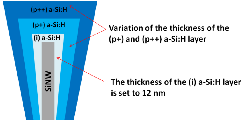
Figure 6-9: Schematic showing the details of the a-Si:H coating.
