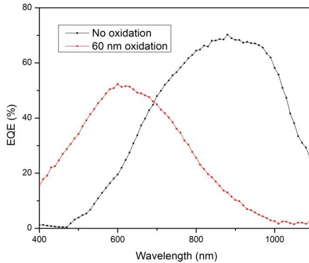
Figure 6-38: Effect of oxidation treatment on EQE
