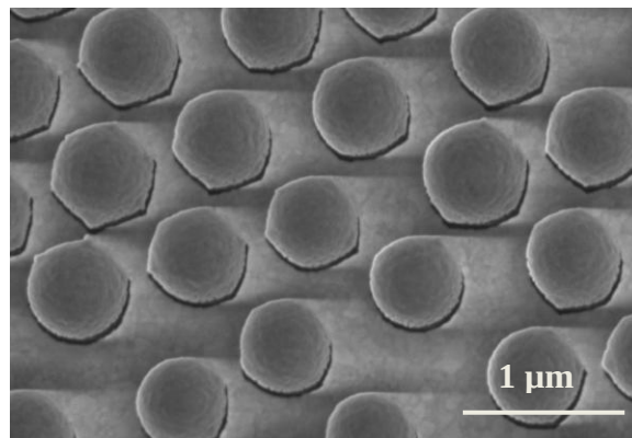
Figure 3-12: SEM pictures of PS sphere arrays covered by a 25 nm gold thin film.
