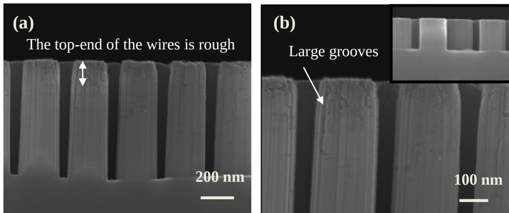
Figure 6-28: Cross-section SEM picture of ordered arrays of SiNWs (pitch 330 nm, diameter 220 nm, length 700 nm) (a) at low and (b) high magnification. The inset (b) shows that the top of the wire is less damaged for short SiNWs (250 nm height).
