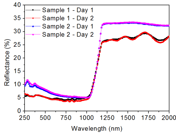
Figure 5-1: Reproducibility of the measured total reflectance data for 2 different samples. Measurements were performed at different locations of the sample on different days, showing good sample uniformity and measurement reproducibility.
