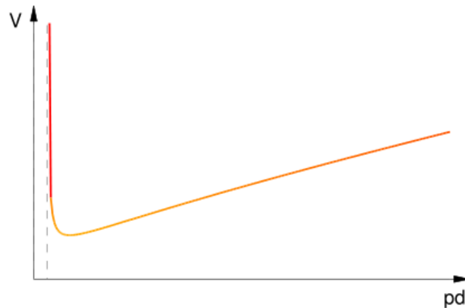
Figure 3-16: The Paschen curve showing the breakdown voltage as a function of the product of the pressure p with the interdistance between the electrodes d [152].
