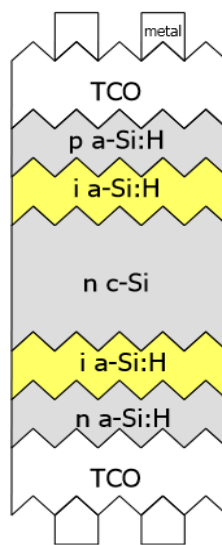
Figure 2-11: Schematics of a standard HIT heterojunction solar cell [125].
