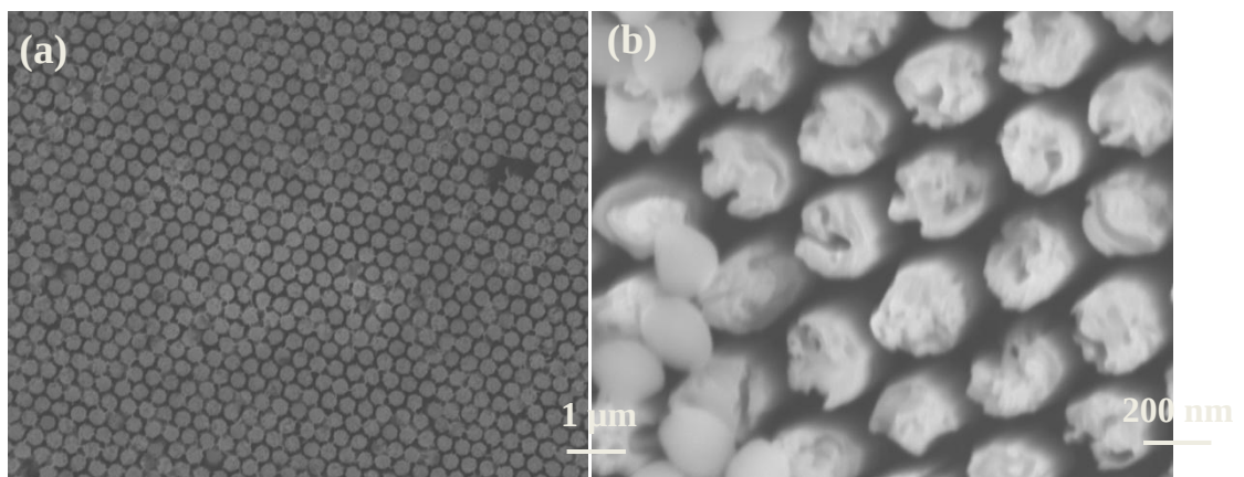
Figure 7-10: Top-view (a) and inclined 30° (b) SEM pictures of a-Si:H NWs.
