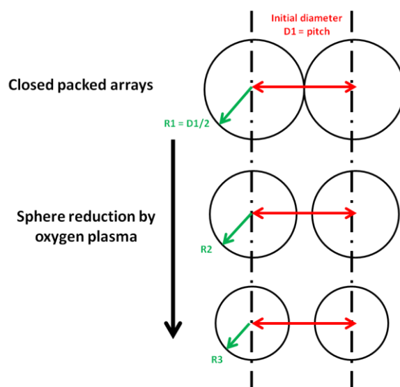
Figure 3-8: Schematics illustrating the effect of the plasma etching treatment on the PS spheres.
