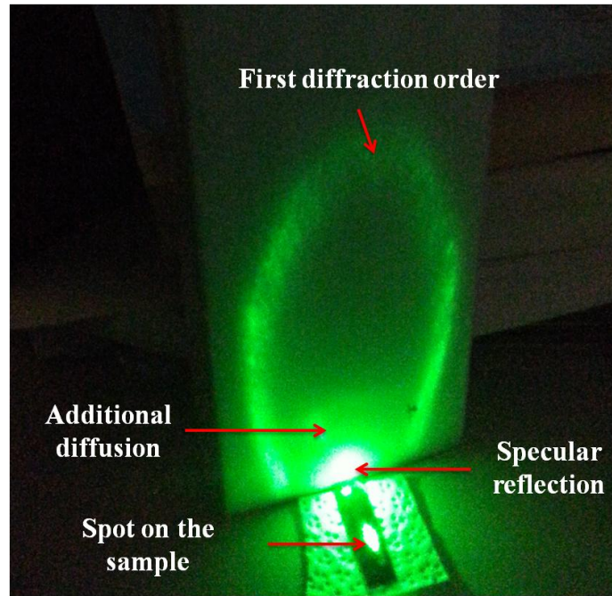
Figure 5-13: Circular diffraction pattern on NWs
