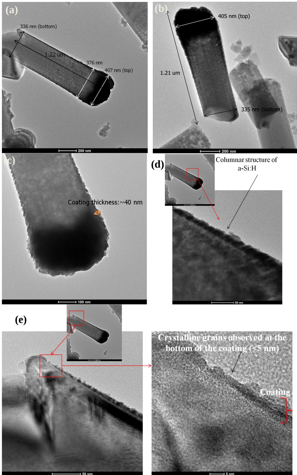
Figure 6-31: TEM analysis of ordered SiNW after a-Si:H coating. The coating of SiNWs by a-Si:H is not uniform (a), (b), it is maximum at the tip of the SiNW (c) and present a columnar structure (c) and (d). Finally, some crystalline grains are observed at the bottom of the coating (e).
