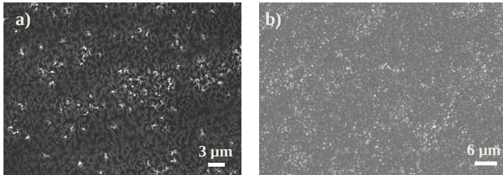
Figure 4-11: Effect of power on the etching of SiNWs (a) At 100 Watt, the SiNWs collapse and lied on the wafer. (b) At 200 Watt, the SiNWs are completely etched away.
