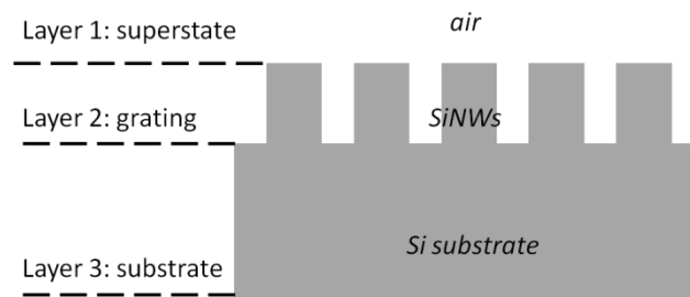
Figure 5-16: Definition of the 3 different layers used in our RCWA modeling.
