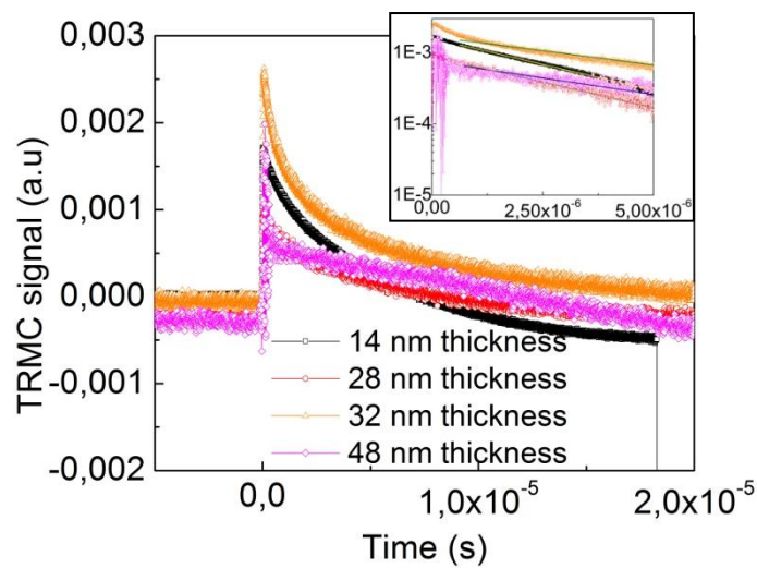
Figure 6-8: TRMC signal as a function of time for HIT solar cells with different a-Si:H thicknesses. The inset shows the signal in logarithmic scale.
