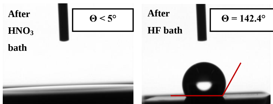
Figure 4-17: Measurement of contact angle on SiNWs after the standard MACE process (after \text{HNO}_3 bath) (left) and after HF post-treatment (right).
