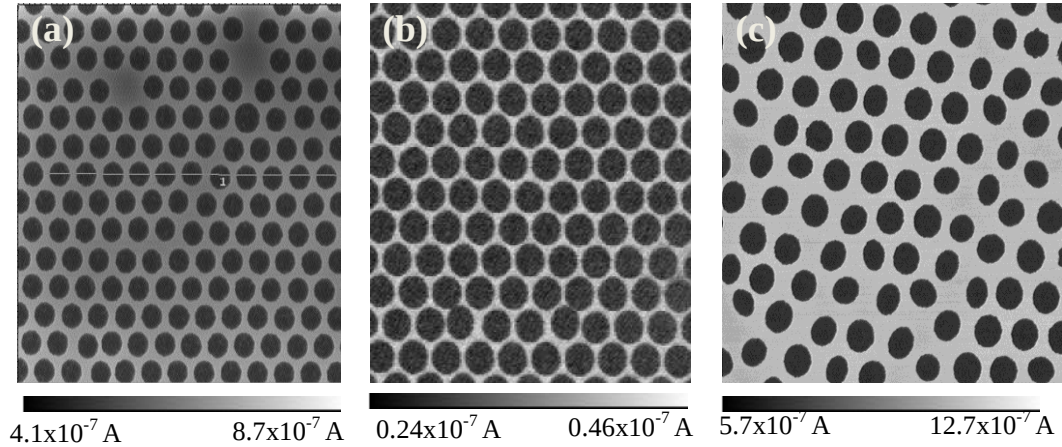
Figure 6-34: Top-view EBIC mapping of ordered SiNWs arrays with a length of (a) 500 nm, (b) 2.2 \mu\text{m} and (c) 3 \mu\text{m} .
