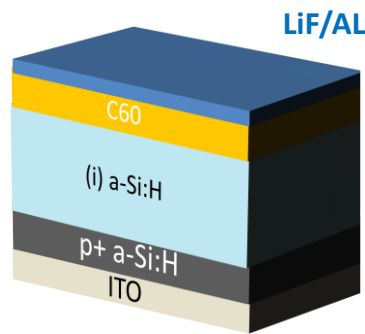
Figure 7-13: Schematic of the hybrid solar cells based on the combination of an organic layer with an amorphous thin film with a LiF/Al rear electrodes.
