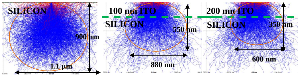
Figure 6-20: Modeling of the volume of excitation produced by a 10 keV electron beam impinging on a 550 \mu\text{m} c-Si substrate with (a) no ITO, (b) 100 nm of ITO and (c) 200 nm of ITO.
