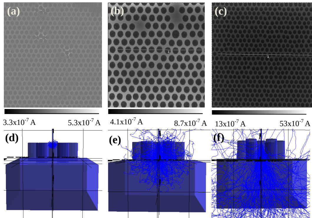
Figure 6-32: Top-view EBIC mapping of ordered SiNWs arrays (pitch of 500 nm, diameter of 280 nm and height of 460 nm) at different gun energies: 3 keV (a), 10 keV (b) and 20 keV (c) with the corresponding modeling (d), (e) and (f).
