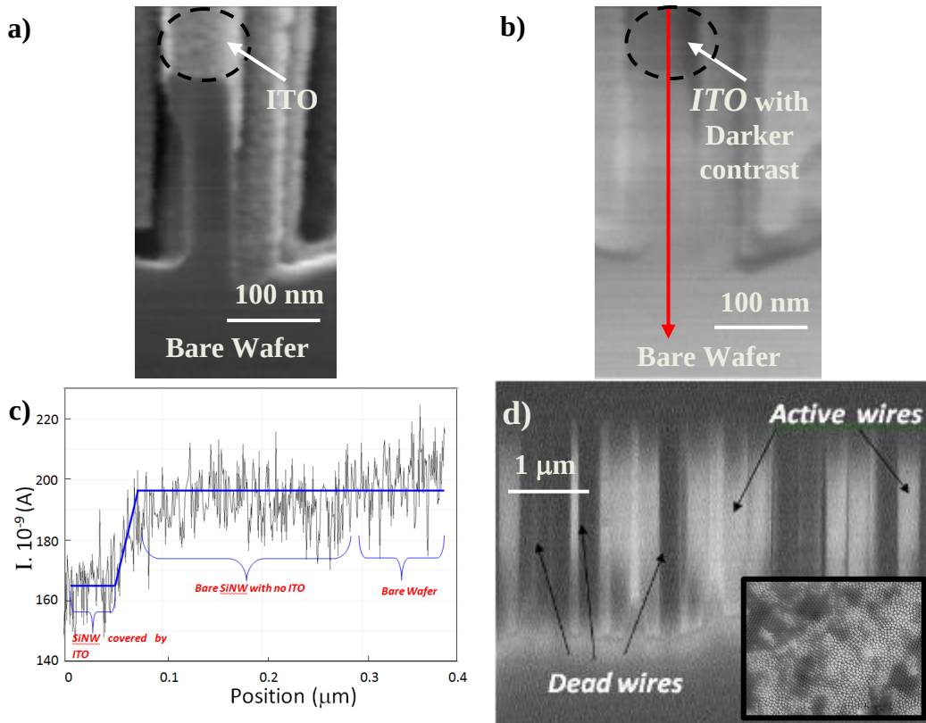
Figure 6-19: (a) Cross-section SEM image of the bottom of a SiNW partially covered by ITO and (b) corresponding EBIC mapping with the red arrow indicating the corresponding signal position on the sample and (c) the corresponding EBIC current profile at 10 keV as a function of the position of the beam on the sample. (d) Cross-section EBIC mapping of samples with “dead” and electrically active SiNWs. The inset shows the EBIC top-view mapping confirming that only few nanowires are active.
