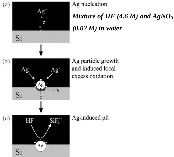
Figure 2-5: Mechanism of formation of SiNW by the MACE process. A silicon substrate is dipped in HF/AgNO 3 solution [61], [62]
