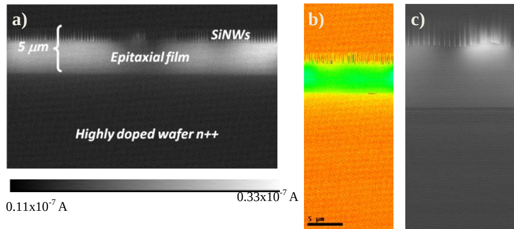
Figure 6-22: EBIC mapping of SiNW solar cells based on 5 \mu\text{m} epitaxial film with low magnification in (a) grey and (b) rainbow magnification and (c) high magnification .
