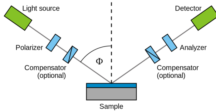
Figure 3-25: Schematics illustrating the working principle of Mueller matrix ellipsometer
