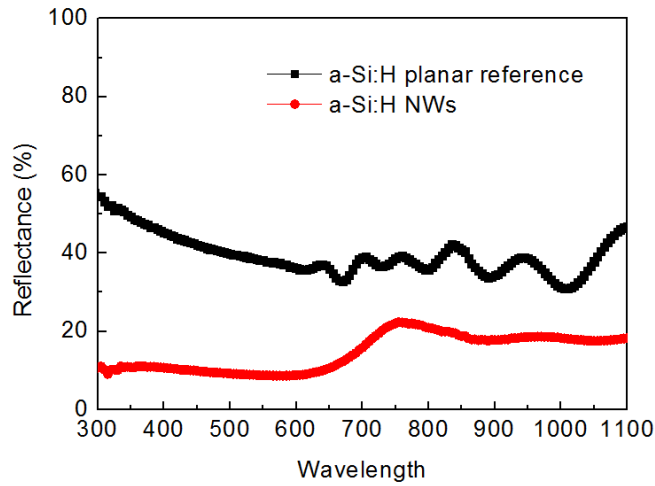
Figure 7-9: Reflectance measurement of planar a-Si:H thin films and a-Si:H nanowires.
