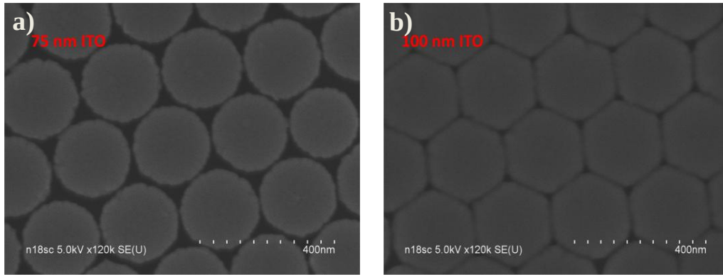
Figure 5-11: Top-view SEM image of ordered arrays of SiNWs with a pitch of 250 nm covered with a thickness of ITO of (a) 75 nm and (b) 100 nm.
