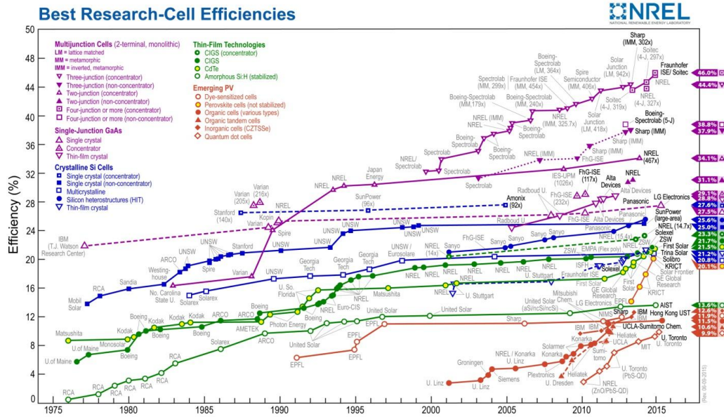
Figure 1-4: Timeline of the best research cell efficiencies for the different PV technologies [19].
