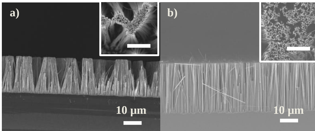
Figure 4-19: Cross-section SEM pictures of 30 \mu\text{m} long nanowires: Effect on the morphology of the SiNWs fabricated by MACE with no post-treatment (a) and after a HF post-treatment (b). The insets show SEM images of the top-view. The scale bar is 5 \mu\text{m} .
