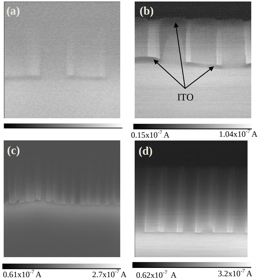
Figure 6-33: Cross-section EBIC mapping of short (a), (b) and long (c), (d) ordered SiNWs arrays at 2 different gun energies: 5 keV (a), (c) and 10 keV (b), (d)
