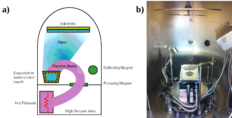
Figure 3-18: (a) Schematics [154] and (b) corresponding photograph of the e-beam evaporator.
