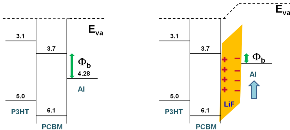
Figure 7-15: Schematic of the vacuum level shift induced by LiF/Al cathode for organic solar cells.
