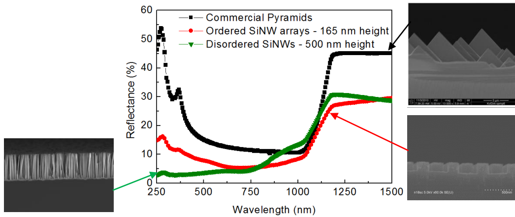
Figure 5-2: Comparison of the total reflectance between commercial pyramids (black curve) and ordered SiNWs arrays of ~165 nm height and pitch of 330 nm (red curve) and disordered SiNWs with a length of 500 nm (green curve) with the corresponding SEM pictures
