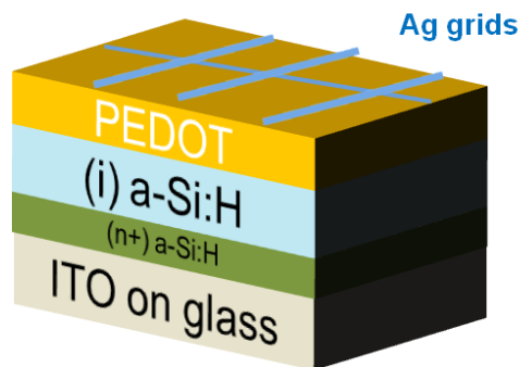
Figure 7-11: Architecture of the device studied – Hybrid thin film solar cells based on a-Si:H.
