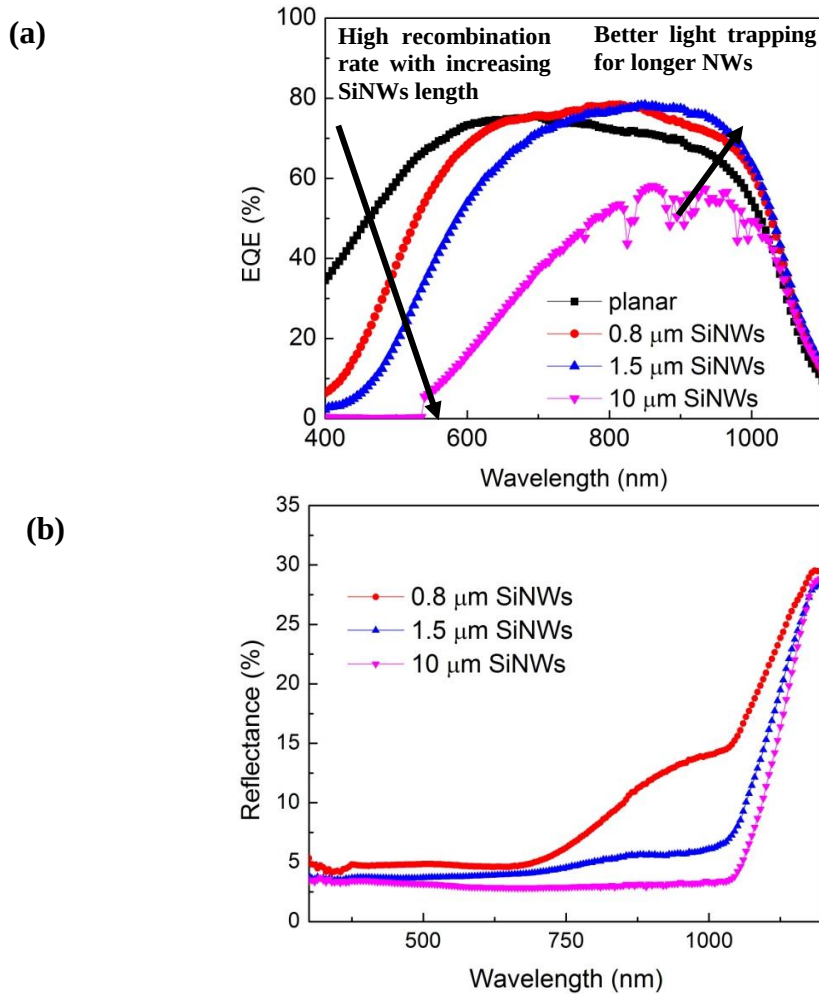
Figure 6-13: Effects of the SiNWs length on the (a) EQE and (b) reflectance of the cells.
