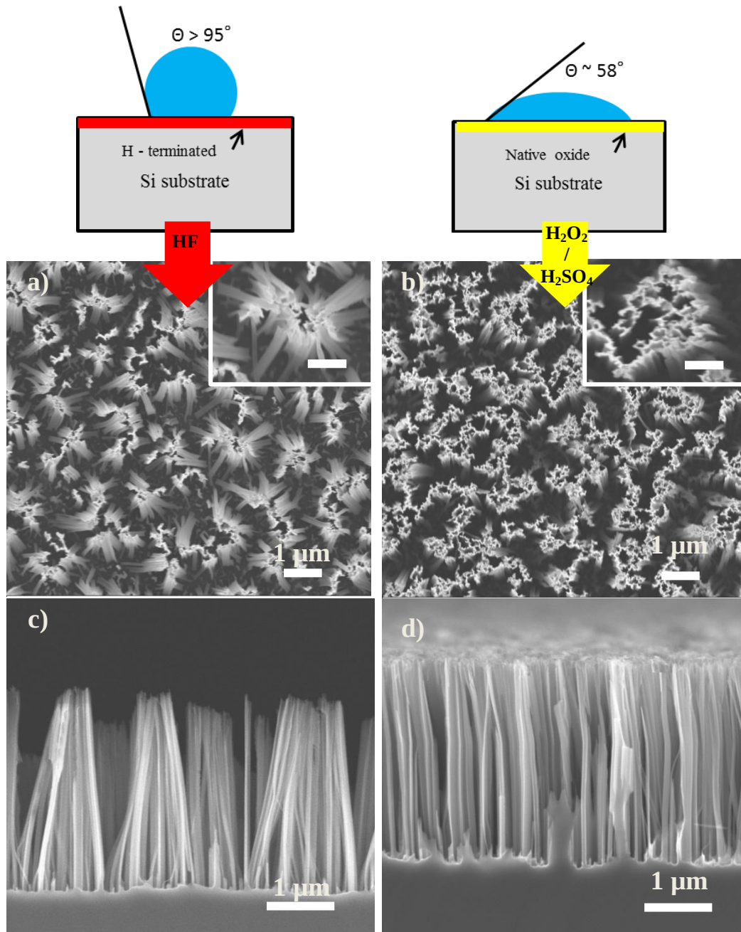
Figure 4-14: Top view (a), (b) and cross-section (c), (d) SEM pictures: Effect on the morphology of the SiNWs fabricated by MACE with a HF pre-treatment (a), (c) and with a \text{H}_2\text{O}_2\text{:H}_2\text{SO}_4 pre-treatment (b), (d). The insets show high magnification SEM images of the top-view. The scale bar is 500 nm.
