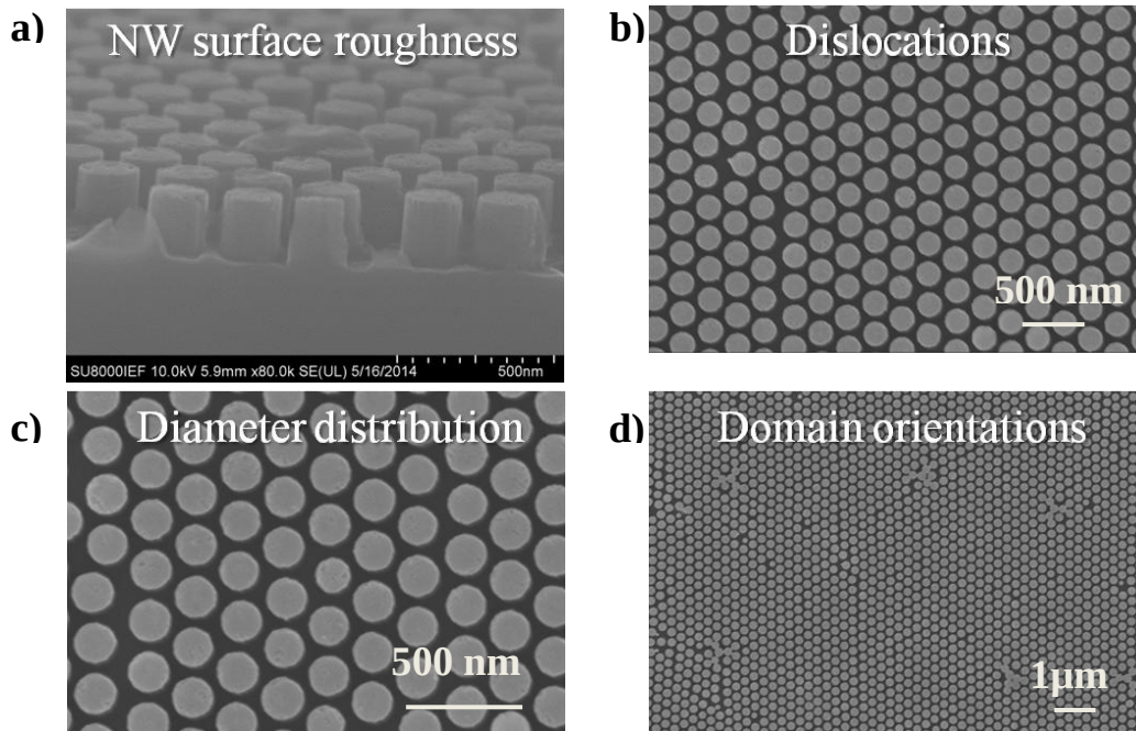
Figure 5-18: Structural imperfections of ordered array of SiNWs fabricated by MACE assisted by NSL such as (a) surface roughness, (b) dislocations, (c) diameter distribution and (d) domain orientations.
