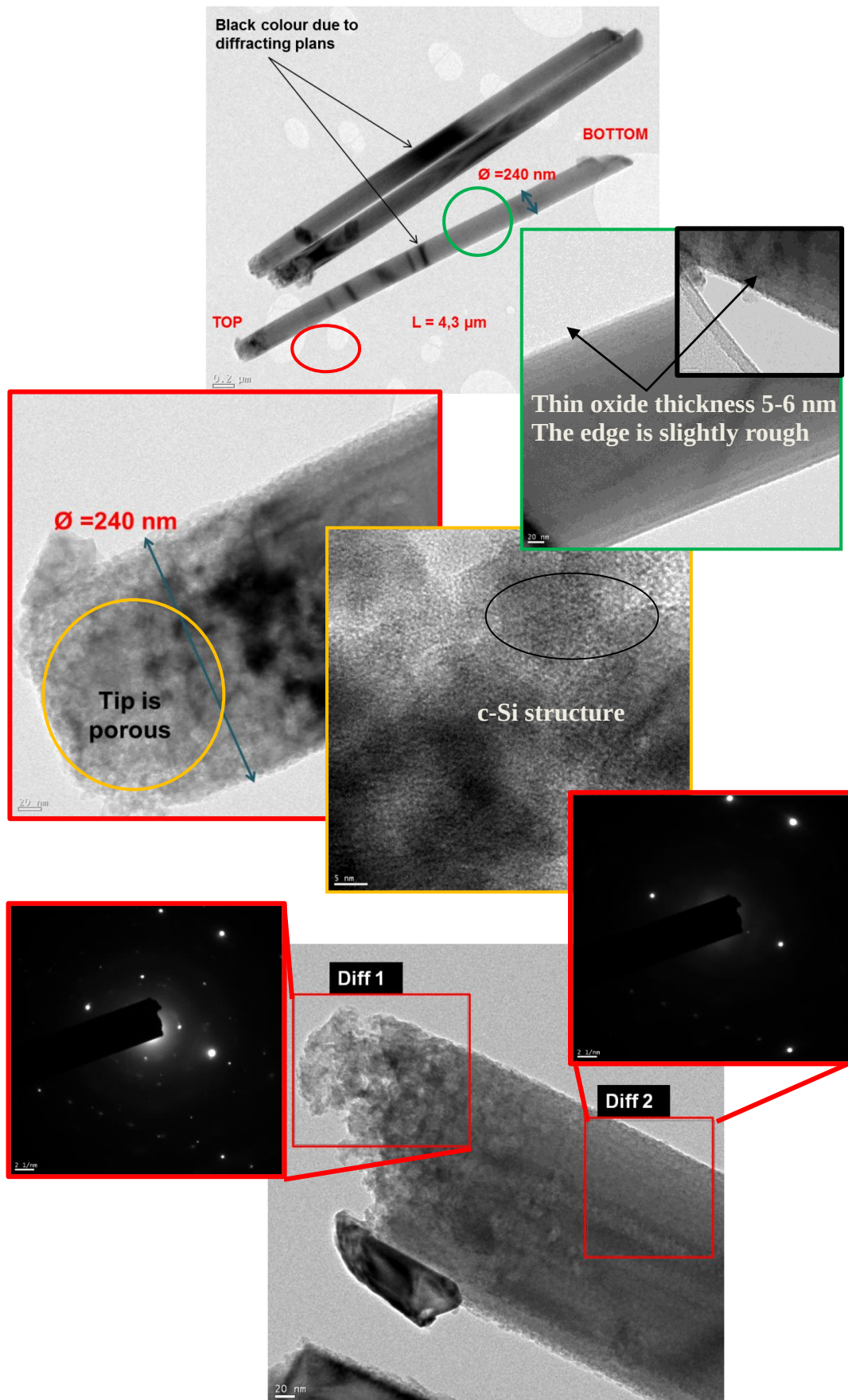
Figure 6-30: TEM analysis of ordered SiNW before a-Si:H coating.
