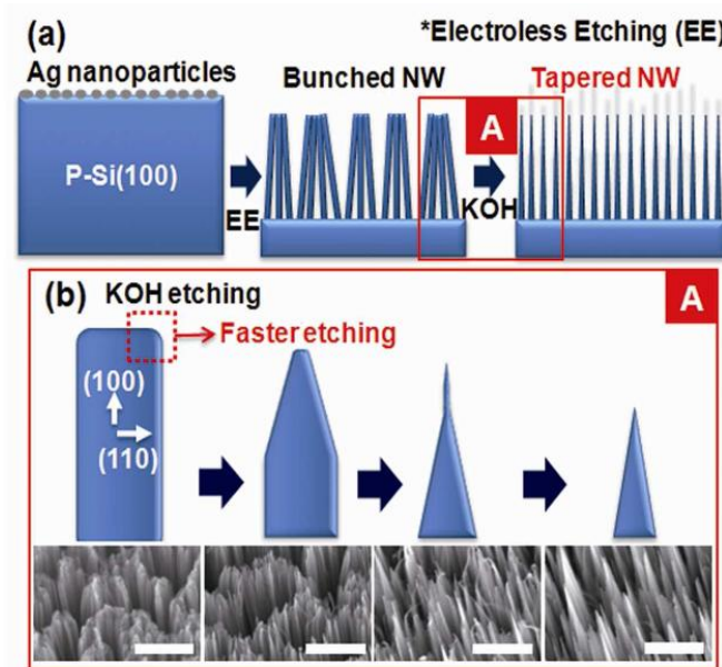
Figure 4-6: (a) Schematic detailing the fabrication process of agglomerated and tapered SiNWs. (b) Schematic showing the effect of KOH post-etching treatment to taper the top-ends of SiNWs [186], [193]
