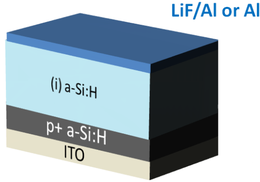
Figure 7-16: Schematic of the structure of the LiF/Al rear electrodes on (p+) a-SiC:H/(i) a-Si:H.
