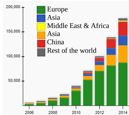
Figure 1-1: Global and regional cumulative capacity in Megawatt (MW) [4].
