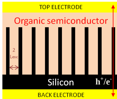
Figure 2-14: Schematic representation of an ideal nanostructure hybrid silicon/organic material solar cell. The nanowires offer a continuous conductive path to the electrode. L_{exc} is the diffusion length of the exciton. The nanowires are separated by a distance of about 2L_{exc} in order to reduce loss in photocurrent due to exciton recombination.
