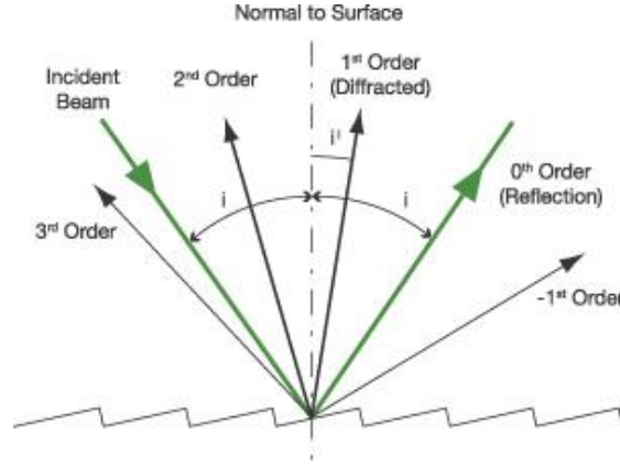
Figure 5-12: Illustration of a diffraction pattern from a periodic diffraction grating [222]
