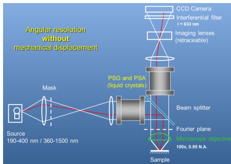
Figure 3-26: Schematics showing the working principle of the Angle-resolved MM polarimeter [179].
