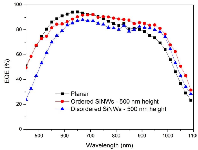
Figure 6-26: Comparison of EQE response for different C-Si substrates: reference planar cells, ordered SiNW arrays cells, disordered SiNW arrays cells.
