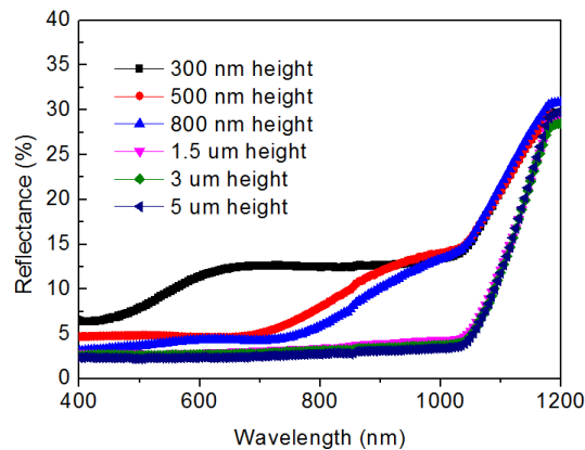
Figure 5-3: Effect of disordered SiNW length on the measured total reflectance plotted as a function of the wavelength.
