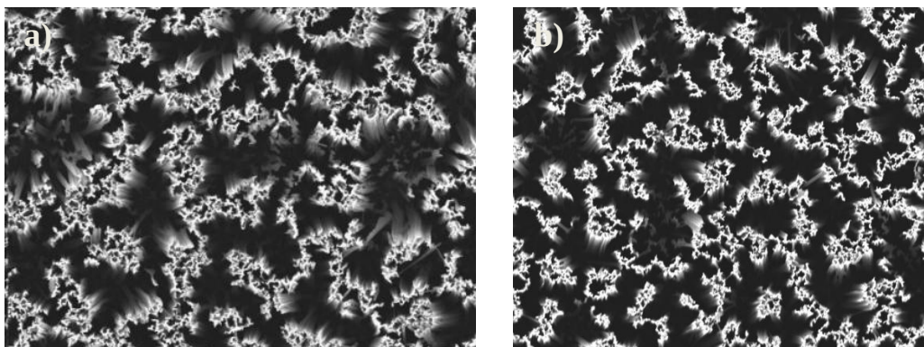
Figure 4-9: SEM pictures of SiNWs arrays (a) before and (b) after the replacement of solvent.
