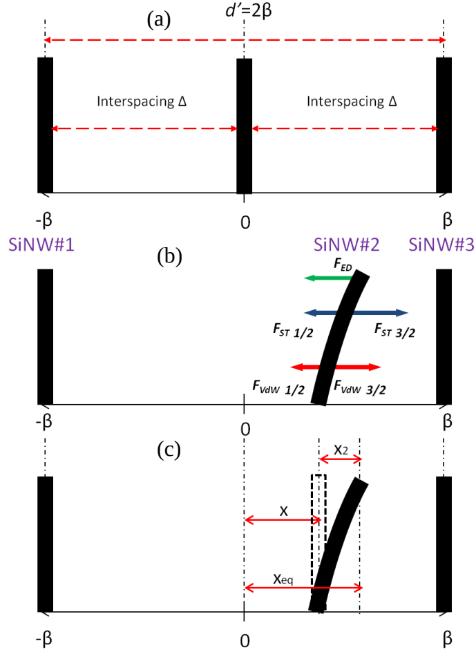
Figure 4-3: Schematic model of an array composed of three 2 \mu\text{m} long-nanowires labeled 1, 2 and 3. Definition of the original geometry- the ideal case (a). Definition of the forces: F_{X/Y} is the force exerted by SiNW #X on SiNW #Y (b). Definition of the equilibrium position before (nanowire in dotted lines) and after bending (c).
