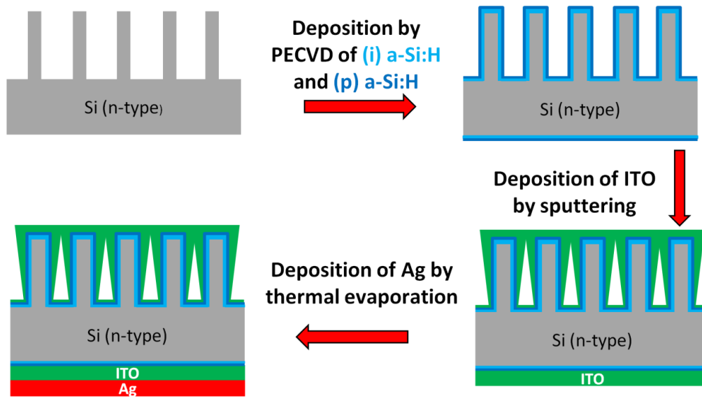
Figure 6-4: Process of fabrication of HIT solar cells based on SiNWs.
