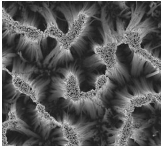
Figure 2-6: SEM picture of 10 \mu\text{m} SiNWs fabricated by MACE showing the strong agglomeration at the top-end of the SiNWs
