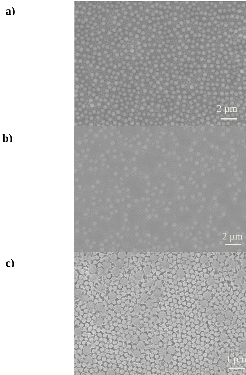
Figure 5-23: Top-view SEM pictures of PS spheres monolayer with a PS sphere (330:600 nm) ratio of (a) (1:2), (b) (2:1) and (c) corresponding SiNW arrays fabricated from (b).
