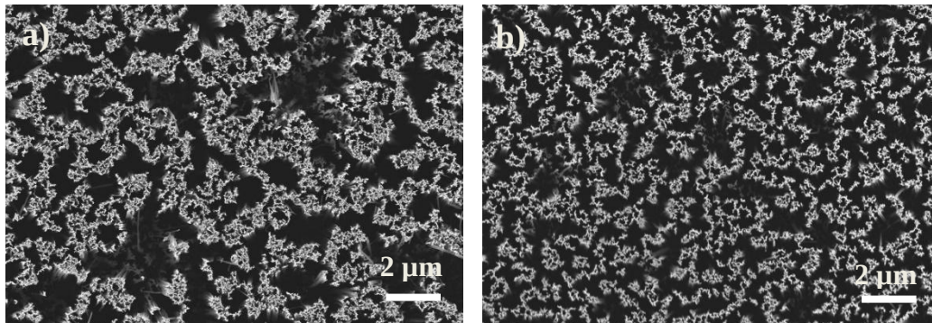
Figure 4-13: SiNWs array (a) before and (b) after CO 2 supercritical drying process.
