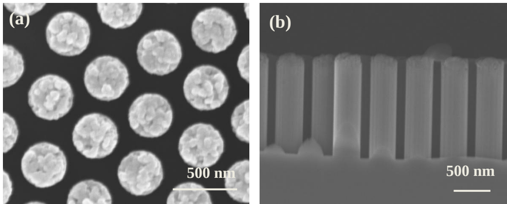
Figure 6-24: SEM picture of ordered arrays of SiNWs (pitch 550 nm, diameter of 345 nm , length of 1.2 \mu\text{m} ) after a-Si:H deposition and before ITO deposition (a) top-view (b) cross-section
