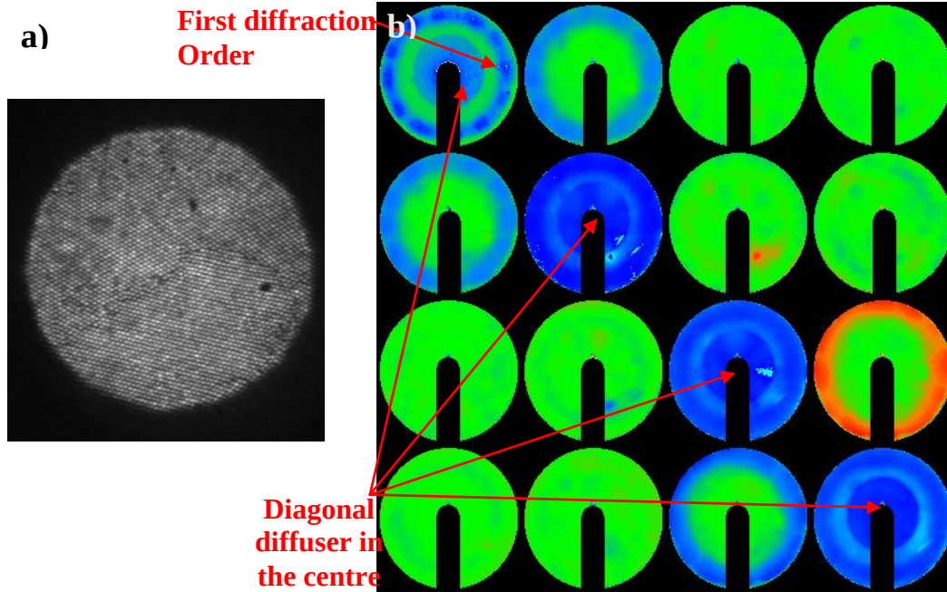
Figure 5-14: (a) Real space (microscopic) image and (b) corresponding measured normalized Mueller matrices of ordered SiNW arrays with a pitch of 800 nm.
