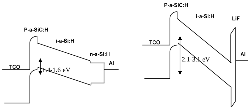
Figure 7-19: Schematic of the band diagram of p-i-n junction and a-Si:H thin film with a LiF/Al rear electrodes.
