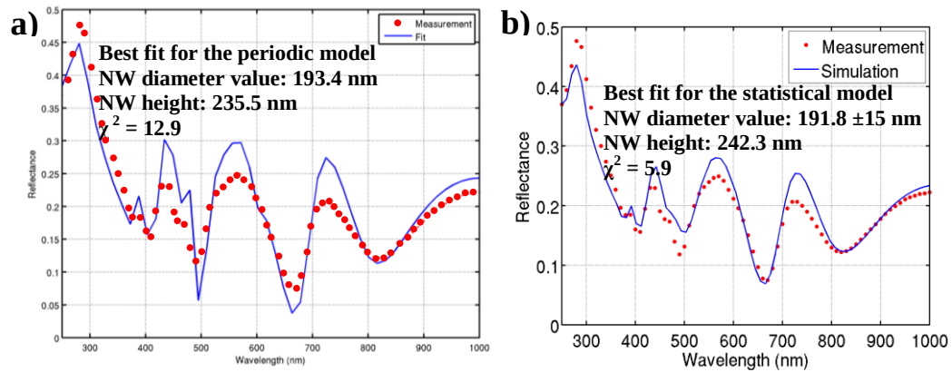
Figure 5-20: Comparison between (a) the "periodic model and (b) the "statistical model" for modeling a short periodic array fabricated by MACE assisted by NSL.
