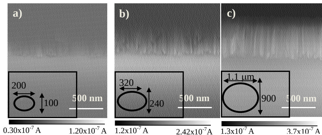
Figure 6-16: : EBIC mapping of the HIT SiNW cross-section under various accelerating voltages (a) 3 keV, (b) 5 keV and (c) 10 keV.
