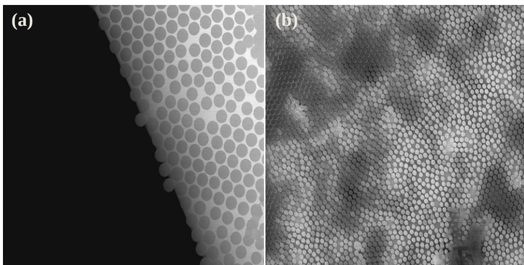
Figure 6-39: Top-view EBIC mapping before (a) and after (b) oxidation pre-treatment.
