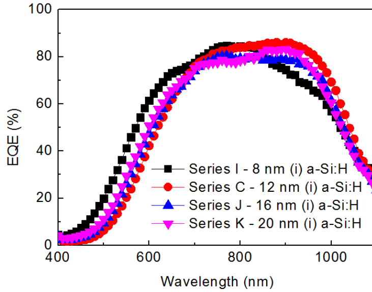
Figure 6-12: Effect of the (i) a-Si:H thickness on the EQE of HIT solar cells based on SiNWs.
