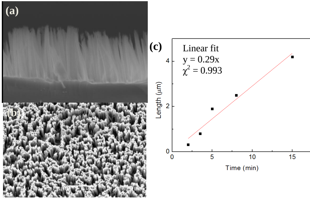
Figure 7-8: (a) Cross section view of a-Si:H nanowires. (b) Top-view of a-Si:H nanowires. (c) Length of nanowires as a function of the etching time.
