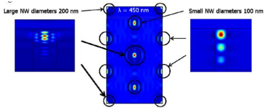
Figure 5-22: Representation of the dual diameter SiNW arrays concept with the corresponding Poynting vector at a wavelength of 450 nm. Every black circle represent a nanowire [37], [38].
