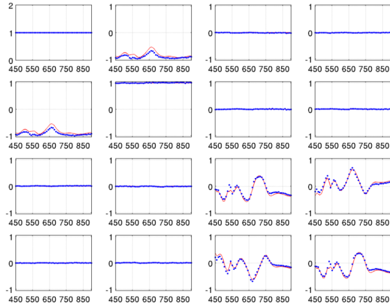
Figure 5-21: Best fit of Mueller Matrix using the statistical model.
