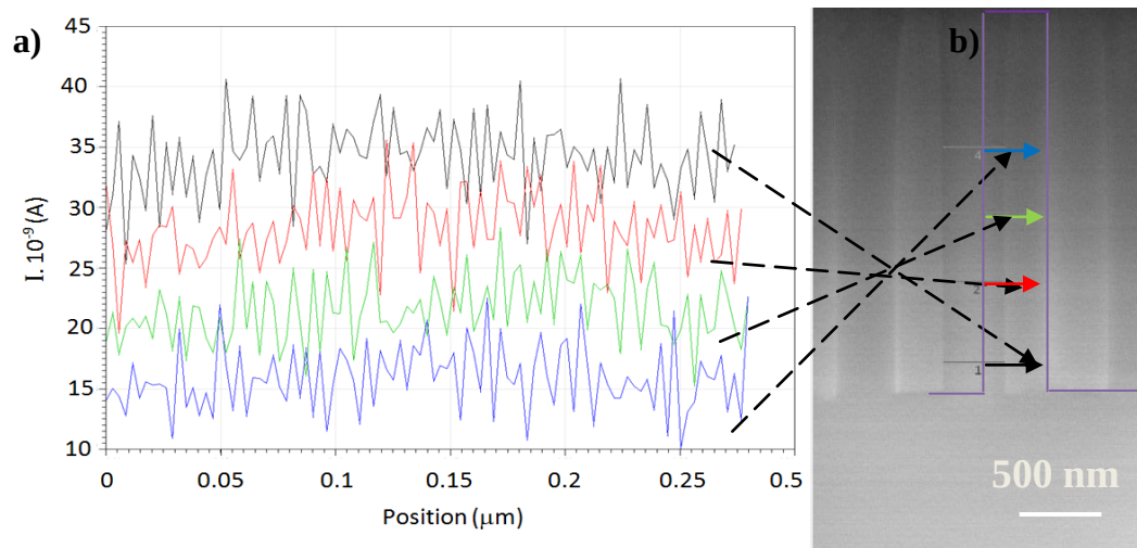
Figure 6-21: EBIC current profiles (a) and cross-section EBIC current mapping (b). The 4 different arrows indicate the localization of the different EBIC profiles measured on the sample.
