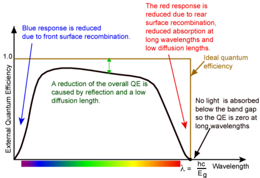
Figure 3-21: The ideal and typical EQE response of a silicon solar cell from www.pveducation.org .
