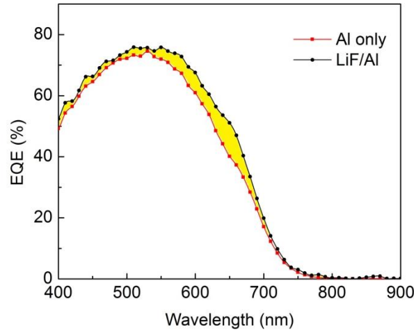
Figure 7-18: EQE curves of the thin film devices with LiF/Al cathode (black) and Al cathode (red)
