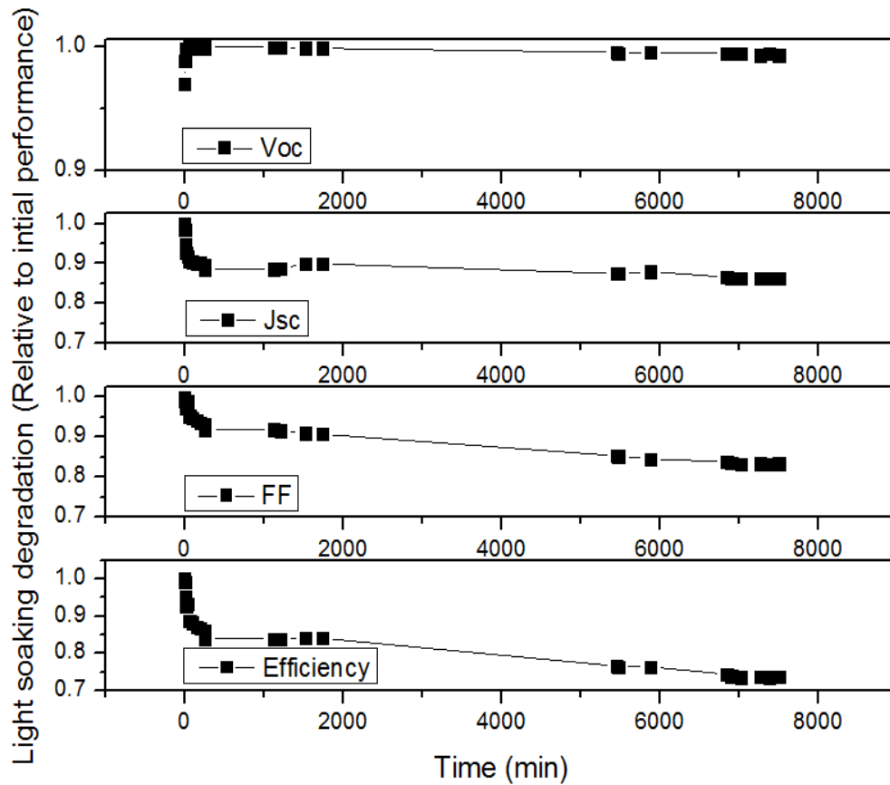
Figure 7-21: Light soaking effect on the cells' performances.
