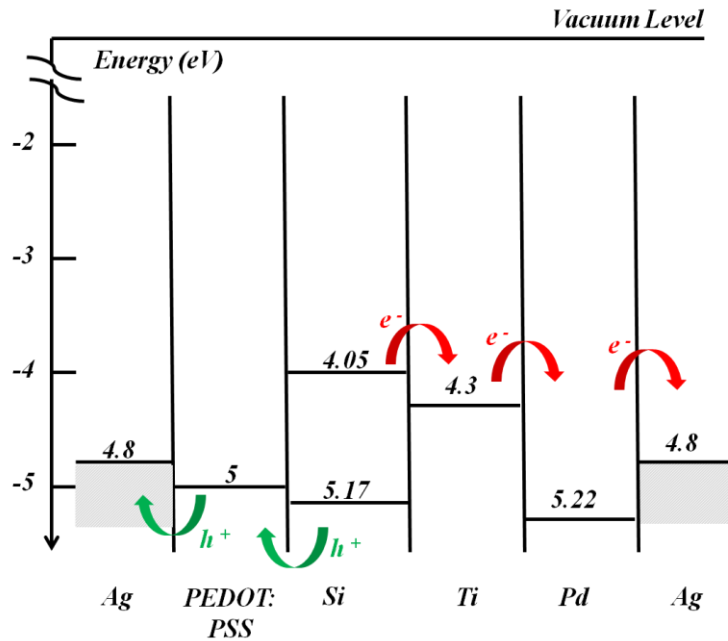
Figure 7-5: Band diagram of the hybrid device
