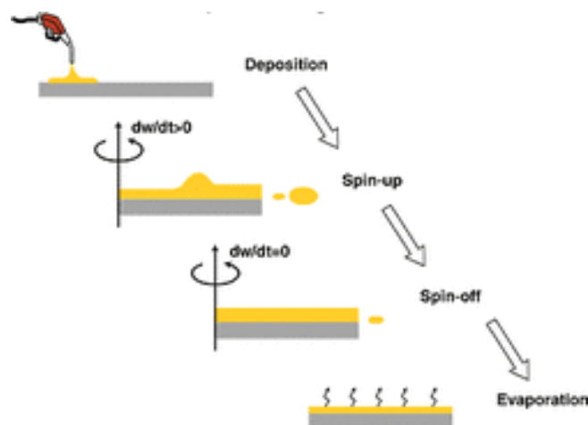
Figure 3-20: Schematics illustrating the key steps of the spin coating technique [156].
