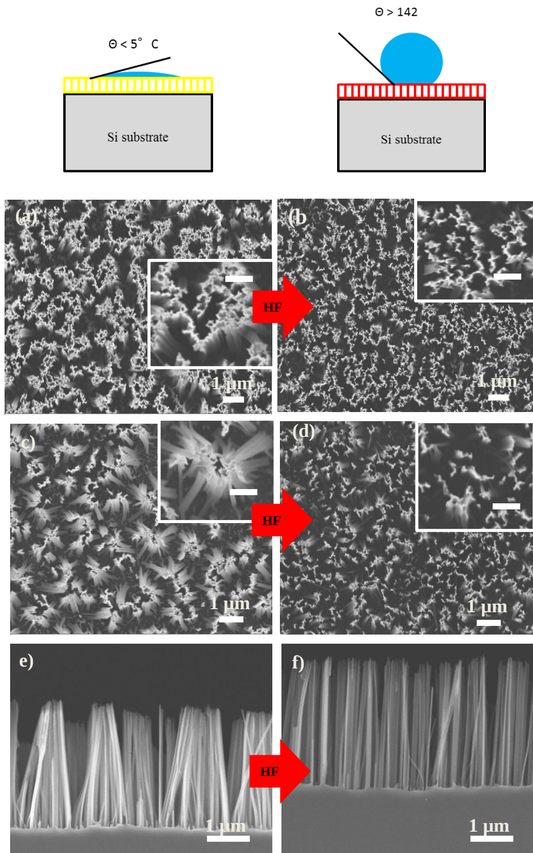
Figure 4-16: SEM pictures - Effect on the morphology of the SiNWs fabricated by MACE after a \text{H}_2\text{O}_2:\text{H}_2\text{SO}_4 pre-treatment (a), after a \text{H}_2\text{O}_2:\text{H}_2\text{SO}_4 pre-treatment and a HF post-treatment (b), after a HF pre-treatment (c), (e), and after a HF pre-treatment and a HF post-treatment (d), (f). The insets show high magnification SEM images of the top-view. The scale bar is 500 nm.
