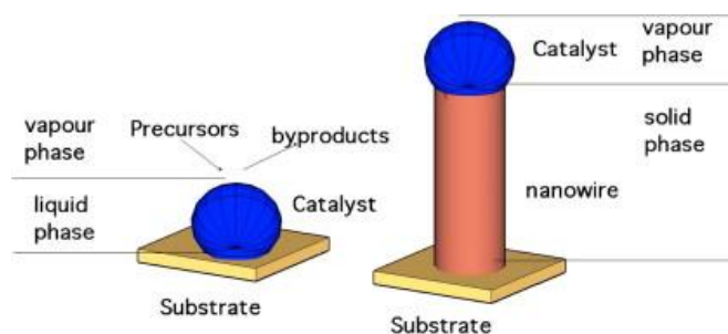
Figure 2-4: Scheme of the VLS Vapor Liquid Solid process [54].
