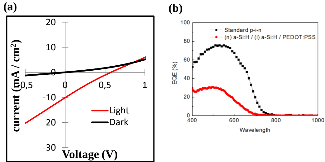
Figure 7-12: (a) (J,V) and (b) EQE planar hybrid a-Si:H / PEDOT:PSS heterojunction
