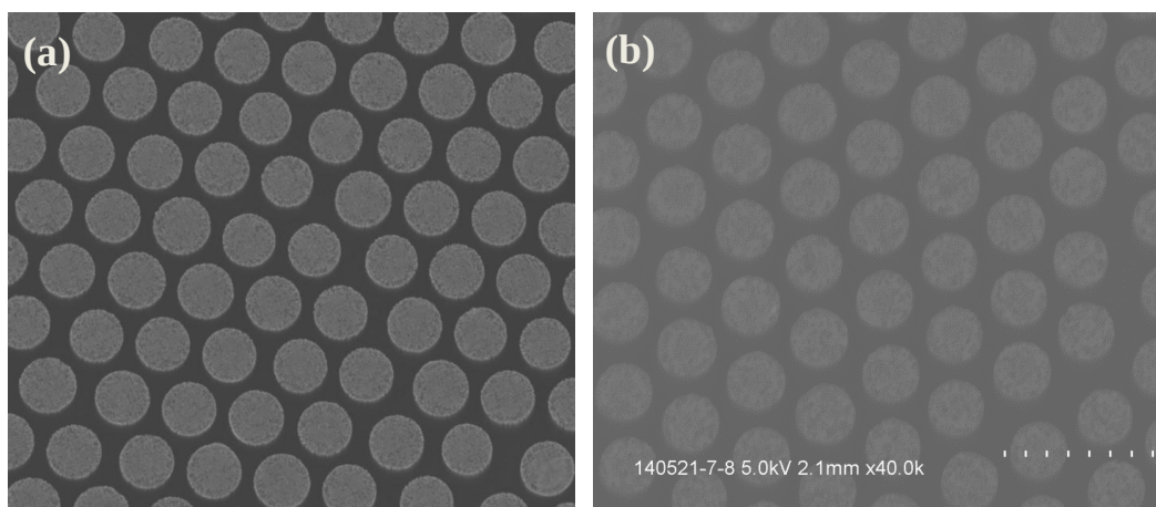
Figure 6-37: Top-view SEM picture of ordered arrays of SiNWs (pitch 800 nm, length of 2.7 \mu m ) before (a) and after (b) oxidation process.
