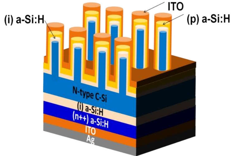
Figure 2-13: Schematic of a HIT structure based on SiNWs. The n-type c-Si wafer has been nanostructured to improve light trapping
