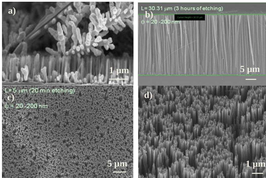
Figure 3-2: (a) SEM picture of silver dendrites covering the SiNW prior the \text{HNO}_3 chemical bath [142], (b) cross-section SEM picture of 30 \mu\text{m} long random SiNWs, (c) inclined ( 15^\circ ) SEM picture of 5 \mu\text{m} long random SiNWs, and (d) inclined ( 30^\circ ) SEM picture of 5 \mu\text{m} long SiNWs.
