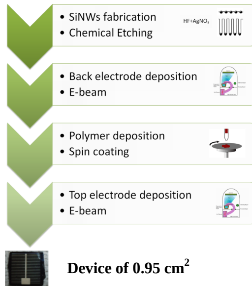
Figure 7-2: Process flow of hybrid solar cells
