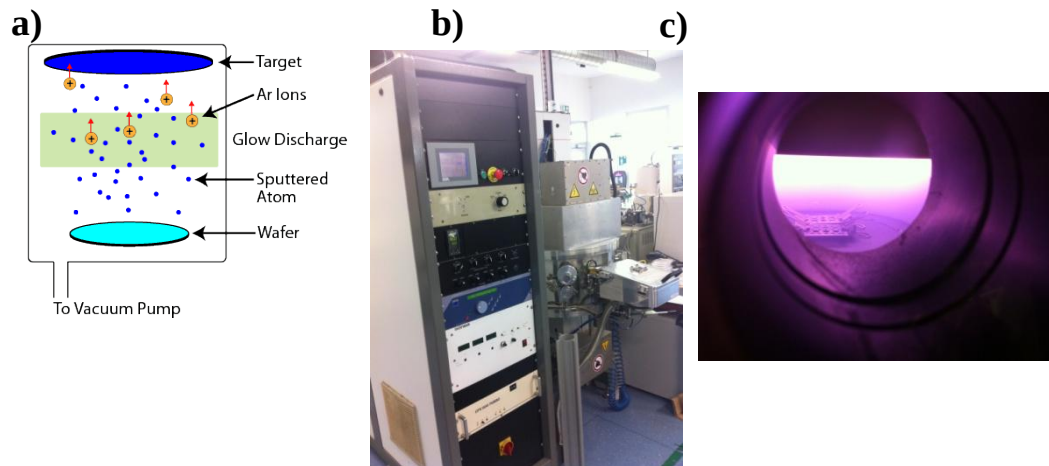
Figure 3-19: (a) Schematics [155] and (b) photograph of the sputtering system. (c) O 2 :Ar plasma during the ITO deposition.
