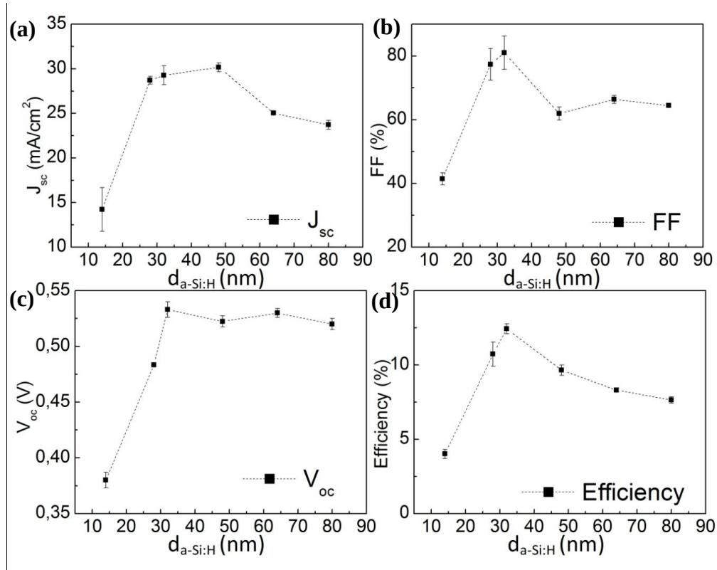
Figure 6-6: The average value and the standard deviation of J_{sc} (a), FF (b), V_{oc} (c) and \eta (d) as function of d_{a-Si:H} .
