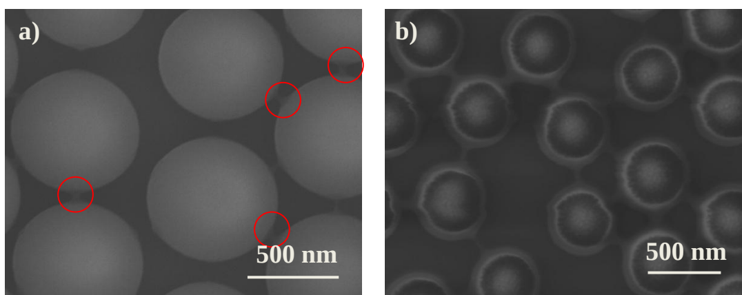
Figure 3-9: SEM picture of (a) slightly annealed PS spheres. The red circles shows the small area melted. (b) Overheated PS spheres causing the excessive melting of the colloidal particles.
