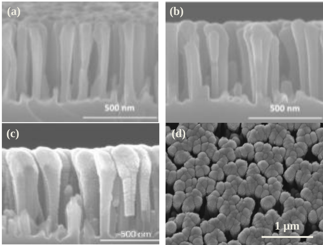
Figure 6-7: SEM pictures of SiNW solar cells after a-Si:H PECVD deposition of sample D (a) and sample F (b) before ITO deposition and sample F (c) after ITO deposition cross-section and (d) after ITO deposition top-view.
