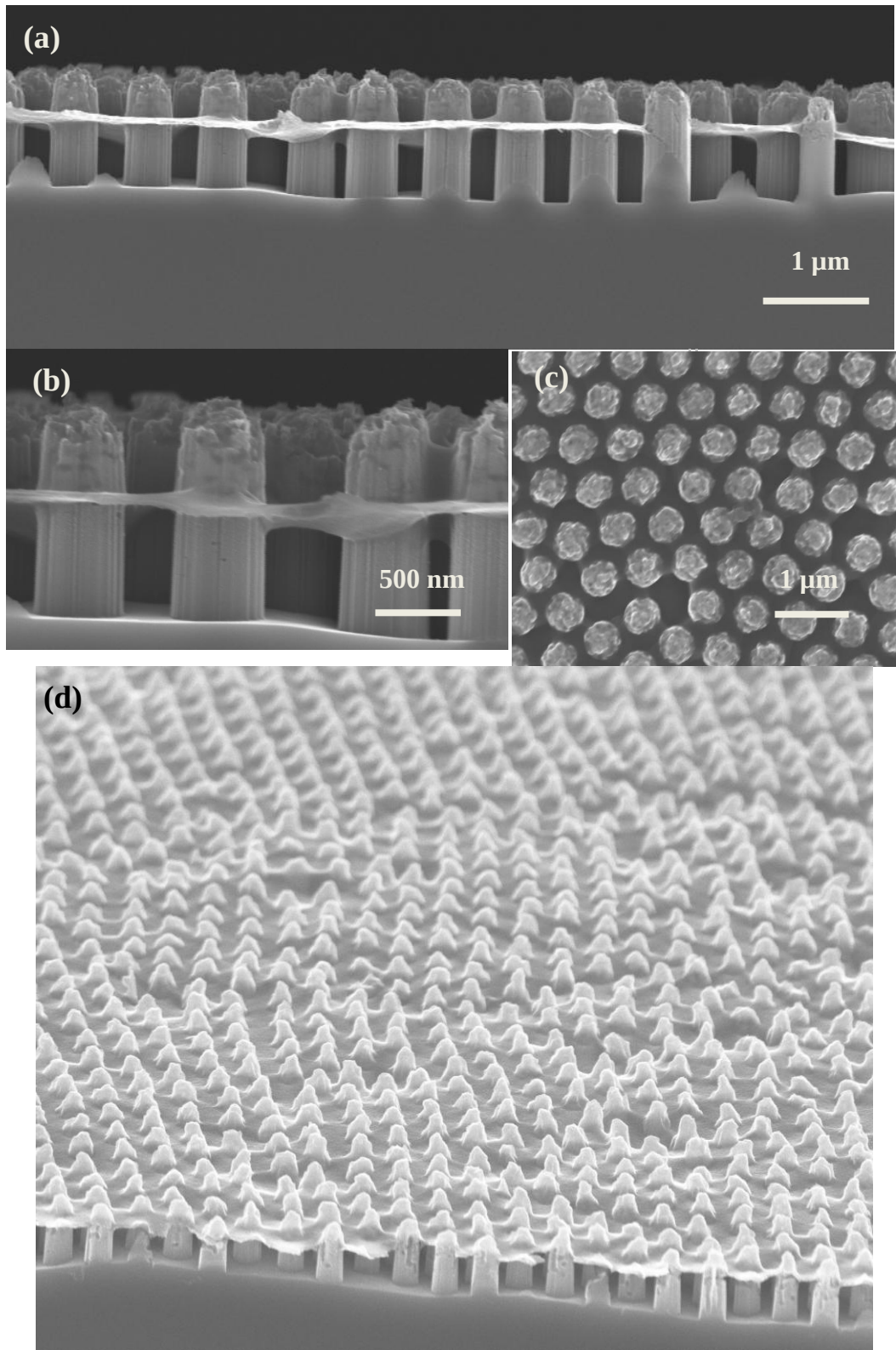
Figure 7-6: Cross-section view (a), (b), Top-view (c) and Inclined-view (d) SEM pictures of SiNWs coated with PEDOT:PSS
