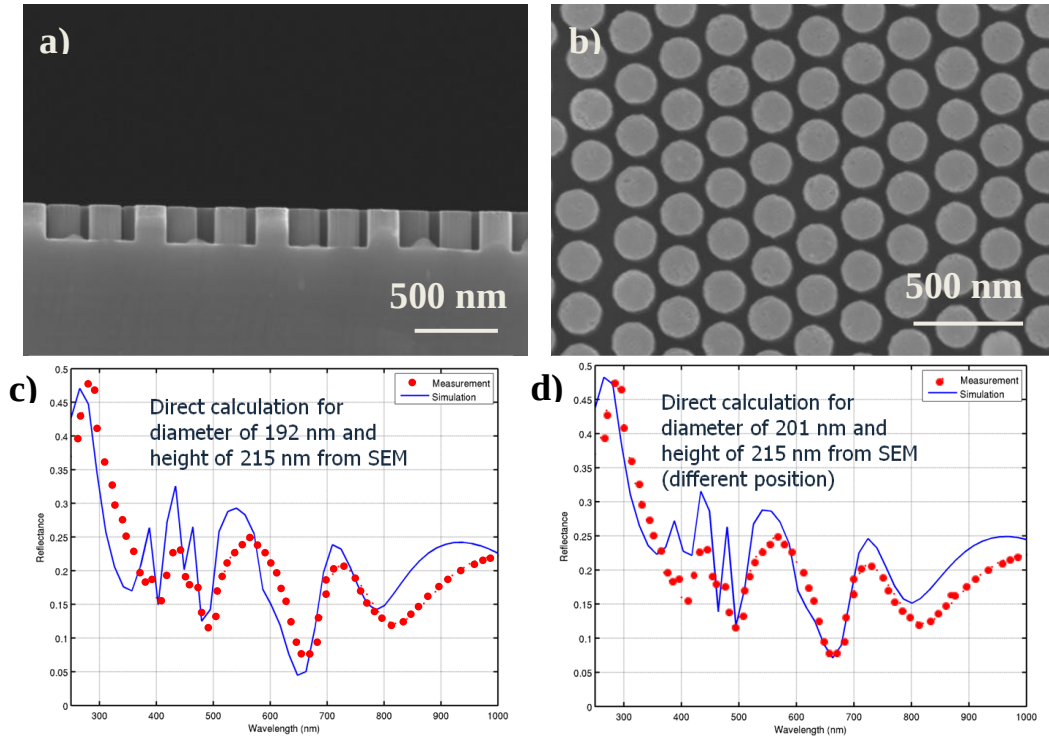
Figure 5-19: (a) Cross-section and (b) top-view SEM image of short ordered arrays of SiNWs and corresponding modeling (c), (d) using the "periodic model".
