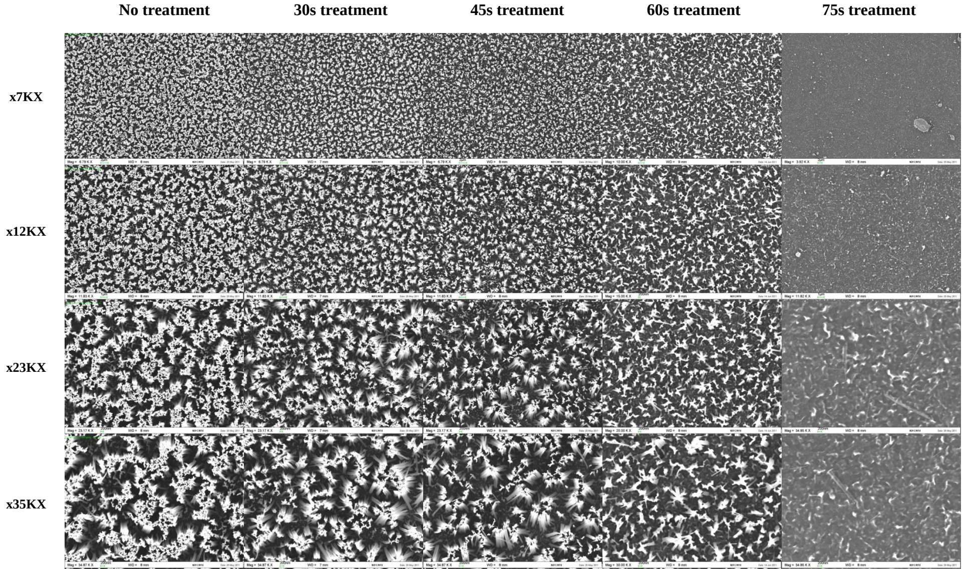
Figure 4-10: Effect of KOH post-treatment on the morphology of SiNWs for different time of treatment and for different magnification.
