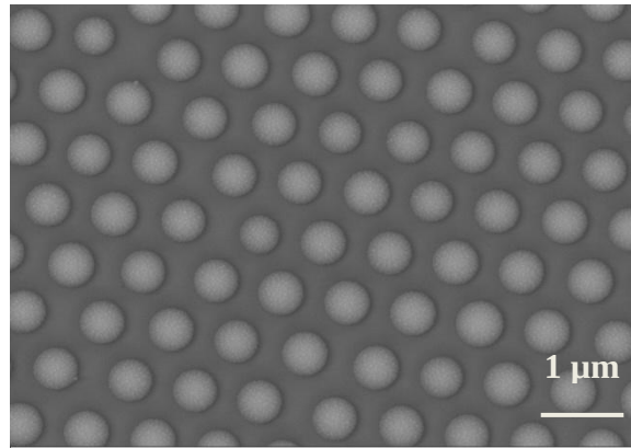
Figure 3-11: SEM picture of the PS spheres arrays after 130s of oxygen plasma treatment. The PS spheres are separated from each other. The initial diameter of PS spheres of 600 nm was reduced down to 392 nm.
