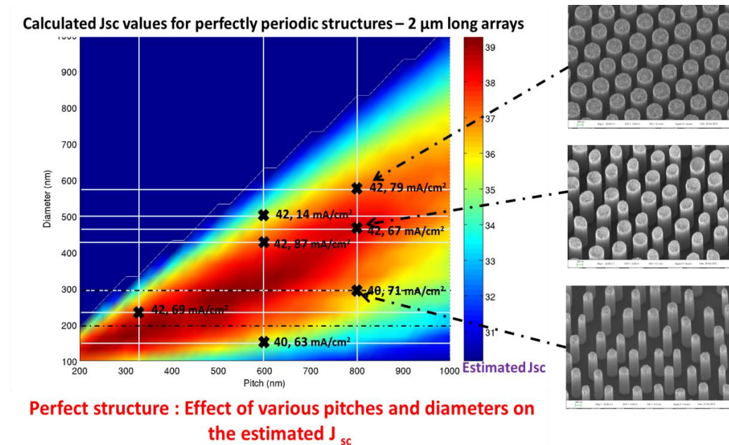
Figure 5-17: Effect of the geometrical parameters (pitch and length) on the estimated J_{sc} for a perfect periodic structure.
