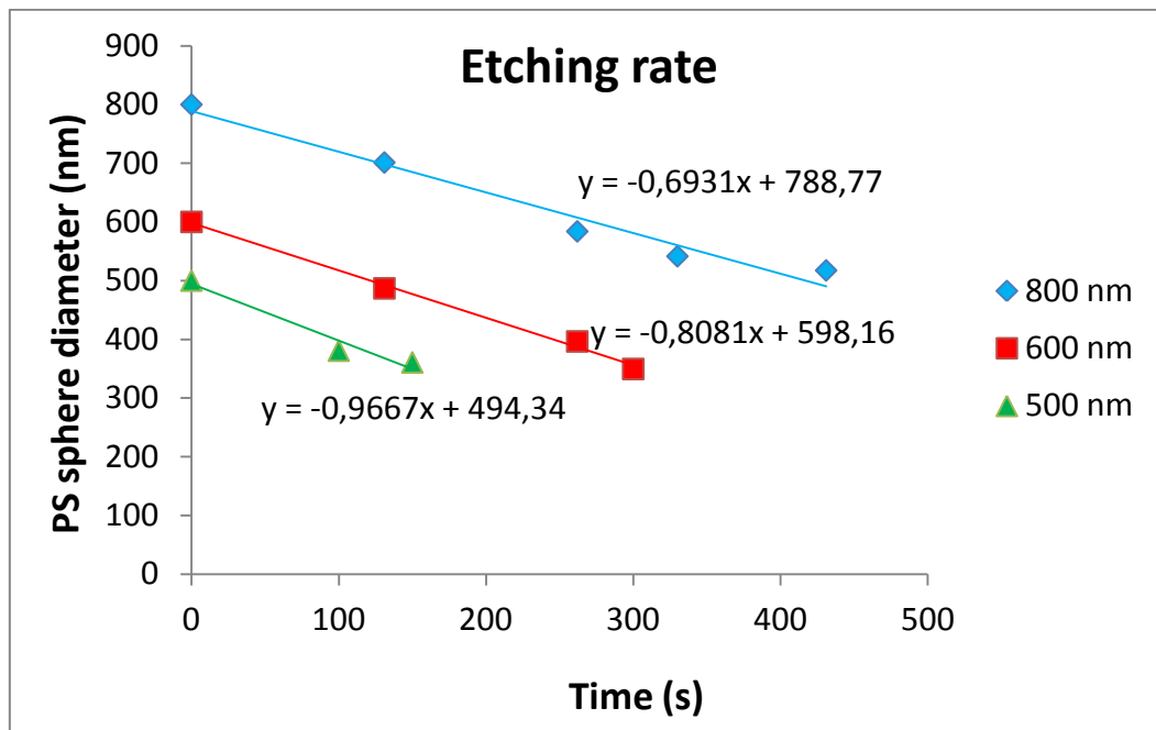
Figure 3-10: The etch rate of the PS spheres with initial nominal diameter of 500 nm, 600 nm and 800 nm by oxygen plasma as a function of time.
