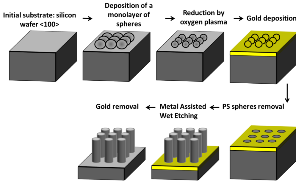
Figure 3-3: Schematics of the nanosphere lithography method coupled with the MACE process
