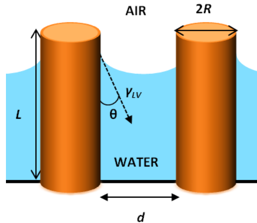
Figure 4-1: Schematic representation of two cylinders of the same length L and radii R , separated by a distance d and partially immersed in a liquid. Once the water level falls below the tip of the cylinders during the drying process, the surface tension of the liquid/vapor interface \gamma_{LV} induces a small curvature of the solvent to reduce the active surface area
