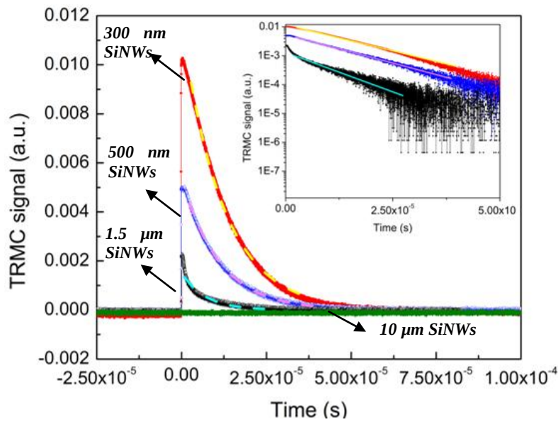
Figure 6-14: TRMC signal as a function of time for samples with different SiNW lengths.
