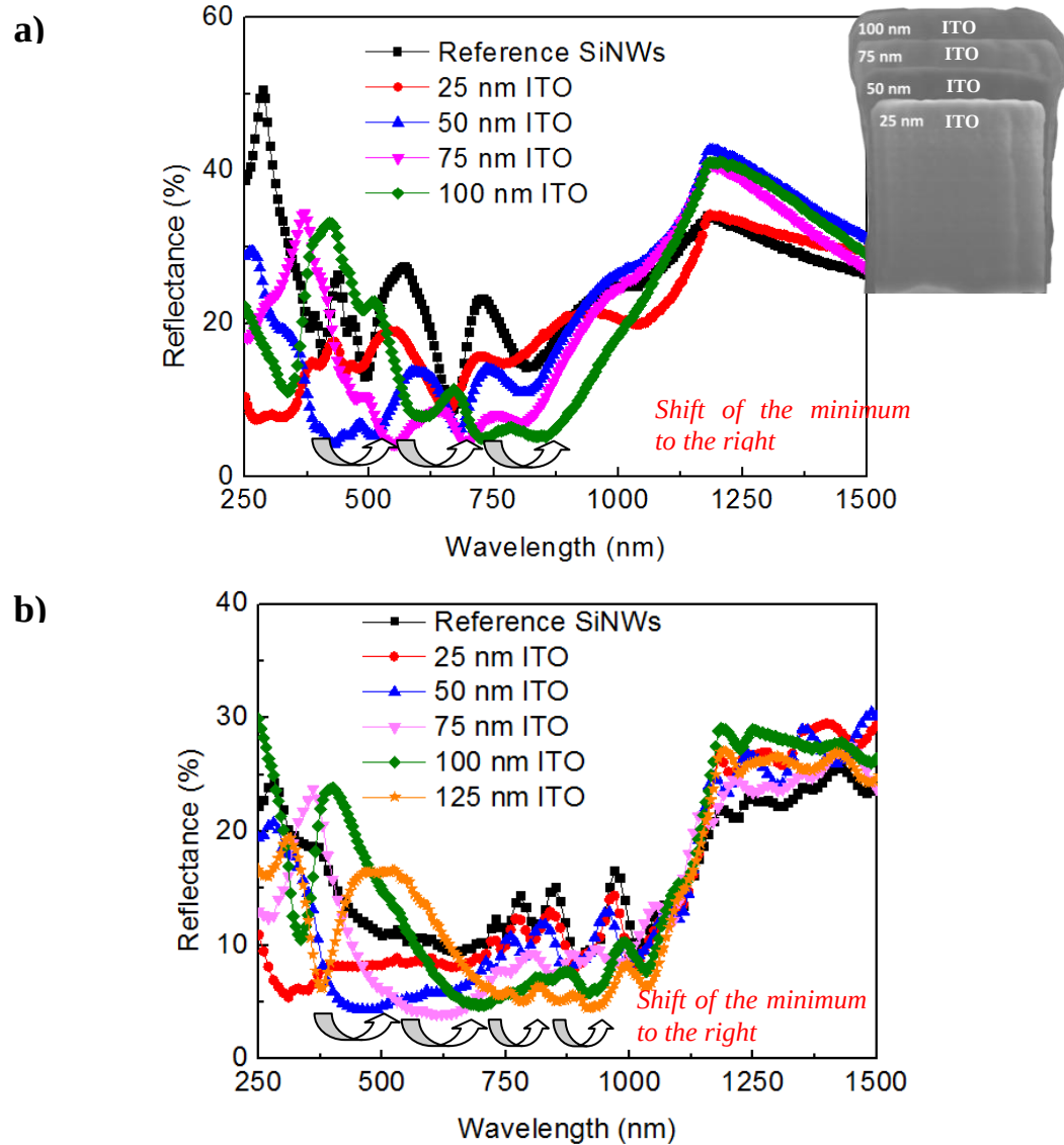
Figure 5-10: Effect of increasing the thickness of ITO on the reflectance of ordered SiNW arrays with a pitch of (a) 250 nm and (b) 500 nm.
