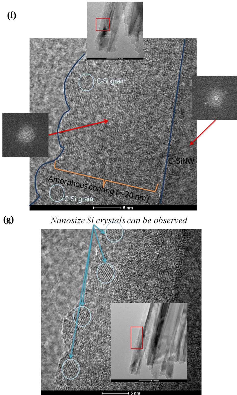
Figure 6-15: TEM analysis of disordered SiNWs. SiNWs agglomerate (a) and (b). Only the tip of the wire is covered by a-Si:H and the coating depth by a-Si:H is between 370- 500 nm (c), (d) and (e). Small crystal grains can be found within the amorphous coating (f) and (g).
