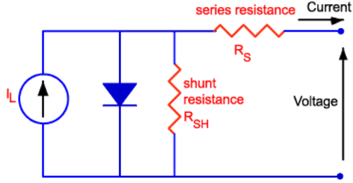
Figure 2-2: Equivalent circuit model of a solar cell [39].
