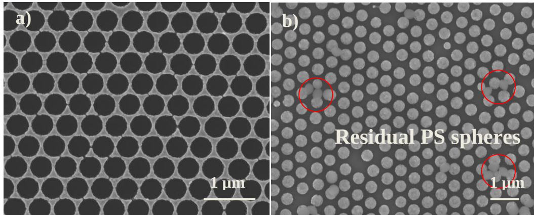
Figure 3-13: (a) SEM pictures of the gold etching mask after the removal of the PS spheres. (b) SEM pictures of SiNWs arrays where the removal stage of PS spheres has been carried out at the last step of the process. The PS spheres are not effectively removed since they are trapped inside the nanostructure.
