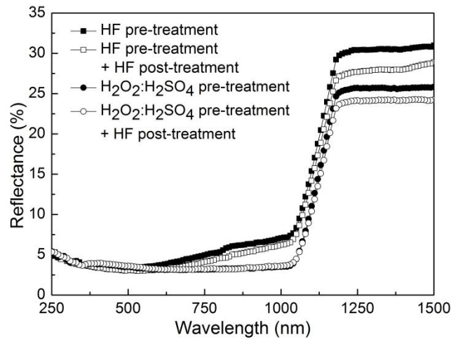
Figure 4-15: Reflectance of the SiNW arrays fabricated by MACE with a HF pre-treatment (solid black squares), a \text{H}_2\text{O}_2\text{:H}_2\text{SO}_4 pre-treatment (black solid circles) a HF pre-treatment and a HF post-treatment (open squares), and after a \text{H}_2\text{O}_2\text{:H}_2\text{SO}_4 pre-treatment and HF post treatment (open circles).
