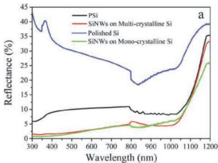
Figure 2-7: Reflectance measurement of porous (PSi), polished c-Si and SiNW arrays [26], [27].
