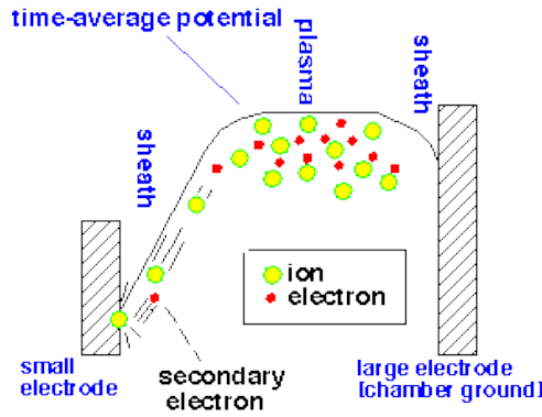
Figure 3-15: Schematics illustrating the voltage distribution of a plasma in the case of asymmetric electrodes [148].
