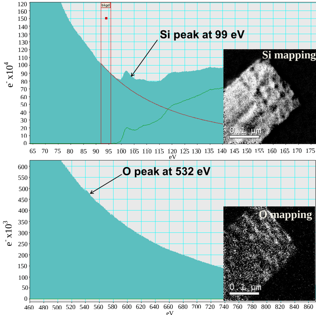
Figure 6-29: EELS analysis of ordered SiNW arrays.
