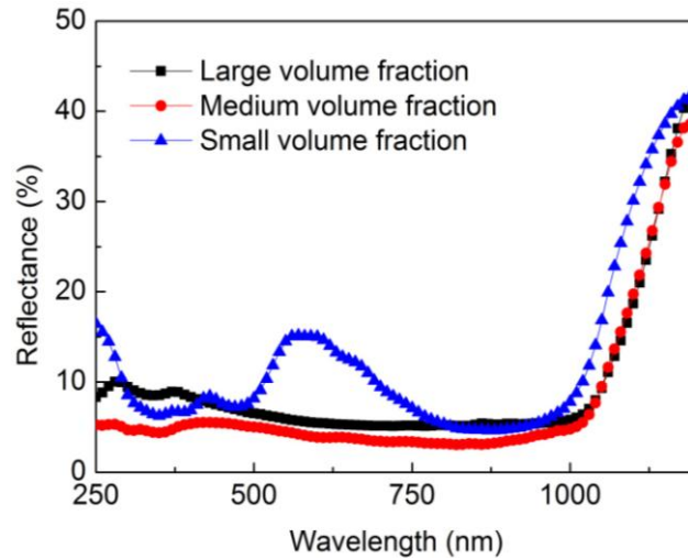
Figure 5-8: Effect of the volume fraction on the reflectance of three ordered arrays of SiNWs with a pitch of 600 nm and a length of 2 \mu\text{m} . The diameters for the high, medium and low density SiNW arrays are 503 nm, 436 nm and 158 nm.
