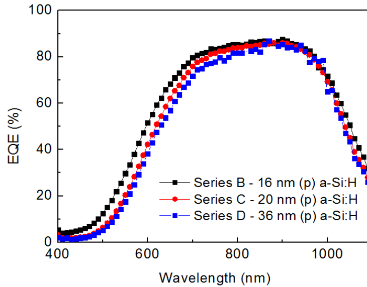
Figure 6-11: Effect of the gradient doping on the EQE of HIT solar cells based on SiNWs.
