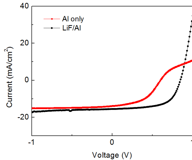
Figure 7-17: (J,V) curves of the thin film devices with LiF/Al cathode (black) and Al cathode (red).
