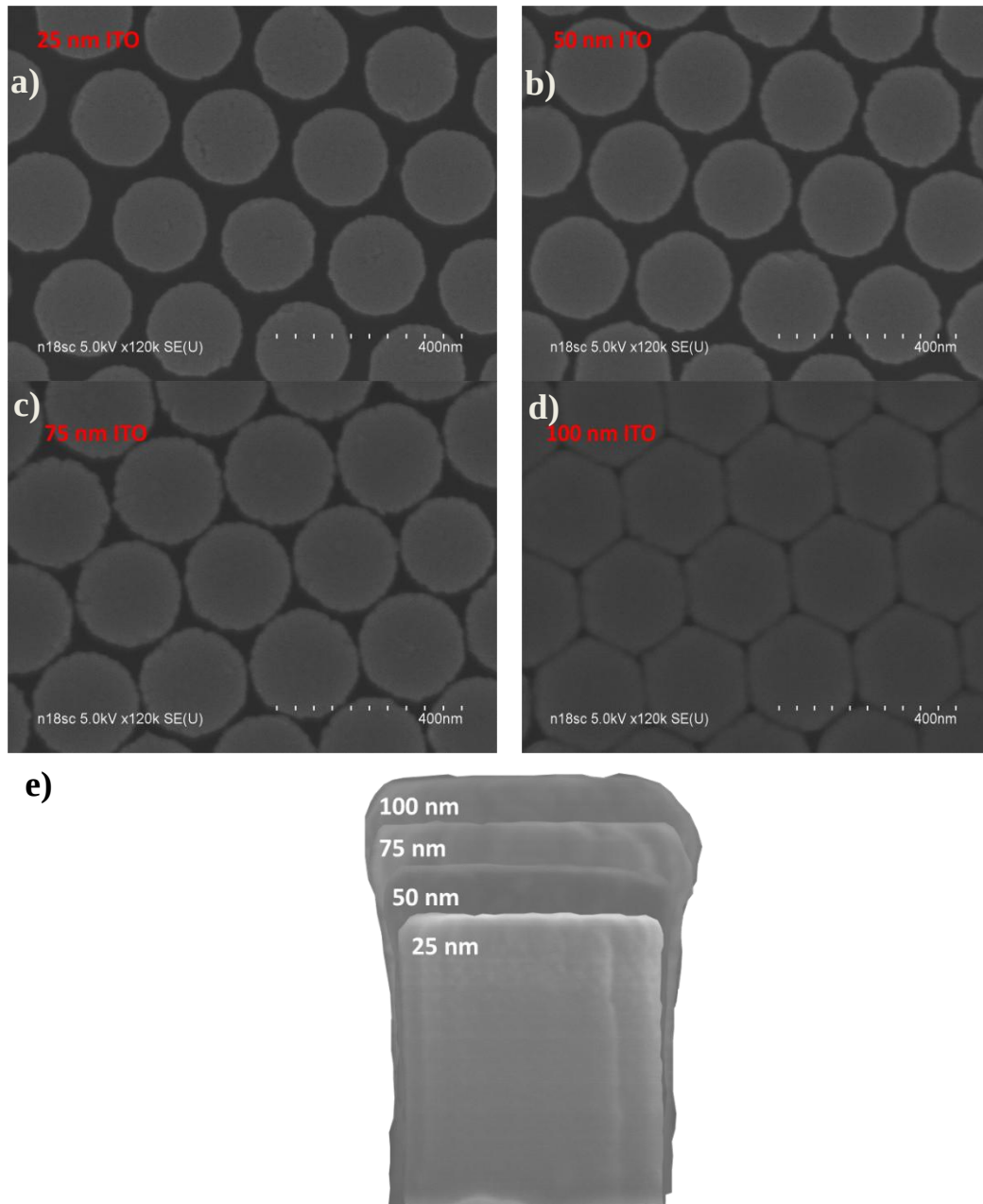
Figure 6-25: Top-view SEM image of ordered arrays of SiNWs covered with a thickness of ITO of (a) 25 nm, (b) 50 nm, (c) 75 nm and (d) 100 nm. (e) shows the cross-section of a single SiNW with various thicknesses of ITO.
