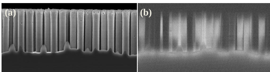
Figure 6-40: Cross-section SEM pictures (a) and corresponding EBIC mapping (b) of samples which underwent an oxidation pre-treatment
