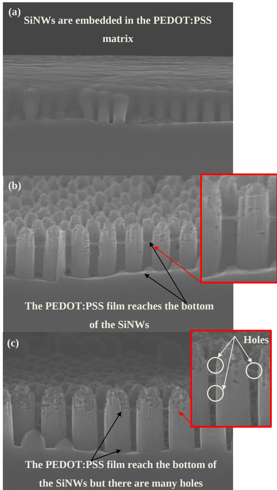
Figure 7-7: SEM pictures of ordered SiNWs after (a) LPAD1, (b) LPAD2 and (c) LPAD3.
