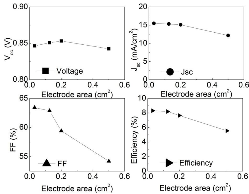
Figure 7-22: Effect of the electrode size on the solar cells' parameters
