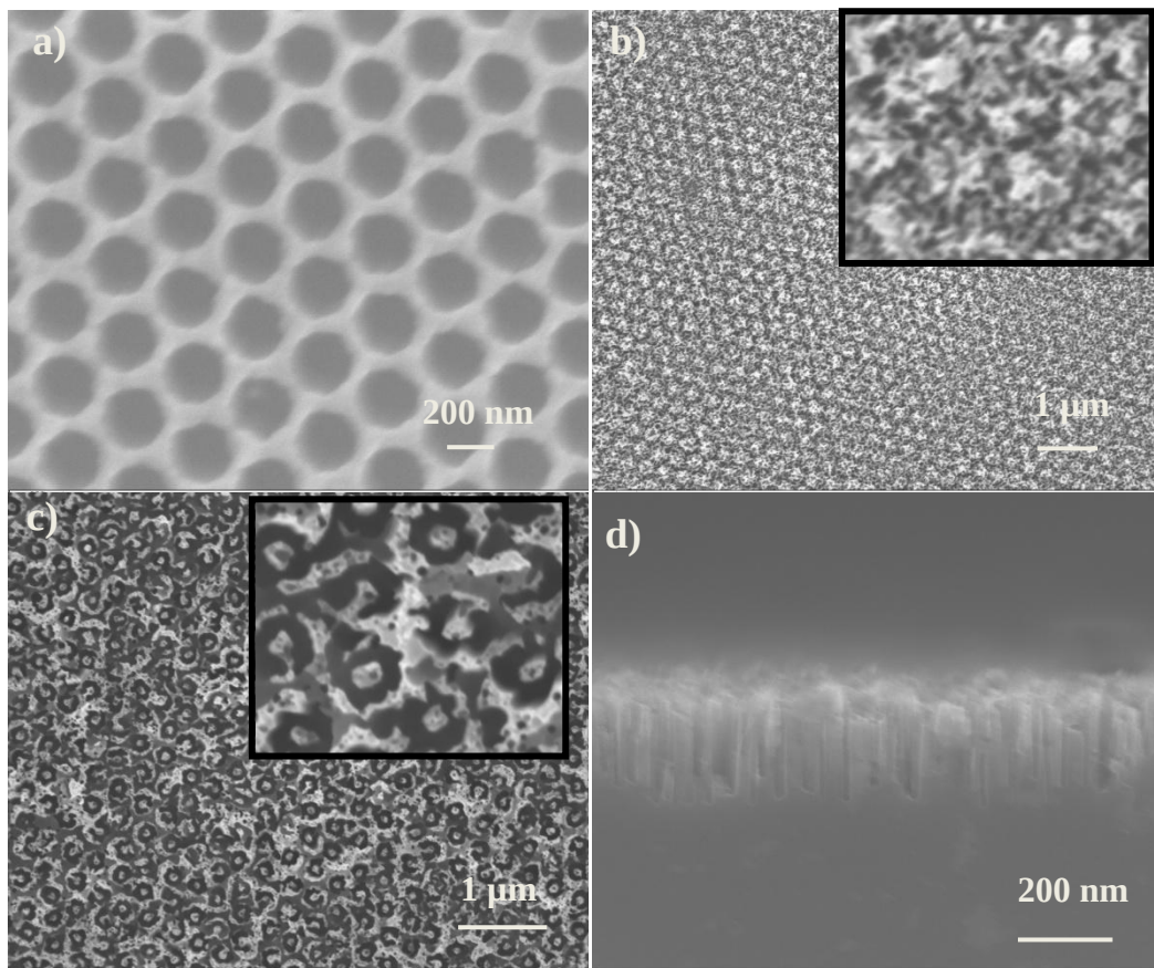
Figure 6-35: (a) Top-view SEM image of the silver etching mask after the removal of the PS spheres. (b) Top view SEM image after 20 s wet chemical etching and removal of silver film (c) ) Top view SEM image after 45 s wet chemical etching and removal of silver film (d) Cross-section SEM picture of SiNWs fabricated by MACE assisted by NSL with silver catalyst after 1 min etching.
