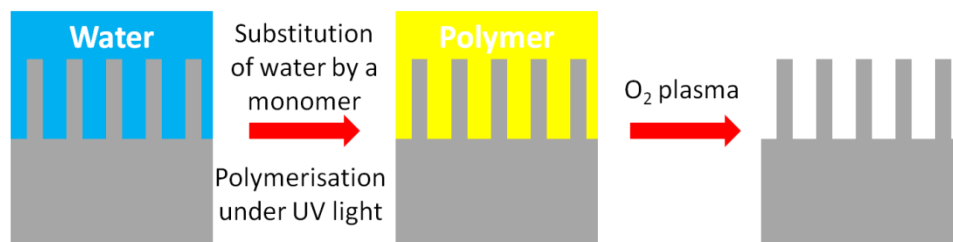
Figure 4-8: Schematic illustrating the principle of strengthen mechanically the nanowires by a polymer.
