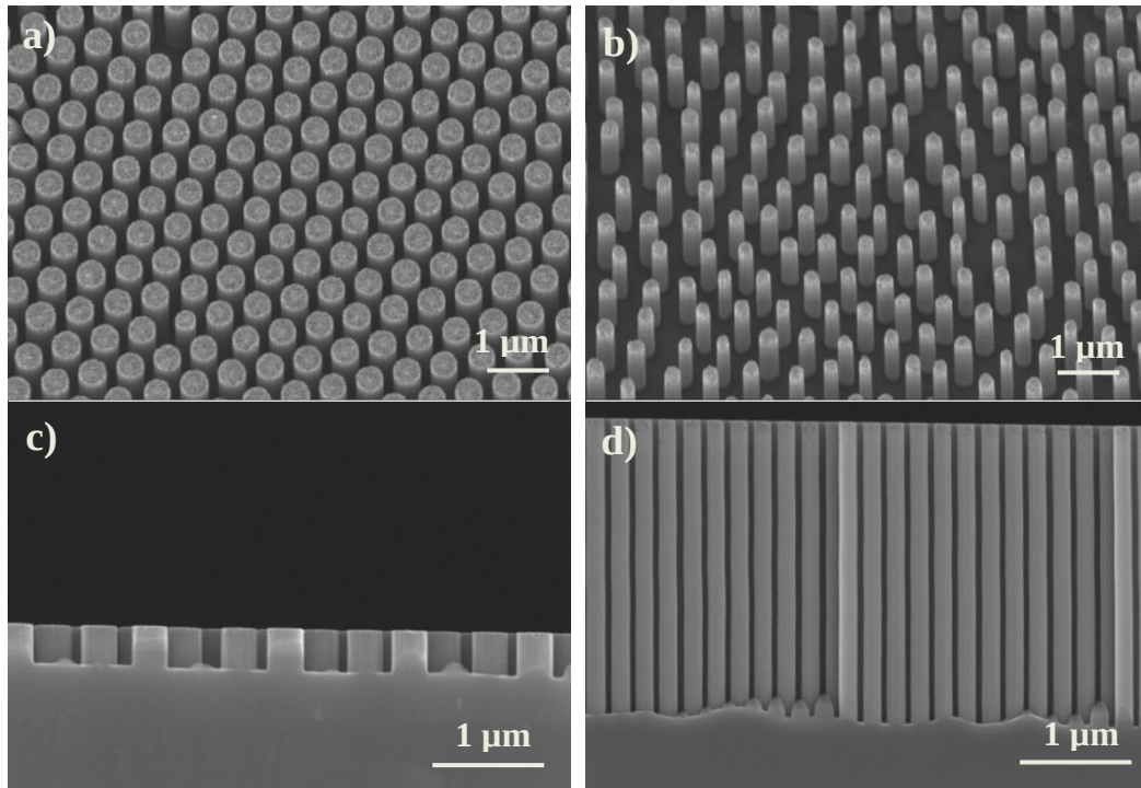
Figure 3-14: (a) SEM pictures of (a) high density SiNWs ordered arrays (inclined 30°) samples with 800 nm pitch , (b) low density SiNWs ordered arrays (inclined 30°) with 800 nm pitch, (c) cross section of short SiNWs, and (d) cross section of long SiNWs.
