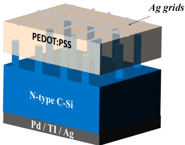
Figure 7-1: Schematic detailing the architecture of the hybrid device
