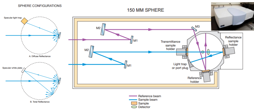
Figure 3-24: Schematics and photograph of the UV/Vis/NIR spectrophotometer (PerkinElmer) using an integrating sphere.
