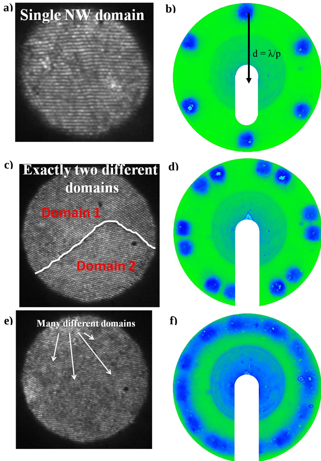
Figure 5-15: (a), (c), (e) Real space (microscopic) image and (b), (d), (f) corresponding M_{11} element detail of the measured Mueller matrices for a single domain (a), (b) , exactly 2 different domains (c), (d) and many small domains (e), (f).
