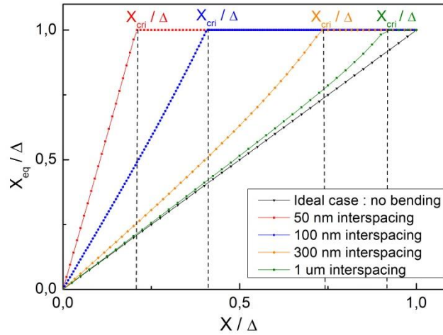
Figure 4-4: Equilibrium position of SiNW #2 as function of its initial position. When the interspacing \Delta between two nanowires in the array is short, any minor irregularity ( X/\Delta > 0.2 or X/\Delta < -0.2 ) lead to adhesion of the nanowires ( X_{\text{eq}}/\Delta = 1/-1 ) whereas for larger nanowires-interspacing \Delta , adhesion occurs for larger irregularities ( X/\Delta > 0.6 or X/\Delta < -0.6 ).
