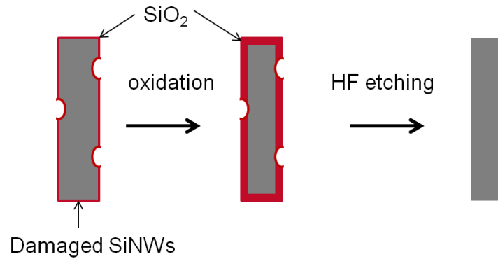
Figure 6-36: Illustration of the oxidation process
