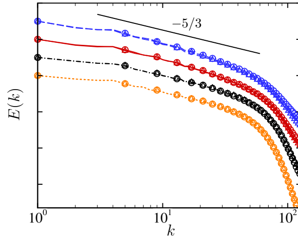
Figure 3.13. PFG and DG simulations. Kinetic energy spectra at t = 2.5 at various initial turbulent Mach numbers. \cdots : M_{t_0} = 0.2 ; \cdots : M_{t_0} = 0.5 ; \cdots : M_{t_0} = 0.8 ; \cdots : M_{t_0} = 1 . \circ : VDW; \triangle : PFG.
