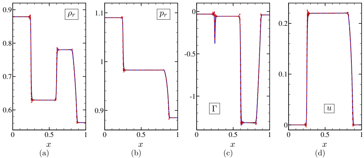
Figure 2.15. Test case DG2. Profiles of reduced density (a), reduced pressure (b), fundamental derivative (c) and velocity (d). Grid: 400 cells, t^* = 0.45 . ---: DRP11 ( r_{th} = 10^{-5} ); - · - · -: DNC9 ( k_2 = 1 ); —: Cinnella (2006).
