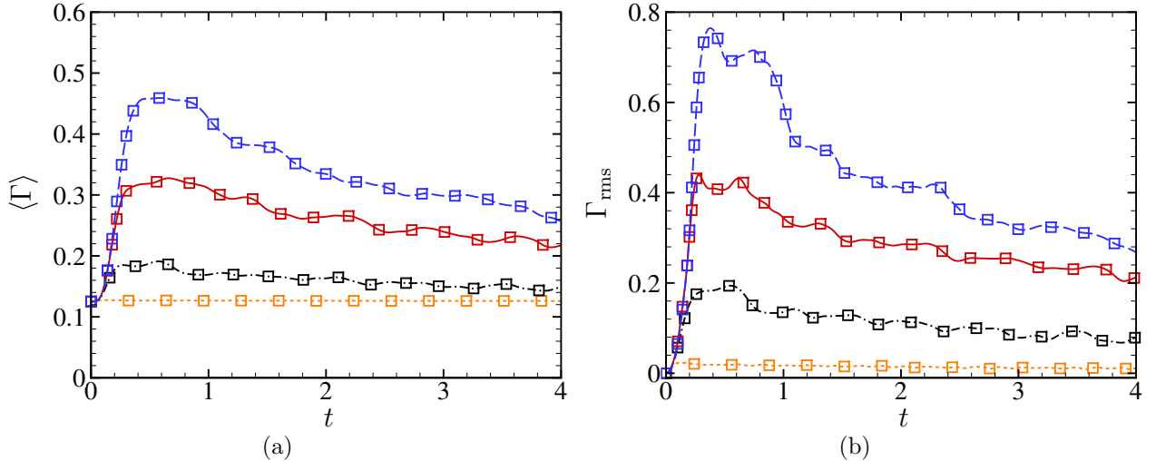
Figure 4.17. Time history of the average (a) and r.m.s. (b) fundamental derivative of gas dynamics at various M_{t_0} . -\cdot-\cdot- : M_{t_0} = 0.2 ; -\cdot-\cdot- : M_{t_0} = 0.5 ; — : M_{t_0} = 0.8 ; -\cdot-\cdot- : M_{t_0} = 1 . \Delta : Air; \square : PP11-MAH.
