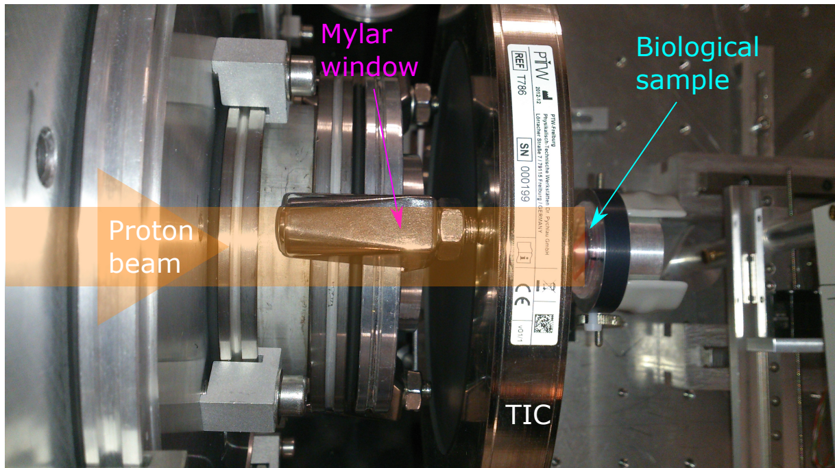
FIGURE 6.1: Picture of the transmission ionization chamber inserted between the biological sample (on the right) and the vacuum chamber (on the left).
