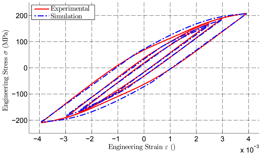
FIGURE 3.18 – Numerical simulation of 3 strain controlled tests ( \Delta\varepsilon/2 = \pm 0.25; 0.3; 0.4\% ) at 20 °C, 10th cycle
