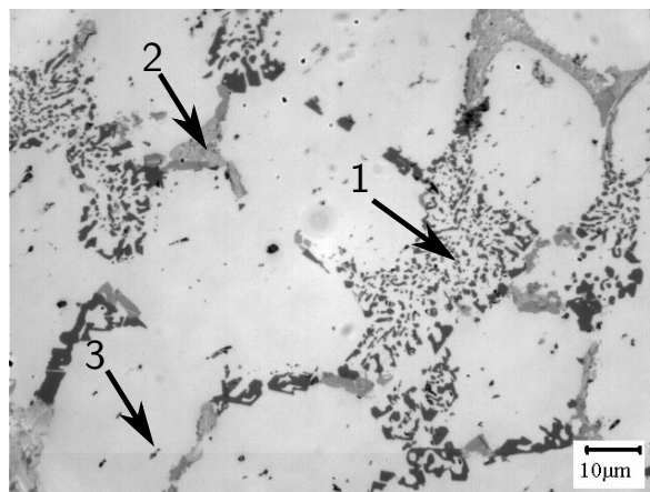
FIGURE 2.3 – Optical microscopy of the material microstructure: (1) small eutectic Si particle, (2) Fe rich intermetallics, (3) Strengthening precipitates trace caused by mirror finish polishing.
