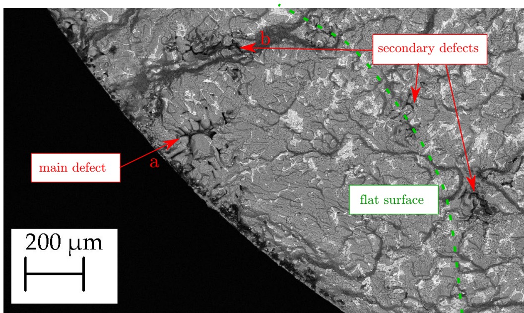
FIGURE 4.14 – SEM-BSE image of shrinkage at specimen edge, (specimen 56T5, \Delta\varepsilon/2 = \pm 0.25\% , R_\varepsilon = -1 , 150^\circ\text{C} , N_f = 4137 cycles).
