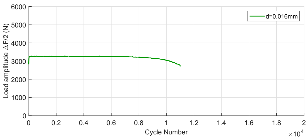
FIGURE 6.4 – Evolution of the load amplitude for T = 150^{\circ}C , on notched specimen ( K_t = 1.78 ).
