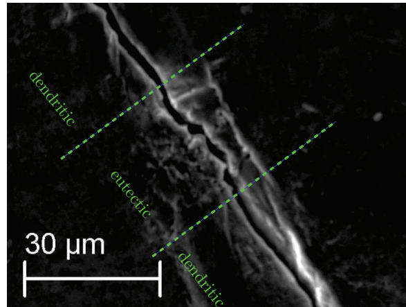
FIGURE 4.49 – SEM-SE1 image of crack coalescence (Specimen 89T5: \Delta\varepsilon/2 = \pm 0.4\% , R_\varepsilon = -1 , 250^\circ\text{C} , N_f = 701 cycles)
