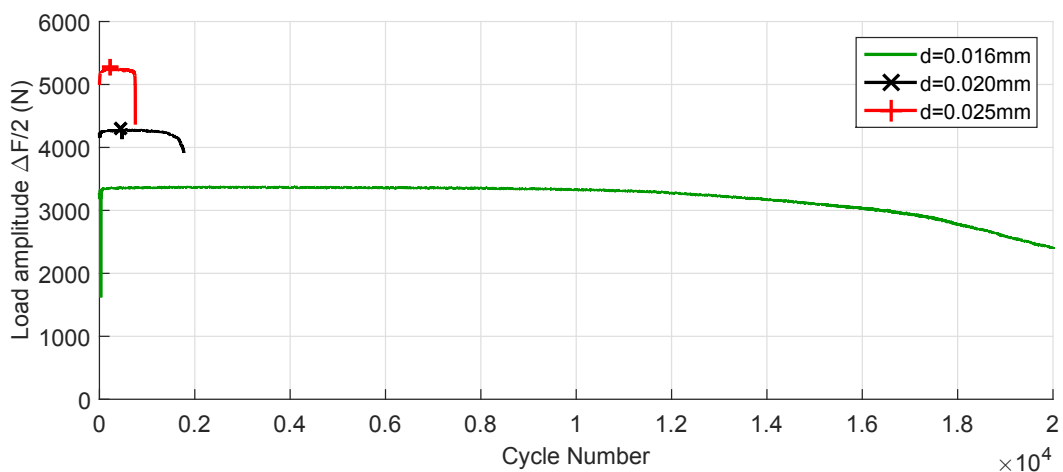
FIGURE 6.3 – Evolution of the load amplitude for T = 20^{\circ}C , on notched specimen ( K_t = 1.78 ).
