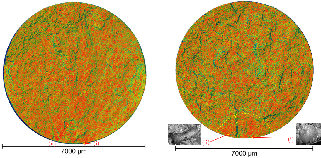
(a) specimen 49T5, \Delta\varepsilon/2 = \pm 0.25\% , R_\varepsilon = -1 , 200^\circ\text{C} , N_f = 3383 cycles
