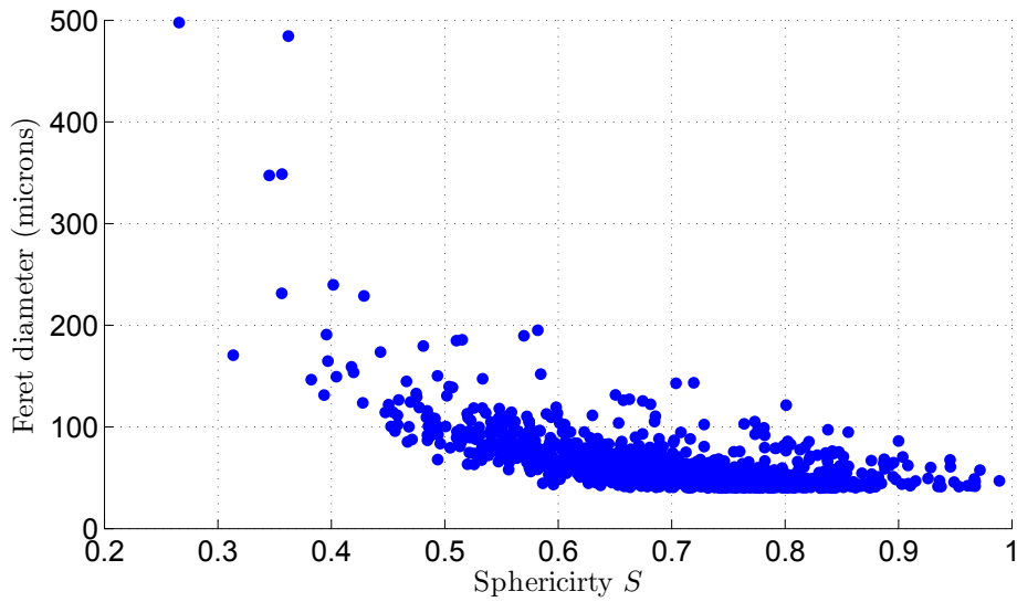
FIGURE 2.25 – Feret diameter d as a function of sphericity S , specimen 12T5.
