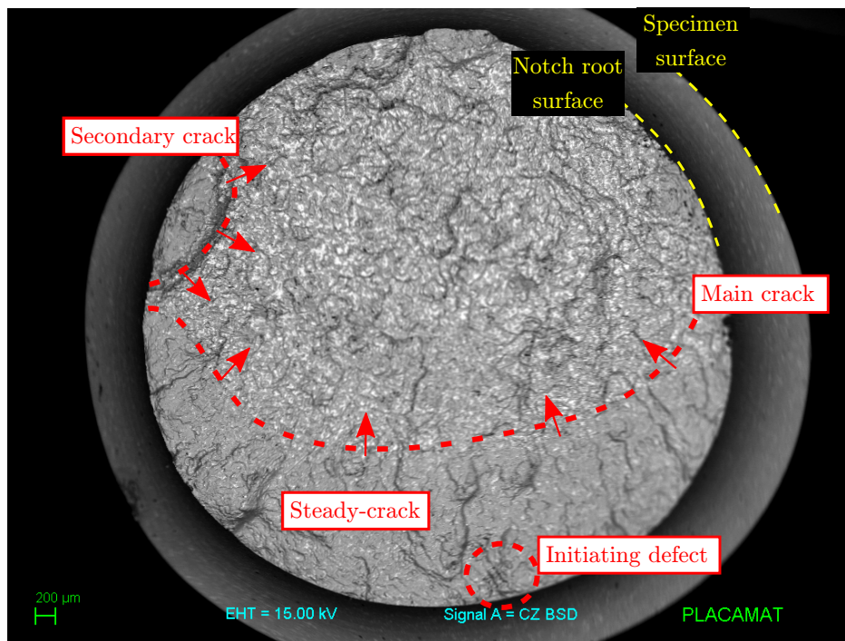
FIGURE 6.9 – General view of the fractured surface of a notched fatigue specimen (specimen 38T5, d = 0.016\text{ mm} , T = 250\text{ °C} , N_f = 3302 cycles).
