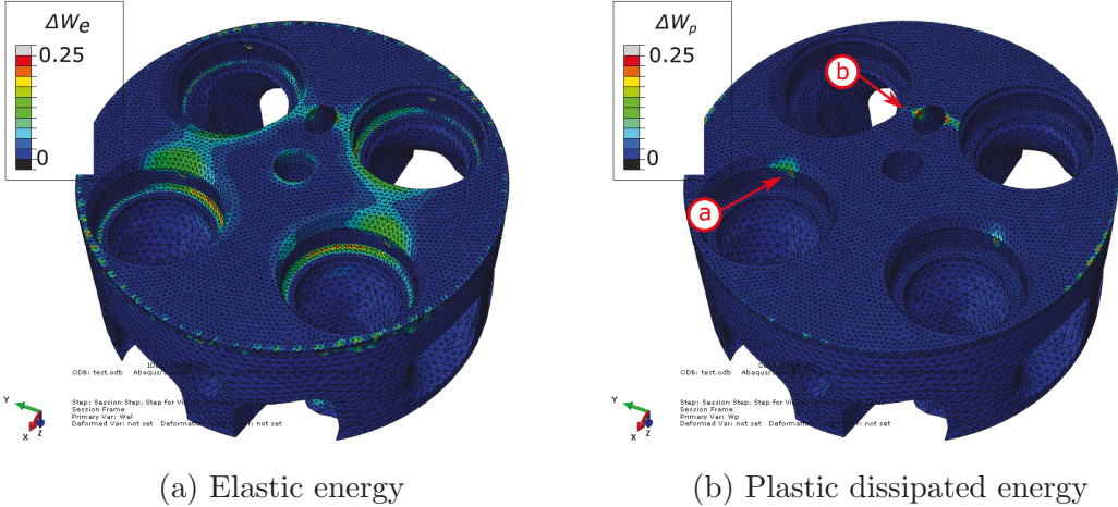
FIGURE 3.31 – Simulated energy quantities (modified values for confidentiality reasons)
