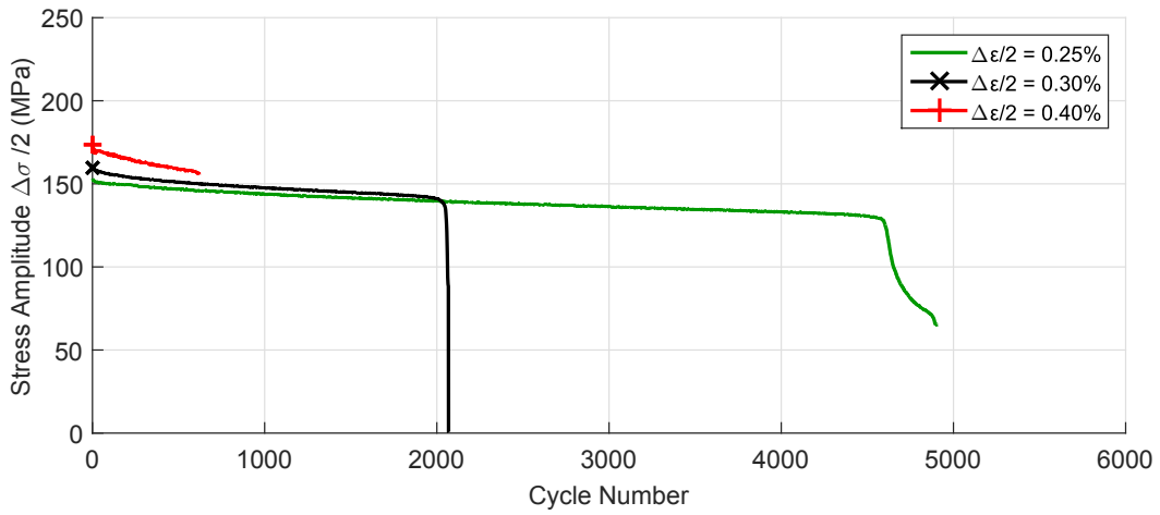
FIGURE 3.11 – Evolution of stress amplitude for T = 200\text{ }^{\circ}\text{C} , R_e = -1
