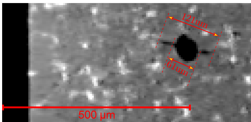
FIGURE 4.23 – Tomography analysis reveals secondary cracks that increase the defect measurement size (Specimen 62T5: \Delta\varepsilon/2 = \pm 0.3\% , R_\varepsilon = -1 , 250^\circ\text{C} , N_f = 2089 cycles)
