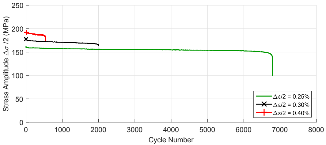
FIGURE 3.10 – Evolution of stress amplitude for T = 150\text{ }^{\circ}\text{C} , R_e = -1
