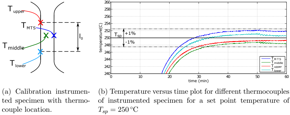
FIGURE 3.3 – Temperature calibration for T_{sp} = 250\text{ }^{\circ}\text{C}
