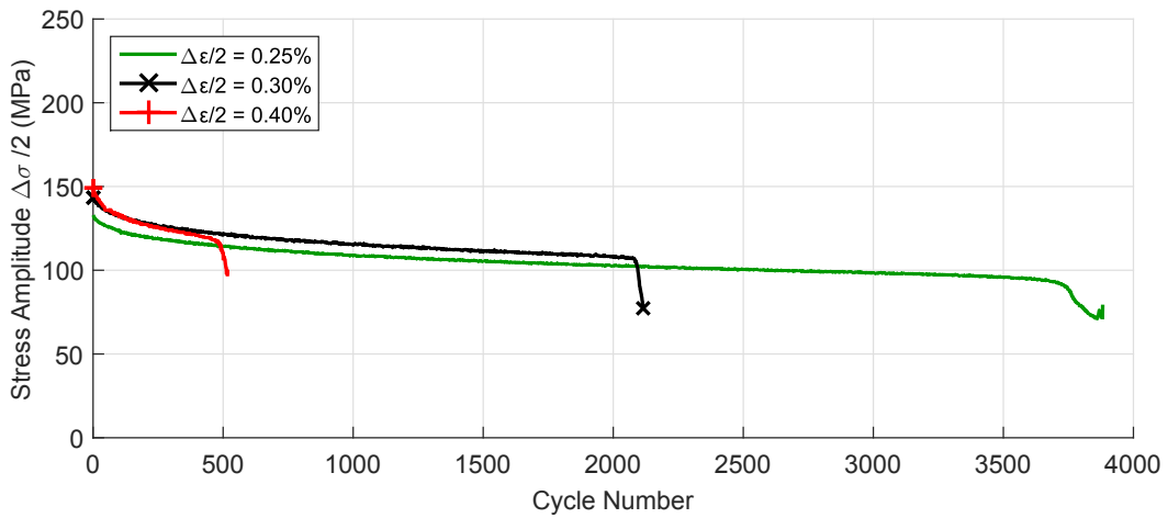
FIGURE 3.12 – Evolution of stress amplitude for T = 250\text{ }^{\circ}\text{C} , R_e = -1
