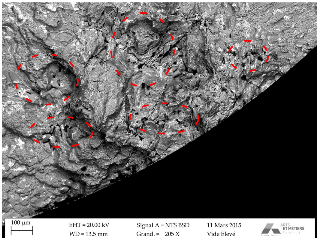
FIGURE 4.15 – SEM-BSE image of defect cluster (specimen 22T5, \Delta\varepsilon/2 = \pm 0.3\% , R_\varepsilon = -1 , 20^\circ\text{C} , N_f = 2689 cycles)
