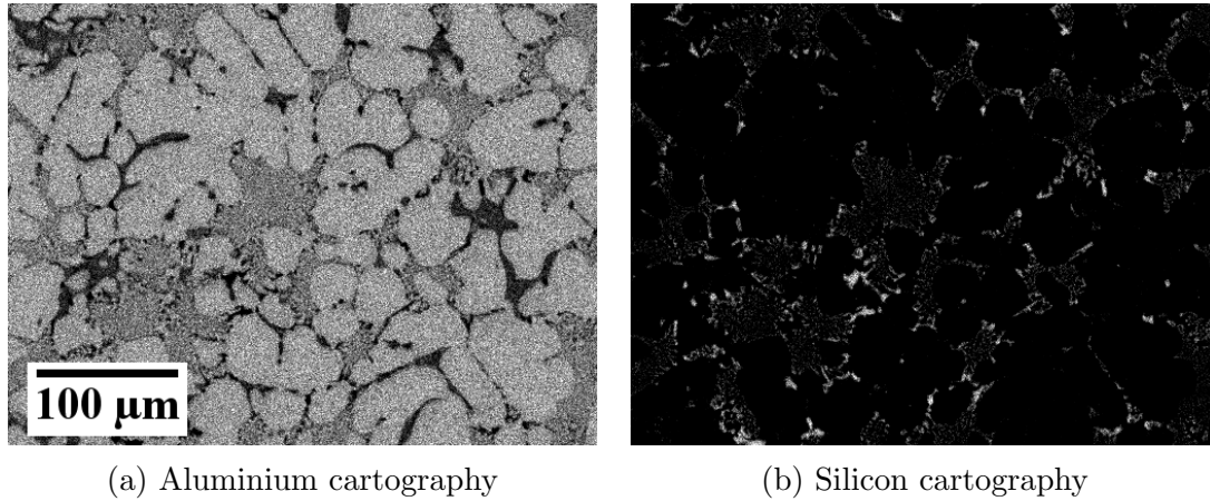
FIGURE 2.2 – EDS cartography
