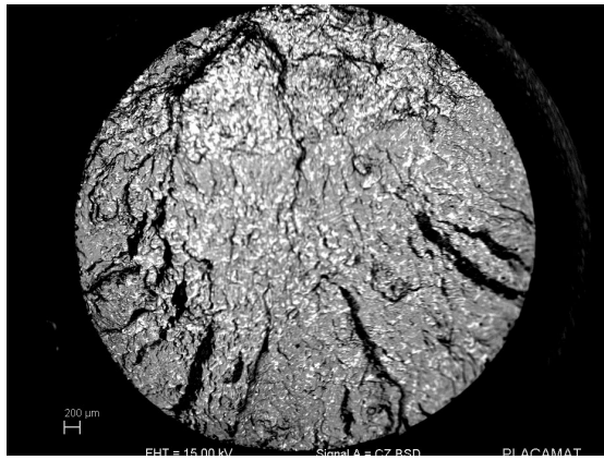
(a) Specimen 41T5, d = 0.016 mm, T = 20 °C, N_f = 11790
