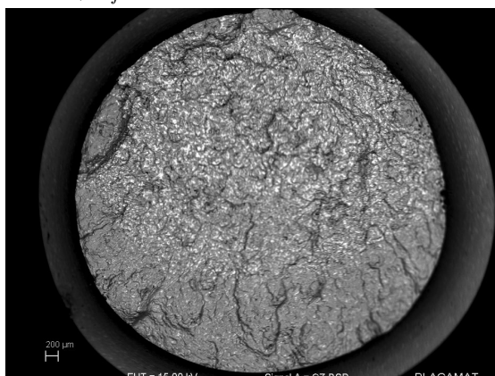
(e) Specimen 38T5, d = 0.016 mm, T = 250 °C, N_f = 3302
