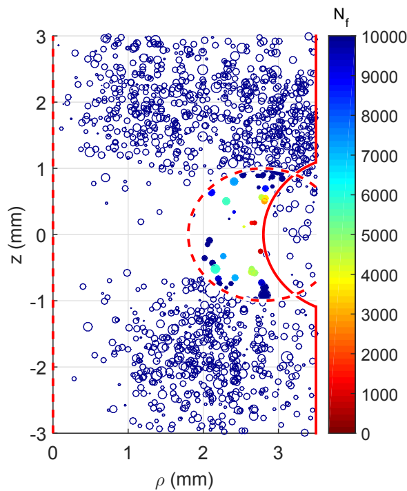
FIGURE 6.33 – Fatigue life simulation of the number of cycles to failure ( N_f ) of notched specimen with defects ( K_t = 1.78 , d = 0.025 mm and T = 20 °C, N_f = 753 ). Specific case of low number of defects close to the notch root. Only the fatigue lives of defects close to the notch root are calculated (full markers)
