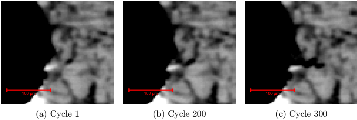
FIGURE 4.26 – Crack initiation on artificial defect. The contrast is purposely set too high revealing crack initiation, which is detected at 186 cycles (Specimen 76T5: \Delta\varepsilon/2 = \pm 0.4\% , R_\varepsilon = -1 , 20^\circ\text{C} , N_f = 731 cycles)
