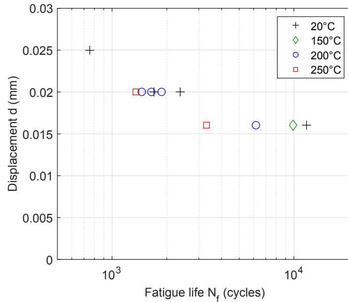
FIGURE 6.8 – Fatigue life for notched specimens ( K_t = 1.78 ).
