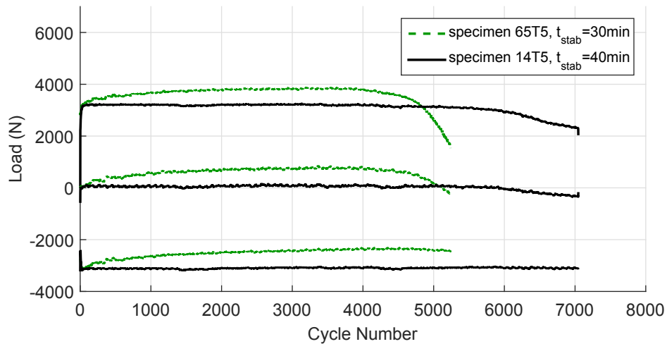
FIGURE 6.2 – Influence of stabilisation time: evolution of load minimum, mean and maximum value per cycle, test temperature T = 200^{\circ}C and displacement d = 0.016 mm . For specimen 65T5 (resp. 14T5), the mechanical loading starts 30 min (resp. 40 min) after thermal loading. The total test time is approximately 5 h.
