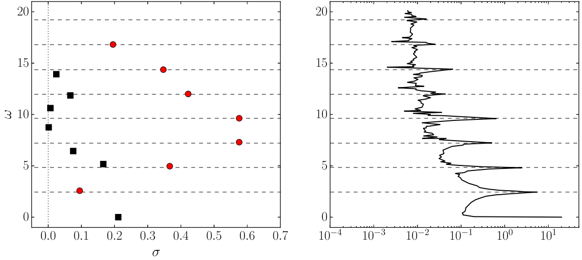
Fig. 4.2 From Mettrot et al. (2014a): cavity flow at a Reynolds number Re = 860000 . Comparison between the unstable ( \sigma > 0 ) eigenvalues obtained from a RANS base flow analysis (left) and the pressure spectrum at a given point in the shear layer, computed by time marching the RANS equations (right). Both results are based on the k - \omega model of Wilcox (Roe scheme). The dashed lines indicates the Rossiter peak and harmonics observed in the experiment by Forestier et al. (2003). The eigenvalues matching these frequencies are indicated by the red dots.
