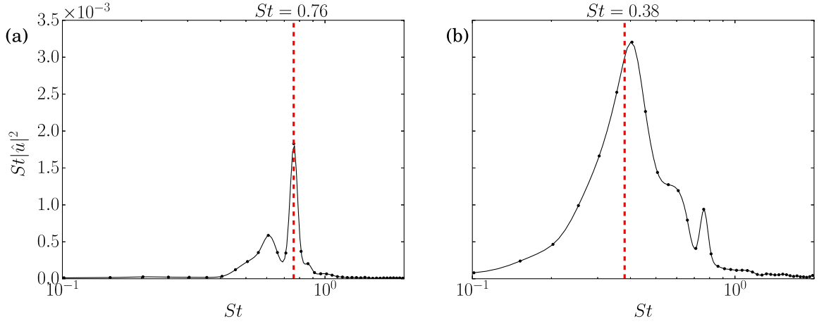
Fig. 6.7 Frequency spectrum of the streamwise velocity at (a) x = 1.0 , y = 0.3 and (b) x = 1.5 , y = 0.25 , computed from the PIV results (reference set). The upstream spectrum (a) displays a clear peak at St = 0.76 , linked to the Kelvin-Helmholtz mechanism, while further downstream, (b) displays a broader spectrum center around St = 0.38 . This latter frequency is related to the typical downstream vortex pairing that occurs in such flows.
