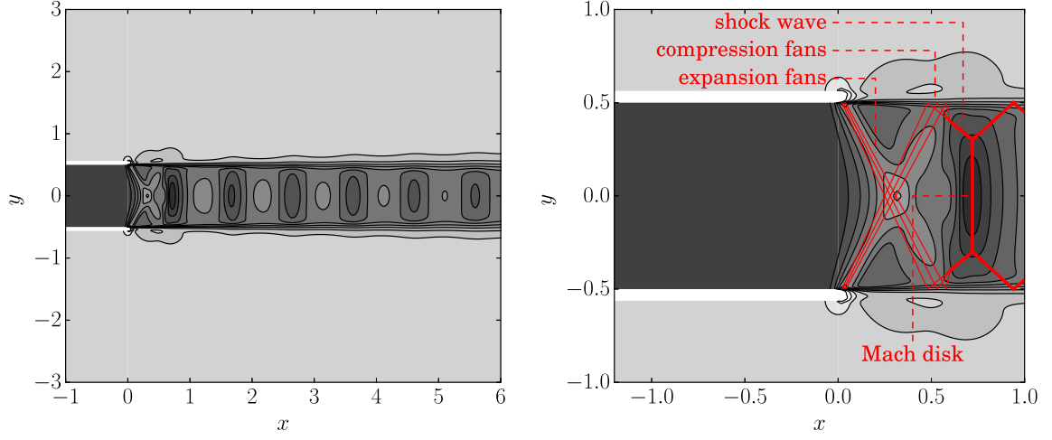
Fig. 3.3 Left: density field of the computed base flow (JPR=1.12, h_l = 0.063 ). One can notice the expected shock-cell structure. Right: zoom on the exit of the nozzle, on which we have represented the main features of underexpanded jets. The figures display 15 contours equally spaced between 0.9 and 1.4 (nondimensional density unit).
