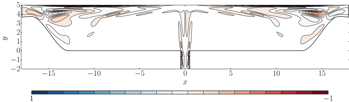
Fig. 2.8 Density field of mode B ( St = 0.55 ) for Re = 660 .
