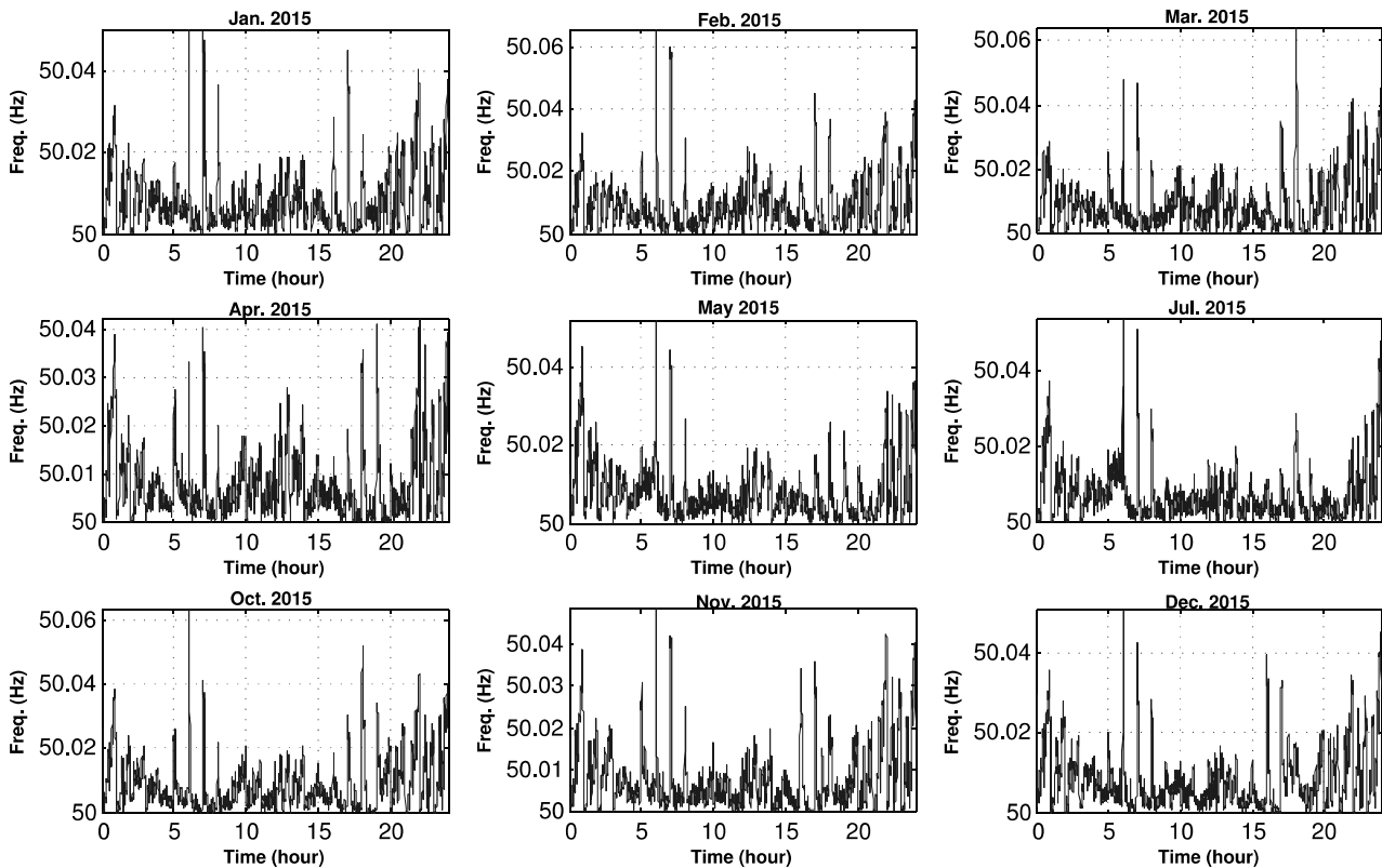
Figure 3.23: Daily averaged absolute frequency variation for 9 months in France.
