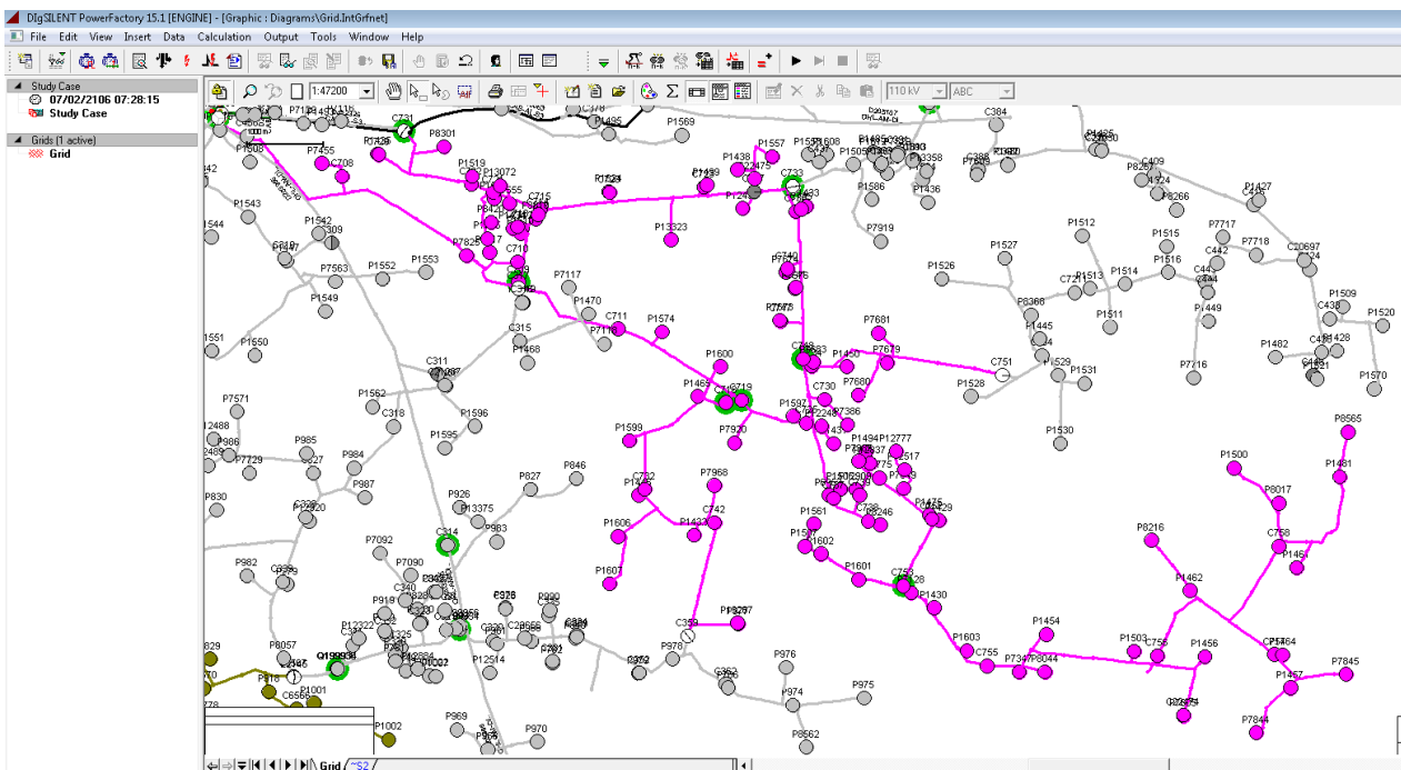
Figure 5.5: MV feeder (E88640) modeled in DIGSILENT illustrated in magenta color. The circles shows MV/LV substations (15/0.4 kV).
