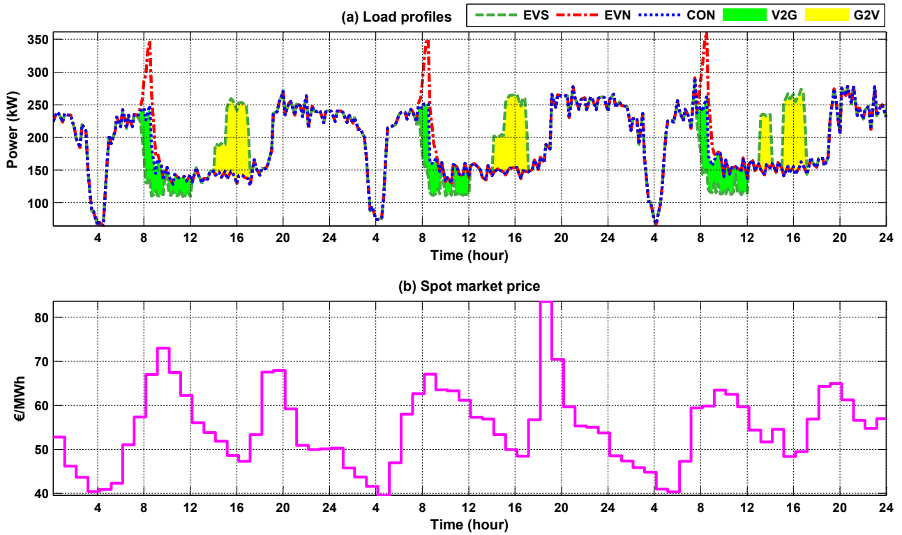
Figure 4.64: Comparison of supervised (EVS), and unsupervised (EVN) scenarios in spot market (Category A).
