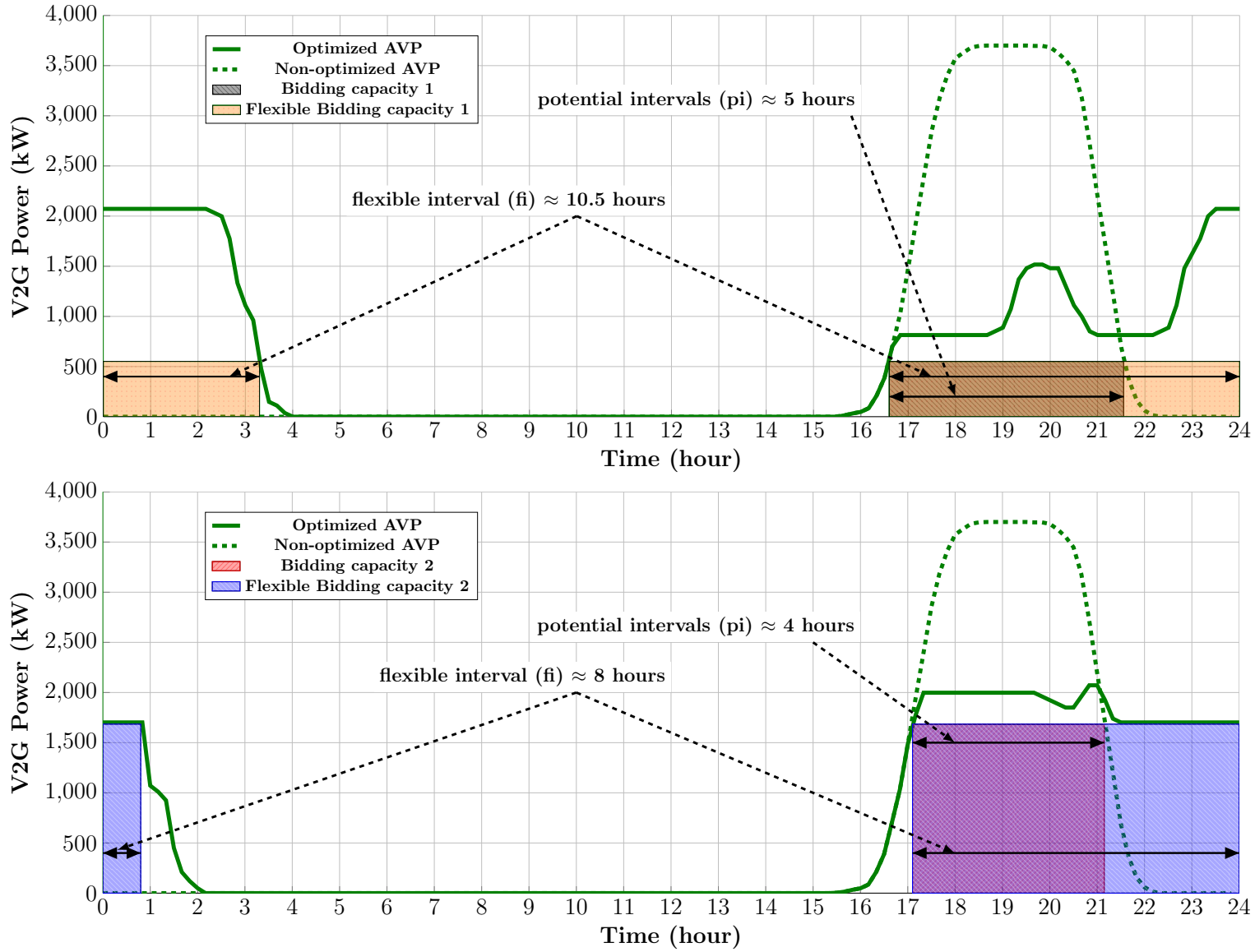
Figure 3.21: Upper plot: BC1 flexible interval, Lower plot: BC2 flexible interval.
