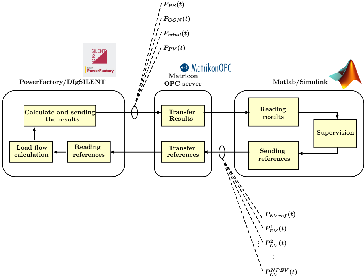
Figure 5.1: Co-simulation flowchart between MATLAB™, OPC server and DiGSILENT for V2G supervision system.
