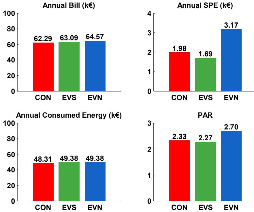
Figure 4.59: Predictive real-time supervision indicator result (Category B).
