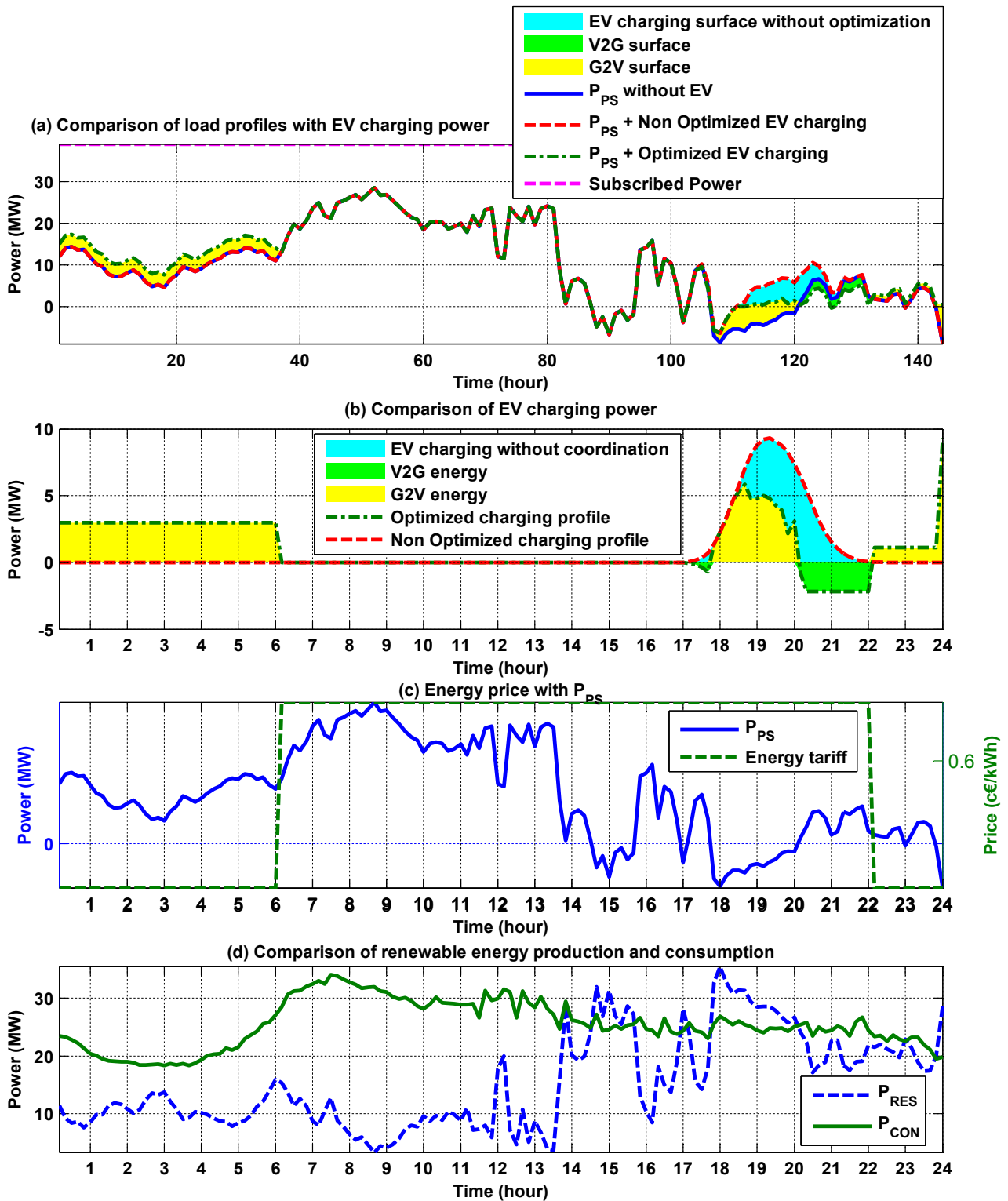
Figure 2.25: Comparing the optimization result for one summer day and home charging scenario, case of local production of renewable energy surplus compared to the consumption.
