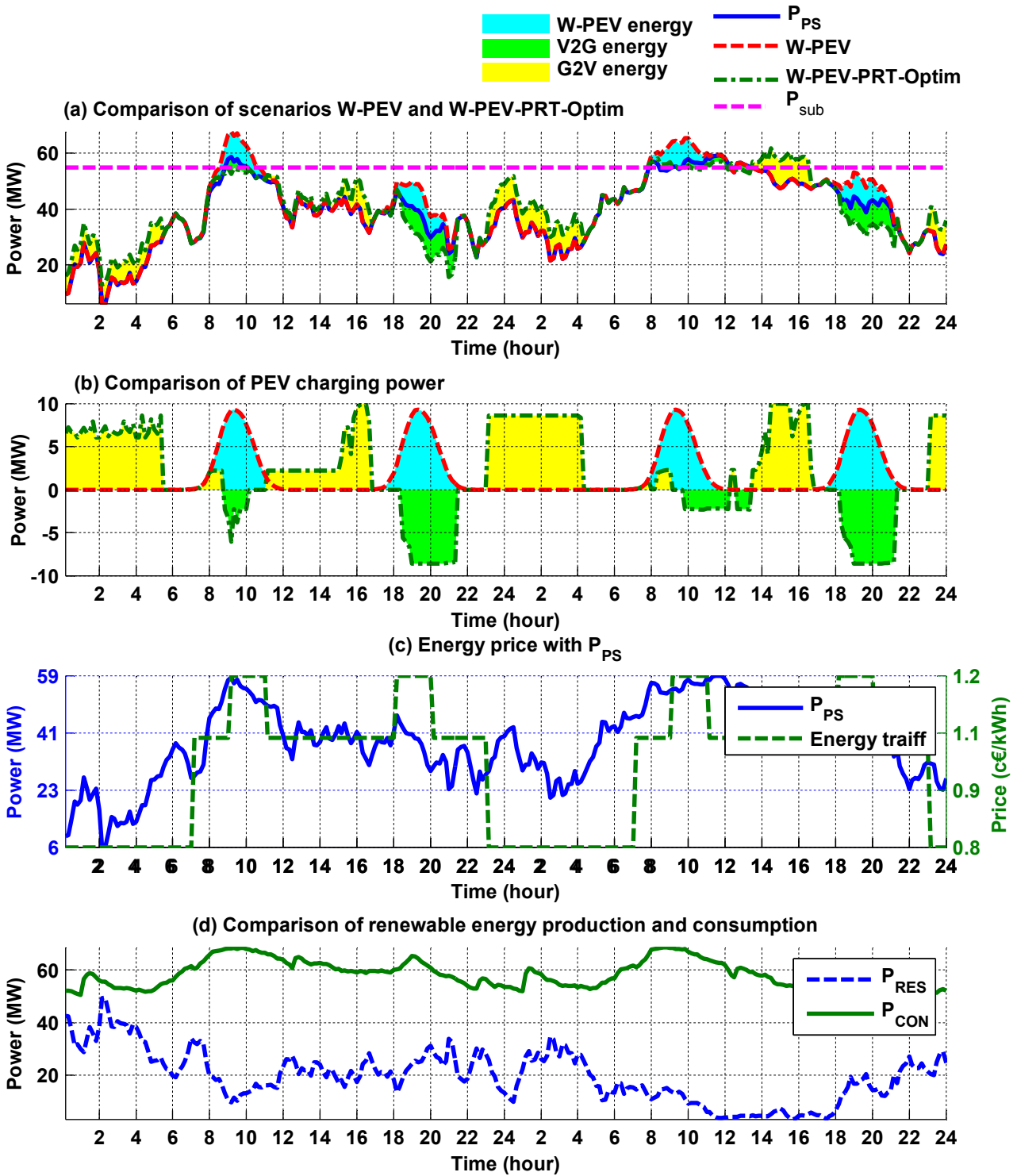
Figure 4.41: 2 days example of supervision for W-PEV-PRT-Optim scenario.
