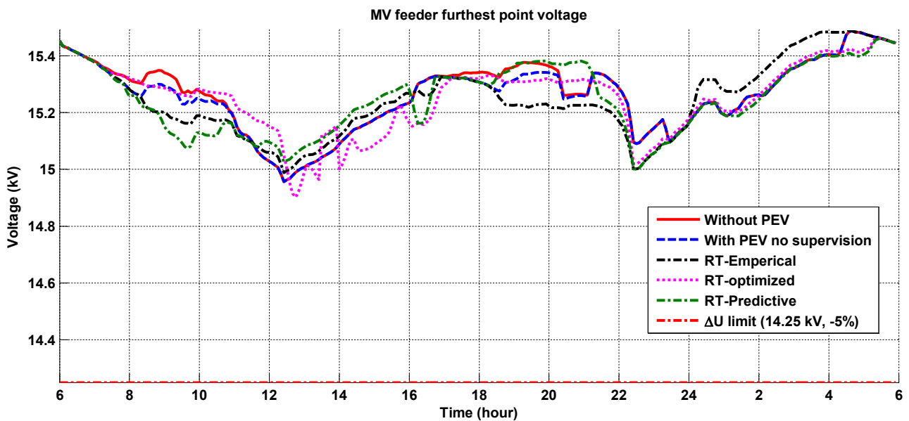
Figure 5.16: MV feeder furthest point voltage profile, day 178.
