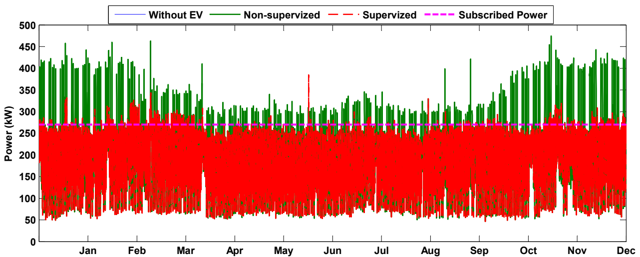
Figure 4.55: Annual load profile comparison for supervised scenario, non-supervised and without PEV scenarios ( Category A ).
