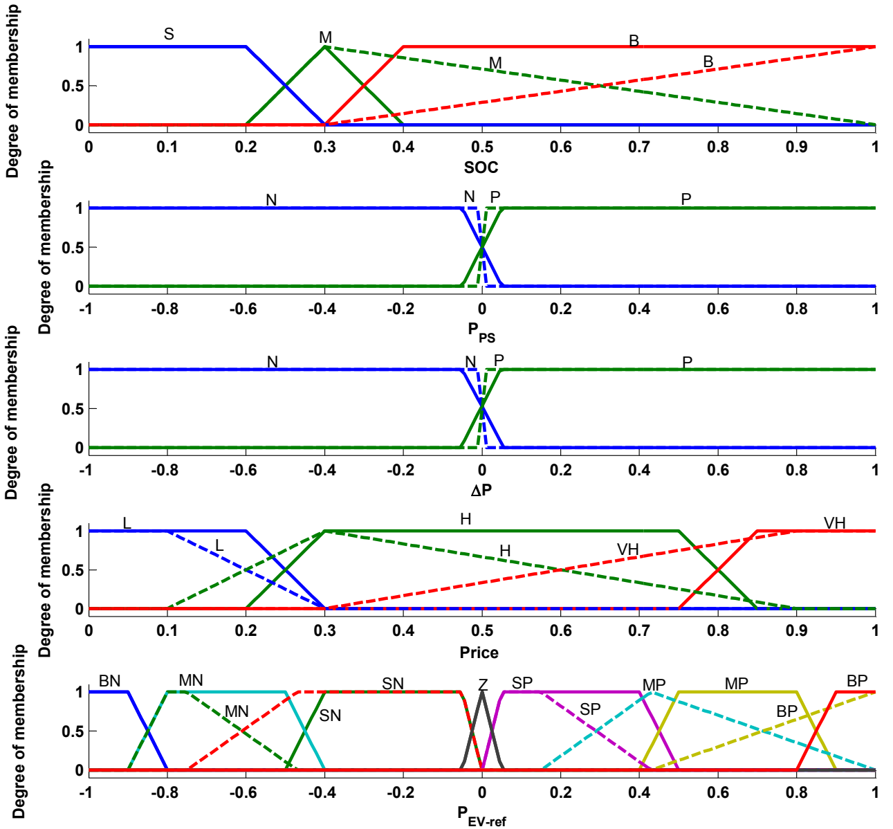
Figure 4.37: Membership functions of Real-time supervision with optimized parameters.
