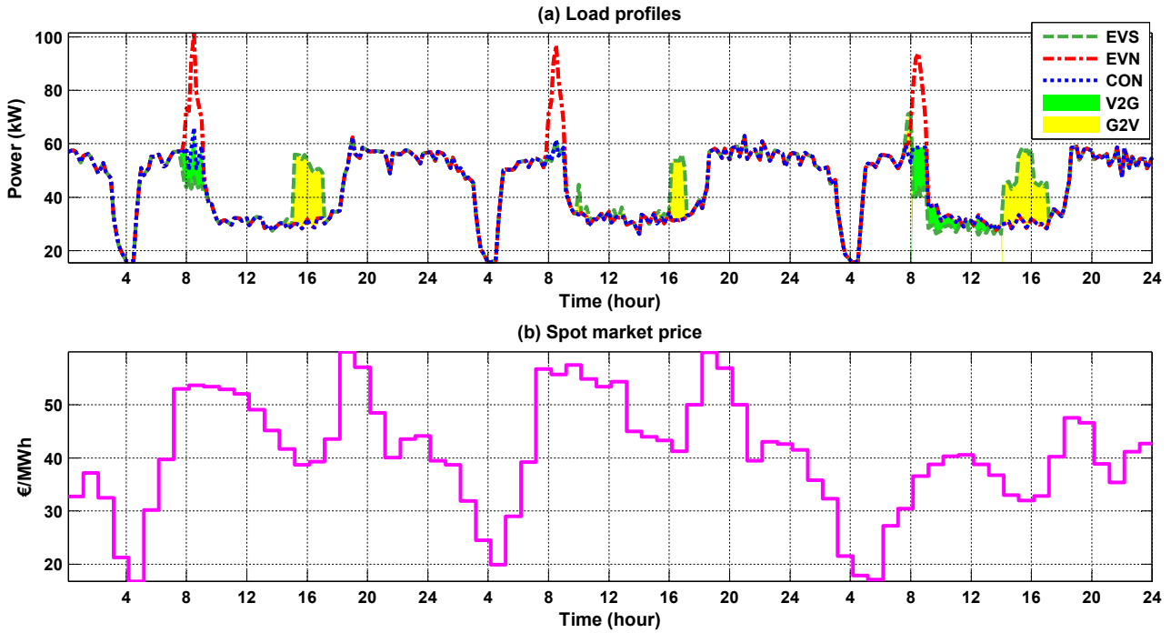
Figure 4.62: Comparison of supervised (EVS), and unsupervised (EVN) scenarios in spot market (Category C).
