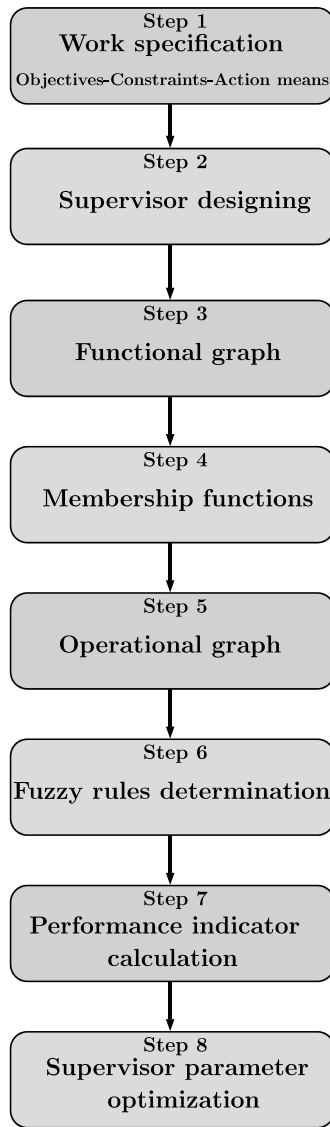
Figure 4.26: Methodology for fuzzy logic supervisor design [Robyns 15a].
