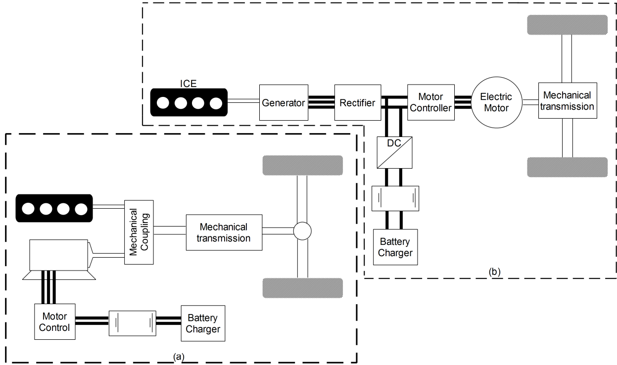
Figure 1.5: Configuration of (a) a parallel hybrid and (b) a series hybrid electric drive train
