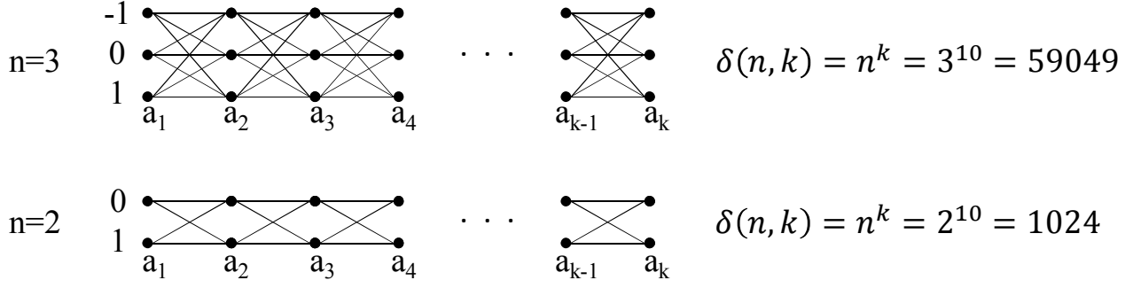
Figure 2.29: Comparison of number of possibilities for case of charging/discharging control with mixed integer variables and binary variables.
