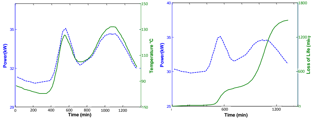
Figure 2.1: Impact of EV charging on hotspot temperature and loss of life of the distribution transformer [Grahm 11].
