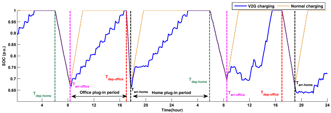
Figure 4.49: Two days example of SOC profile for a single PEV with arrival and departure times to the office and home, comparison of V2G charging and Normal charging scenarios.
