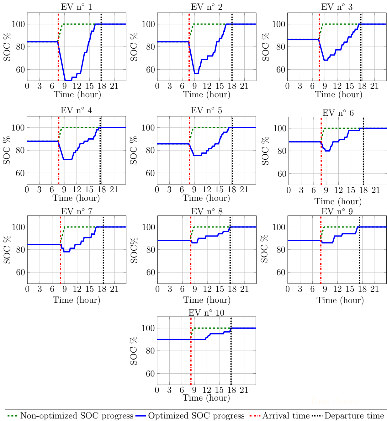
Figure 2.30: SOC evolution comparison for a case of 10 PEVs.
