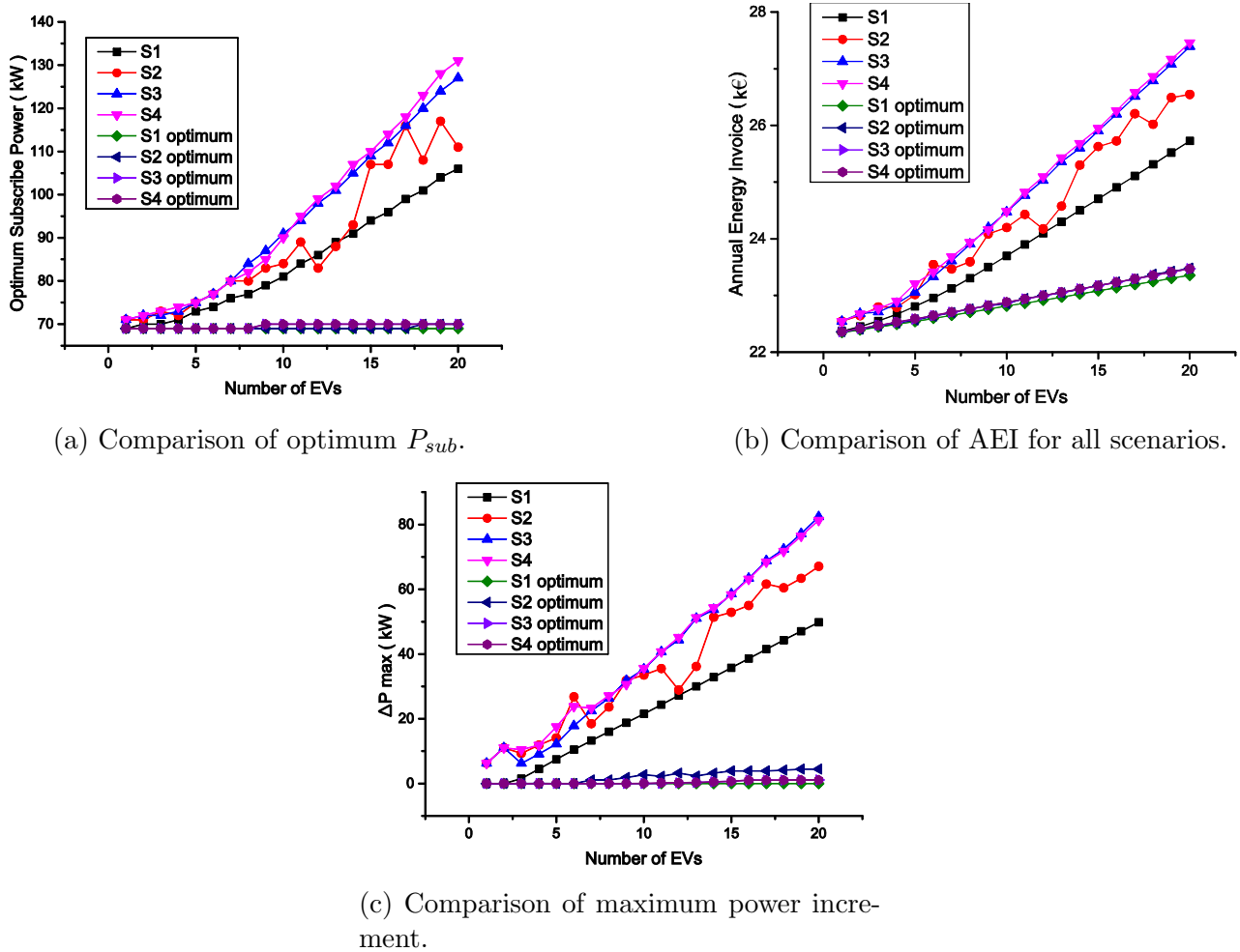
Figure 2.32: Comparison of different indicator for optimum and non-optimum scenarios
