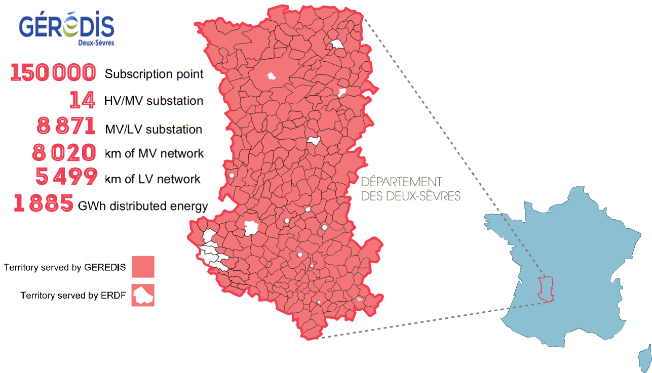
Figure 2.5: GEREDIS territory and grid key values
