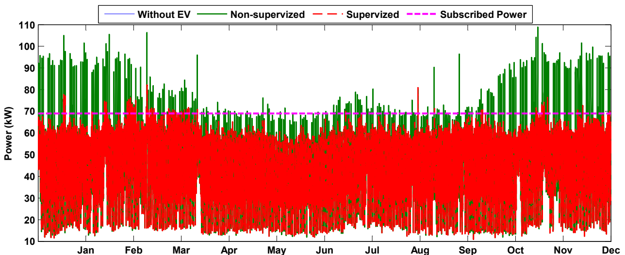
Figure 4.57: Annual load profile comparison for supervised scenario, non-supervised and without PEV scenarios ( Category C ).
