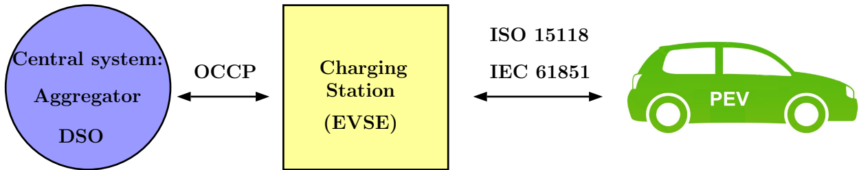
Figure 1.17: Smart charging communication protocol containing V2G communication.
