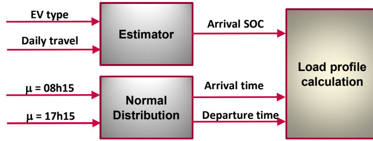
Figure 2.8: Probabilistic algorithm for load profile calculation of electric vehicles.
