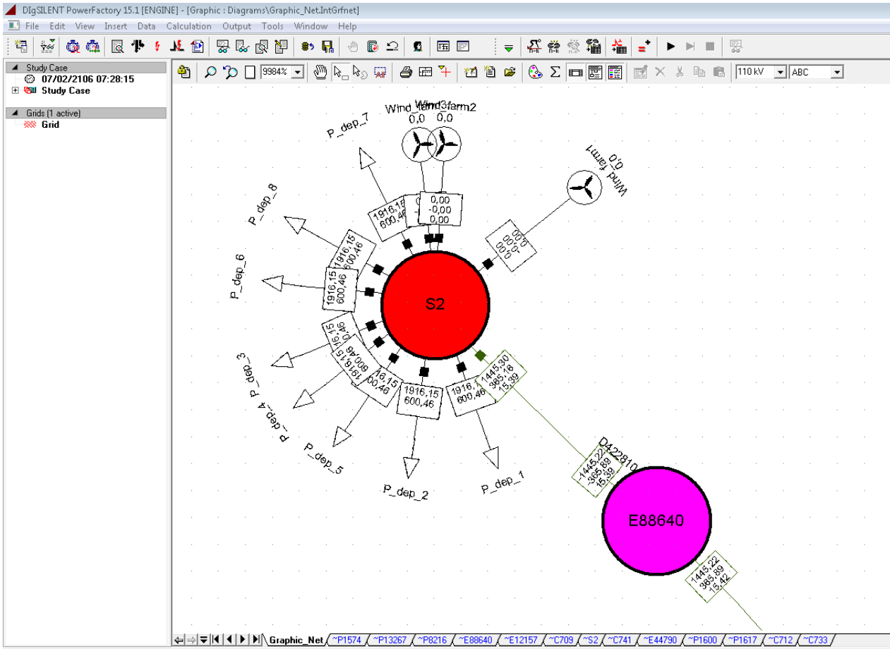
Figure 5.4: HV/MV substation model in DIGSILENT containing three dedicated wind farms MV feeders and 9 consumption feeders. E88640 denotes the modeled MV feeder (15 kV) . S2 indicates the HV/MV substation (90/15 kV).
