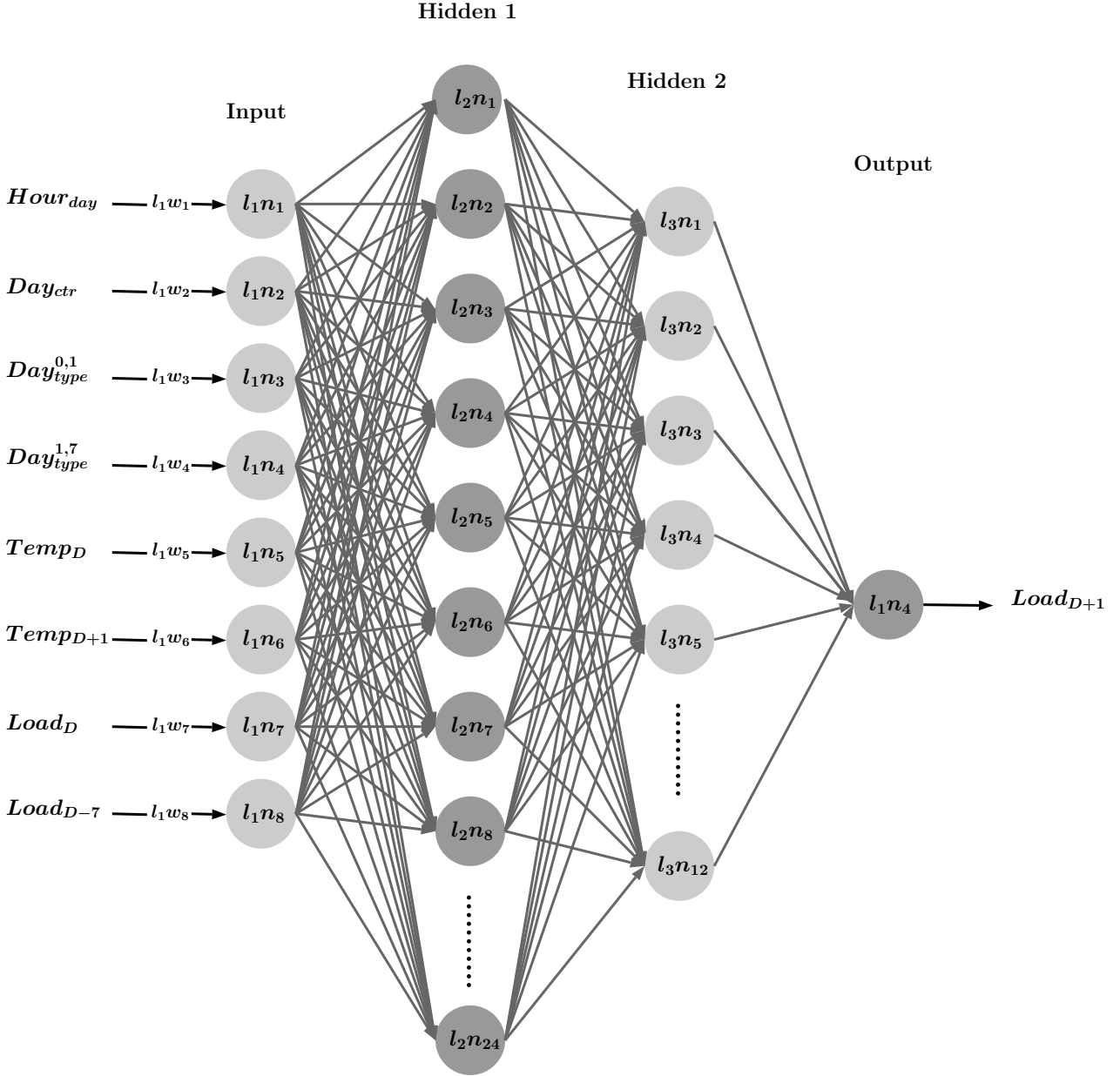
Figure 4.9: Multi-layer feed-forward backpropagation ANN for STLF application.
