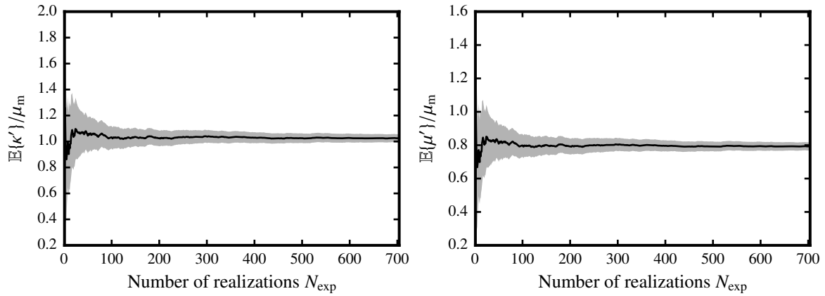
Figure 3.6. Convergence of the statistical estimators for the mean values of the random bulk (left panel) and shear (right panel) moduli. The error bar (gray zone) represents 99% confidence interval.
