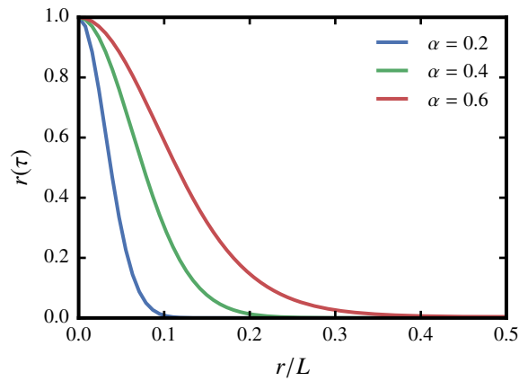
Figure 3.1. Correlation function (46) for various values of \alpha .
