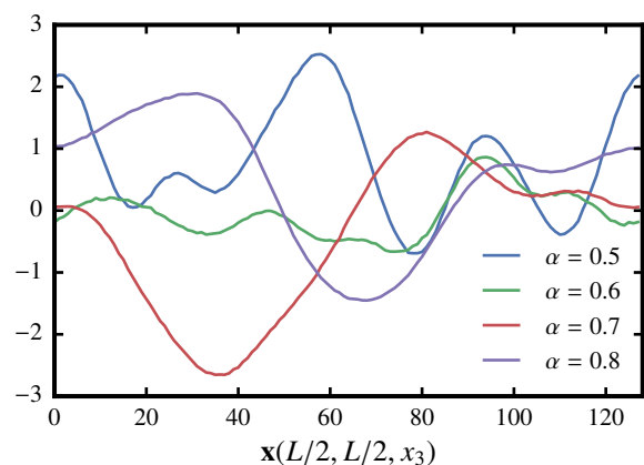
Figure 3.4. Sample paths of the gaussian random field for various values of \alpha (see equation (46)).
