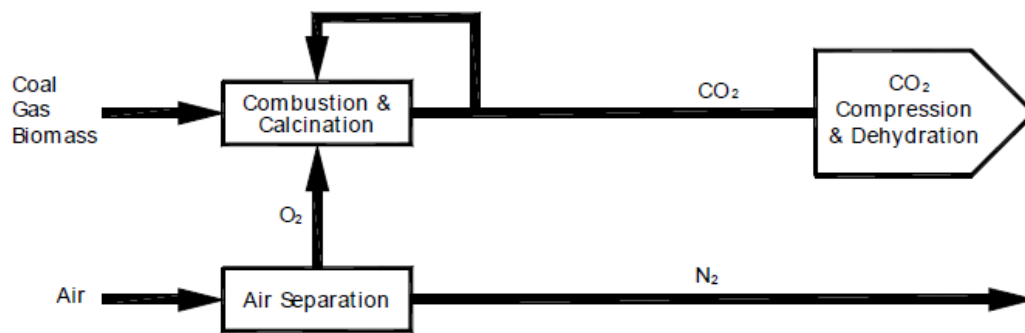
Figure 5.9 Oxy-fuel combustion carbon capture (Source: [International Energy Agency 2008])
