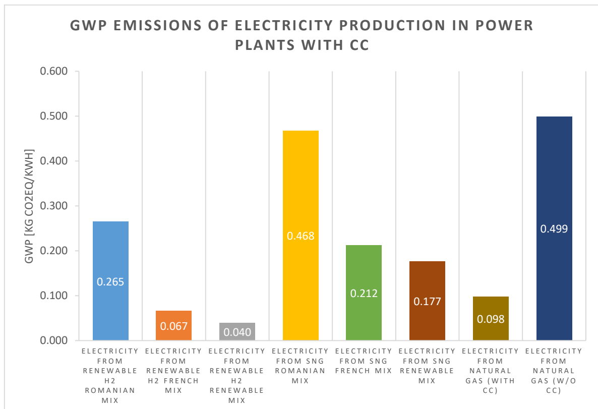
Figure 10.6 GWP emissions of electricity production scenarios
