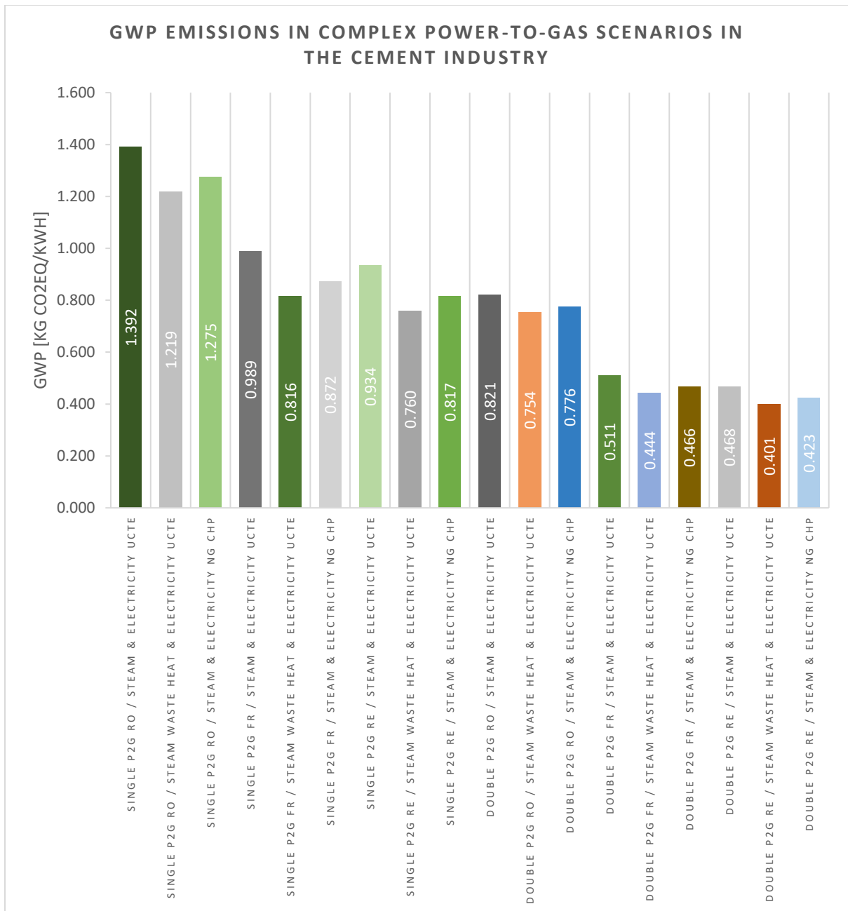
Figure 10.8 GWP emissions of electricity production in complex Power-to-Gas scenarios using fossil carbon from the cement industry
