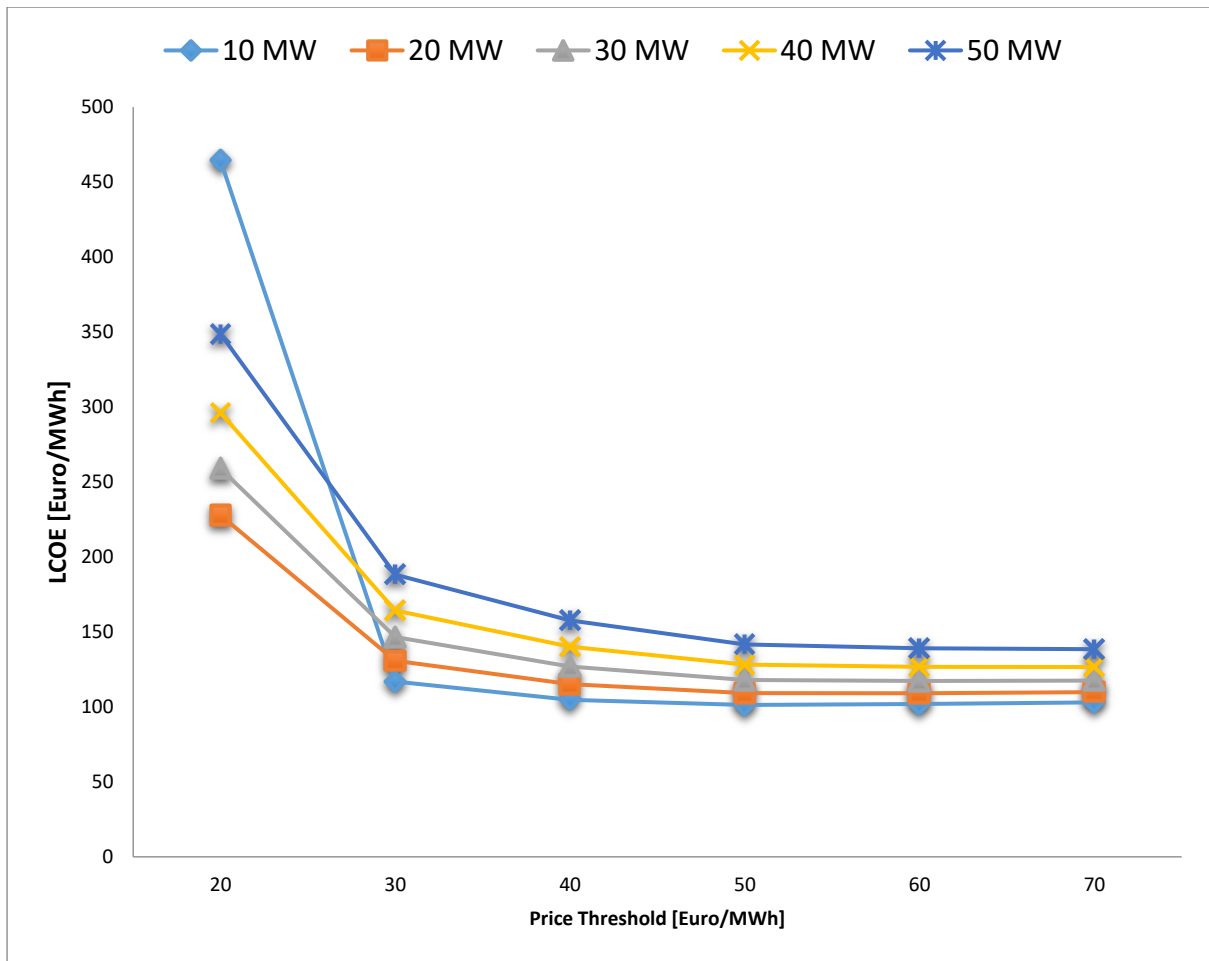
Figure 8.17 Levelized Cost of Energy depending on different energy market price threshold values in the 2030 Power-to-Gas SNG pathway using PEM electrolysis
