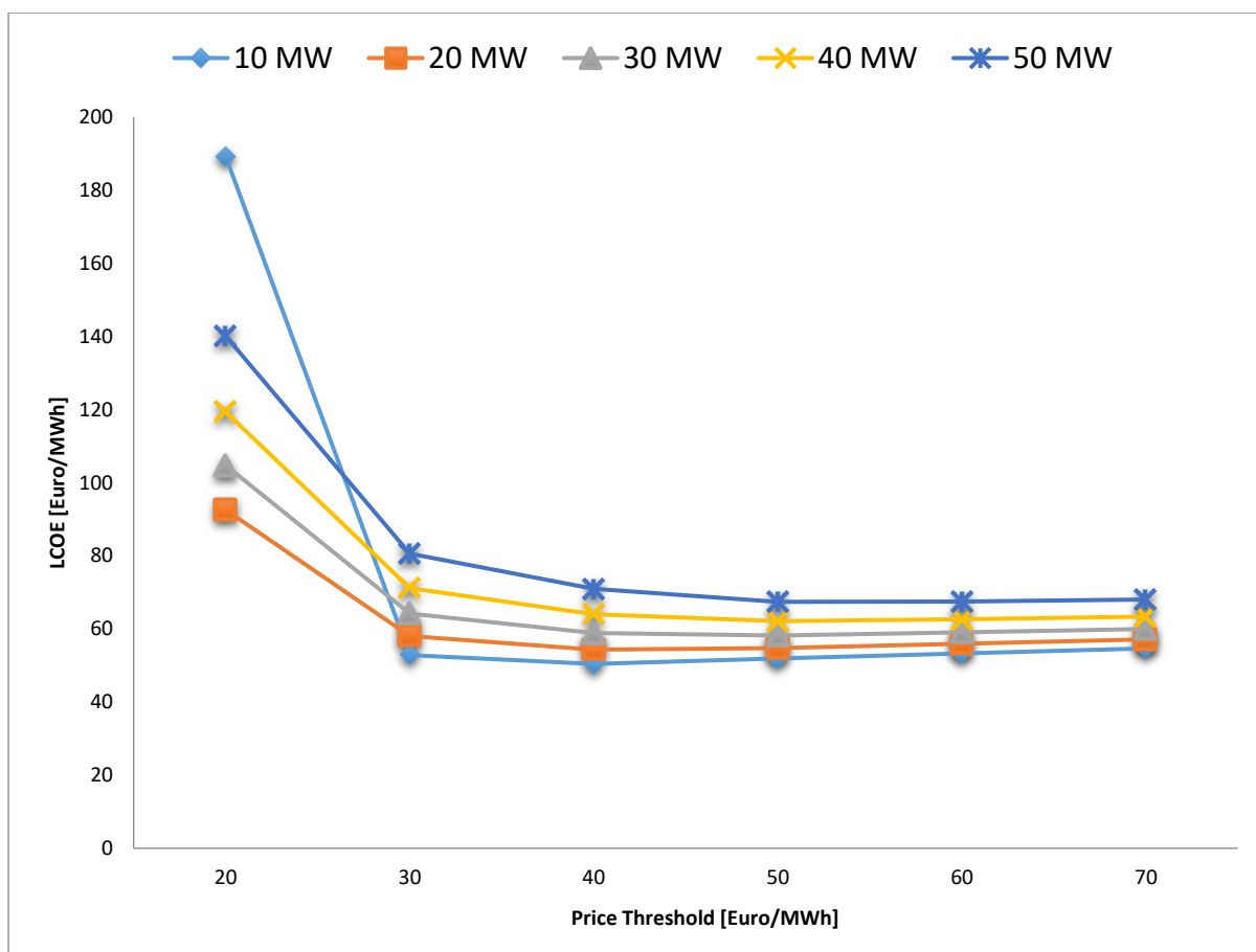
Figure 8.12 Levelized Cost of Energy depending on different energy market price threshold values in the 2030 Power-to-Gas Hydrogen pathway using alkaline electrolysis
