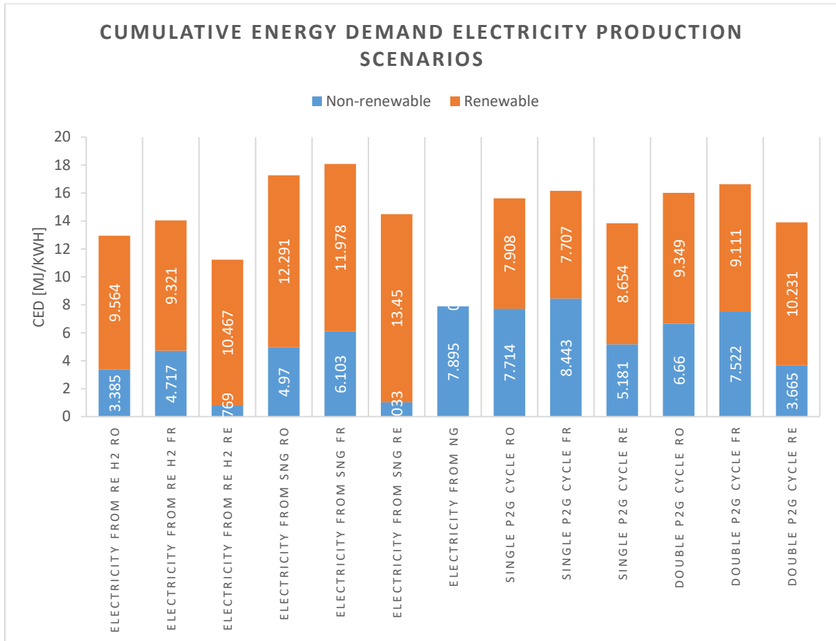
Figure 10.11 CED of electricity production scenarios
