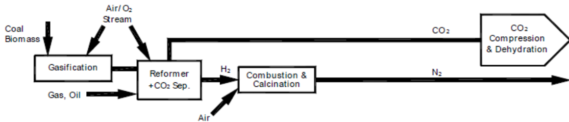
Figure 5.8 Pre-combustion carbon capture (Source: [International Energy Agency 2008])
