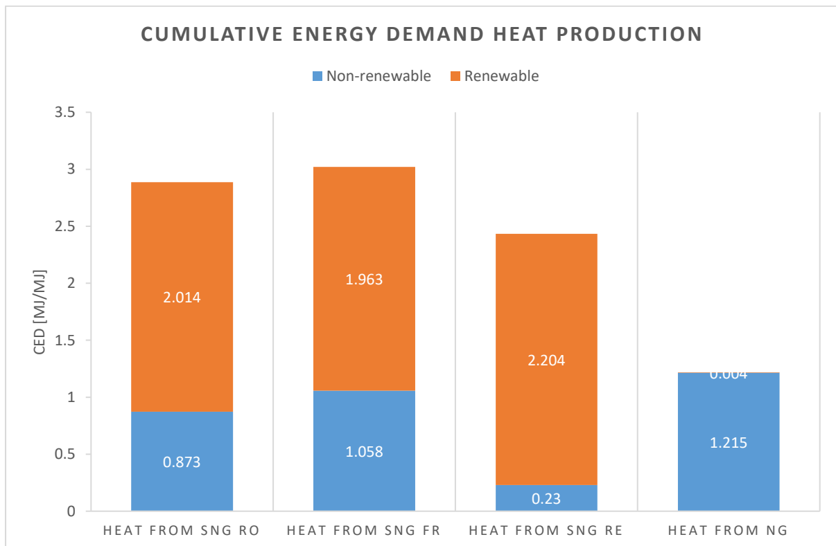
Figure 10.12 CED of heat production scenarios
