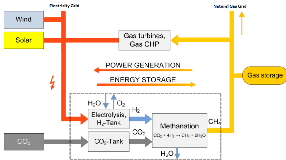
Figure 4.1 Le concept Power-to-Gas (source: [Sternier 2009])
