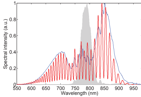
Figure 8.23 – Initial laser spectrum (shaded area). Combined pulse spectra (blue) and fringed spectrum (red) are registered for 2 bars Ne pressure.
