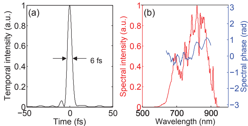
Figure 8.26 – Characterization of the combined pulse with a Wizzler-USP device: (a) temporal intensity and (b) spectral intensity and phase.
