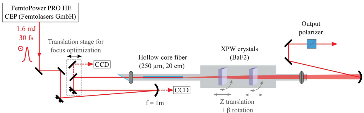
Figure 3.21 – XPW setup for contrast enhancement between the two CPA. The orientation of each crystal is defined by \beta , the angle between the input polarization direction (P) and the crystallographic axis of the crystal.
