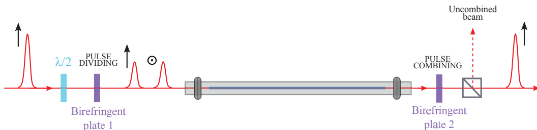
Figure 8.5 – Implementation of temporal pulse dividing in a 'One trip configuration' with two similar birefringent plates.
