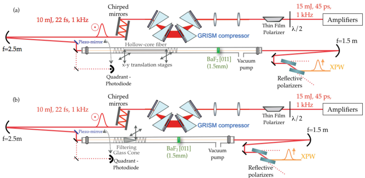
Figure 7.6 – Experimental implementation of high-energy XPW filtering, including a hollow-core fiber (a) or a glass cone filter (b).
