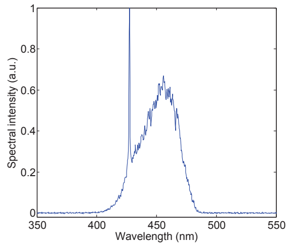
Figure 9.9 – Forward spectrum of air lasing recorded with a 2 cm focal length lens as a coupling optics in the spectrometer. A strong laser emission is noticed at 428 nm.
