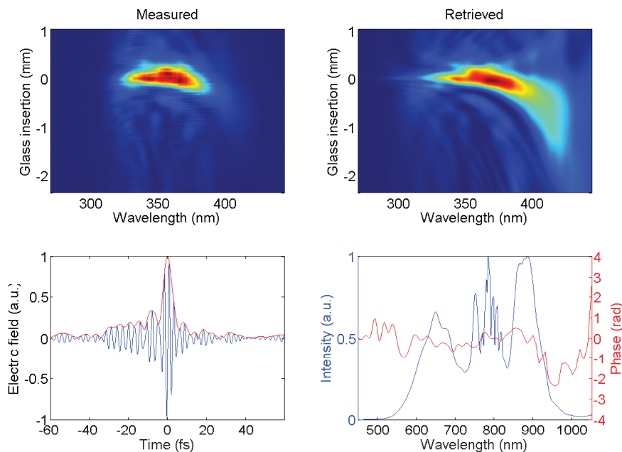
Figure 5.4 – D-scan measurement.
