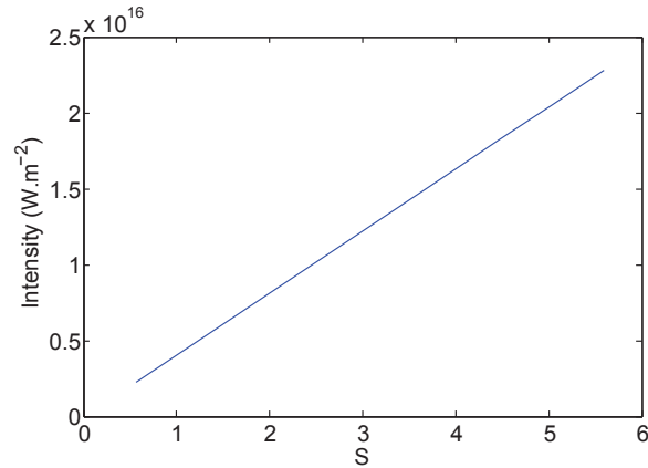
Figure 7.5 – Intensity on the XPW crystal as a function of S . This calculation is performed with a 25 fs input pulse with flat spectral phase and L = 1.5 mm.
