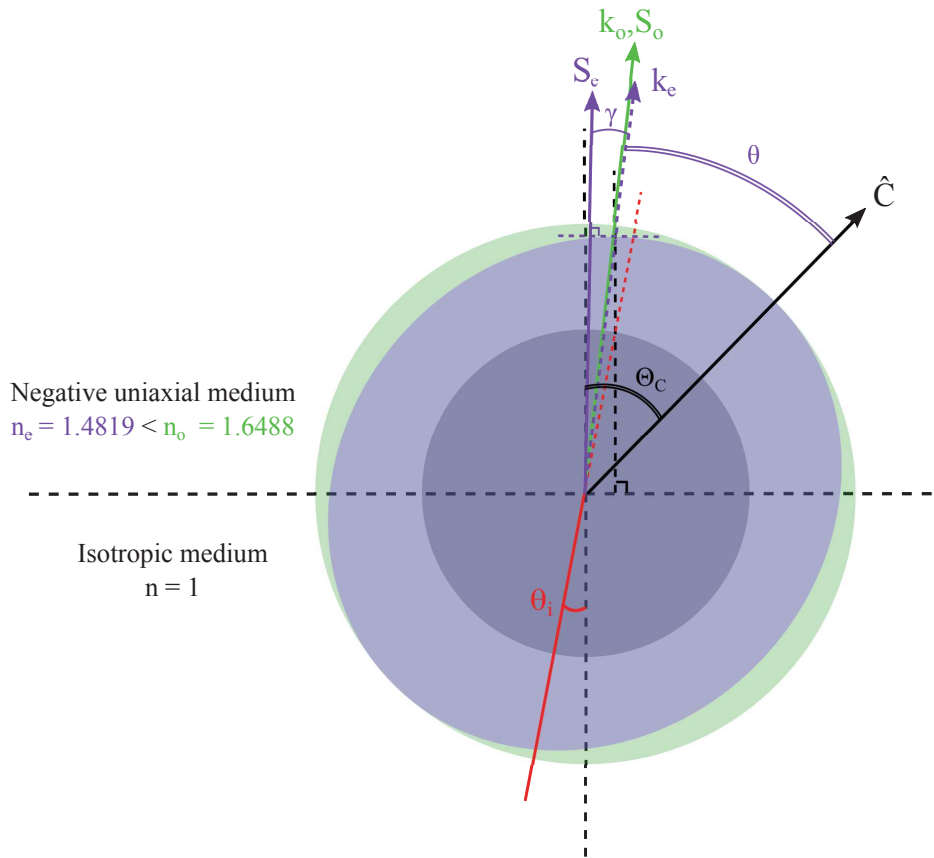
Figure 8.11 – Descartes diagram to scale for construction of refraction angles between an isotropic medium and a negative uniaxial medium. The S_e vector direction is normal to the tangent to the extraordinary indicatrix (purple) taken at the point of intersection with k_e
