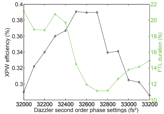
Figure 7.23 – XPW efficiency and FTL duration (1 single crystal) as a function of input chirp for 9.6 mJ input energy.
