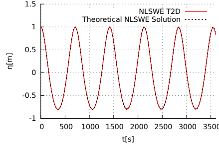
Figure 4.12: Parabolic basin – Temporal evolution of free surface elevation at the center of the basin. The thick black line is the analytical NLSWE solution. The red line represents numerical results issued of the NLSWE model of T2D. The L^2 -error on h was calculated by the BRGM, partners of the TANDEM project, for the different codes. The error for the the NLSWE model of Telemac2D is less than 1%, see Violeau [2015] .
