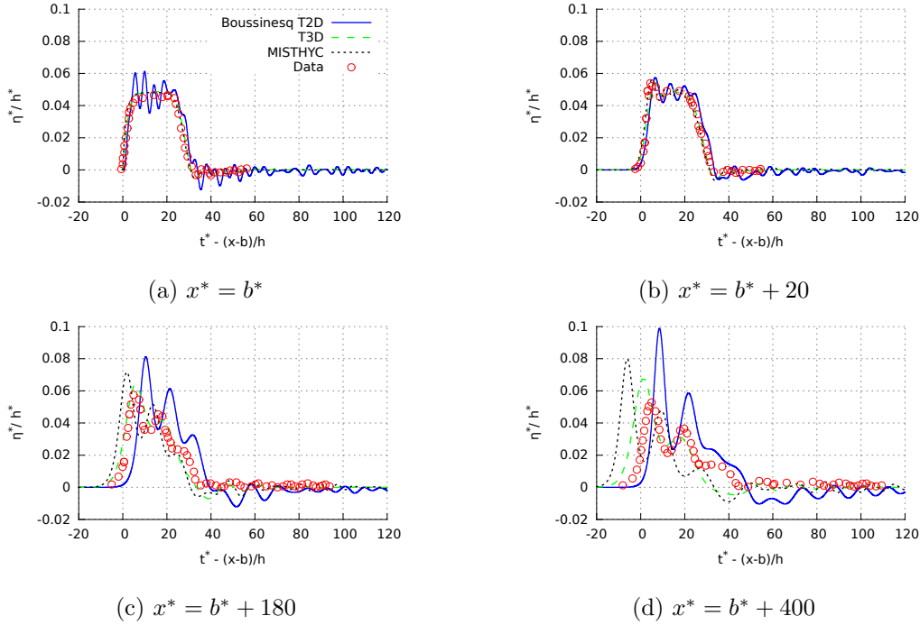
Figure 4.6: Generation and propagation from a moving bed – Temporal free surface deformation during the propagation of a wave initiated by an impulsive exponential motion ( b^* = 12 , \zeta_0^* = 0.1 , t_c^* = 0.148 ) at four places along the flume. The time is modified to fit the same scale. Same nomenclature as Figure 4.4.
