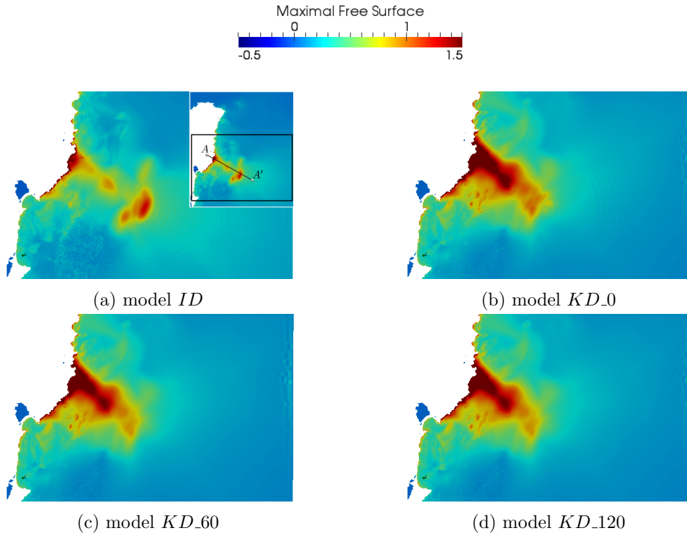
Figure 3.12: 1947 New Zealand event – Snapshots of the temporal maximal free surface elevation (in m) calculated during one hour with the NLSWE model of Telemac2D for the different generation models.
