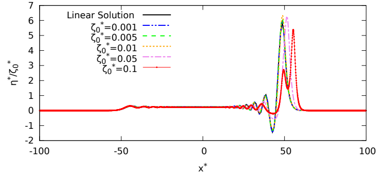
Figure 2.20: Deformation of the free surface at t^* = T^* and for v_p^* = 1 and \tau^* = 0 : comparison of the linear solution (black line) and non-linear numerical results. The coloured dashed lines represent the dimensionless non-linear numerical results for different increasing non-linearity levels: \zeta_0^* = 0.001, 0.005, 0.01, 0.1 .
