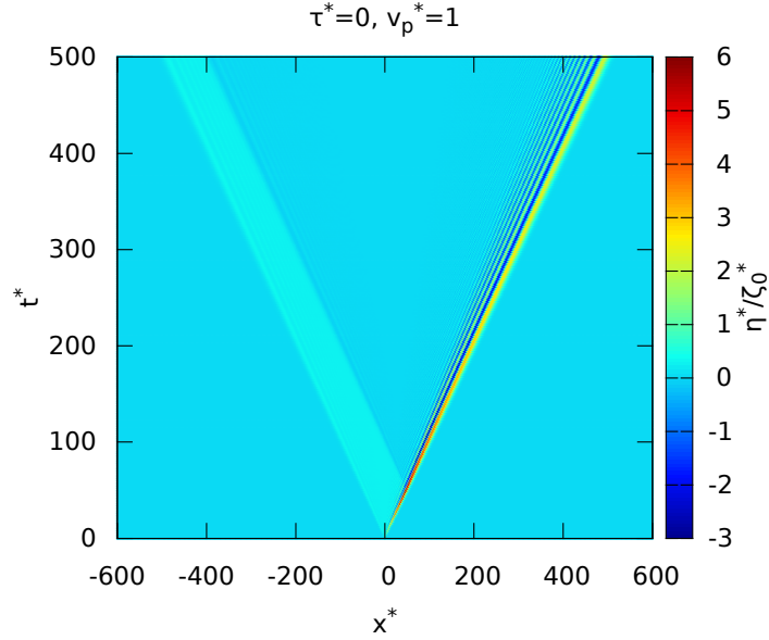
Figure 2.11: Evolution in space and time of the free surface deformation \eta^*/\zeta_0^* for v_p^* = 1 and \tau^* = 0 . The colour represents the wave amplitude.
