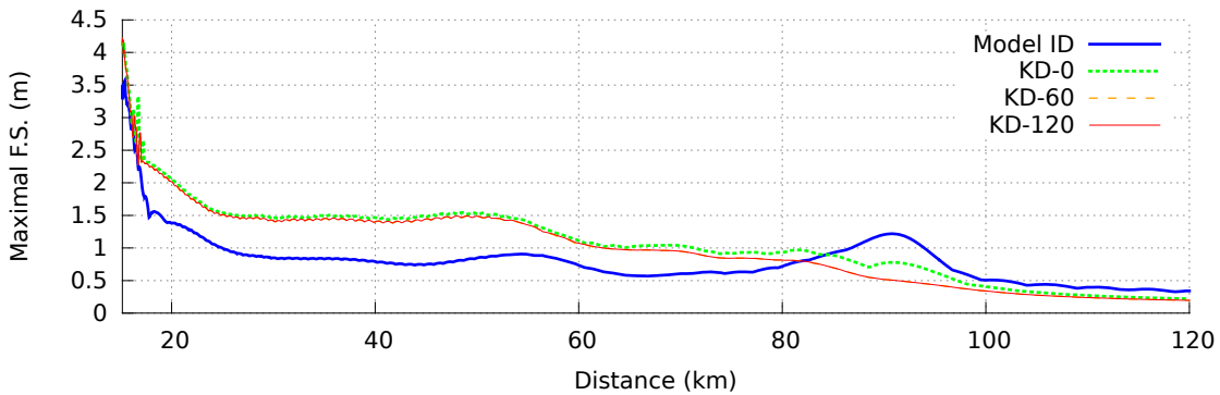
Figure 3.13: 1947 New Zealand – Maximal free surface elevations reached during the propagation along the transect A - A' as defined in Figure 3.12. Only result for negative bathymetry is plotted. The colourful lines are numerical results from the different generation models. The orange and red lines are superimposed, models KD_60 and KD_120 respectively.
