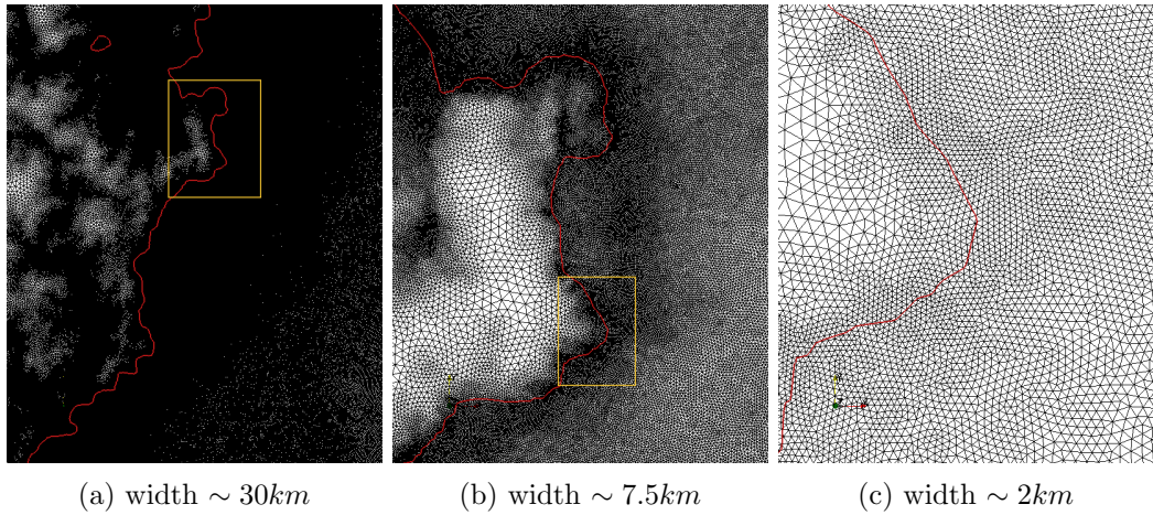
Figure 3.8: 1947 New Zealand event – Details of the mesh built for the event. The yellow boxes correspond to the boundary of the next zoom. The red line is the initial coast line.
