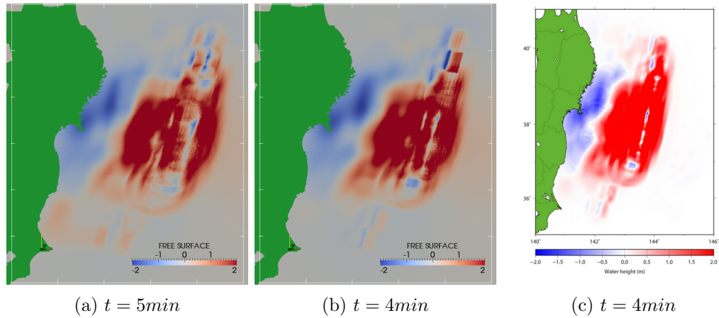
Figure 5.9: 2011 Tohoku-Oki event – Snapshots of the free surface deformation calculated from the source model of Satake et al. [2013] with Telemac2D at the end of the ground motion (5.9a) and at t = 4\text{min} (5.9b) in comparison with the free surface deformation obtained by Satake et al. at the same time (5.9c).
