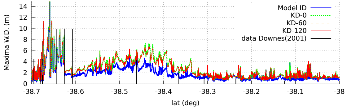
Figure 3.15: 1947 New Zealand event – Maximal water depth obtained at the coastline (black line in Figure 3.7a) during the event. The colourful lines represent the different generation models, and the black vertical bars the data of Downes and Stirling [2001] . The horizontal axis corresponds to the latitudes.
