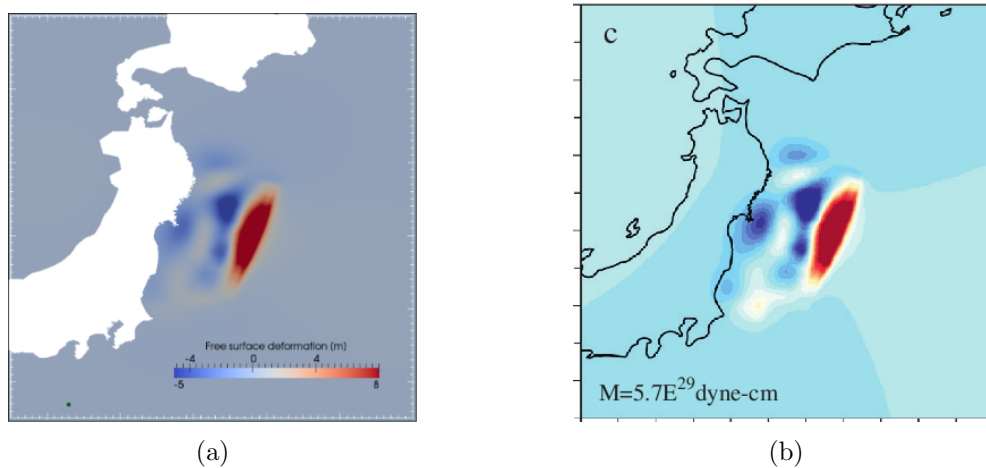
Figure 5.5: 2011 Tohoku-Oki event – Comparison of the initial free surface deformation (using the traditional way to generate tsunami) with the NLSWE model of Telemac2D (5.5a) and the seafloor deformation calculated by Chen et al. [2014] (5.5b). The scale is identical for both graphs.
