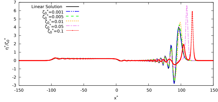
(a) t^* = 100
