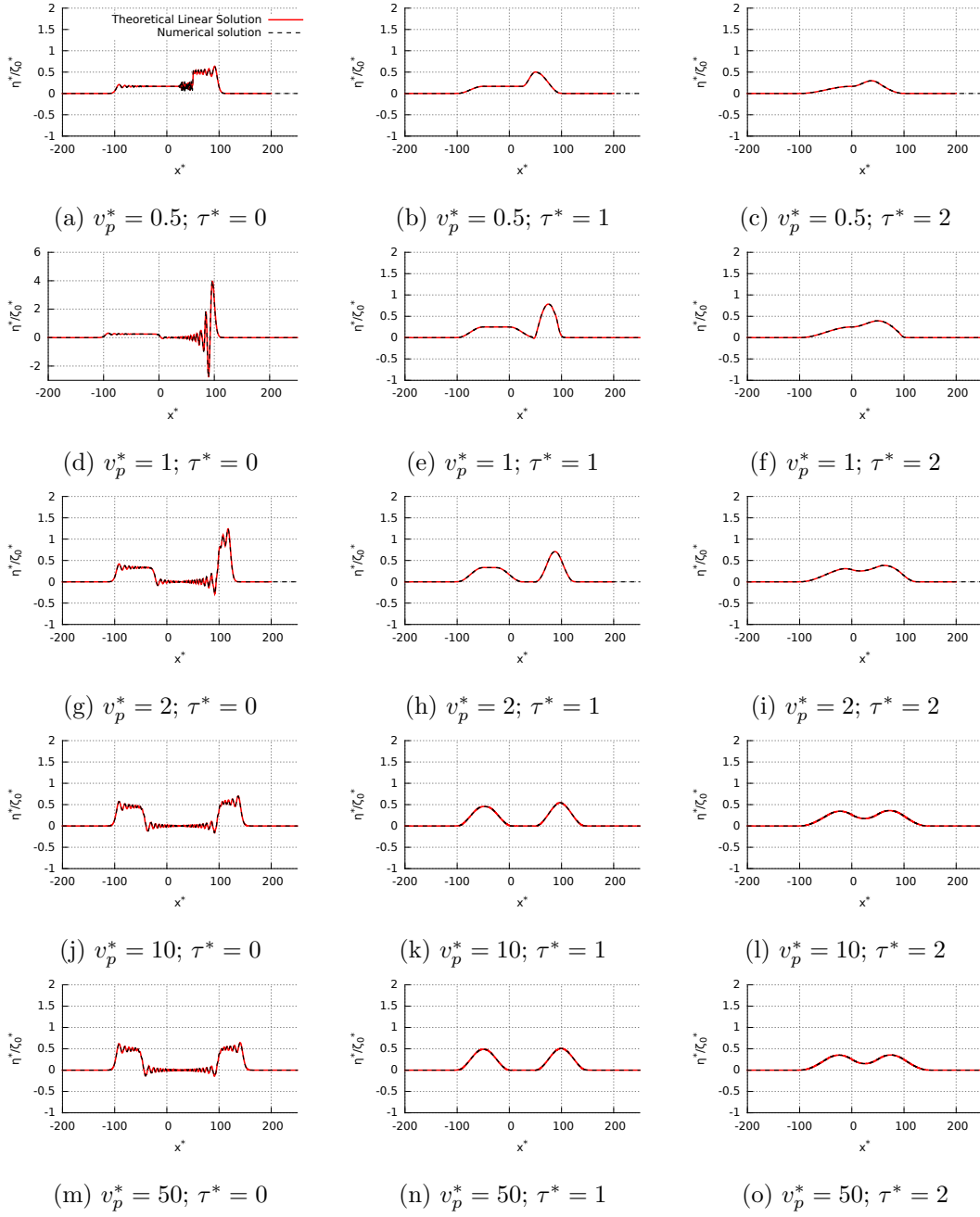
Figure 2.8: Free surface profiles at t^* = 100 for L^* = 50 and different values of v_p^* and \tau^* . Same legend as Figure 2.4.
