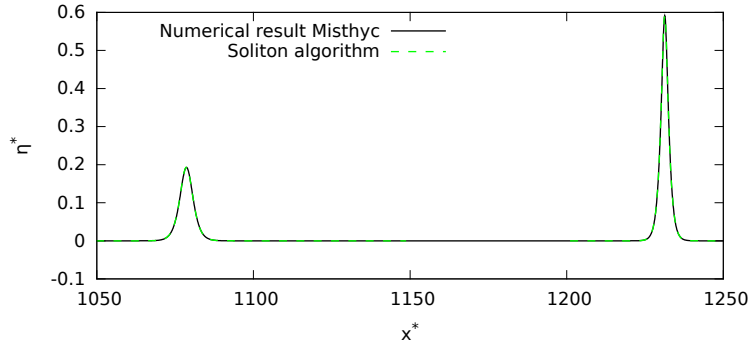
(a) \zeta_0^* = 0.05
