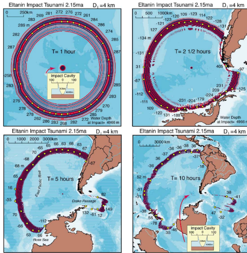
Figure 1.10: Cosmogenic tsunami – Numerical propagation of the tsunami generated by the impact of the Eltanin asteroid 2.15 Ma ago. The yellow dots show numerical tsunami heights. Work issued from Ward and Asphaug [2002] .
