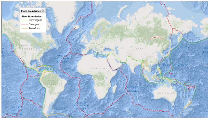
Figure 1.14: Seismic source – World map of the main faults between the tectonic plates available on the website of the NOAA. The red, green and yellow faults correspond to the divergent, convergent and transform motion of the plates respectively.
