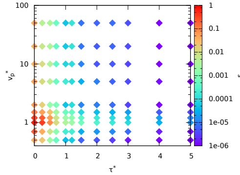
Figure 2.16: Energy ratio \varepsilon = \frac{E_l}{E_t} , at t^* = T^* as a function of v_p^* and \tau^* .
