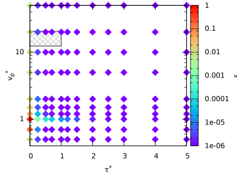
Figure 5.20: 2011 Tohoku-Oki event – Potential energy ratio \varepsilon at t^* = T^* for L^* = 267 . The striped grey zone shows the possible parameter values for the Tohoku, 2011 event.
