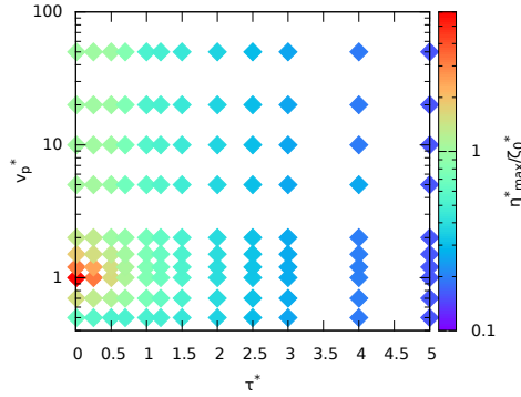
Figure 2.18: The maximum free surface amplitude ( \eta_{max}^*/\zeta_0^* ) calculated with the non-linear numerical model as function of v_p^* and \tau^* for L^* = 50 and \zeta_0 = 0.001 at t^* = T^* (colour in log scale).
