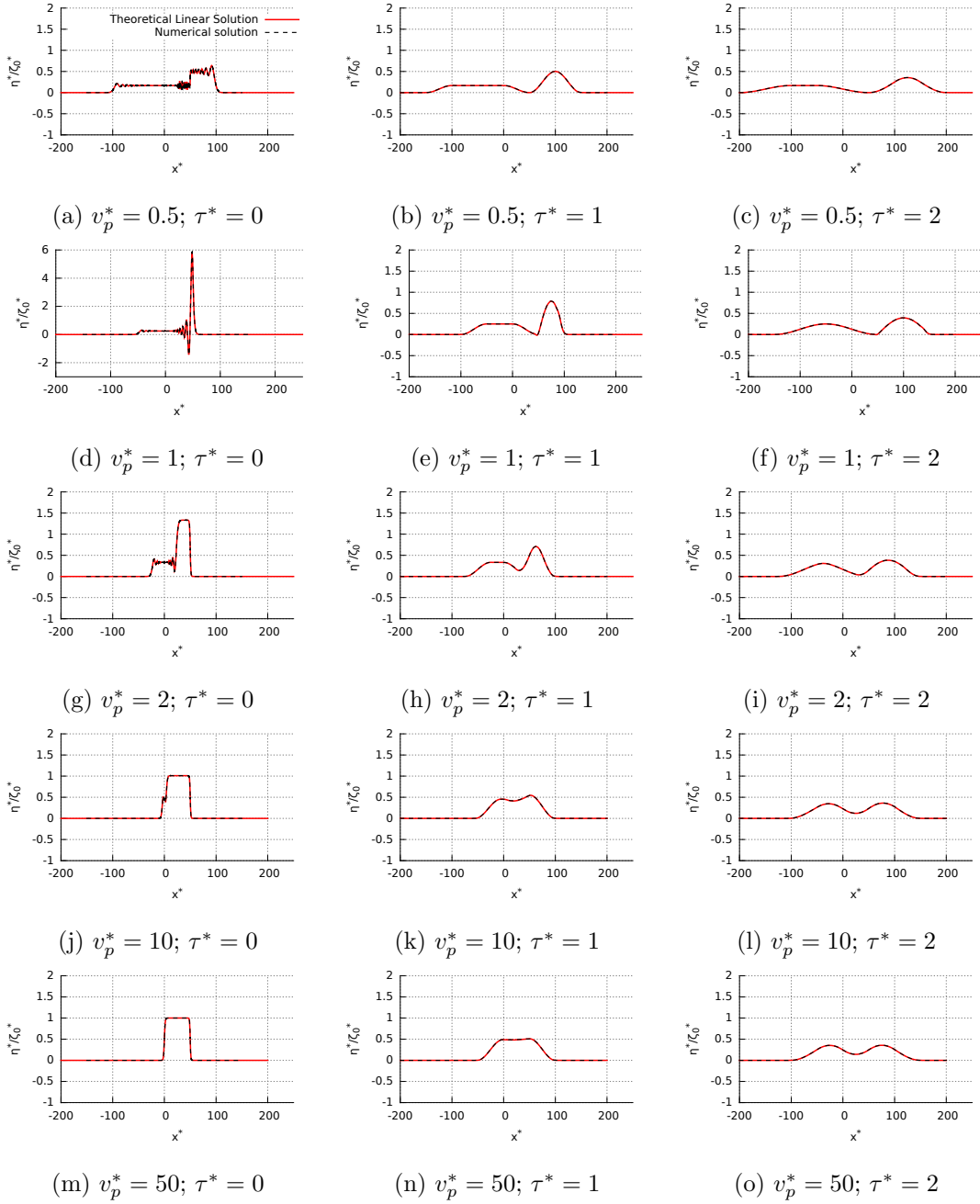
Figure 2.4: Free surface profiles at t^* = T^* for L^* = 50 and different values of v_p^* and \tau^* ( v_p^* increases from top to bottom and \tau^* increases from left to right). The red line is the linear solution 2.21-2.23, and the dashed black line is the numerical simulation results from the linear version of the Misthyc code (see section 2.3.3). The vertical scale of graph (d) for v_p^* = 1 and \tau^* = 0 differs from the others for clarity.
