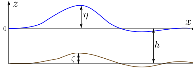
Figure 2.1: Definition of the fluid domain and coordinate system (x, z) , with h the initial depth, \zeta(x, t) the deformation of the sea floor and \eta(x, t) the deformation of the free surface.
