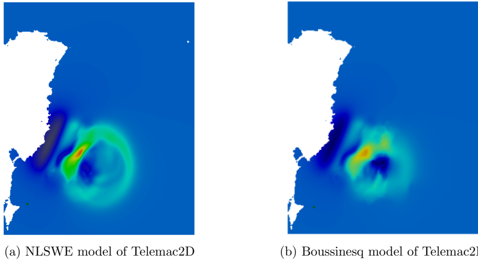
Figure 3.17: 1947 New Zealand event – Free surface deformation (in m) at the end of the sea floor motion, t = 190s , obtained with the NLSWE and the Boussinesq models of Telemac2D for v_p = 300m/s and t_r = 0s . Same scale as Figure 3.9.
