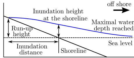
Figure 3.14: 1947 New Zealand event – Definition of the different measures during a run-up. The data given by Downes and Stirling [2001] corresponds to run-up heights. The height measured in the numerical models is the inundation height at the shoreline. The blue line corresponds to the temporal maximal free surface elevation reached during the event.
