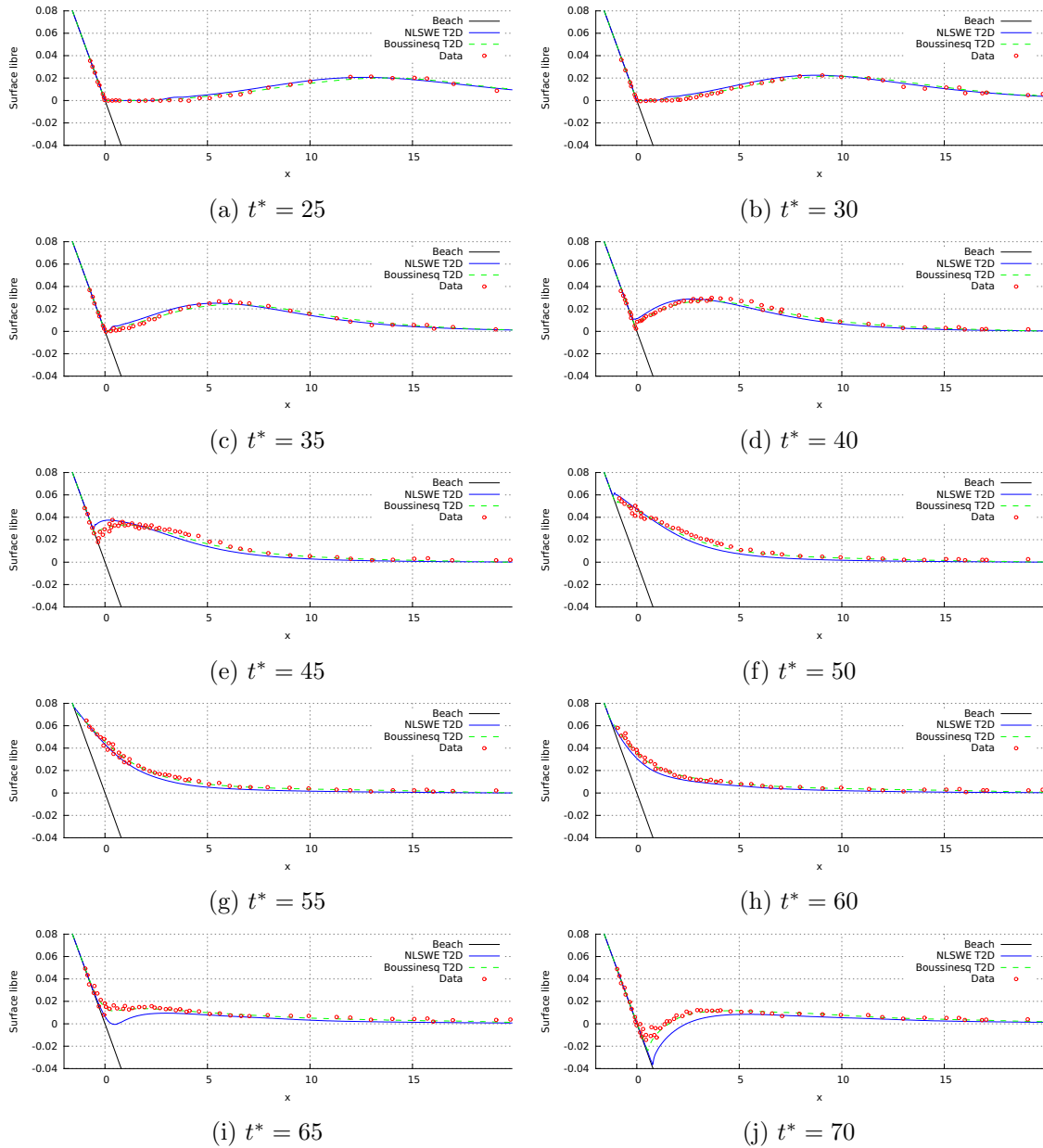
Figure 4.19: Run-up of a solitary wave on a uniform beach – Spatial free surface deformation profiles at different instants. Same nomenclature as Figure 4.18.
