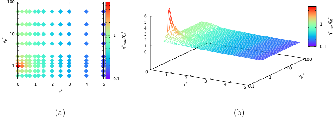
Figure 2.6: The maximum free surface amplitude, \eta_{max}^*/\zeta_0^* as function of v_p^* and \tau^* for L^* = 50 at t^* = T^* (colour in log scale). Figure 2.6a represents the original values while Figure 2.6b is an interpolation using a weighted average of the data.
