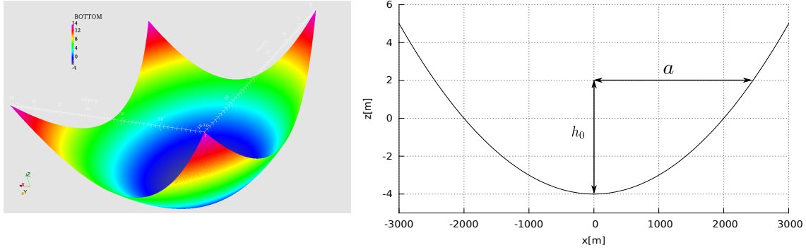
Figure 4.10: Parabolic basin – Geometry of the perfect paraboloid basin.
