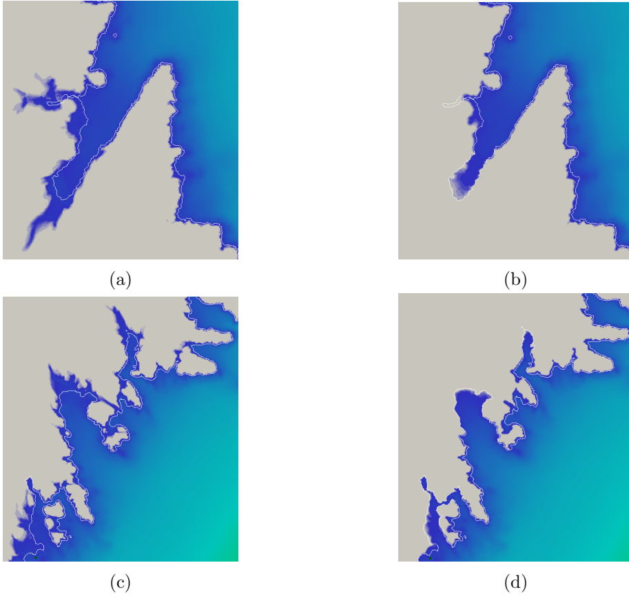
Figure 5.19: 2011 Tohoku-Oki event – Snapshots of the flooded area obtained in the North and South areas of the Iwate bay by the NLSWE model of Telemac2D without and with friction bottom, Figures 5.19a, 5.19c and Figures 5.19b, 5.19d, respectively. The friction law is the Strickler law with a coefficient of 30m^{1/3}/s . The white line is the initial coastline.
