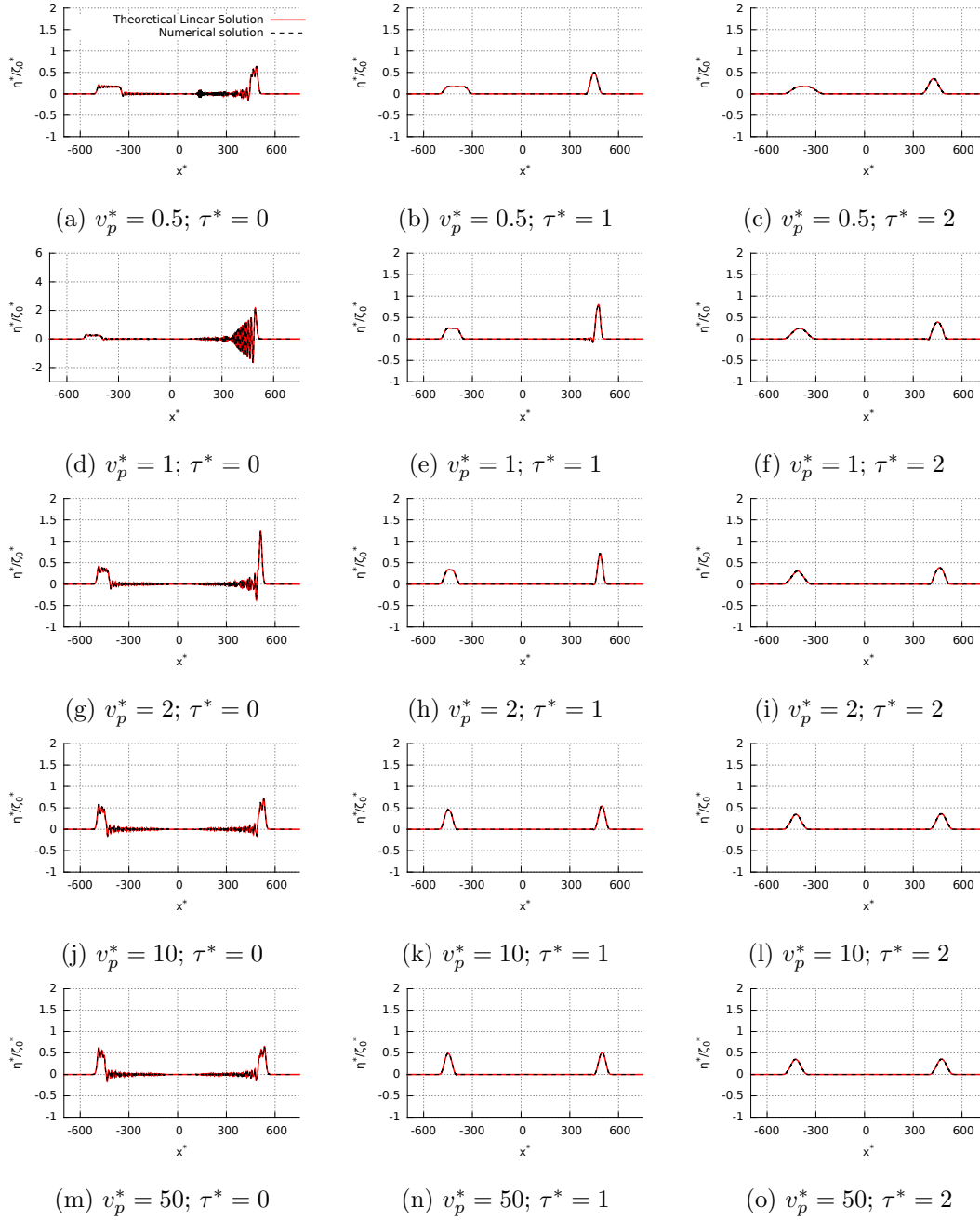
Figure 2.9: Free surface profiles at t^* = 500 for L^* = 50 and different values of v_p^* and \tau^* . Same legend as Figure 2.4.
