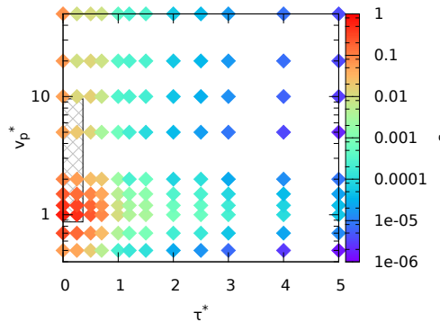
Figure 3.16: 1947 New Zealand event – Energetic ratio \varepsilon for L^* = 35 at t^* = T^* . Grey zone represents the ranges of values of the temporal parameters \tau^* and v_p^* for the New Zealand 1947 event (see Table 3.2).
