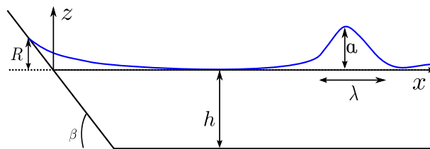
Figure 1.12: Run-up – Geometry and parameters of the model.
