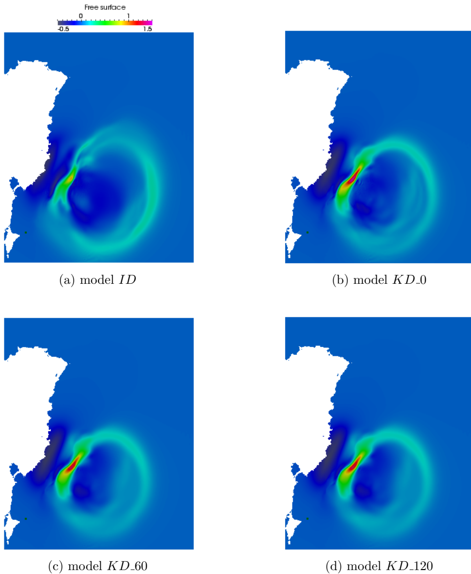
Figure 3.10: 1947 New Zealand event – Free surface deformation (in m) for the four generation models calculated with the NLSWE model of Telemac2D at t = 310s .
