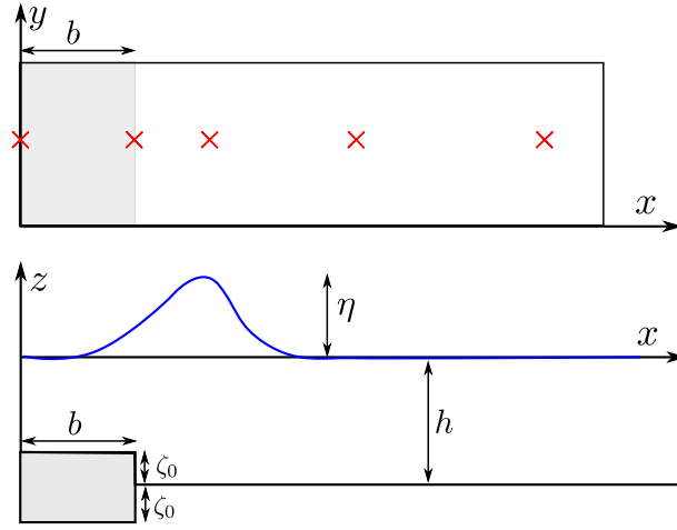
Figure 4.3: Generation and propagation from a moving bed – Geometry of the experiment of Hammack [1973], not at scale. The top frame is a top view and the bottom frame is a slice view. The gray zone is the moving area of length b . The red crosses are locations of measurement gauges.
