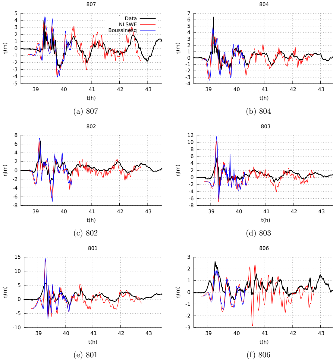
Figure 5.21: 2011 Tohoku-Oki event – Comparisons between measurements and numerical results of the free surface deformation. The black thick line is the data. The red and blue lines are the result from the NLSWE and Boussinesq models of Telemac2D, respectively. The source is the one from the model of Shao et al. [2011] .
