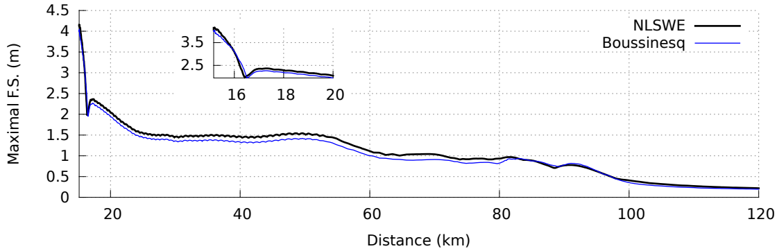
Figure 3.19: 1947 New Zealand event – Maximal free surface elevations reached during the propagation along the transect A - A' as defined in Figure 3.12. Only result in the ocean part is plotted. The black and blue lines are the numerical results from the NLSWE and the Boussinesq models of Telemac2D, respectively. The model generation corresponds to KD_0 . The encapsulated figure is a zoom of the global curve near the coastline (distance \in [15; 20]km ).
