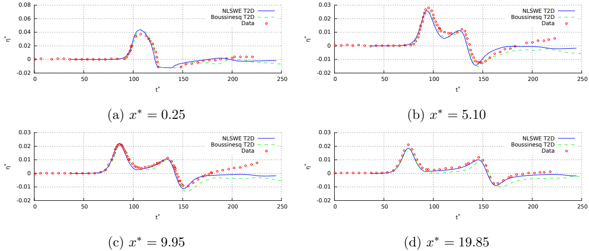
Figure 4.18: Run-up of a solitary wave on a uniform beach – Temporal free surface deformation for the solitary wave run-up on a plane beach at different places on the slope. The blue line is the numerical result from the NLSWE Telemac2D model. The dashed green line is the numerical result from the Boussinesq Telemac2D model. The red symbols are the data from Synolakis [1987].
