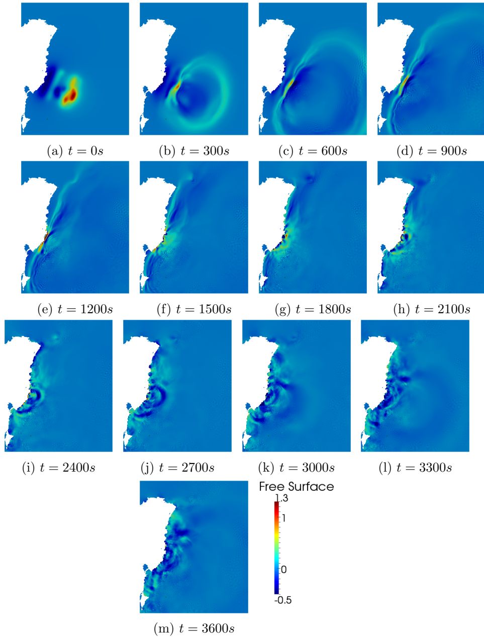
Figure 3.11: 1947 New Zealand event – Snapshots of the free surface (in m) every 5 min. during the numerical propagation of the wave generated by an instantaneous sea floor deformation (model ID ) with the NLSWE model of Telemac2D.
