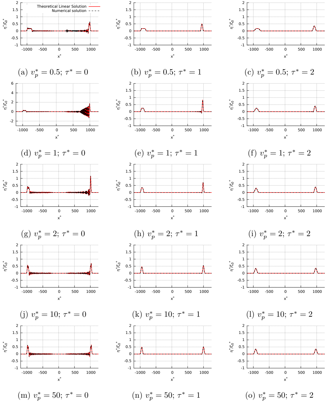
Figure 2.10: Free surface profiles at t^* = 1000 for L^* = 50 and different values of v_p^* and \tau^* . Same legend as Figure 2.4.
