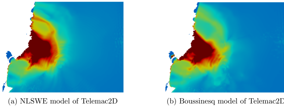
Figure 3.23: 1947 New Zealand event – Same nomenclature as Figure 3.18 for v_p = 150\text{m/s} and t_r = 0\text{s} . (Free surface deformation in m.)
