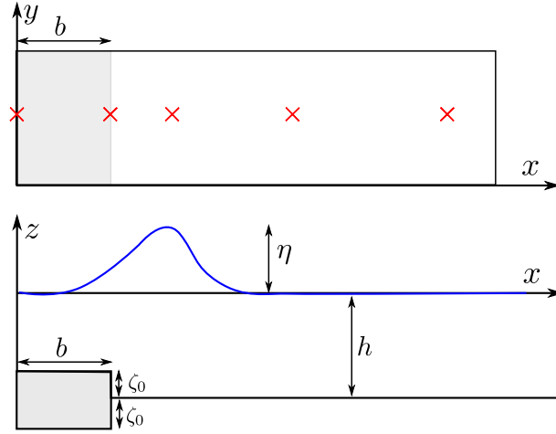
Figure 1.18: Kinematic generation – Geometry of the experiment of Hammack [1973], not at scale. The top frame is a top view and the bottom frame is a side view. The gray zone is the moving area of length b . The red crosses are locations of measurement gauges.
