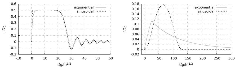
Figure 1.19: Kinematic generation – Free surface elevation comparison at \frac{x}{h} = \frac{b}{h} between the exponential and the sinusoidal time history deformation for an impulsive motion (left) and a creeping motion (right). The geometrical parameters are: b/h = 12.2 , \zeta_0/h = 0.2 , t_r \sqrt{gh}/b = 0.069 for the impulsive motion and t_r \sqrt{gh}/b = 106.14 for the creeping motion. The figure is adapted from the work of Hammack [1973].
