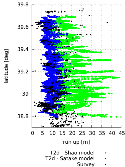
Figure 5.15: 2011 Tohoku-Oki event – Comparison between the inundation heights obtained by the numerical models and the survey measurements at the Iwate Bay. The black dots are data from the 2011 Tohoku Earthquake Tsunami Joint Survey Group, release 20120330, http://www.coastal.jp/ttjt/ , the blue dots are numerical result from Telemac2D with the generation from Satake et al. [2013] and the green dots numerical results with the generation from Shao et al. [2011].
