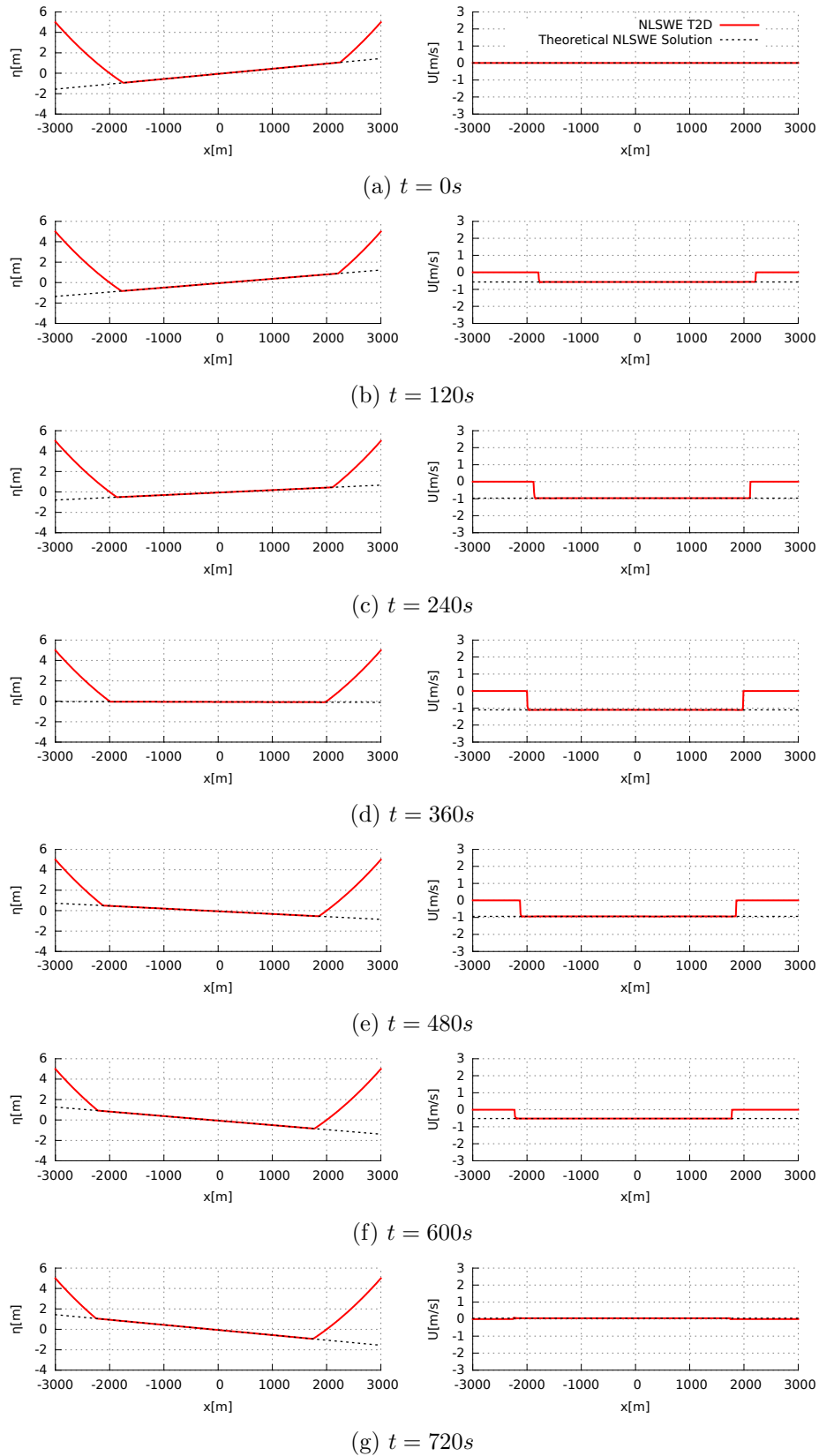
Figure 4.13: Parabolic basin – Initial flat configuration. Same nomenclature as Figure 4.11.
