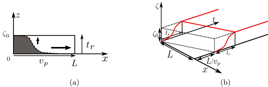
Figure 2.2: Definition of the sea floor uplift \zeta(x, t) : 2.2a spatial profile of the sea floor and 2.2b, the black dashed lines represent the motion defined by Todorovska and Trifunac [2001], and the solid red lines are the motion used in this study.
