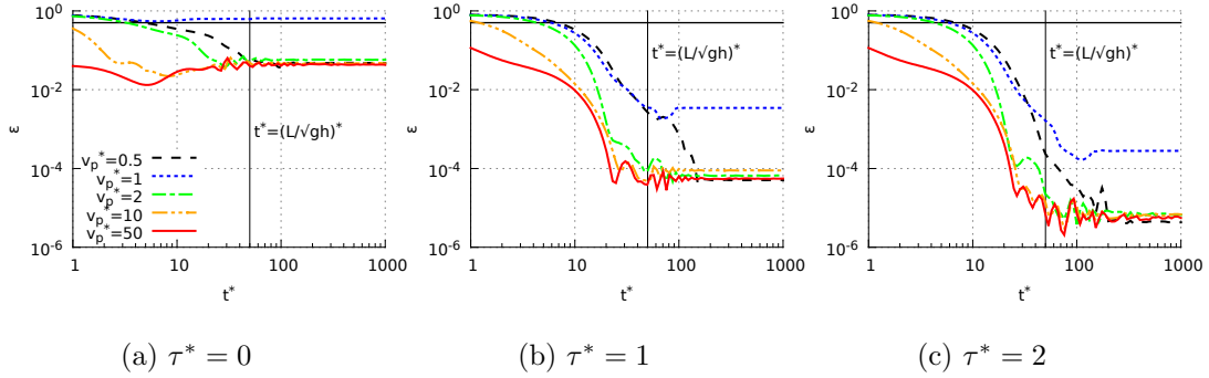
Figure 2.17: Time profiles of the energy ratio \varepsilon = \frac{E_l}{E_t} for different values of \tau^* and v_p^* . The horizontal black line represents \varepsilon = 0.5 . The vertical black line is at t^* = (L/\sqrt{gh})^* .
