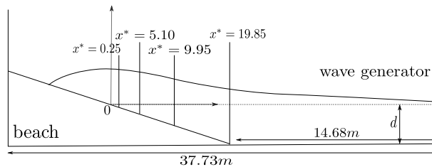
Figure 4.16: Run-up of a solitary wave on a uniform beach – Set up of the experiment of Synolakis [1987] . Not at scale.
