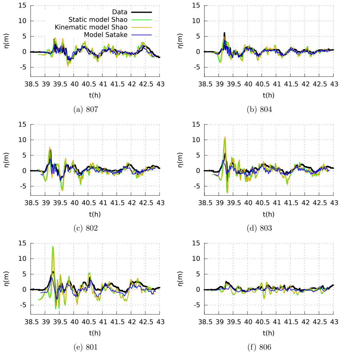
Figure 5.12: 2011 Tohoku-Oki event – Comparisons between measurements from GPS gauges and numerical results of the free surface deformation. The black thick line is the data. The blue line is Telemac2D result from Satake et al. [2013] source. The orange and the green lines are respectively the Telemac2D results from the kinematic and static Shao et al. [2011] sources.
