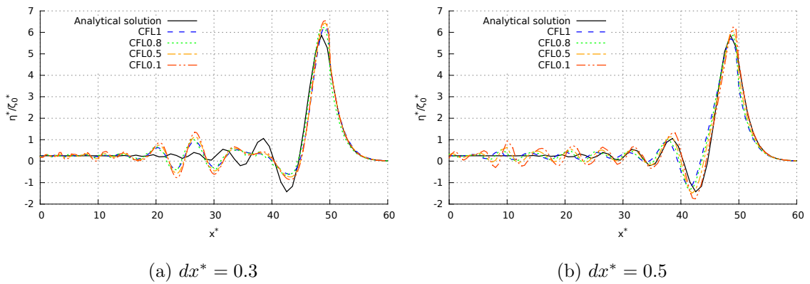
Figure 3.4: Resonance phenomenon simulated with Telemac2D and Boussinesq model – Spatial profiles of the free surface deformation at the end of the ground motion ( t^* = T^* ) for dx^* = 0.3 and dx^* = 0.5 meshes. The black line is the analytical free surface calculated from the linear theory. The coloured dashed curves are the different values of the CFL .
