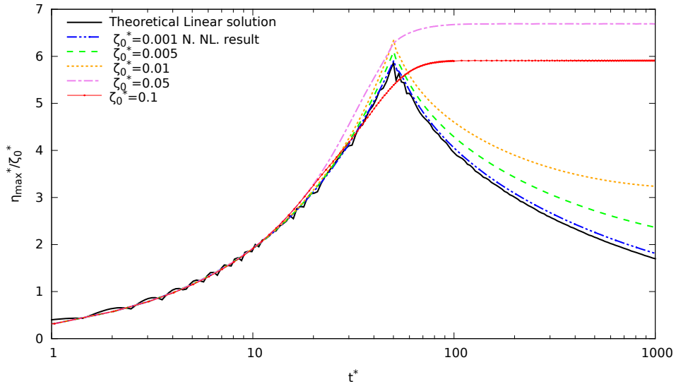
Figure 2.21: Temporal profiles of \eta_{max}^*/\zeta_0^* for v_p^* = 1 , \tau^* = 0 and L^* = 50 . The solid black line is the theoretical linear solution. The coloured dashed lines are non-linear numerical results from Misthyc for \zeta_0^* = 0.001, 0.005, 0.01 and 0.1.
