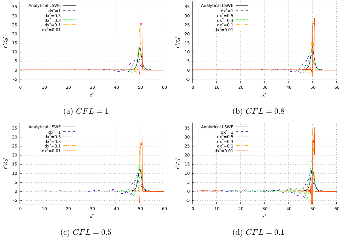
Figure 3.1: Resonance phenomenon simulated with Telemac2D and NLSWE – Spatial profiles of the free surface deformation at the end of the ground motion ( t^* = T^* with an accuracy of dt^* ) for different values of CFL and dx^* . The black line is the analytical free surface calculated from the LSWE theory. The coloured dashed curves represent numerical free surface profiles calculated with the different meshes.
