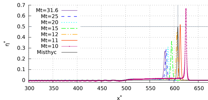
Figure 4.7: Propagation of a solitary wave – Spatial profiles of free surface deformation obtained with Telemac3D after t^* = 500 of propagation of a \frac{H}{h} = 0.5 high solitary wave for different values of CFL = \frac{M_t}{M_x} with M_x = 5 . The horizontal and vertical lines show the expected wave height and mean position, respectively.
