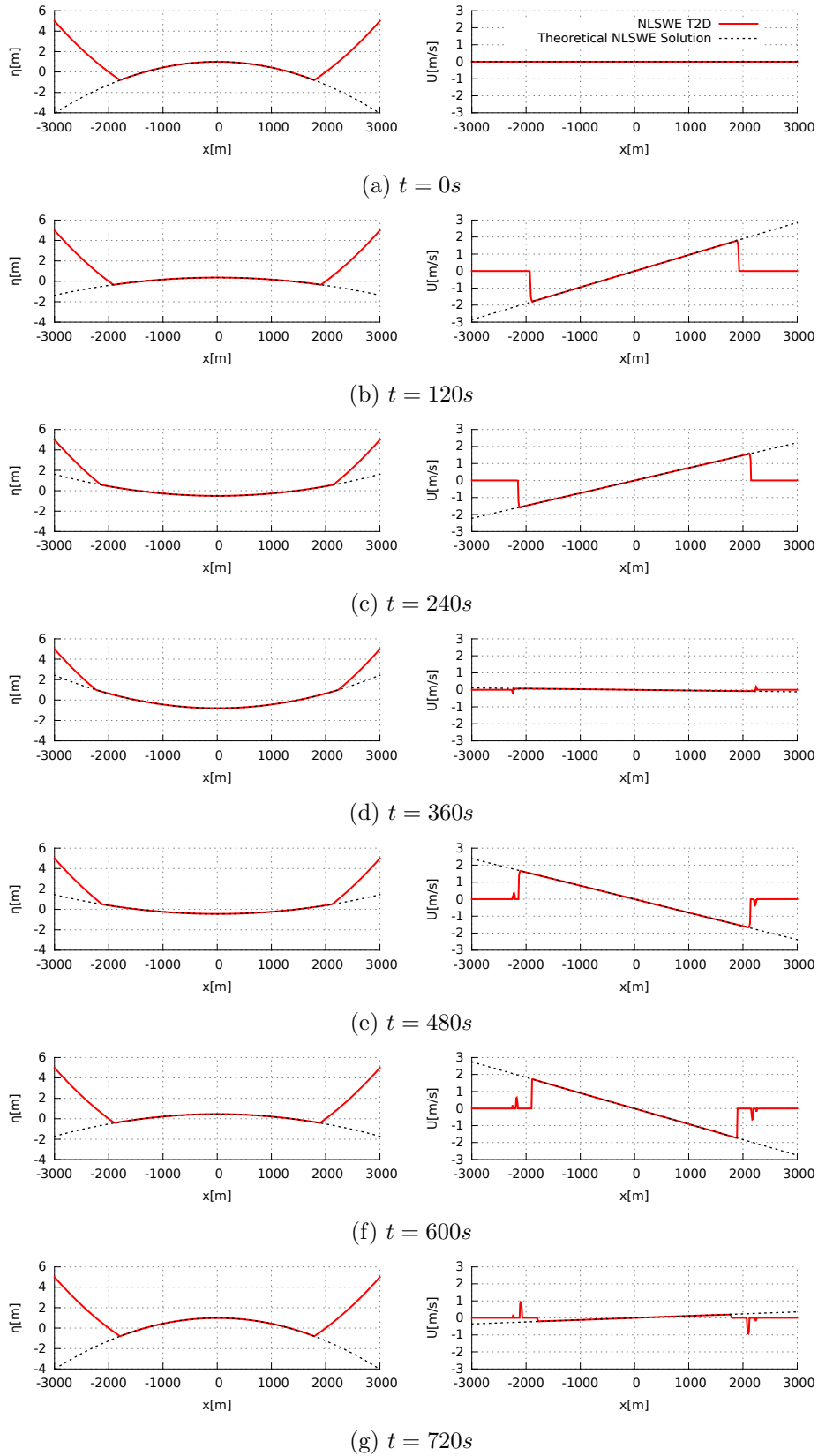
Figure 4.11: Parabolic basin – Initial paraboloid configuration. Spatial profiles on the slice y = 0 of the free surface deformation and of the horizontal velocity during one period. The dashed black line is the analytical NLSWE solution. The red line represents numerical results issued from the NLSWE model of T2D.
