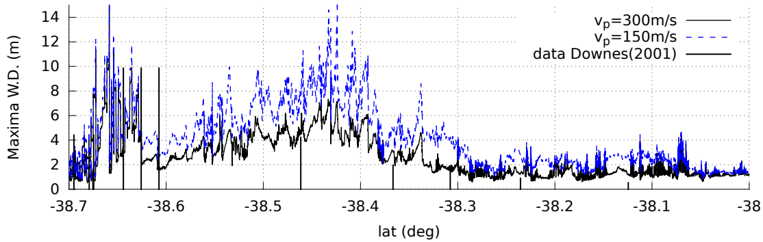
Figure 3.25: 1947 New Zealand event – Maximal water depth obtained at the coastline during the event. The black and blue lines represent numerical model issued of the generation with v_p = 300m/s and v_p = 150m/s respectively. The black vertical bars the data of Downes and Stirling [2001]. The horizontal axis corresponds to the latitude.
