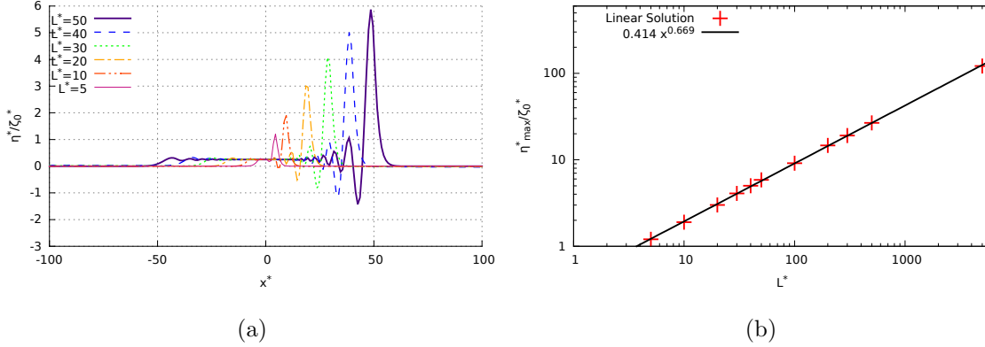
Figure 2.7: Impact of the deformation length L^* for v_p^* = 1 and \tau^* = 0 at the end of the generation. 2.7a Spatial profiles of the free surface for different values of L^* . 2.7b Red crosses represent the \eta_{max}^*/\zeta_0^* of the linear solution and the black line is the trend line 0.414(L^*)^{0.669} .
