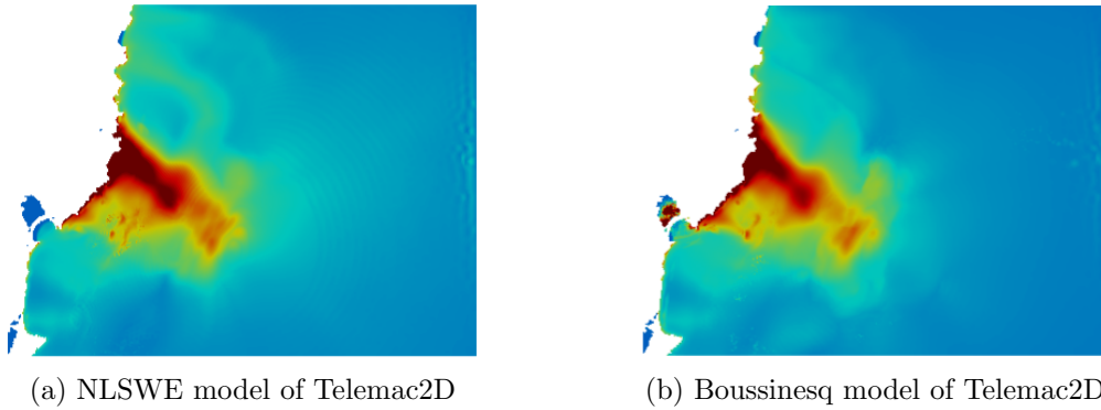
Figure 3.18: 1947 New Zealand event – Snapshots of the temporal maximal free surface elevation (in m) calculated during one hour obtained with the NLSWE and the Boussinesq models of Telemac2D for v_p = 300m/s and t_r = 0s . Same scale as Figure 3.12.
