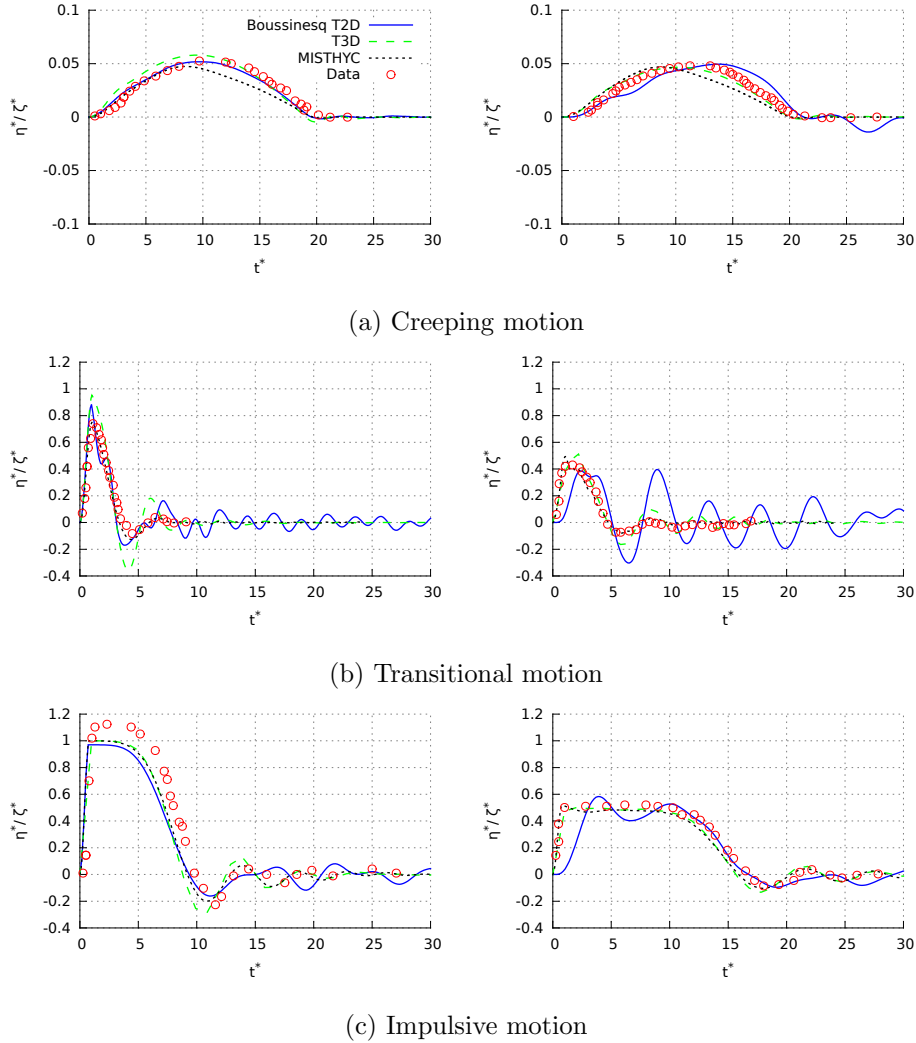
Figure 4.5: Generation and propagation from a moving bed – Temporal free surface profiles during the generation at x^* = 0 (left) and x^* = b^* (right) for a sinusoidal motion. Same nomenclature as Figure 4.4.
