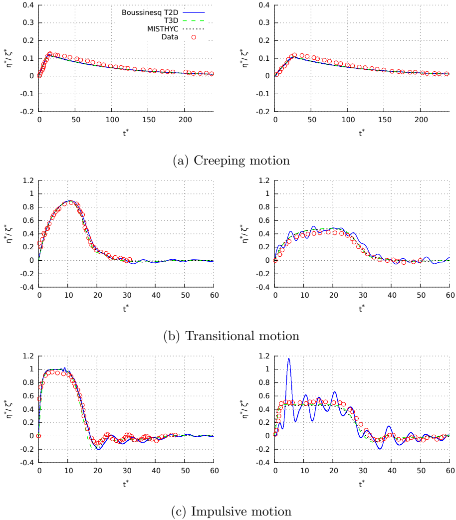
Figure 4.4: Generation and propagation from a moving bed – Temporal free surface profiles during the generation at x^* = 0 (left) and x^* = b^* (right) for an exponential motion. The blue lines are the numerical Boussinesq model of Telemac2D while Telemac3D is represented by the green dashed line. The numerical results issued from the code MISTHYC are also plotted (black dashed line), Benoit et al. [2014] . The red points are measurements from Hammack [1973] .
