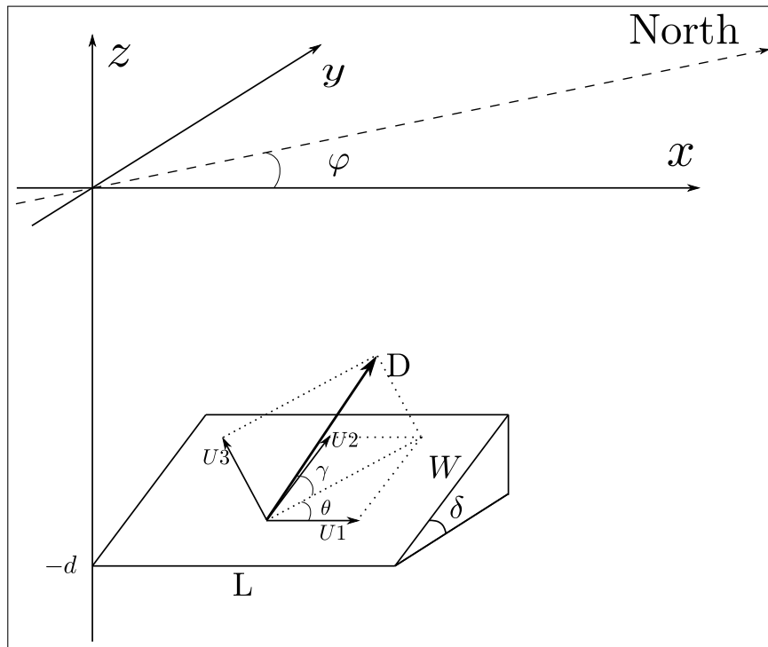
Figure 1.16: Seismic tsunami source – Definition of the geometrical parameters of the fault for the Okada method.
