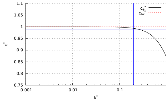
Figure 2.14: Wave celerities (adimensionalised by \sqrt{gh} ) from the general and the long wave theories, c_e^* , in black thick line, and c_{lw}^* , in dashed red line, respectively. The blue vertical line corresponds to k^* = 0.2 and the horizontal one to c^* = 0.99 . The horizontal axis is in log scale.
