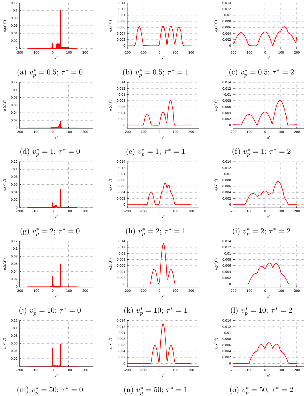
Figure 2.13: Spatial relative error of the numerical free surface issued from Misthyc at t^* = T^* for L^* = 50 and different values of v_p^* and \tau^* .
