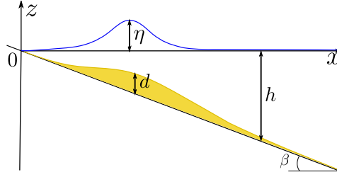
Figure 4.1: 1D analytical sliding mass – Geometry of the generation of a wave by a landslide. The coloured area represents the moving layer of the ground while the black line is the fixed bed.
