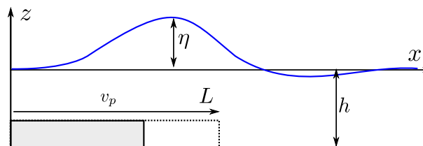
Figure 1.20: Kinematic generation – Geometry of the domain considered by Todorovska and Trifunac [2001] at a time smaller than the generation duration. The solid line is the instant deformation (propagation at velocity v_p ) while the dashed line is the final deformation. The graph is a vertical cut of their 2D domain.
