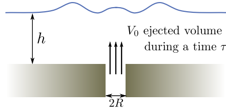
Figure 1.5: Volcanic tsunami generation – Schematising of the tsunami generation by a discharge into water of a large volume of matter. Adapted from Levin and Nosov [2009] .
