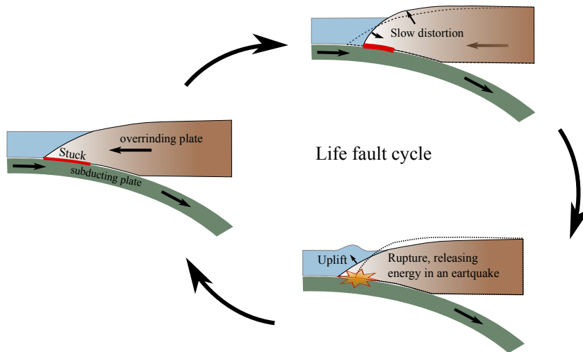
Figure 1.15: Seismic source – Life cycle of a convergent fault with generation of tsunamis.
