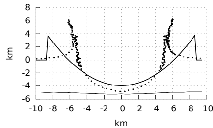
Figure 1.9: Cosmogenic tsunami – Comparison between the idealized impact cavity 1.4 (solid line) and numerical simulation of Ward and Asphaug [2003] at t = 25s (dot line). The thin line is the sea ground. Graph adapted from Levin and Nosov [2009].
