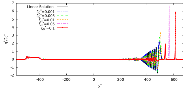
(a) t^* = 100
