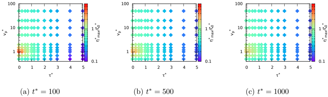
Figure 2.12: Maximum free surface amplitude \eta_{max}^*/\zeta_0^* as a function of v_p^* and \tau^* for L^* = 50 at different times t^* .
