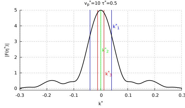
Figure 2.3: An example of the free surface Fourier transform \tilde{\eta}^* with critical k^* for v_p^* = 10 and \tau^* = 0.5 at t^* = T^* = \frac{L^*}{v_p^*} + t_r^* . The black line is the modulus of the Fourier transform |\tilde{\eta}^*| . The vertical blue, green and red lines represent the locations of the singularities k_1^* , k_2^* , k_3^* , respectively.
