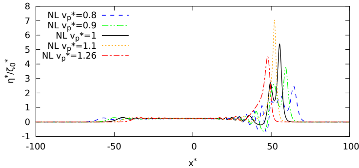
Figure 2.19: Free surface profiles from non-linear numerical results Misthyc, for \zeta_0^* = 0.1 for v_p^* = 0.8, 0.9, 1, 1.1, 1.26 at the end of the ground motion.
