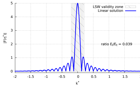
Figure 2.15: The blue line represents the modulus of \tilde{\eta}^* for v_p^* = 50 and \tau^* = 0 at t^* = T^* . The grey striped zone shows the domain of validity of the long wave approximation. Waves with wavenumbers outside of this zone are not taken into account properly in the SWE model.
