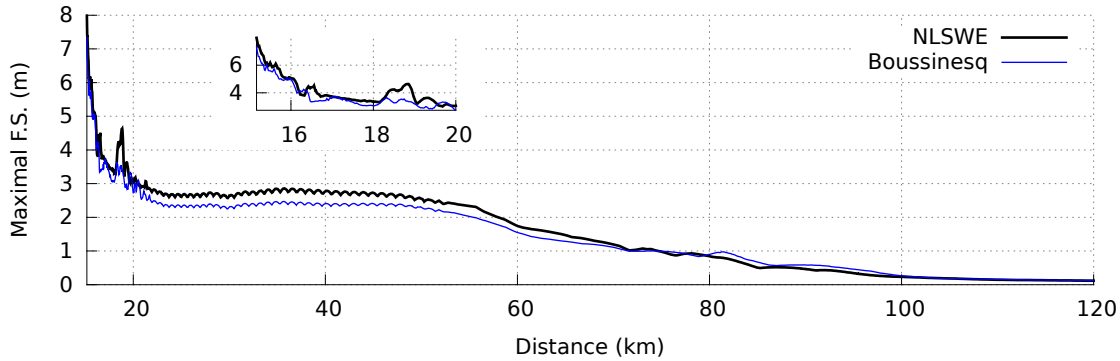
Figure 3.24: 1947 New Zealand event – Maximal free surface elevations reached during the propagation along the transect A - A' as defined in Figure 3.12. Only result for negative bathymetry is plotted. The black and blue line are the numerical results from the NLSWE and the Boussinesq models of Telemac2D, respectively. The model generation corresponds to v_p = 150m/s and t_r = 0s . The encapsulated figure is a zoom of the global curve near the coastline (distance \in [15; 23]km ).
