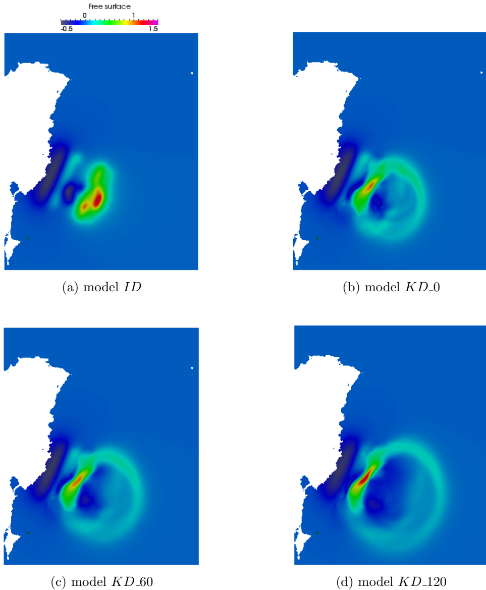
Figure 3.9: 1947 New Zealand event – Free surface deformation (in m) at the end of the ground motion for the four generation models calculated with the NLSWE model of Telemac2D. The indicated time corresponds to the time of end of ground motion varying between t = 0s for the instantaneous deformation to t = 310s for the generation with v_p = 300m/s and t_r = 120s .
