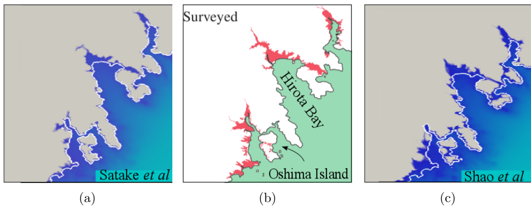
Figure 5.18: 2011 Tohoku-Oki event – Snapshots of the flooded area obtained by the numerical models in the South area of the bay of Iwate. Results in Figures 5.18a and 5.18c are obtained respectively from the model of Satake et al. [2013] and Shao et al. [2011]. Figure 5.18b is adapted of the work of Chen et al. [2014].
