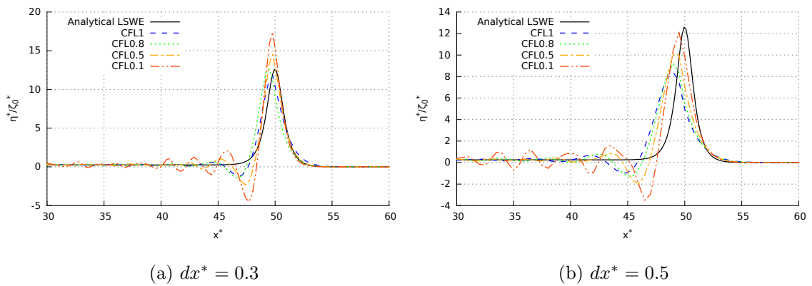
Figure 3.2: Resonance phenomenon simulated with Telemac2D and NLSWE – Spatial profiles of the free surface deformation at the end of the ground motion ( t^* = T^* ) for dx^* = 0.3 and dx^* = 0.5 meshes. The black line is the analytical free surface calculated from the LSWE theory. The coloured dashed curves are the different values of the CFL .
