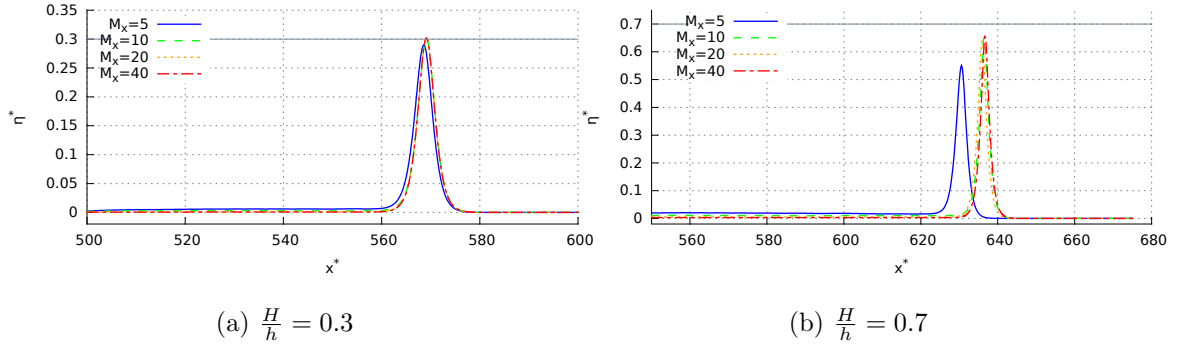
Figure 4.9: Propagation of a solitary wave – Same nomenclature as Figure 4.8 for \frac{H}{h} = 0.3 and 0.7
