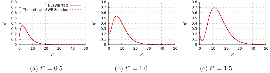
Figure 4.2: 1D analytical sliding mass – Comparisons of the spatial free surface profiles between the analytical solution (black line) and the numerical result from NLSWE Model of T2D (red line) at different times.
