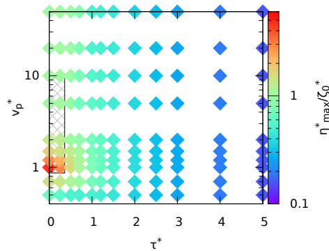
Figure 3.6: 1947 New Zealand event – Maximal amplitude of the free surface for L^* = 35 at t^* = T^* . Grey zone represents the ranges of values of the temporal parameters \tau^* and v_p^* of the 1947 New Zealand event. (see Table 3.2).
