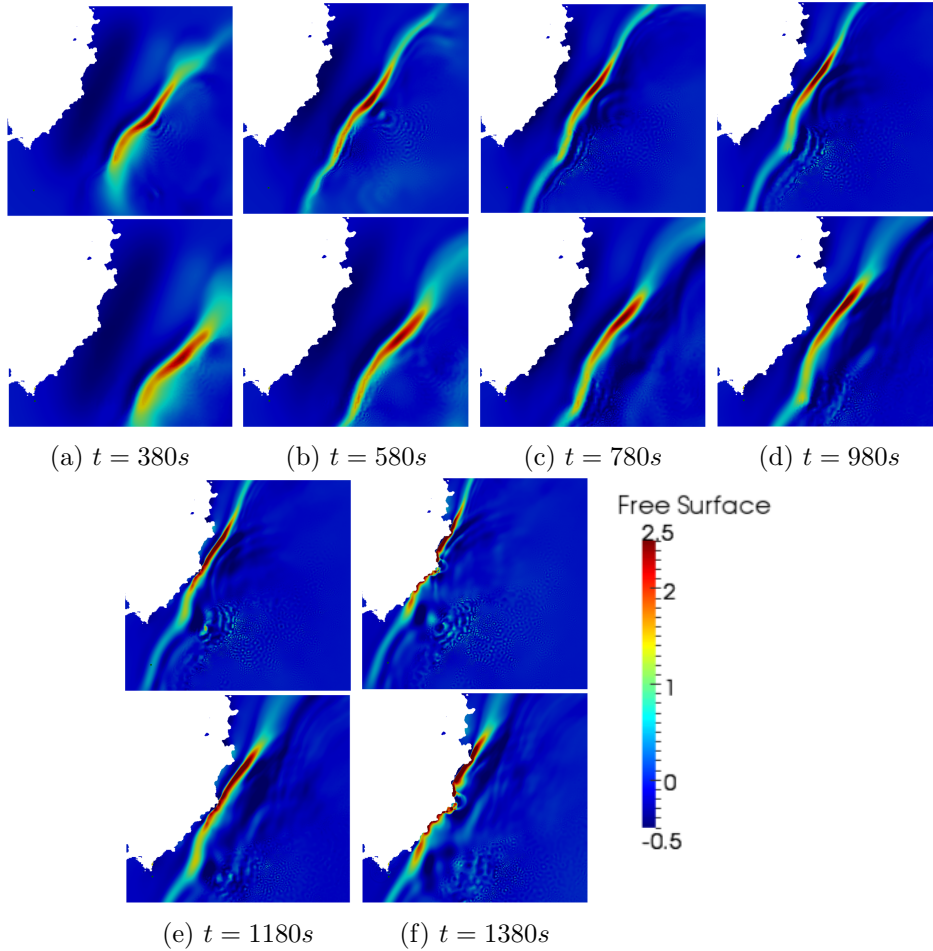
Figure 3.21: 1947 New Zealand event – Snapshots of the free surface deformation (in m) during the propagation for NLSWE model (up) and Boussinesq model (down) of Telemac2D for v_p = 150m/s and t_r = 0s .
