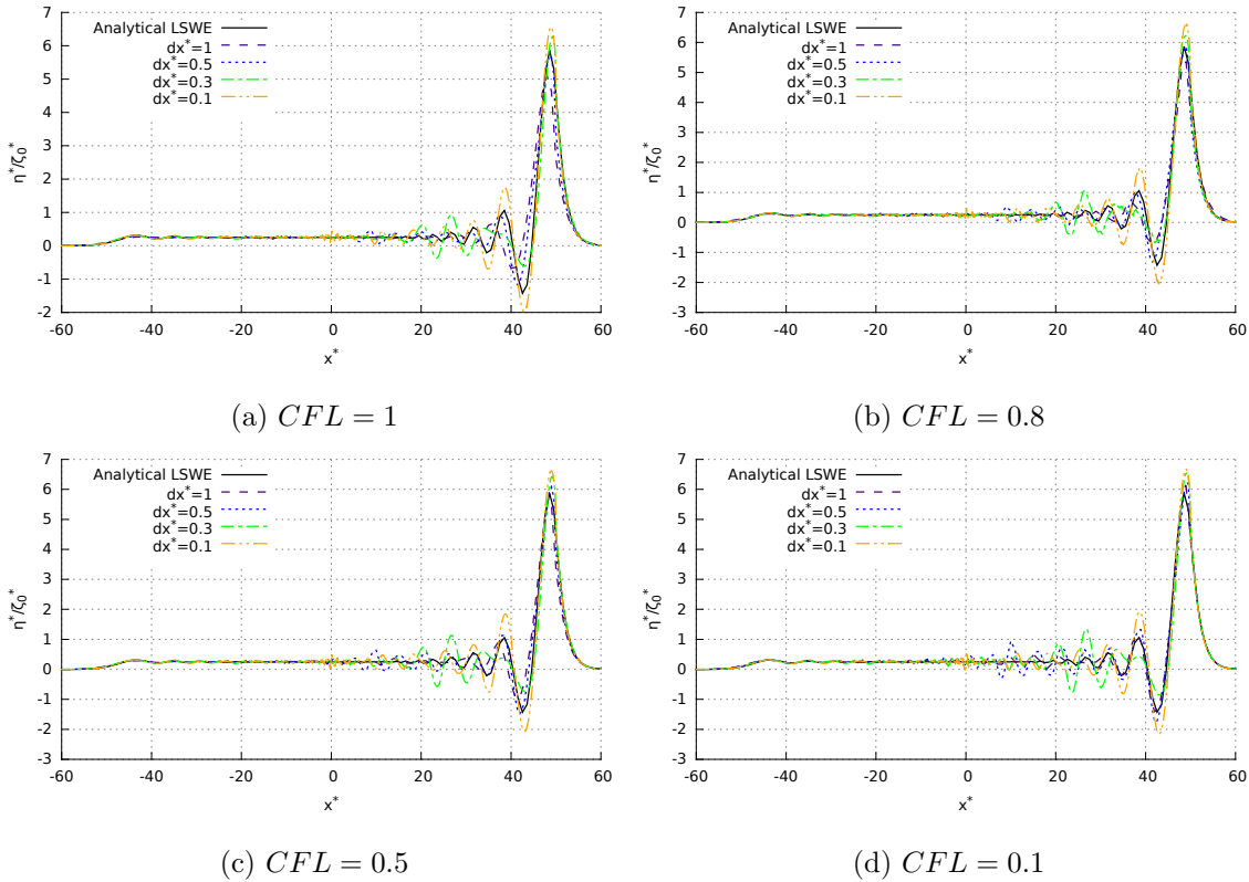
Figure 3.3: Resonance phenomenon simulated with Telemac2D and Boussinesq model – Spatial profiles of the free surface deformation at the end of the ground motion ( t^* = T^* with an accuracy of dt^* ) for different values of CFL and dx^* . The black line is the analytical free surface calculated from the linear theory. The coloured dashed curves represent numerical free surface profiles calculated with the different meshes.
