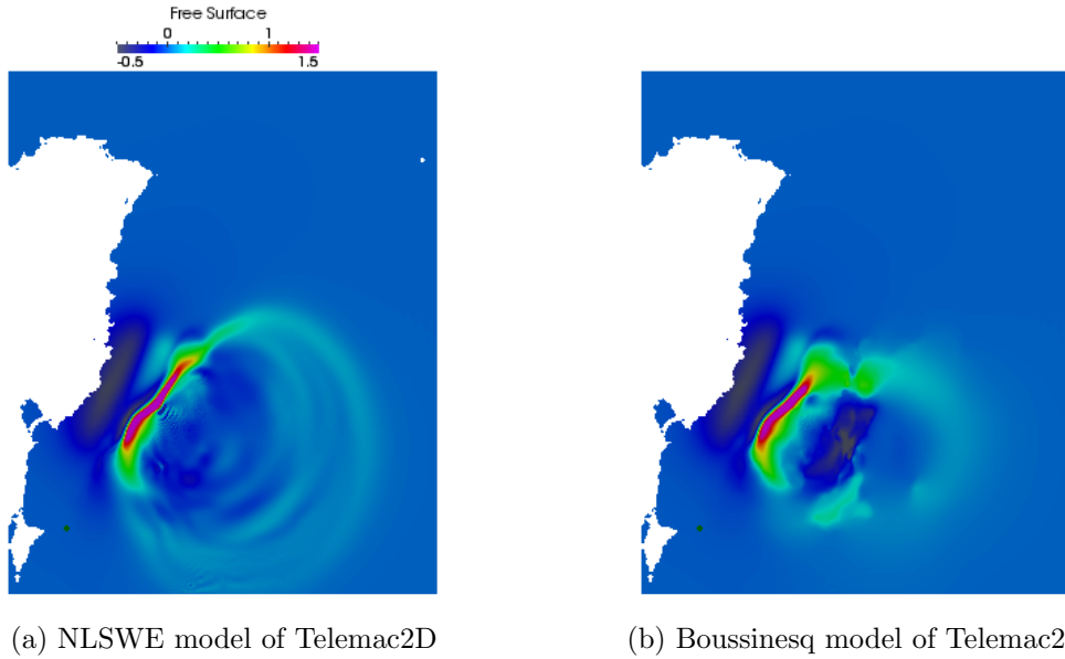
Figure 3.20: 1947 New Zealand event – Snapshots of the free surface elevation (in m) at the end of the generation ( t = 380s ) with the NLSWE and the Boussinesq models of Telemac2D for v_p = 150m/s and t_r = 0s . Same scale as Figure 3.9.
