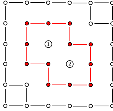
Figure 4.: The connectivity paradox using 4-adjacency
