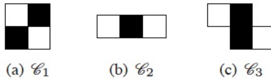
Figure 31.: Forbidden pattern in regular images [135]
