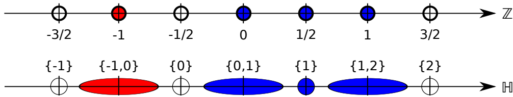
Figure 2.: Bijection between \mathbb{H}^1 and (\mathbb{Z}/2)
