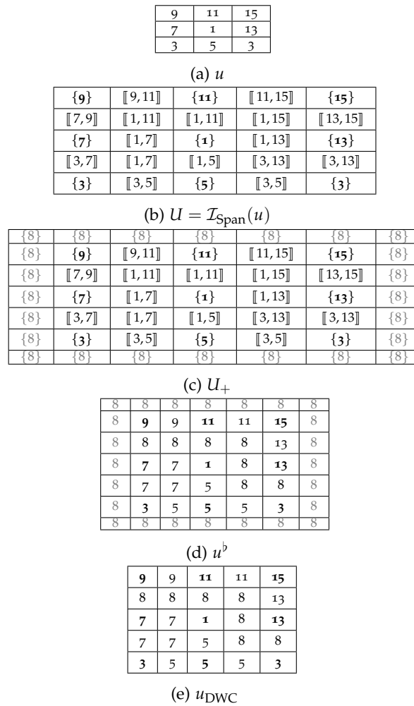
Figure 24.: The complete process in detail
