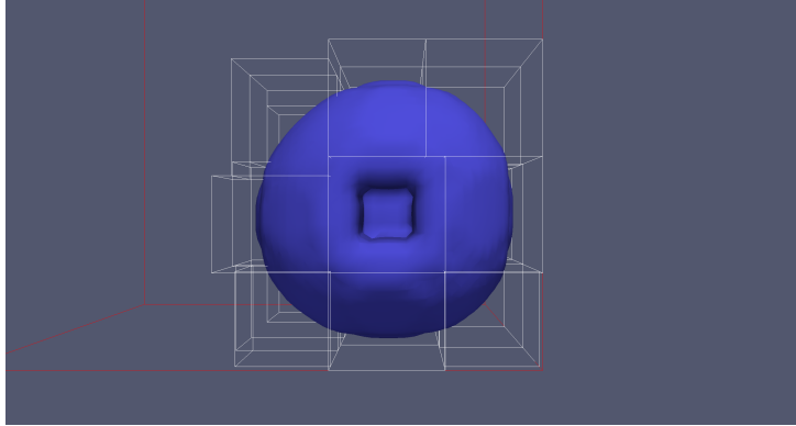
Figure 4.17 – Y field at t = 3.046 , 3D case: zoom on a corner of \Omega
