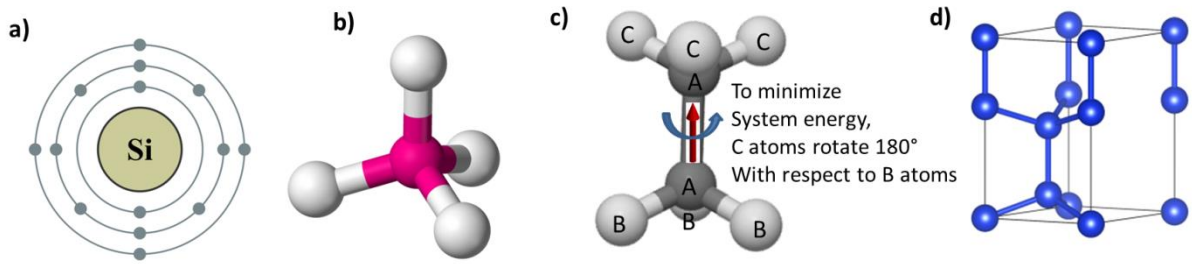
Figure 3.23. a) Si atom with electron orbitals. b) A tetrahedron formed by 5 Si atoms. c) Two tetrahedrons formed by 8 Si atoms, they share the two A atoms. The positions of the C atoms rotate 180^\circ along AA axis with respect to B atoms. d) Similar structure with c), but there is no 180^\circ rotation along AA axis.
