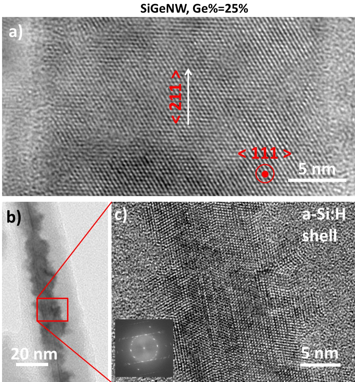
Figure 4.21. High resolution TEM image of SiGeNWs catalyzed by Sn. a) HRTEM image of a SiGeNW. b) HRTEM image of another SiGeNW. c) Zoom of the area indicated in b), with the FFT shown in the inset.
