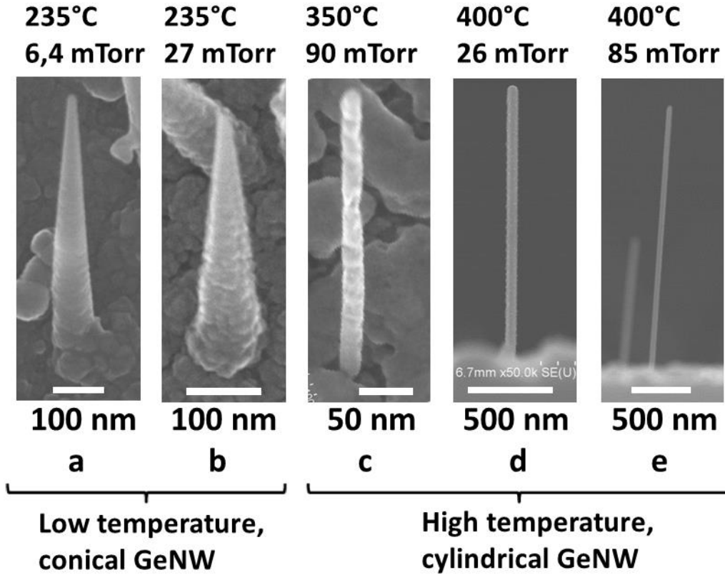
Figure 4.10. GeNWs grown by plasma-assisted VLS method at different temperatures and GeH 4 partial pressures. a) 235°C, 6.4 mTorr; b) 235°C, 27 mTorr; c) 350°C, 90 mTorr; d) 400°C, 26mTorr; and e) 400°C, 85 mTorr. The catalyst is In.
