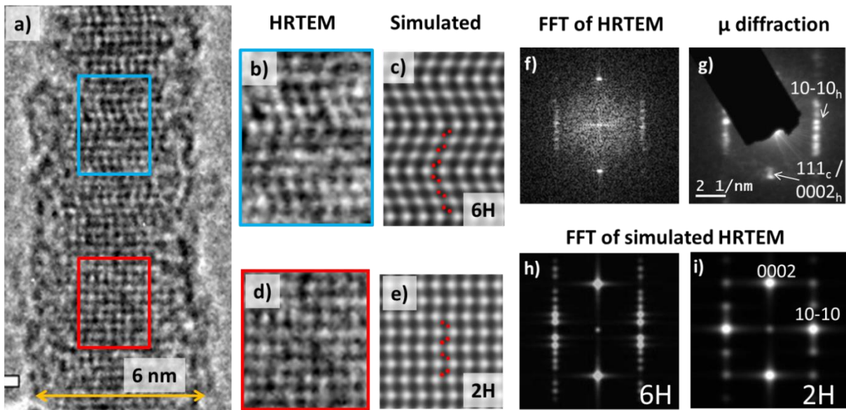
Figure 3.28. TEM characterization results of a hexagonal SiNW. a) High resolution TEM images of the SiNWs in a [11\bar{2}0]_H/[110]_C zone axis. b) and d) are the zoom of the indicated area. c) and e) are simulated 6H and 2H Si HRTEM image, respectively. f) FFT of the HRTEM image shown in a). g) Micro diffraction pattern of the NW in a). h) FFT of the simulated 6H Si HRTEM image. i) FFT of the simulated 2H Si HRTEM image.
