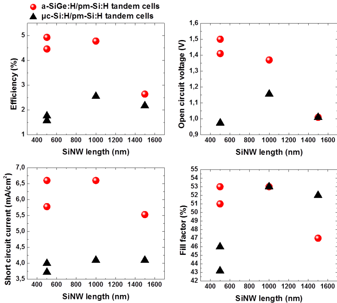
Figure 5.12. Efficiency, V_{oc} , J_{sc} and FF of the tandem solar cells as a function of NW core length. The red circles represent the a-SiGe:H/pm-Si:H tandem solar cells and the black triangles represent the \mu c-Si:H/pm-Si:H cells.
