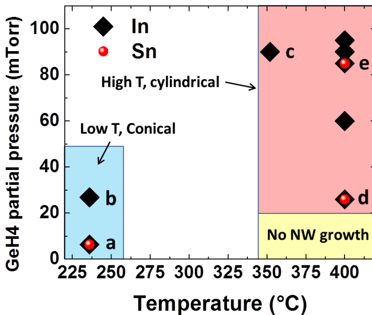
Figure 4.11. GeH 4 partial pressure and the substrate temperature of the GeNW growth experiments. Note the changing in shape from conical to cylindrical with the increase of substrate temperature.
