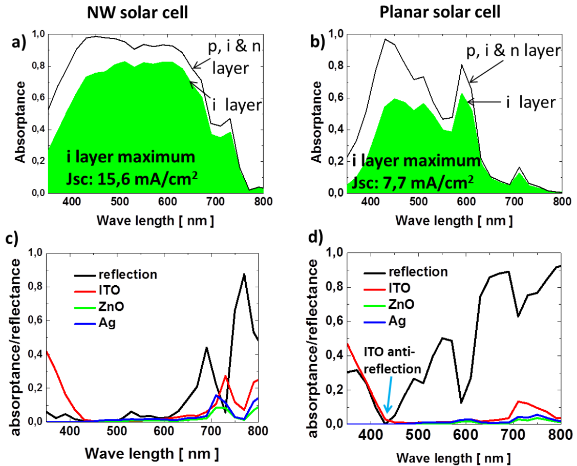
Figure 2.12. Absorbance as a function of wavelength in different layers of a) NW and b) planar solar cells. The black curve shows the sum of p i and n-layers, while the green part shows the absorption in the i-layer. c)-d) Absorbance in ITO, ZnO and Ag layers, together with the reflectance shown in black curve: c) in NW solar cell, d) in planar solar cell.
