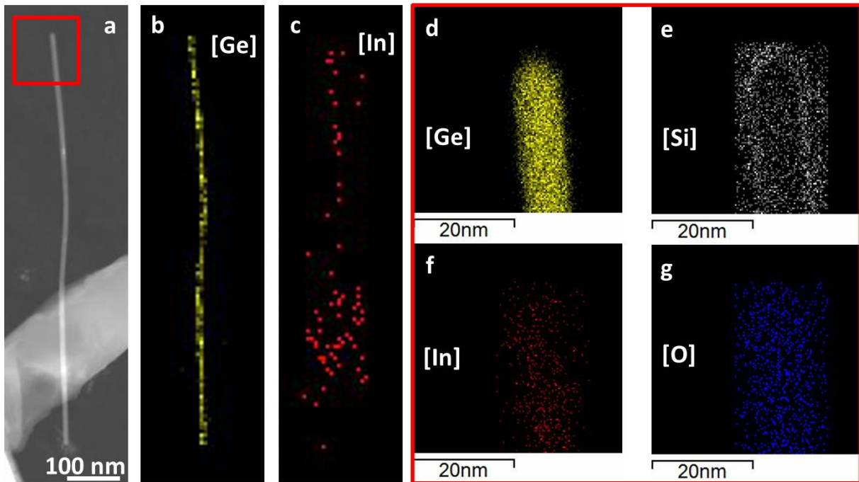
Figure 4.23. STEM-EDX study of a In catalyzed GeNW grown at 400°C. a) High Angle Annular Dark Field (HAADF) image of a GeNW. b) Ge map of the GeNW shown in a). c) In map of the GeNW shown in a). d)-e) Ge, Si, In and O maps of the area indicated by the red frame in a).
