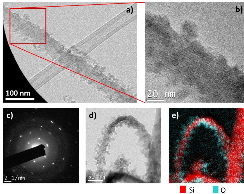
Figure 3.18. TEM characterization of a SiNW after H 2 plasma etching. a) Bright field image of the NW. b) HRTEM image of the region indicated by the red box in a). c) Diffraction pattern of the NW shown in a). d) Bright field image of another NW. e) Si and O map of the NW shown in d).
