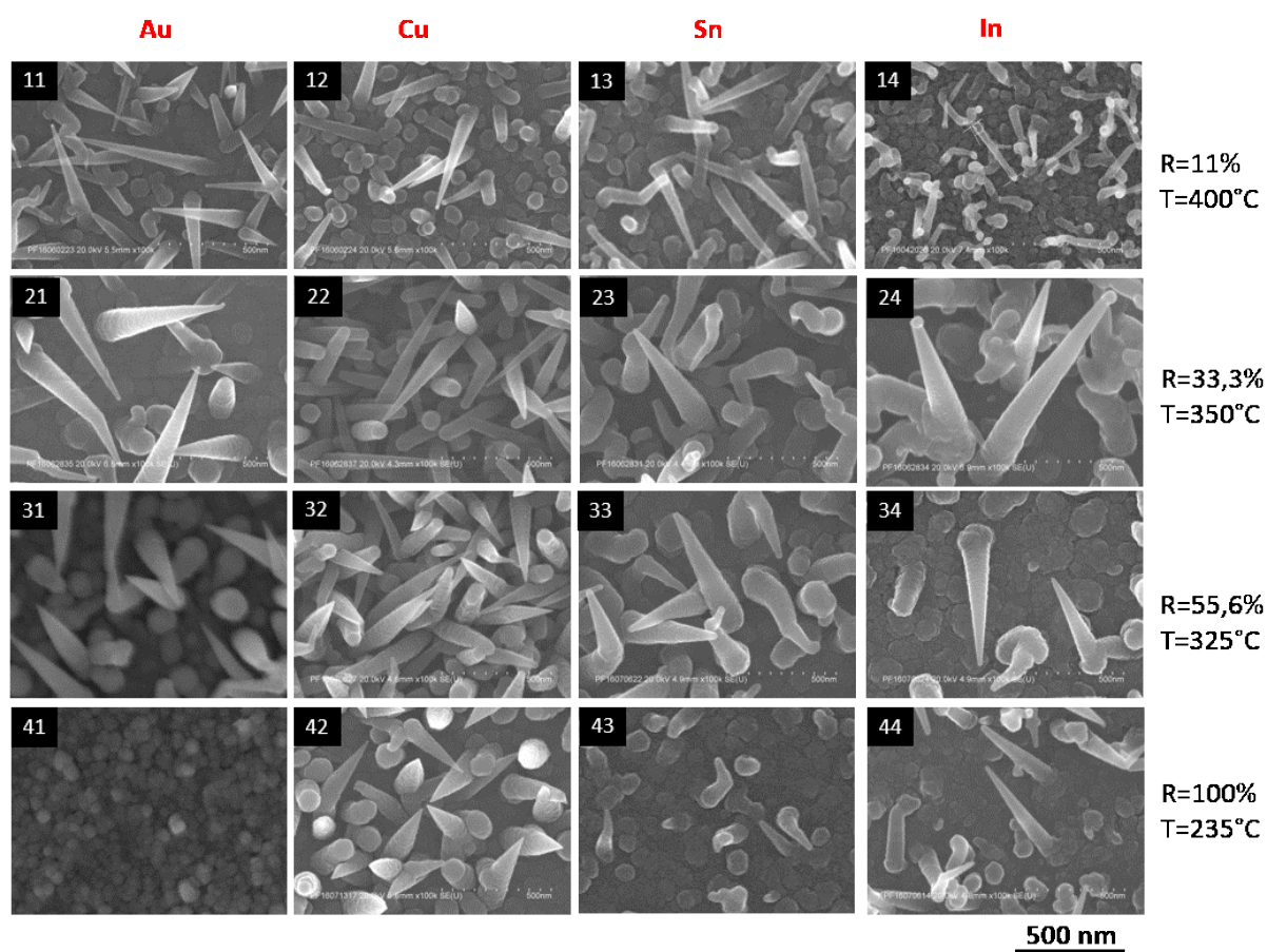
Figure 4.6. Top view of SiGeNWs catalyzed by Au, Cu, Sn and In. From 11 to 14, the \text{GeH}_4/(\text{GeH}_4+\text{SiH}_4) partial pressure ratio is 11%, and the substrate temperature is 400^\circ\text{C} . From 21 to 24, the \text{GeH}_4/(\text{GeH}_4+\text{SiH}_4) partial pressure ratio is 33.3%, and the substrate temperature is 350^\circ\text{C} . From 31 to 34, the \text{GeH}_4/(\text{GeH}_4+\text{SiH}_4) partial pressure ratio is 55.6%, and the substrate temperature is 325^\circ\text{C} . From 41 to 44, the \text{GeH}_4/(\text{GeH}_4+\text{SiH}_4) partial pressure ratio is 100%, and the substrate temperature is 235^\circ\text{C} .
