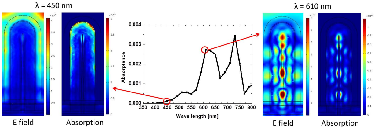
Figure 2.13. Absorbance by the SiNW core inside the NW solar cell. The E field and absorption maps at 450 nm and 610 nm wavelength are shown on the left and right, respectively.
