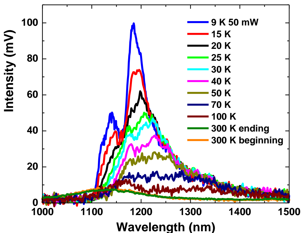
Figure 4.24. Photoluminescence signal of a SiGeNW (Ge content \sim 14\% ) sample measured at different temperatures.
