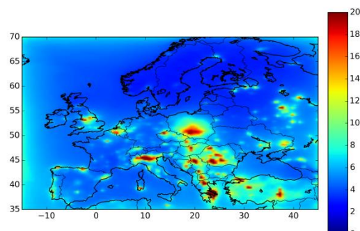
Figure 7-54. Annual average ambient concentration of \text{Hg}_p [ \text{pg.m}^{-3} ] at the surface.
