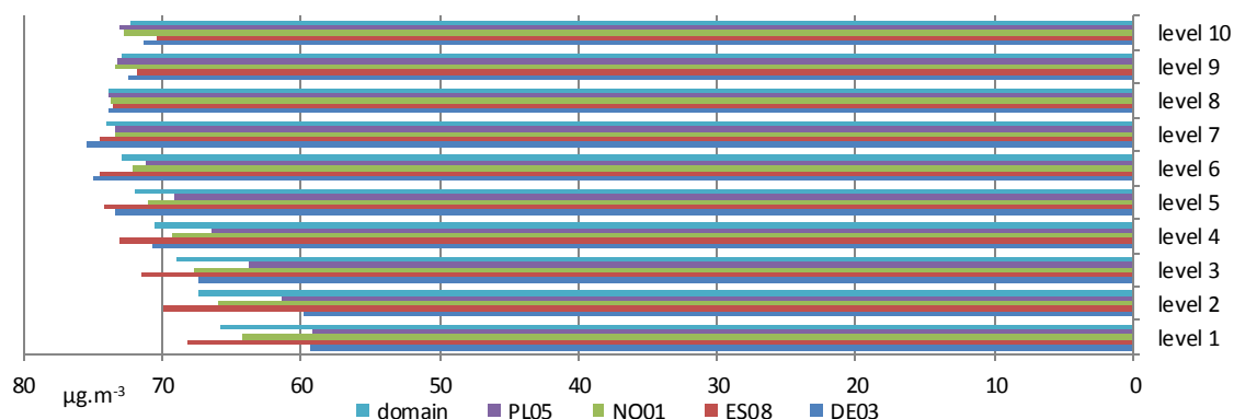
Figure 7-12. Annual average concentrations of O_{3(g)} [ \mu\text{g.m}^{-3} ] at 10 vertical levels.
