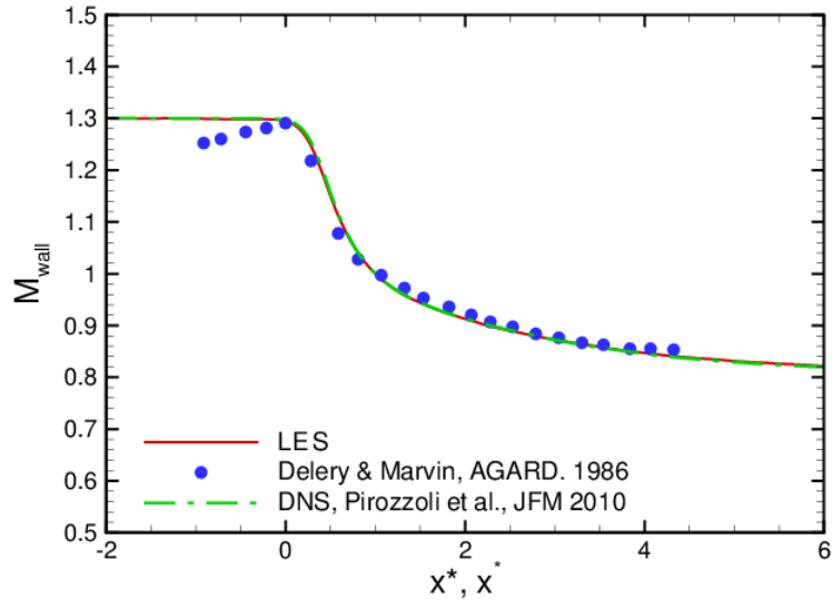
Figure 4.8: Isentropic wall Mach number for the transonic shock-wave turbulent boundary layer interaction at M_\infty = 1.3 and Re_{\theta_{in}} = 750 .
