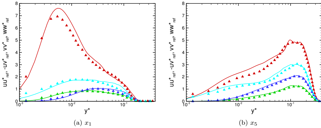
Figure 4.14: Reynolds stresses for the transonic shock-wave turbulent boundary layer interaction at M_\infty = 1.3 and Re_{\theta_{in}} = 750 . Red curve, uu^* , blue curve vv^* , cyan curve ww^* and green curve uv^* . Lines, current LES; symbols, DNS of Ref. [76]
