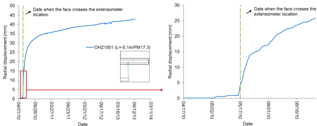
Fig. 2. 15. Radial displacement in GCS drift obtained from extensometer data (L - distance to GCS wall)
