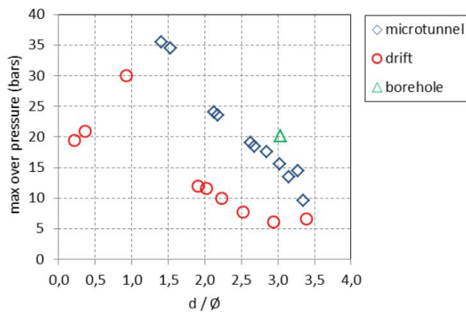
Fig. B. 5. Maximum over-pressure measured at the wall side of different diameter openings: drift of 5 m diameter, micro tunnel of 0.7 m diameter and borehole of 0.15 m diameter (d: distance to the wall, φ diameter of the drift). (Fig. 11 from Armand et al. 2015b)
