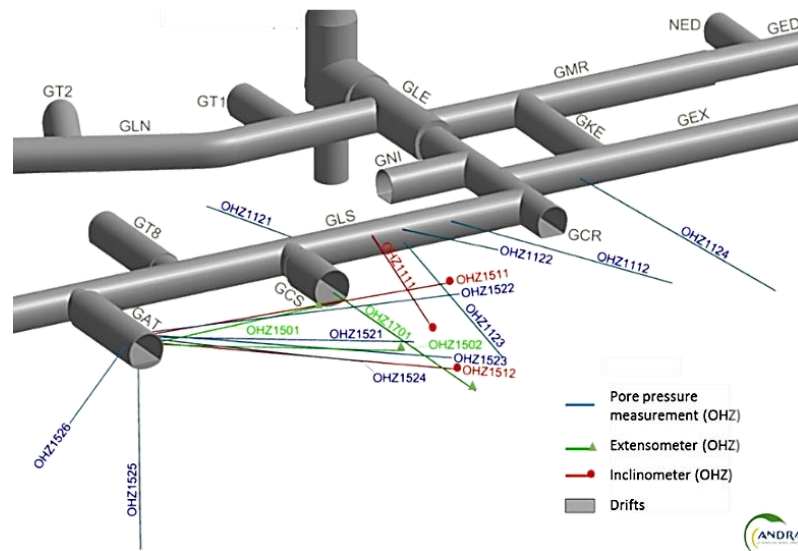
Fig. 1. 12. Instrumentation of mine-by experiment (Armand et al. 2011)
