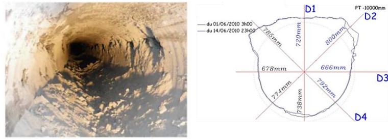
Fig. 2. 6. State of the ALC1603 micro-tunnel wall (adapted from Morel et al. 2013). At left: Photo after the end of excavation. At right: typical profile of the micro-tunnel wall after excavation
